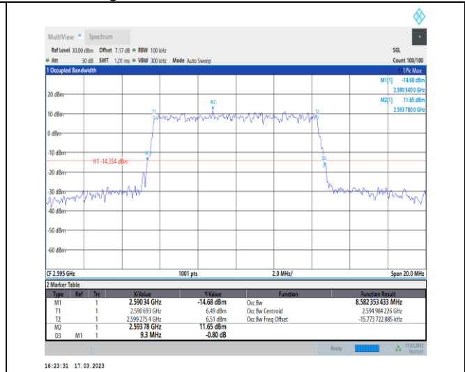
1-N38-30-10-M-5-DFT-256QAM-Outer_Full-24@0-A nt1-8.582-9.300-≤10-PASS
