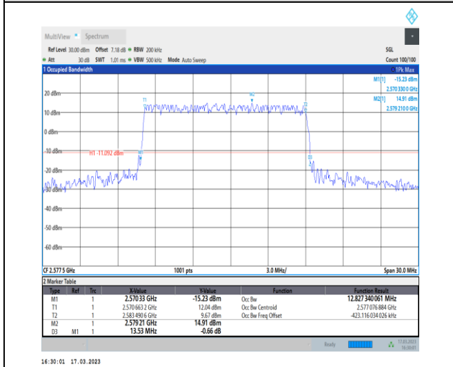
1-N38-30-15-L-4-DFT-64QAM-Outer_Full-36@0-Ant 1-12.827-13.530-≤15-PASS
