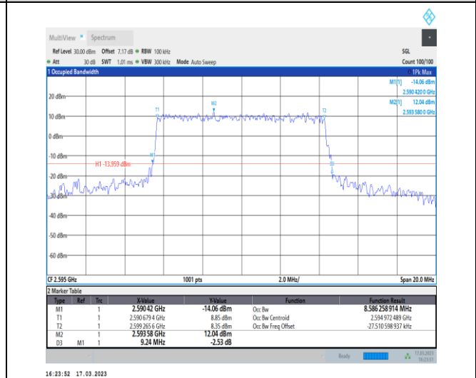
1-N38-30-10-M-7-CP-16QAM-Outer_Full-24@0-Ant1 -8.586-9.240-≤10-PASS
