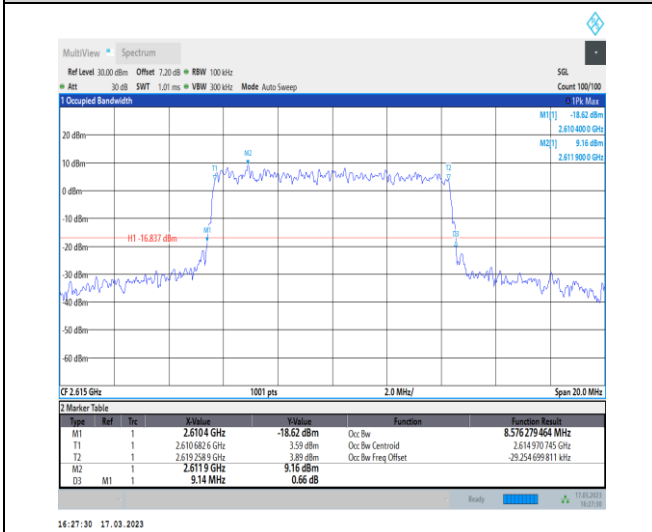
1-N38-30-10-H-9-CP-256QAM-Outer_Full-24@0-Ant 1-8.576-9.140-≤10-PASS
