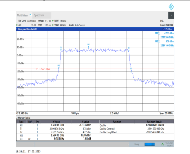
1-N38-30-10-M-9-CP-256QAM-Outer_Full-24@0-Ant 1-8.588-9.180-≤10-PASS
