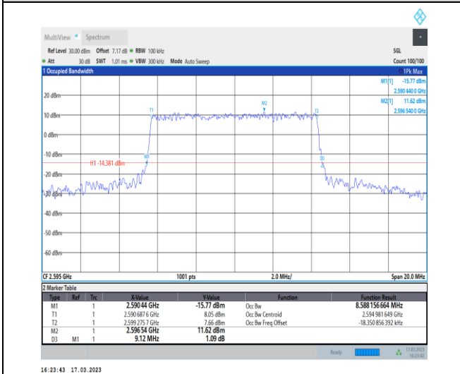
1-N38-30-10-M-6-CP-QPSK-Outer_Full-24@0-Ant1 8.588-9.120-≤10-PASS
