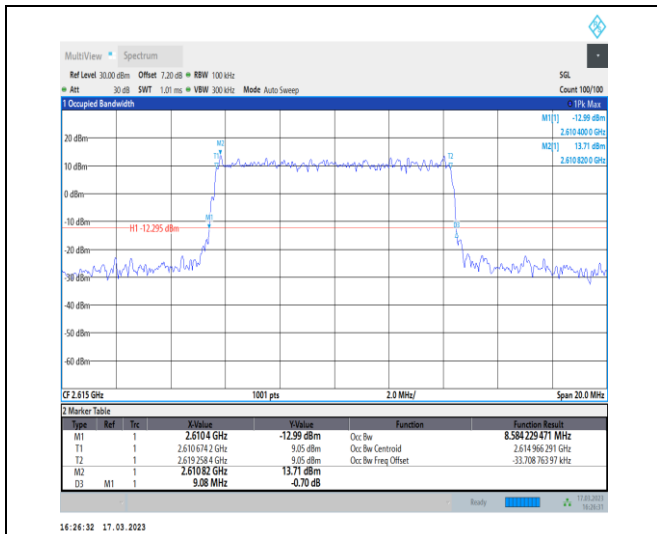
1-N38-30-10-H-3-DFT-16QAM-Outer_Full-24@0-Ant 1-8.584-9.080-≤10-PASS
