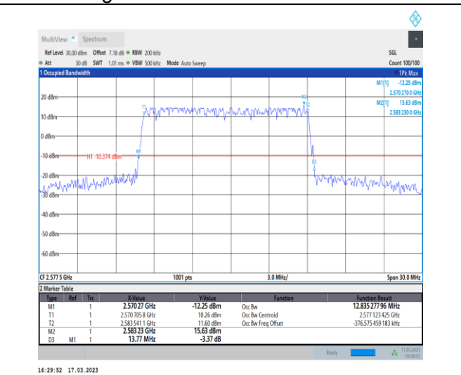
1-N38-30-15-L-3-DFT-16QAM-Outer_Full-36@0-Ant 1-12.835-13.770-≤15-PASS
