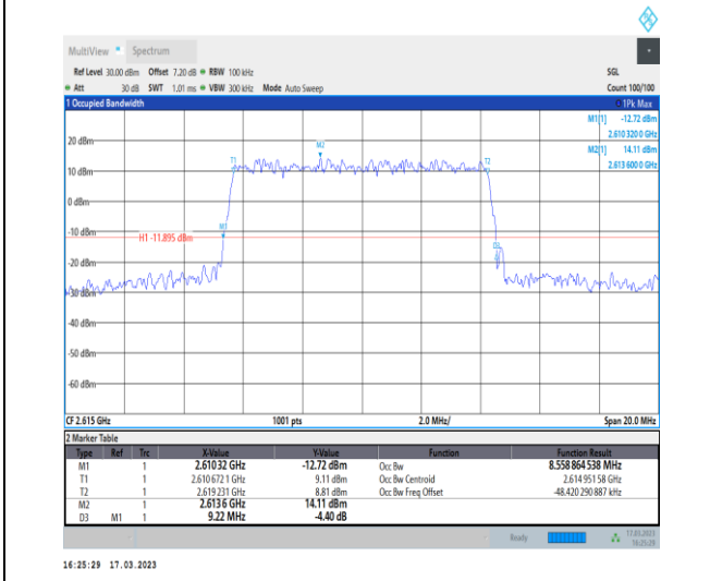
1-N38-30-10-H-1-DFT-QPSK-Outer_Full-24@0-Ant1 -8.559-9.220-≤10-PASS
