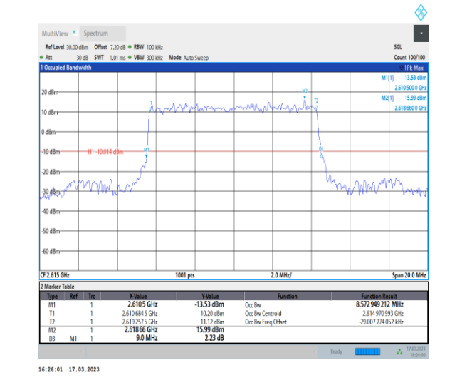
1-N38-30-10-H-2-DFT-PI2BPSK-Outer_Full-24@0-A nt1-8.573-9.000-≤10-PASS
