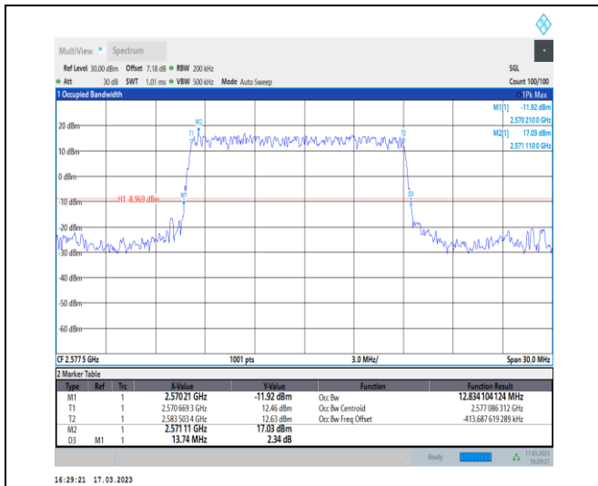
1-N38-30-15-L-2-DFT-PI2BPSK-Outer_Full-36@0-A nt1-12.834-13.740-≤15-PASS
