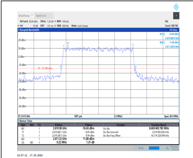
1-N38-30-10-H-7-CP-16QAM-Outer_Full-24@0-Ant1 -8.603-9.220-≤10-PASS
