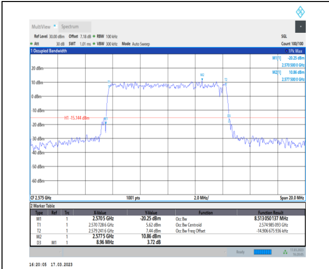
1-N38-30-10-L-5-DFT-256QAM-Outer_Full-24@0-An t1-8.513-8.960-≤10-PASS
