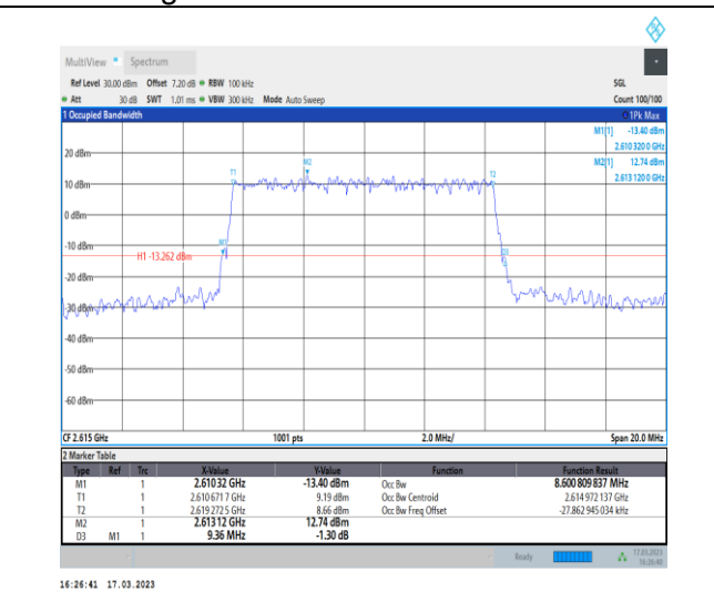
1-N38-30-10-H-4-DFT-64QAM-Outer_Full-24@0-Ant 1-8.601-9.360-≤10-PASS
