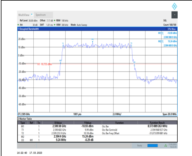
1-N38-30-10-M-2-DFT-PI2BPSK-Outer_Full-24@0-A nt1-8.574-9.240≤10-PASS
