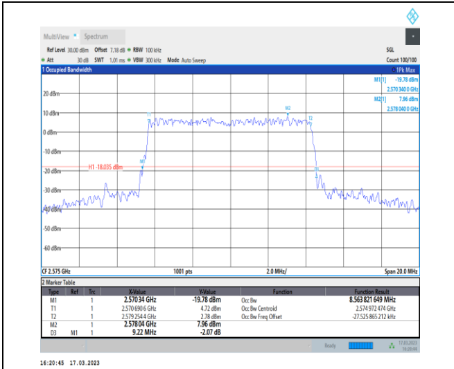
1-N38-30-10-L-9-CP-256QAM-Outer_Full-24@0-Ant 1-8.564-9.220≤10-PASS
