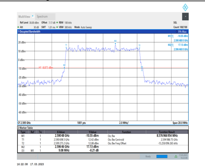
1-N38-30-10-M-1-DFT-QPSK-Outer_Full-24@0-Ant1 -8.577-9.080≤10-PASS
