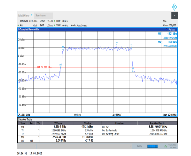
1-N38-30-10-M-8-CP-64QAM-Outer_Full-24@0-Ant 1-8.581-9.040-≤10-PASS
