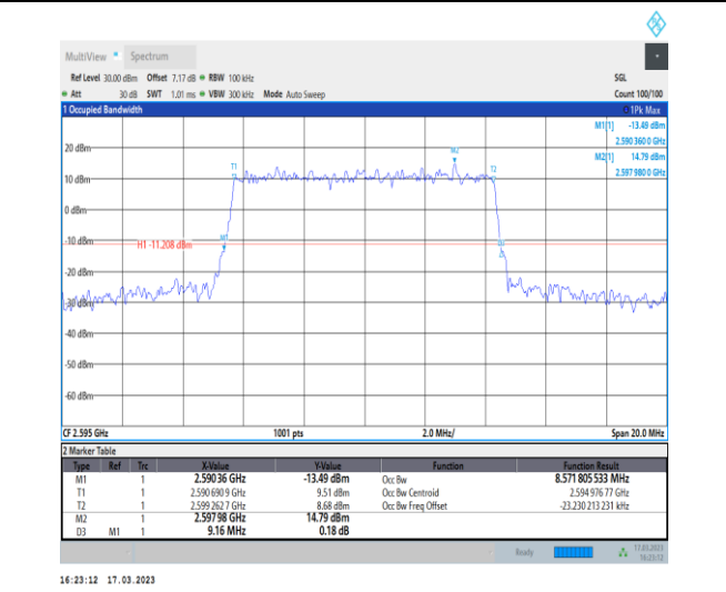
1-N38-30-10-M-3-DFT-16QAM-Outer_Full-24@0-Ant 1-8.572-9.160≤10-PASS
