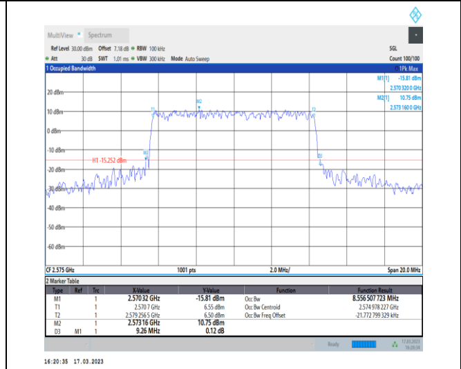
1-N38-30-10-L-8-CP-64QAM-Outer_Full-24@0-Ant1-8.557-9.260-≤10-PASS
