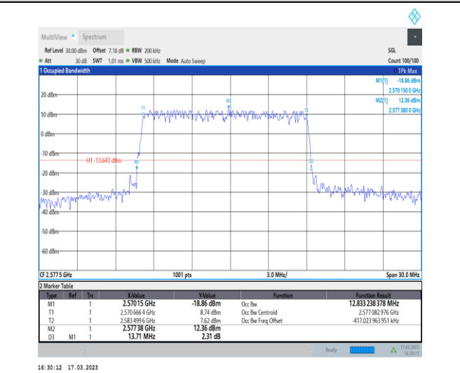
1-N38-30-15-L-5-DFT-256QAM-Outer_Full-36@0-Ant t1-12.833-13.710-≤15-PASS
