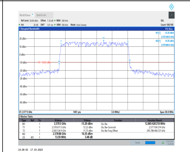
1-N38-30-15-L-1-DFT-QPSK-Outer_Full-36@0-Ant1 12.865-13.590-≤15-PASS
