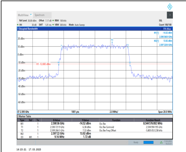
1-N38-30-10-M-4-DFT-64QAM-Outer_Full-24@0-Ant 1-8.545-9.160-≤10-PASS
