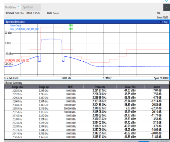
1-N30-PC3-15-10-L-6-CP-QPSK-Outer_Full-52@0-Ant1-1--PASS-see graph
