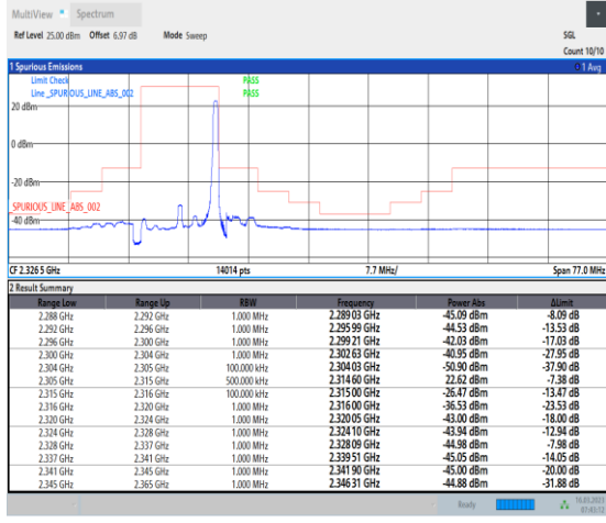
1-N30-PC3-15-10-H-2-DFT-PI2BPSK-Edge_1RB_Right-t-1@51-Ant1-1--PASS-see graph
