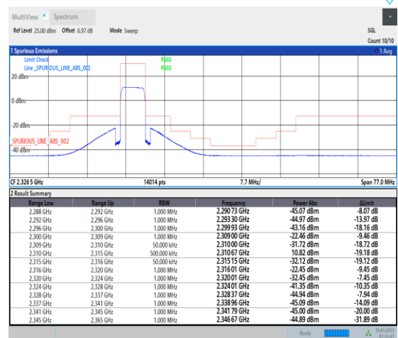
1-N30-PC3-15-5-H-6-CP-QPSK-Outer_Full-25@0-Ant1-1--PASS-see graph
