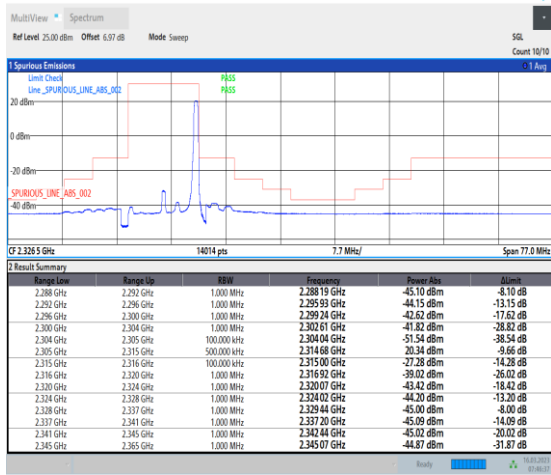
1-N30-PC3-15-10-H-5-CP-QPSK-Edge_1RB_Right-1@51-Ant1-1--PASS-see graph
