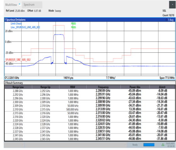
1-N30-PC3-15-5-H-3-DFT-PI2BPSK-Outer_Full-25@0-Ant1-1--PASS-see graph
