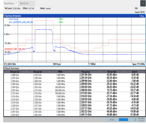
1-N30-PC3-15-10-H-3-DFT-PI2BPSK-Outer_Full-50@0-Ant1-1--PASS-see graph
