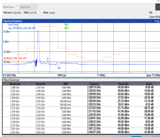
1-N30-PC3-15-10-L-4-CP-QPSK-Edge_1RB_Left-1@0-Ant1-1--PASS-see graph
