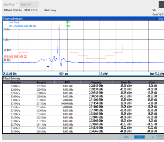
1-N30-PC3-15-5-H-2-DFT-PI2BPSK-Edge_1RB_Right-1@24-Ant1-1--PASS-see graph
