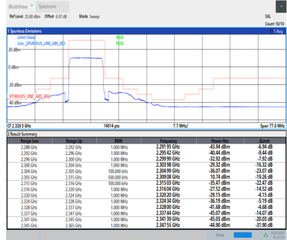
1-N30-PC3-15-10-L-3-DFT-PI2BPSK-Outer_Full-50@0-Ant1-1--PASS-see graph
