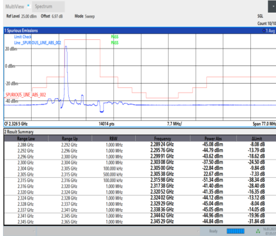
1-N30-PC3-15-10-L-1-DFT-PI2BPSK-Edge_1RB_Left-1@0-Ant1-1--PASS-see graph
