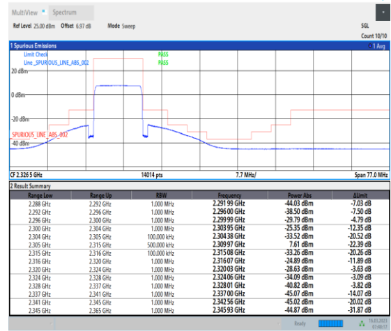
1-N30-PC3-15-10-H-6-CP-QPSK-Outer_Full-52@0-Ant1-1--PASS-see graph
