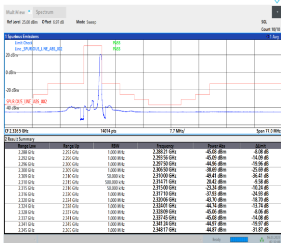
1-N30-PC3-15-5-H-5-CP-QPSK-Edge_1RB_Right-1@24-Ant1-1--PASS-see graph
