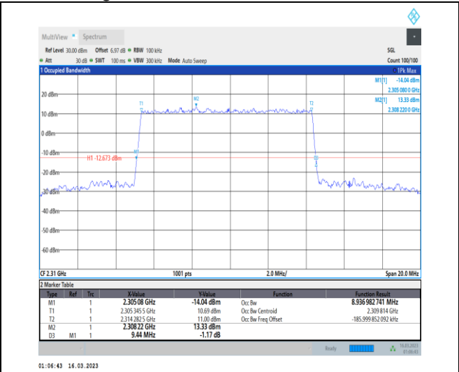
1-N30-PC3-15-10-H-1-DFT-QPSK-Outer_Full-50@ 0-Ant1-8.937-9.440-≤10-PASS
