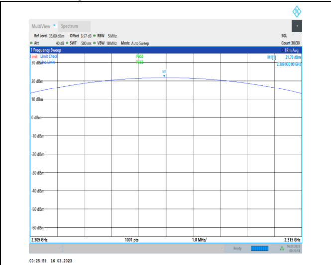
1-N30-PC3-15-5-M-3-DFT-PI2BPSK-Outer_Full-25@ 0-2305-2315-Ant1-2309.93-21.76-99-PASS
