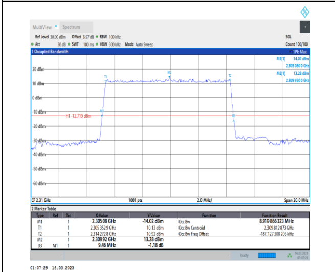
1-N30-PC3-15-10-H-2-DFT-PI2BPSK-Outer_Full-50 @0-Ant1-8.92-9.460-≤10-PASS
