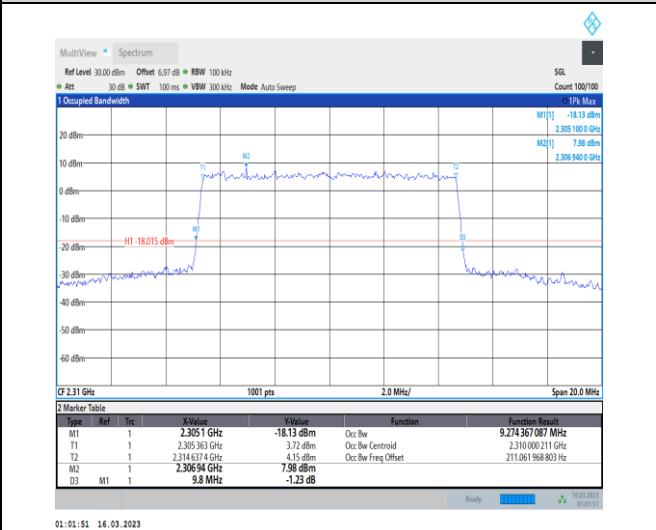
1-N30-PC3-15-10-L-9-CP-256QAM-Outer_Full-52@0- Ant1-9.274-9.800-≤10-PASS
