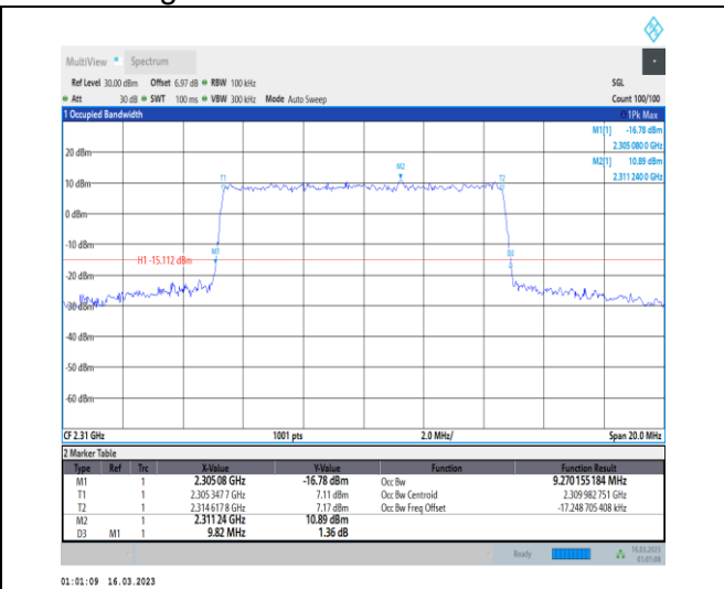
1-N30-PC3-15-10-L-7-CP-16QAM-Outer_Full-52@0- Ant1-9.27-9.820-≤10-PASS
