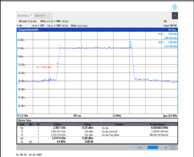
1-N30-PC3-15-10-H-3-DFT-16QAM-Outer_Full-50@ 0-Ant1-8.928-9.400-≤10-PASS
