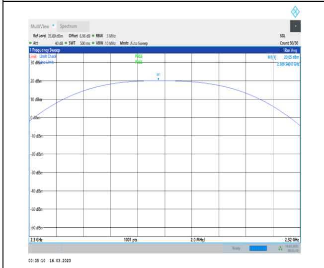
1-N30-PC3-15-10-M-3-DFT-PI2BPSK-Outer_Full-50 @0-2300-2320-Ant1-2309.54-20.05-99-PASS
