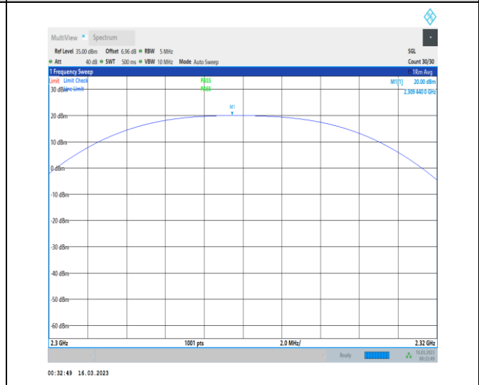
1-N30-PC3-15-10-L-3-DFT-PI2BPSK-Outer_Full-50 @0-2300-2320-Ant1-2309.44-20.00-99-PASS
