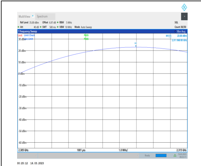
1-N30-PC3-15-5-M-2-DFT-PI2BPSK-Inner_1RB_Ri ght-1@23-2305-2315-Ant1-2311.96-23.00-99-PASS
