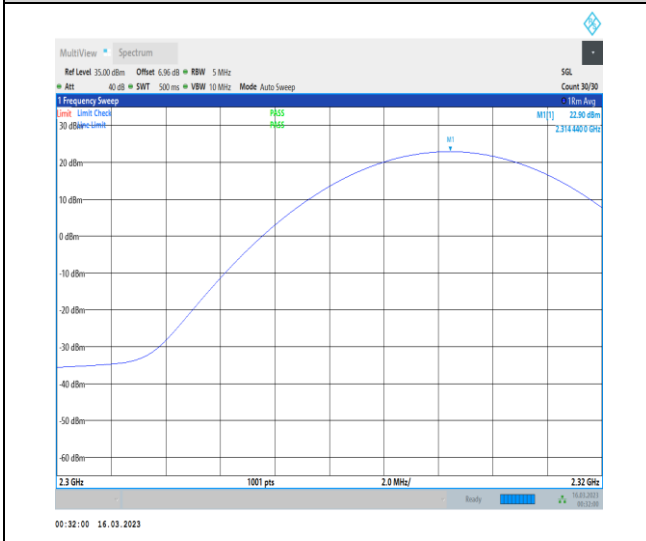
1-N30-PC3-15-10-L-2-DFT-PI2BPSK-Inner_1RB_Ri ght-1@50-2300-2320-Ant1-2314.44-22.90-99-PASS
