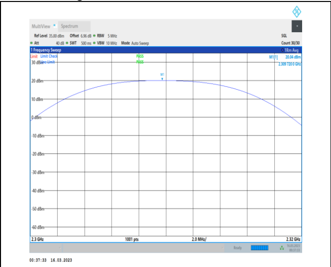
1-N30-PC3-15-10-H-3-DFT-PI2BPSK-Outer_Full-50 @0-2300-2320-Ant1-2309.72-20.04-99-PASS
