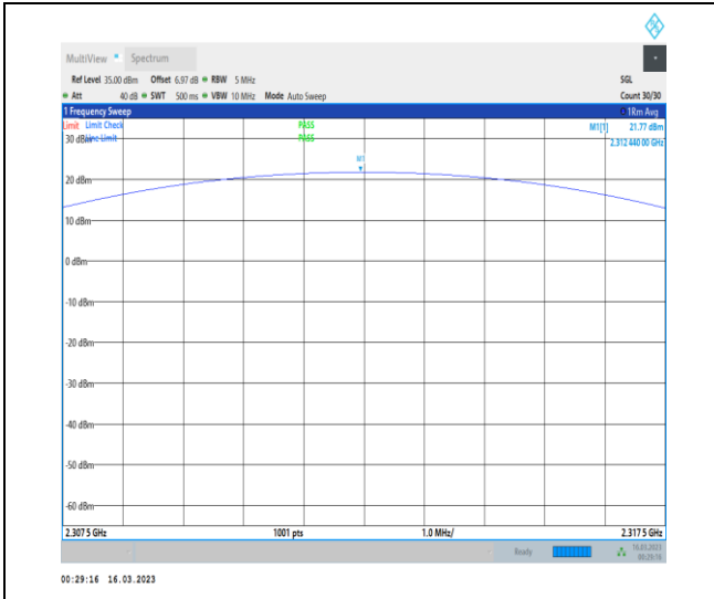
1-N30-PC3-15-5-H-3-DFT-PI2BPSK-Outer_Full-25 @0-2307.5-2317.5-Ant1-2312.44-21.77-99-PASS
