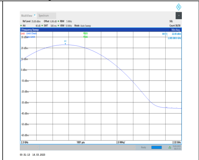
1-N30-PC3-15-10-L-1-DFT-PI2BPSK-Inner_1RB_Left -1@1-2300-2320-Ant1-2305.58-22.93-99-PASS
