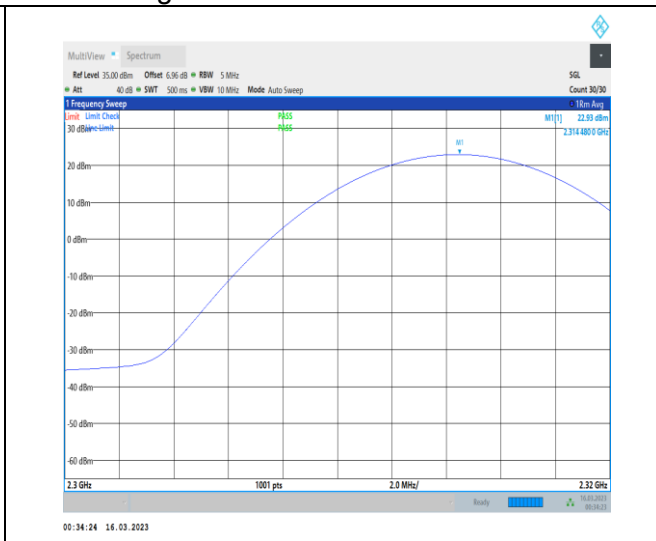
1-N30-PC3-15-10-M-2-DFT-PI2BPSK-Inner_1RB_Ri ght-1@50-2300-2320-Ant1-2314.48-22.93-99-PASS
