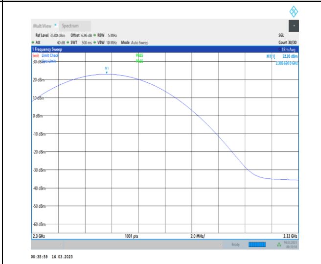
1-N30-PC3-15-10-H-1-DFT-PI2BPSK-Inner_1RB_Lef t-1@1-2300-2320-Ant1-2305.62-22.93-99-PASS
