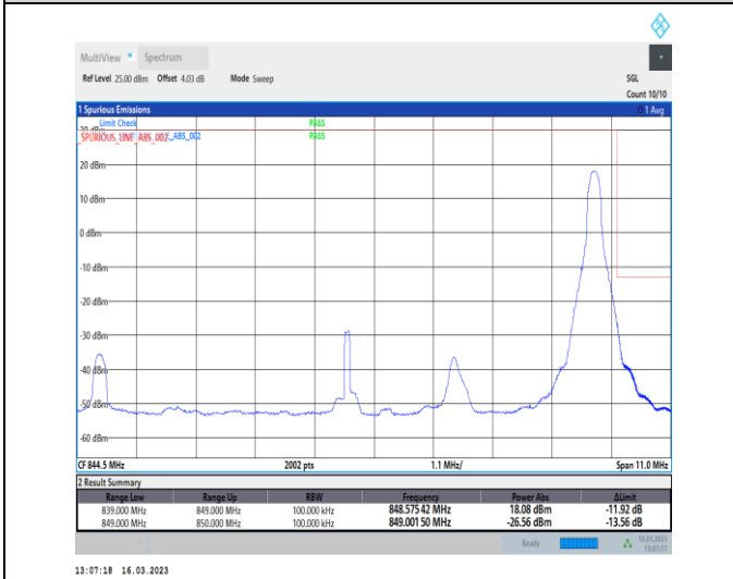
1-N26-824-849-PC3-15-10-H-5-CP-QPSK-Edge_1RB_Right-1@51-Ant1-1-seegraph-PASS-see graph
