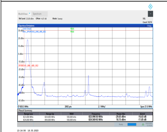
1-N26-824-849-PC3-15-20-L-4-CP-QPSK-Edge_1RB_Left-1@0-Ant1-1-seegraph-PASS-see graph
