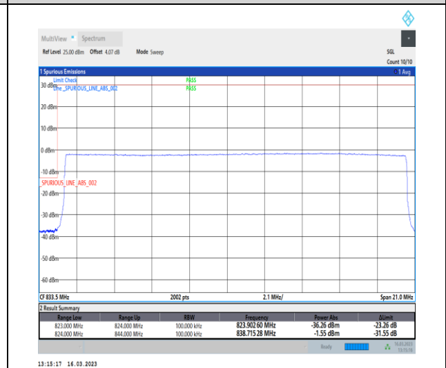
1-N26-824-849-PC3-15-20-L-6-CP-QPSK-Outer_Full-106@0-Ant1-1-seegraph-PASS-see graph
