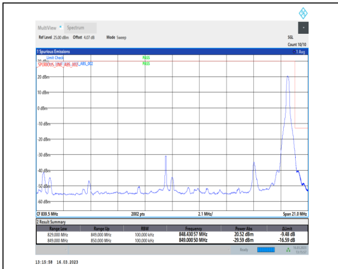
1-N26-824-849-PC3-15-20-H-2-DFT-PI2BPSK-Edge_1_RB_Right-1@105-Ant1-1-seegraph-PASS-see graph
