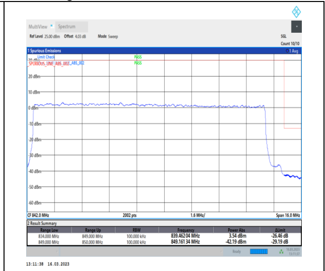
1-N26-824-849-PC3-15-15-H-3-DFT-PI2BPSK-Outer_Full-75@0-Ant1-1-seegraph-PASS-see graph
