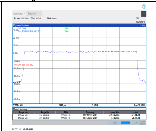
1-N26-824-849-PC3-15-15-L-3-DFT-PI2BPSK-Outer_Full-75@0-Ant1-1-seegraph-PASS-see graph
