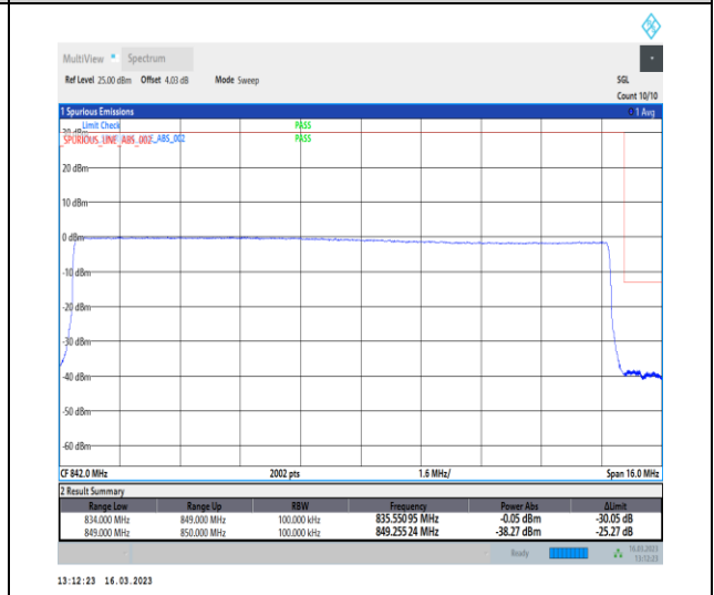
1-N26-824-849-PC3-15-15-H-6-CP-QPSK-Outer_Full-79@0-Ant1-1-seegraph-PASS-see graph
