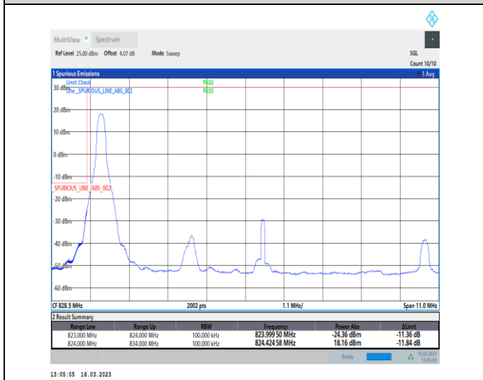
1-N26-824-849-PC3-15-10-L-4-CP-QPSK-Edge_1RB_Left-1@0-Ant1-1-seegraph-PASS-see graph
