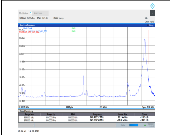
1-N26-824-849-PC3-15-20-H-5-CP-QPSK-Edge_1RB_Right-1@105-Ant1-1-seegraph-PASS-see graph
