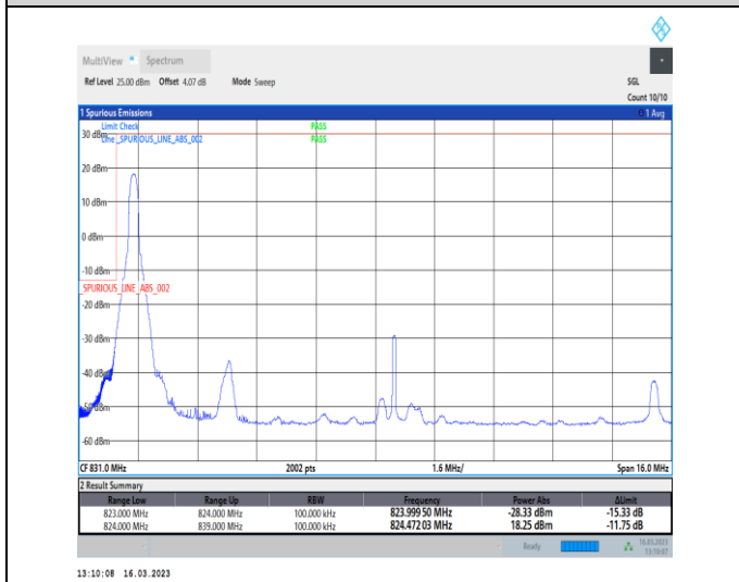
1-N26-824-849-PC3-15-15-L-4-CP-QPSK-Edge_1RB_Left-1@0-Ant1-1-seegraph-PASS-see graph
