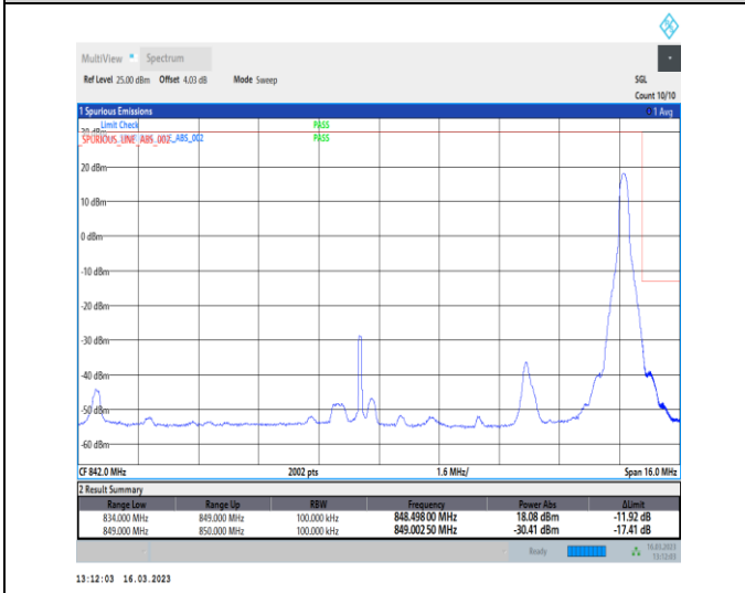
1-N26-824-849-PC3-15-15-H-5-CP-QPSK-Edge_1RB_Right-1@78-Ant1-1-seegraph-PASS-see graph
