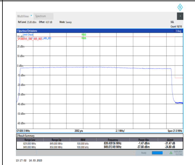
1-N26-824-849-PC3-15-20-H-6-CP-QPSK-Outer_Full-106@0-Ant1-1-seegraph-PASS-see graph
