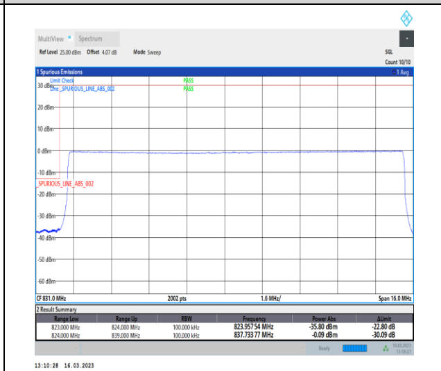
1-N26-824-849-PC3-15-15-L-6-CP-QPSK-Outer_Full-79@0-Ant1-1-seegraph-PASS-see graph
