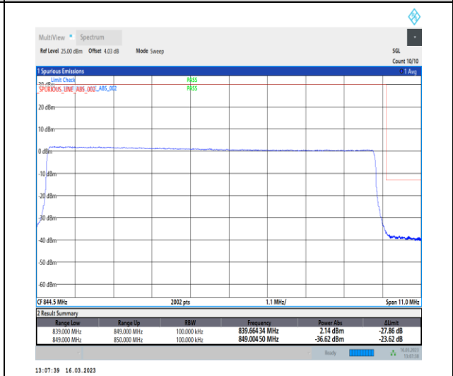
1-N26-824-849-PC3-15-10-H-6-CP-QPSK-Outer_Full-52@0-Ant1-1-seegraph-PASS-see graph
