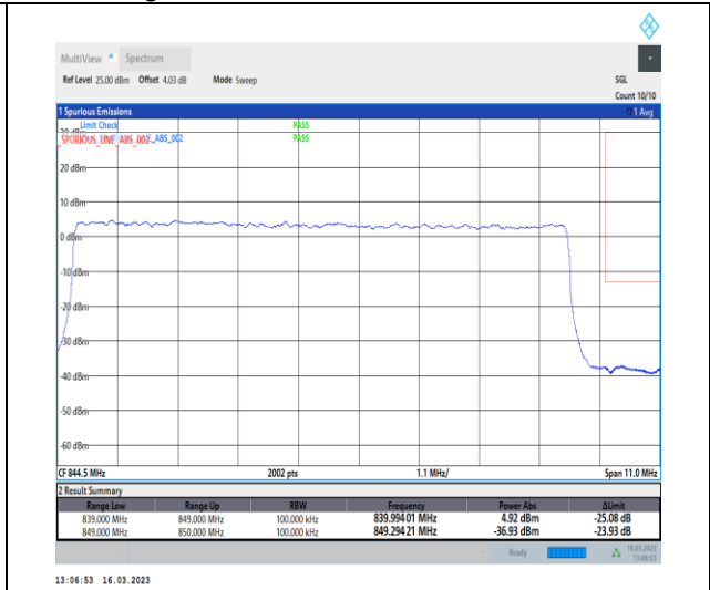
1-N26-824-849-PC3-15-10-H-3-DFT-PI2BPSK-Outer_Full-50@0-Ant1-1-seegraph-PASS-see graph
