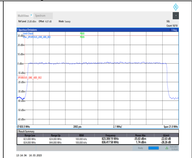
1-N26-824-849-PC3-15-20-L-3-DFT-PI2BPSK-Outer_Full-100@0-Ant1-1-seegraph-PASS-see graph
