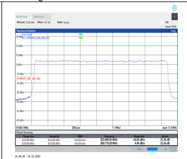
1-N26-824-849-PC3-15-10-L-3-DFT-PI2BPSK-Outer_Full-50@0-Ant1-1-seegraph-PASS-see graph
