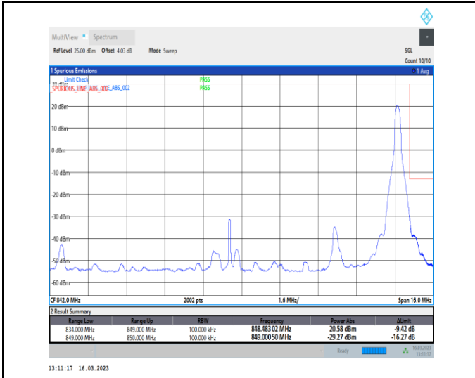
1-N26-824-849-PC3-15-15-H-2-DFT-PI2BPSK-Edge_1_RB_Right-1@78-Ant1-1-seegraph-PASS-see graph
