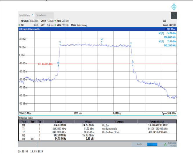
1-N26-824-849-PC3-15-15-H-2-DFT-PI2BPSK-Outer_Full-75@0-Ant1-13.397-14.130-≤15-PASS
