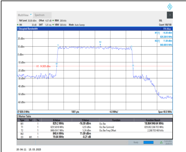
1-N26-824-849-PC3-15-20-H-6-CP-QPSK-Outer_Ful I-106@0-Ant1-18.865-19.640-≤20-PASS
