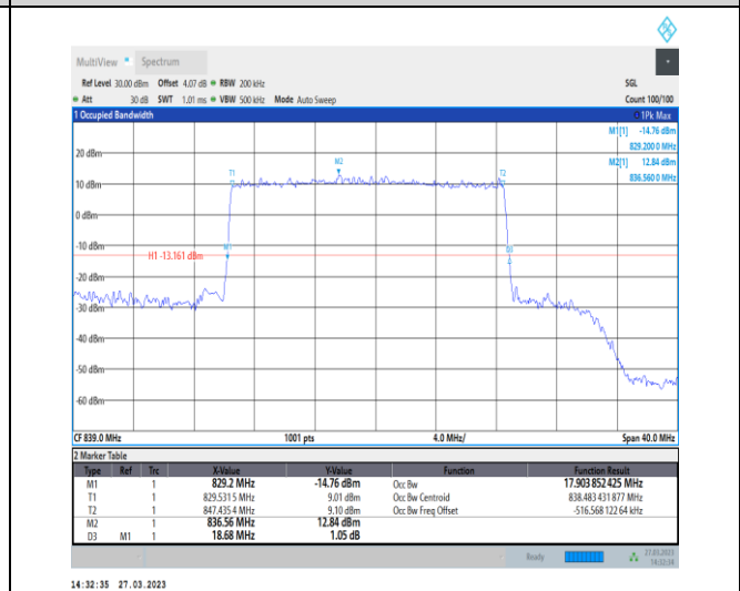
1-N26-824-849-PC3-15-20-H-1-DFT-QPSK-Outer_F ull-100@0-Ant1-17.904-18.680-≤20-PASS
