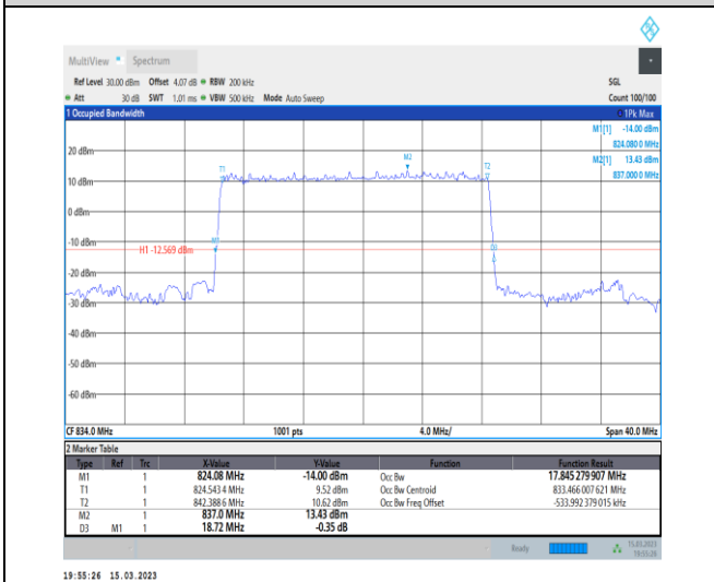
1-N26-824-849-PC3-15-20-L-2-DFT-PI2BPSK-Outer_Full-100@0-Ant1-17.845-18.720-≤20-PASS
