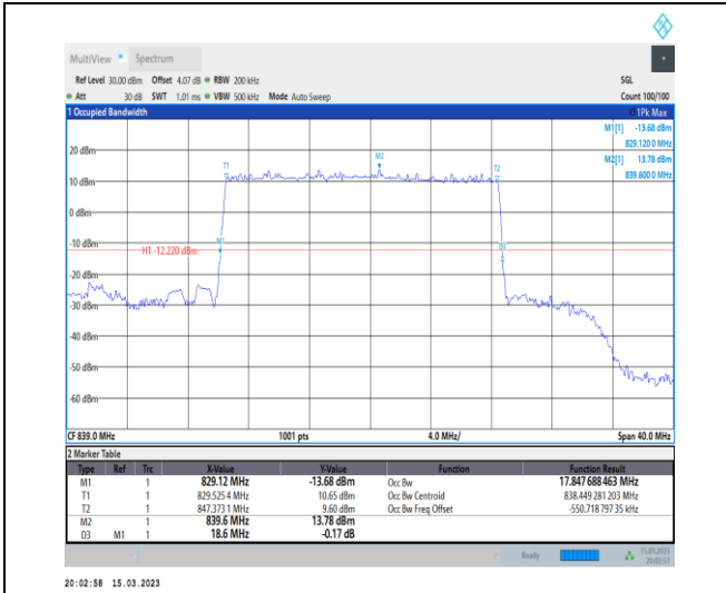
1-N26-824-849-PC3-15-20-H-2-DFT-PI2BPSK-Outer_Full-100@0-Ant1-17.848-18.600-≤20-PASS
