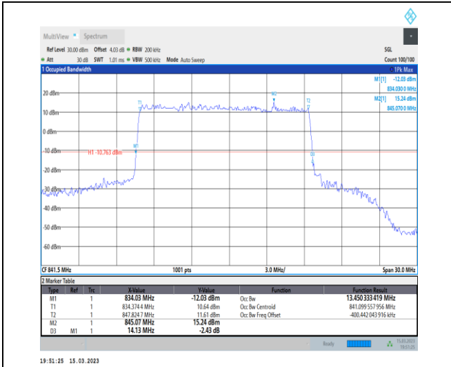
1-N26-824-849-PC3-15-15-H-1-DFT-QPSK-Outer_Full-75@0-Ant1-13.45-14.130-≤15-PASS
