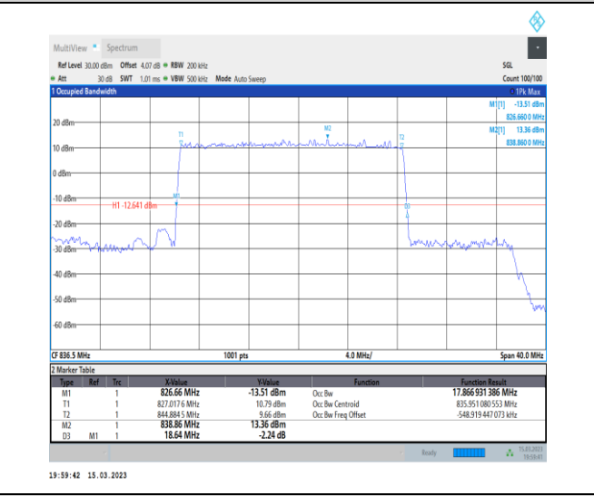
1-N26-824-849-PC3-15-20-M-2-DFT-PI2BPSK-Outer_Full-100@0-Ant1-17.867-18.640-≤20-PASS
