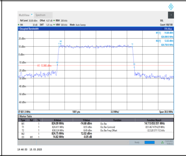
1-N26-824-849-PC3-15-15-L-6-CP-QPSK-Outer_Full-79@0-Ant1-14.113-14.820-≤15-PASS
