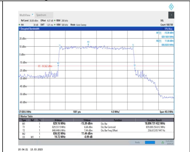
1-N26-824-849-PC3-15-20-H-7-CP-16QAM-Outer_Full-106@0-Ant1-18.897-19.720-≤20-PASS
