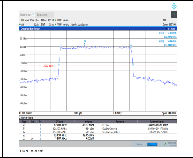
1-N26-824-849-PC3-15-15-M-5-DFT-256QAM-Outer_Full-75@0-Ant1-13.403-14.070-≤15-PASS
