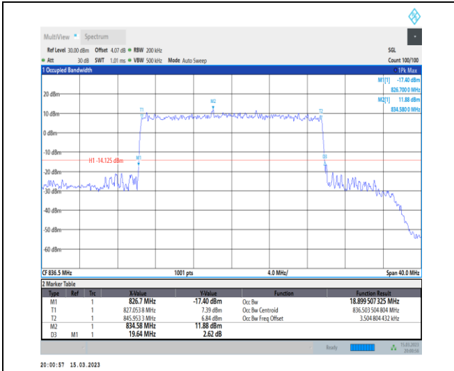
1-N26-824-849-PC3-15-20-M-7-CP-16QAM-Outer_F ull-106@0-Ant1-18.9-19.640-≤20-PASS
