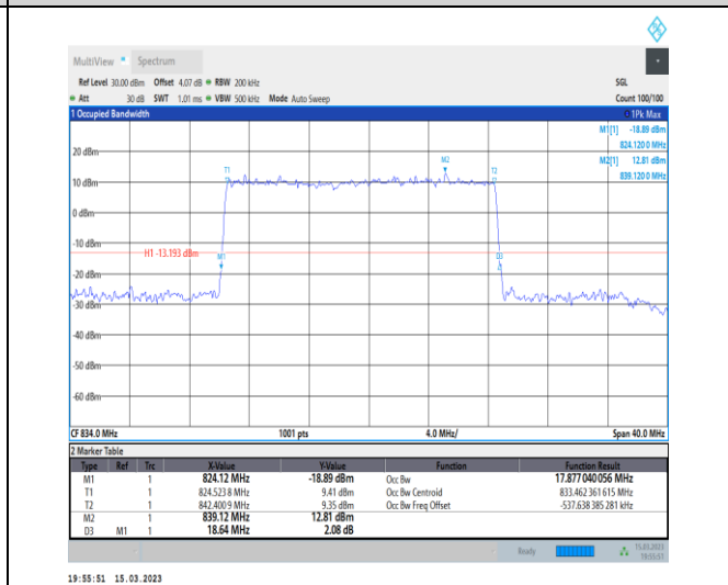
1-N26-824-849-PC3-15-20-L-3-DFT-16QAM-Outer_Full-100@0-Ant1-17.877-18.640-≤20-PASS
