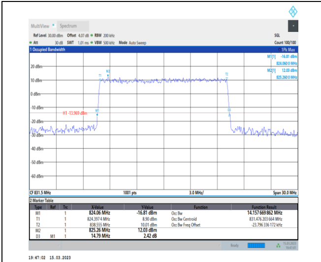
1-N26-824-849-PC3-15-15-L-7-CP-16QAM-Outer_Full-79@0-Ant1-14.158-14.790-≤15-PASS
