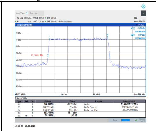
1-N26-824-849-PC3-15-15-L-4-DFT-64QAM-Outer_Full-75@0-Ant1-13.445-14.160-≤15-PASS
