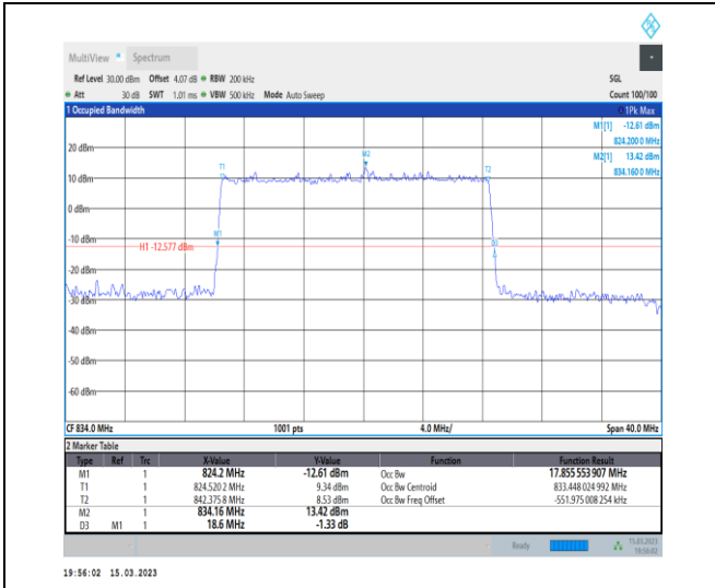
1-N26-824-849-PC3-15-20-L-4-DFT-64QAM-Outer_Full-100@0-Ant1-17.856-18.600-≤20-PASS
