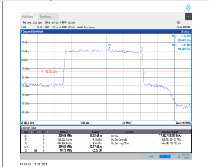
1-N26-824-849-PC3-15-20-H-3-DFT-16QAM-Outer_Full-100@0-Ant1-17.862-18.720-≤20-PASS
