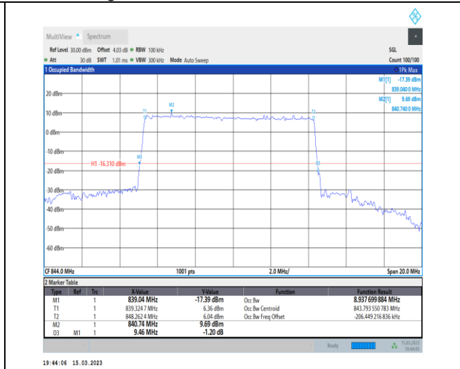
1-N26-824-849-PC3-15-10-H-5-DFT-256QAM-Outer_Full-50@0-Ant1-8.938-9.460-≤10-PASS
