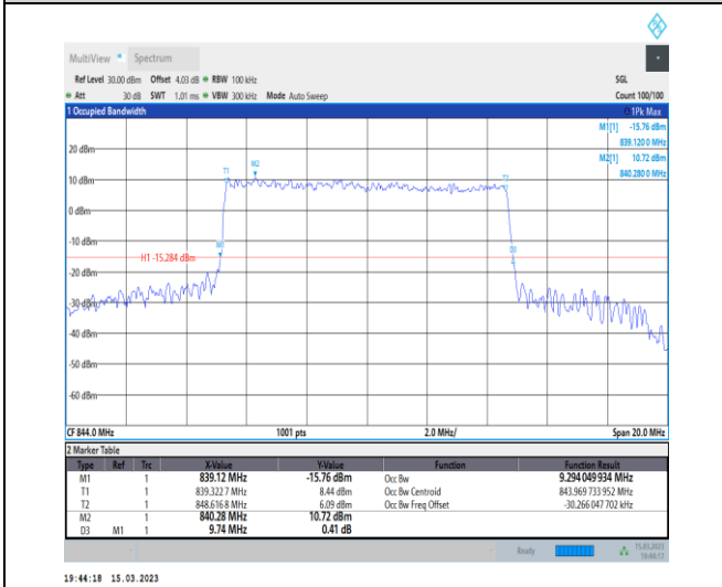
1-N26-824-849-PC3-15-10-H-6-CP-QPSK-Outer_Ful I-52@0-Ant1-9.294-9.740-≤10-PASS
