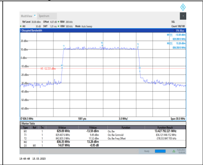
1-N26-824-849-PC3-15-15-M-3-DFT-16QAM-Outer_Full-75@0-Ant1-13.428-14.070-≤15-PASS
