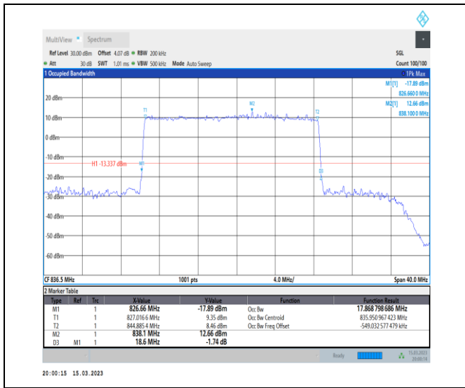
1-N26-824-849-PC3-15-20-M-3-DFT-16QAM-Outer_Full-100@0-Ant1-17.869-18.600-≤20-PASS
