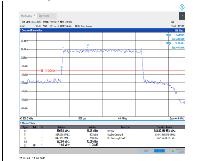
1-N26-824-849-PC3-15-20-M-8-CP-64QAM-Outer_F ull-106@0-Ant1-18.887-19.800-≤20-PASS
