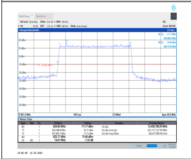
1-N26-824-849-PC3-15-15-L-1-DFT-QPSK-Outer_Full-75@0-Ant1-13.457-14.070-≤15-PASS
