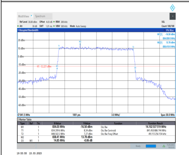
1-N26-824-849-PC3-15-15-H-7-CP-16QAM-Outer_Full-79@0-Ant1-14.103-14.850-≤15-PASS
