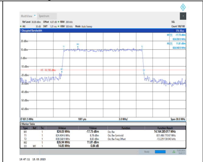
1-N26-824-849-PC3-15-15-L-8-CP-64QAM-Outer_Full-79@0-Ant1-14.164-14.850-≤15-PASS
