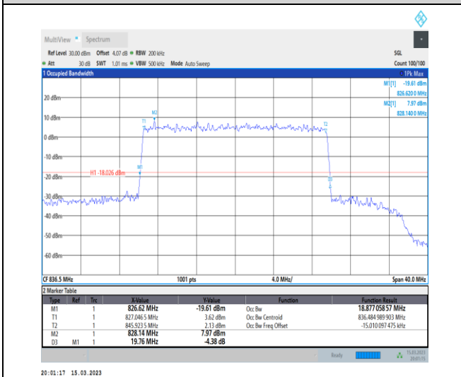
1-N26-824-849-PC3-15-20-M-9-CP-256QAM-Outer_F ull-106@0-Ant1-18.877-19.760-≤20-PASS
