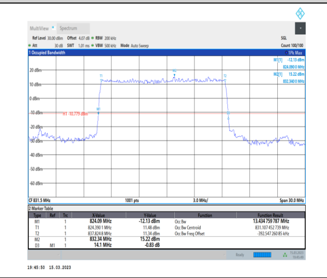
1-N26-824-849-PC3-15-15-L-2-DFT-PI2BPSK-Outer_Full-75@0-Ant1-13.435-14.100-≤15-PASS
