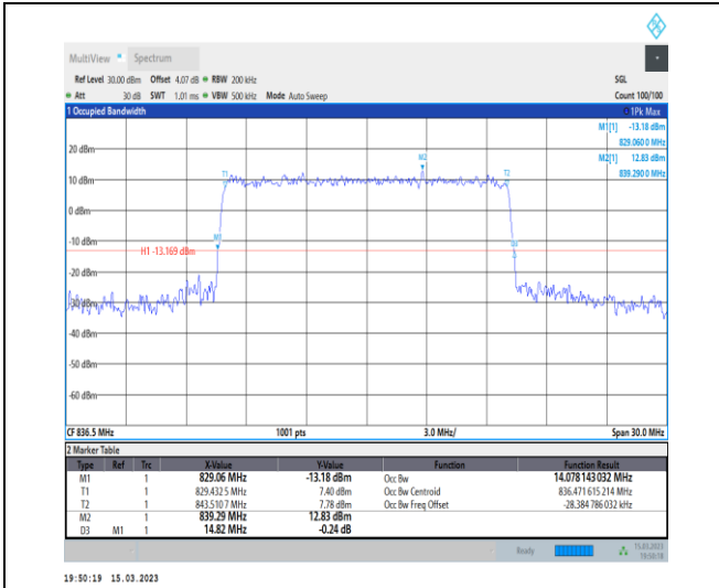
1-N26-824-849-PC3-15-15-M-6-CP-QPSK-Outer_Fu II-79@0-Ant1-14.078-14.820-≤15-PASS
