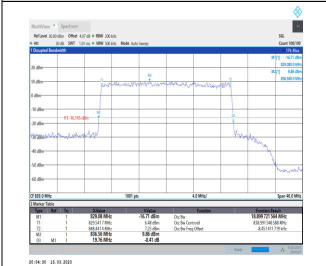
1-N26-824-849-PC3-15-20-H-8-CP-64QAM-Outer_Full-106@0-Ant1-18.9-19.760-≤20-PASS
