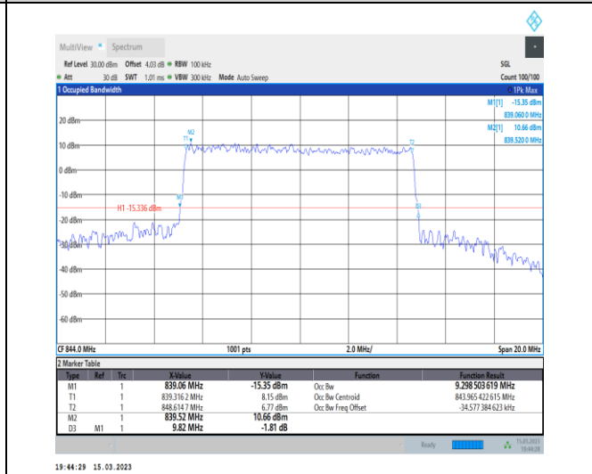
1-N26-824-849-PC3-15-10-H-7-CP-16QAM-Outer_Full-52@0-Ant1-9.299-9.820-≤10-PASS
