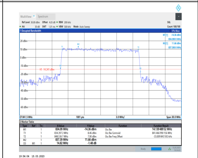
1-N26-824-849-PC3-15-15-H-8-CP-64QAM-Outer_Full-79@0-Ant1-14.139-14.820-≤15-PASS
