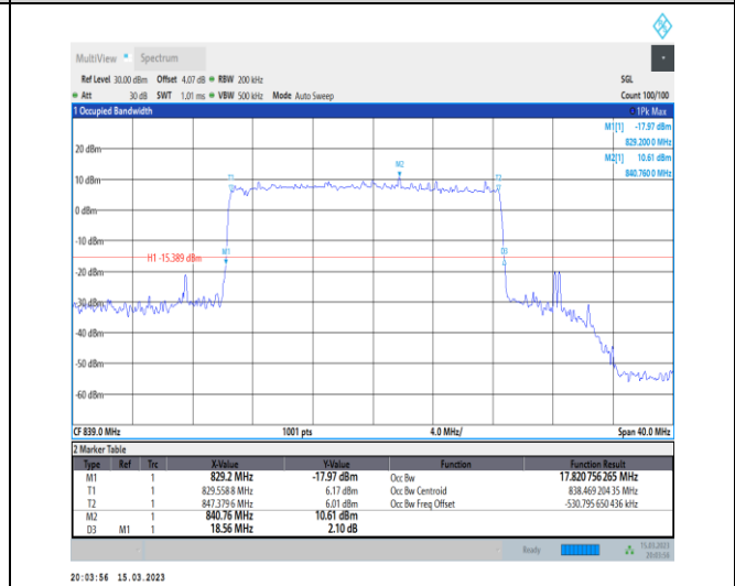
1-N26-824-849-PC3-15-20-H-5-DFT-256QAM-Outer_Full-100@0-Ant1-17.821-18.560-≤20-PASS
