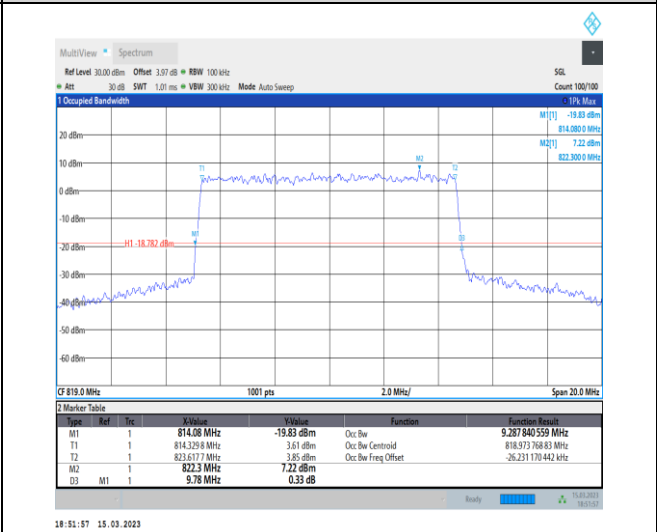
1-N26-814-824-PC3-15-10-M-9-CP-256QAM-Outer_F ull-52@0-Ant1-9.288-9.780-≤10-PASS
