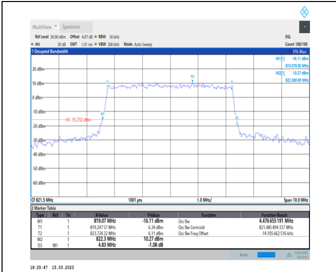
1-N26-814-824-PC3-15-5-H-7-CP-16QAM-Outer_Ful I-25@0-Ant1-4.477-4.830-≤5-PASS
