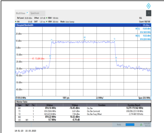
1-N26-814-824-PC3-15-10-M-6-CP-QPSK-Outer_Ful I-52@0-Ant1-9.275-9.700-≤10-PASS
