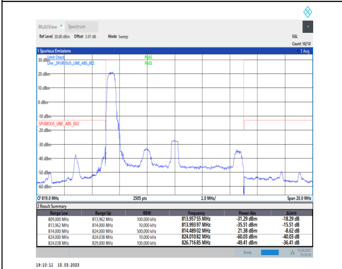
1-N26-814-824-PC3-15-10-L-4-CP-QPSK-Edge_1RB_Left-1@0-Ant1-1--PASS-see graph
