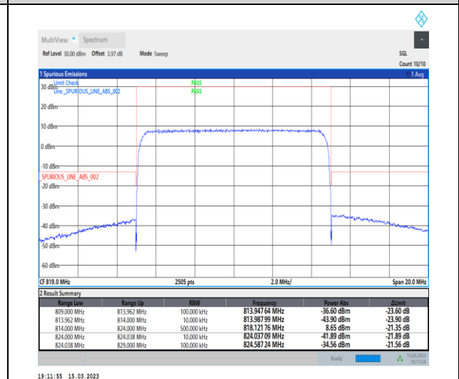
1-N26-814-824-PC3-15-10-H-6-CP-QPSK-Outer_Full-52@0-Ant1-1--PASS-see graph
