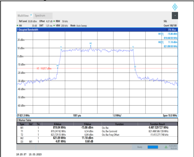
1-N26-814-824-PC3-15-5-H-8-CP-64QAM-Outer_Fu ll-25@0-Ant1-4.482-4.810-≤5-PASS
