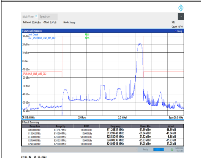
1-N26-814-824-PC3-15-10-H-5-CP-QPSK-Edge_1RB_Right-1@51-Ant1-1--PASS-see graph
