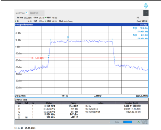
1-N26-814-824-PC3-15-10-M-8-CP-64QAM-Outer_F ull-52@0-Ant1-9.255-9.860-≤10-PASS
