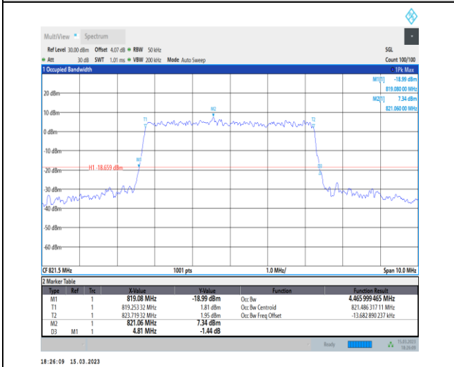
1-N26-814-824-PC3-15-5-H-9-CP-256QAM-Outer_F ull-25@0-Ant1-4.466-4.810-≤5-PASS
