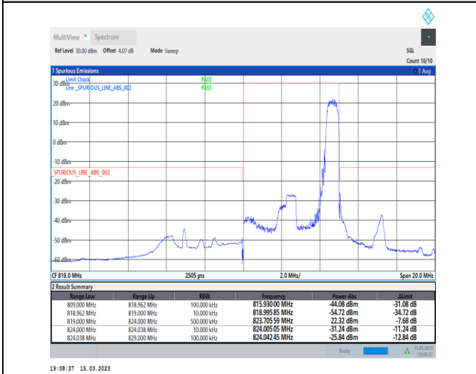
1-N26-814-824-PC3-15-5-H-5-CP-QPSK-Edge_1RB_Right-1@24-Ant1-1--PASS-see graph
