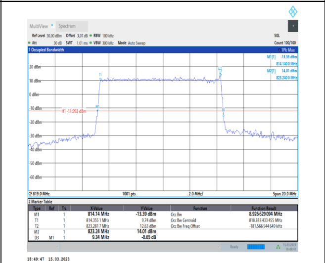
1-N26-814-824-PC3-15-10-M-1-DFT-QPSK-Outer_F ull-50@0-Ant1-8.927-9.340-≤10-PASS
