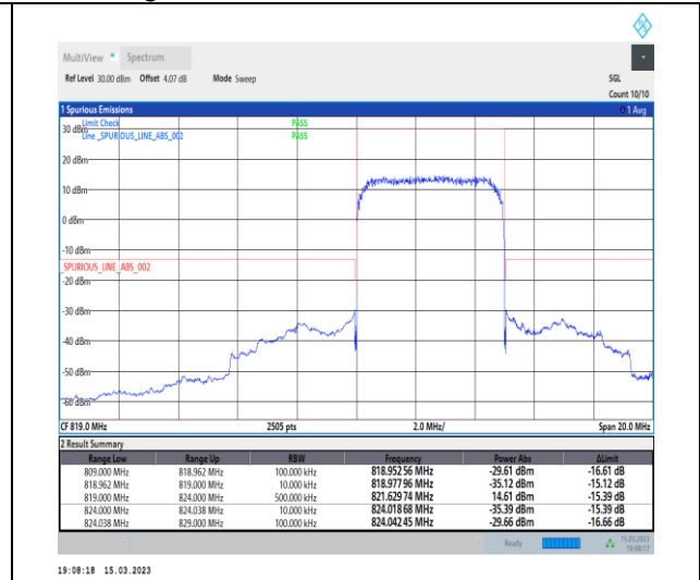
1-N26-814-824-PC3-15-5-H-3-DFT-PI2BPSK-Outer_Full-25@0-Ant1-1--PASS-see graph
