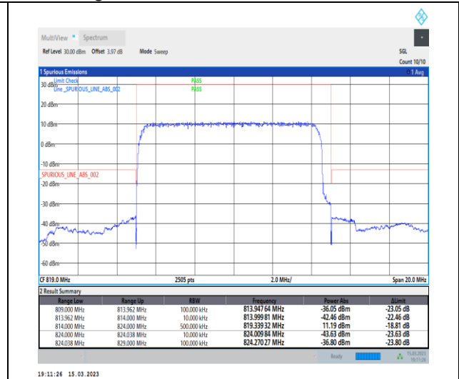
1-N26-814-824-PC3-15-10-H-3-DFT-PI2BPSK-Out er_Full-50@0-Ant1-1--PASS-see graph
