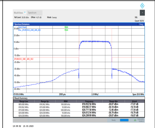
1-N26-814-824-PC3-15-5-H-6-CP-QPSK-Outer_Full-25@0-Ant1-1--PASS-see graph
