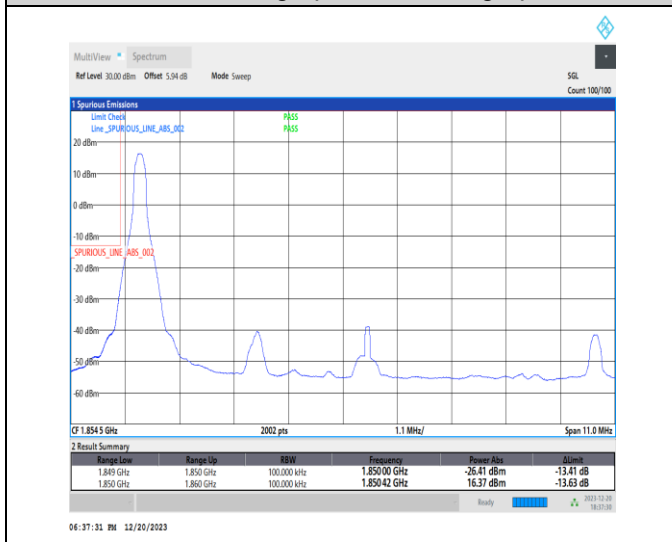
1-N25-15-10-L-4-CP-QPSK-Edge_1RB_Left-1@0-Ant1-1-seegraph-PASS-see graph
