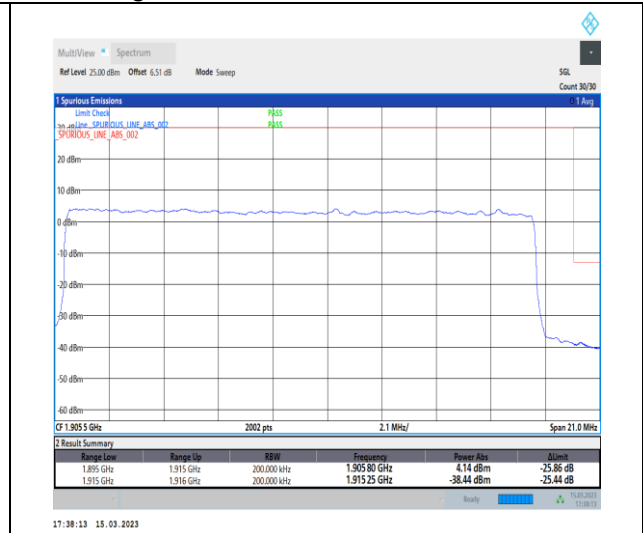
1-N25-PC3-15-20-H-3-DFT-PI2BPSK-Outer_Full-100@0-Ant1-1-seegraph-PASS-see graph
