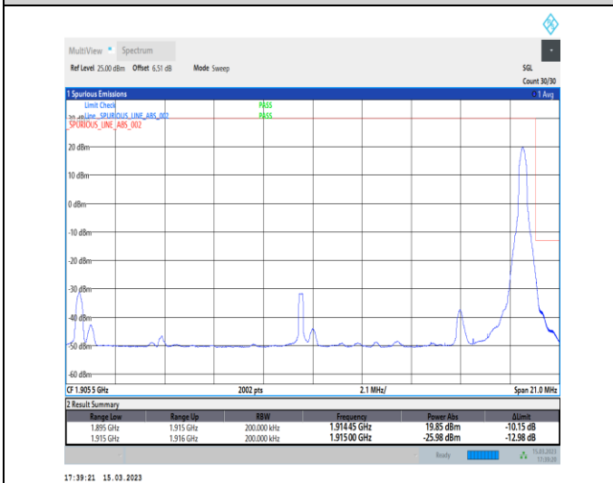
1-N25-PC3-15-20-H-5-CP-QPSK-Edge_1RB_Right-1@105-Ant1-1-seegraph-PASS-see graph
