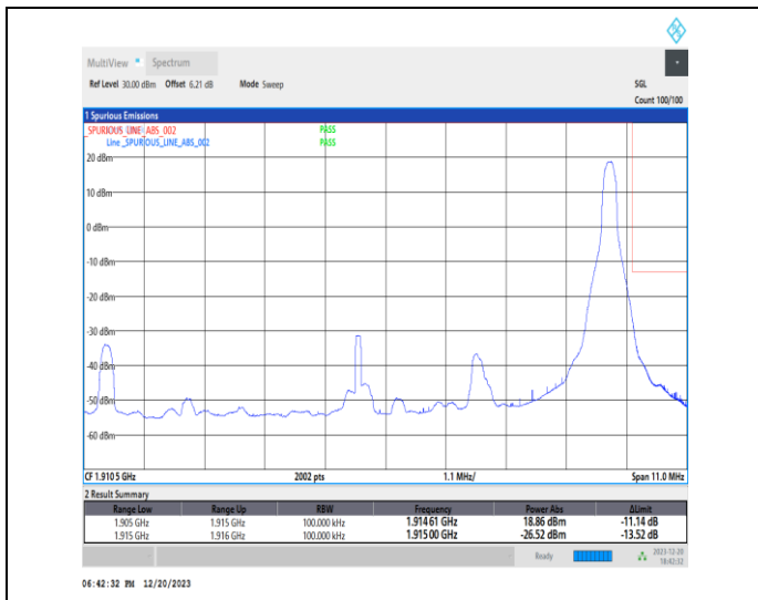
1-N25-15-10-H-2-DFT-PI2BPSK-Edge_1RB_Right-1@51-Ant1-1-seegraph-PASS-see graph
