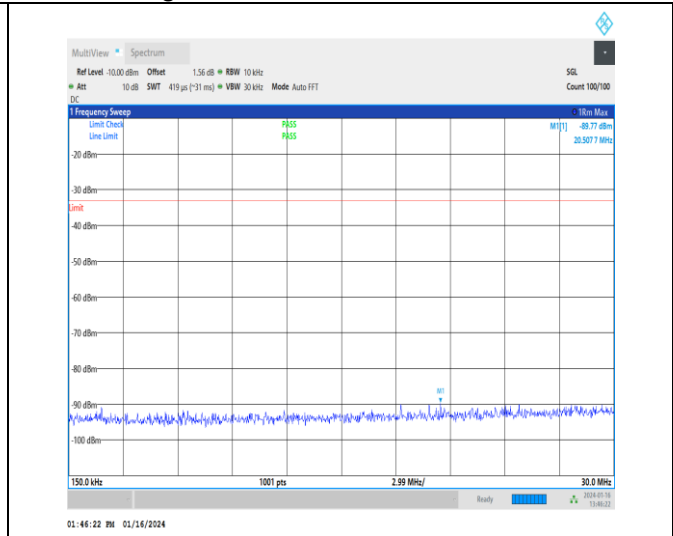
1-N25-15-20-H-1-DFT-PI2BPSK-Inner_1RB_Left-1 @1-0.15-30-Ant1-4.57--89.77--33-PASS
