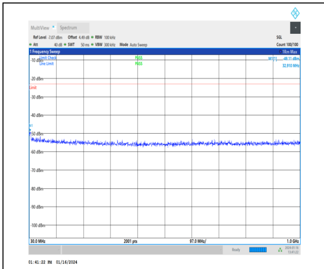
1-N25-15-20-M-1-DFT-PI2BPSK-Inner_1RB_Left-1 @ 1-30-1000-Ant1-32.91--49.11--23-PASS
