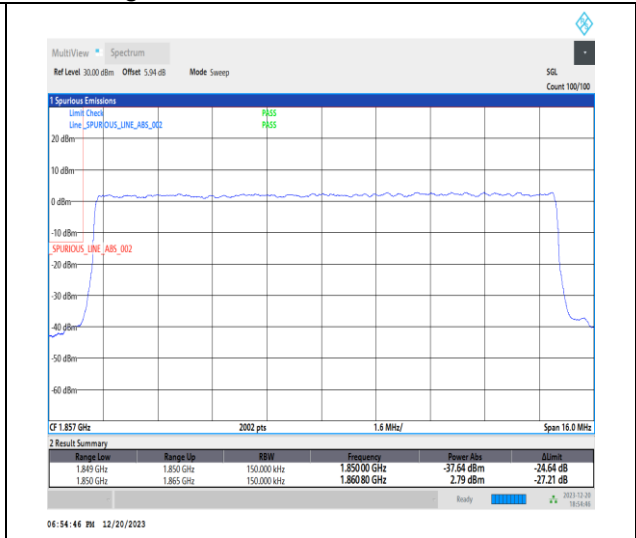
1-N25-15-15-L-3-DFT-PI2BPSK-Outer_Full-75@0-Ant1-1-seegraph-PASS-see graph
