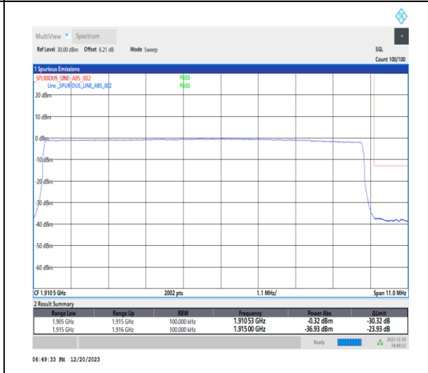
1-N25-15-10-H-6-CP-QPSK-Outer_Full-52@0-Ant1-1-seegraph-PASS-see graph
