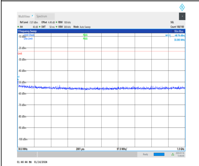
1-N25-15-20-H-1-DFT-PI2BPSK-Inner_1RB_Left-1 @1-30-1000-Ant1-30.49--48.76--23-PASS
