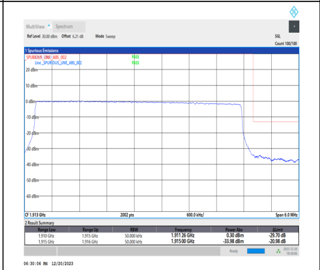
1-N25-15-5-H-6-CP-QPSK-Outer_Full-25@0-Ant1-1-seegraph-PASS-see graph
