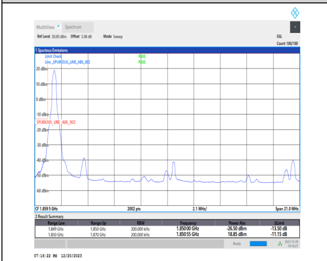
1-N25-15-20-L-4-CP-QPSK-Edge_1RB_Left-1@0-Ant1-1-seegraph-PASS-see graph
