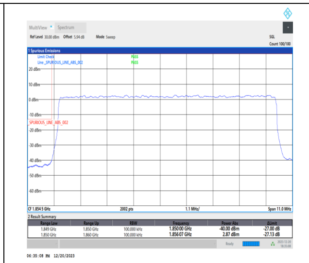
1-N25-15-10-L-3-DFT-PI2BPSK-Outer_Full-50@0-Ant1-1-seegraph-PASS-see graph
