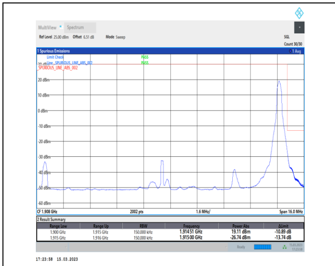
1-N25-PC3-15-15-H-2-DFT-PI2BPSK-Edge_1RB_Righ t-1@78-Ant1-1-seegraph-PASS-see graph
