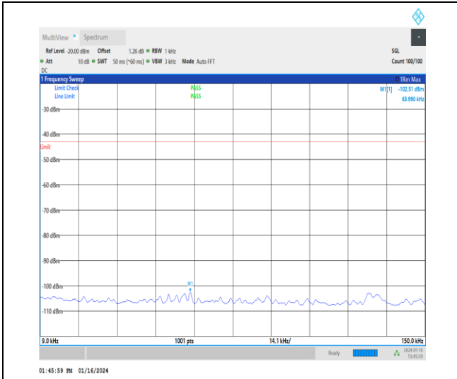
1-N25-15-20-H-1-DFT-PI2BPSK-Inner_1RB_Left-1 @1-0.009-0.15-Ant1-0.06--102.51--43-PASS
