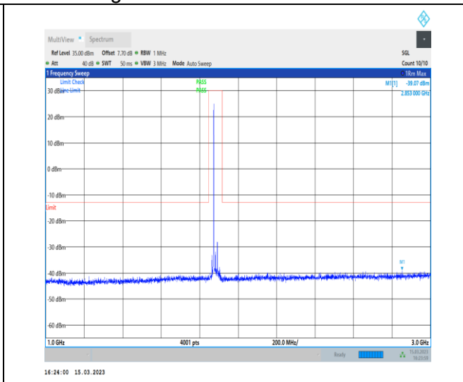
1-N25-PC3-15-20-M-1-DFT-PI2BPSK-Inner_1RB_L eft-1@1-1000-3000-Ant1-2853.00--39.07--13-PASS
