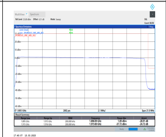
1-N25-PC3-15-20-H-6-CP-QPSK-Outer_Full-106@0-Ant1-1-seegraph-PASS-see graph
