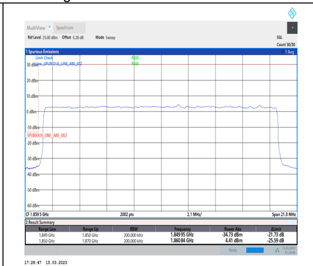
1-N25-PC3-15-20-L-3-DFT-PI2BPSK-Outer_Full-100@0-Ant1-1-seegraph-PASS-see graph
