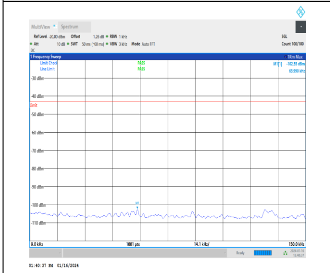
1-N25-15-20-M-1-DFT-PI2BPSK-Inner_1RB_Left-1 @1-0.009-0.15-Ant1-0.06--102.55--43-PASS
