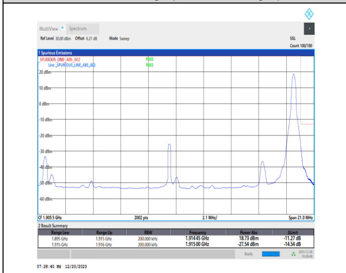
1-N25-15-20-H-5-CP-QPSK-Edge_1RB_Right-1@105-Ant1-1-seegraph-PASS-see graph
