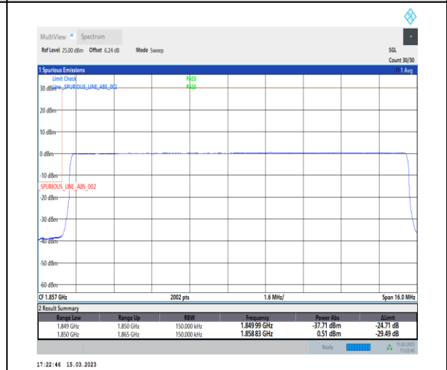
1-N25-PC3-15-15-L-6-CP-QPSK-Outer_Full-79@0-Ant1-1-seegraph-PASS-see graph
