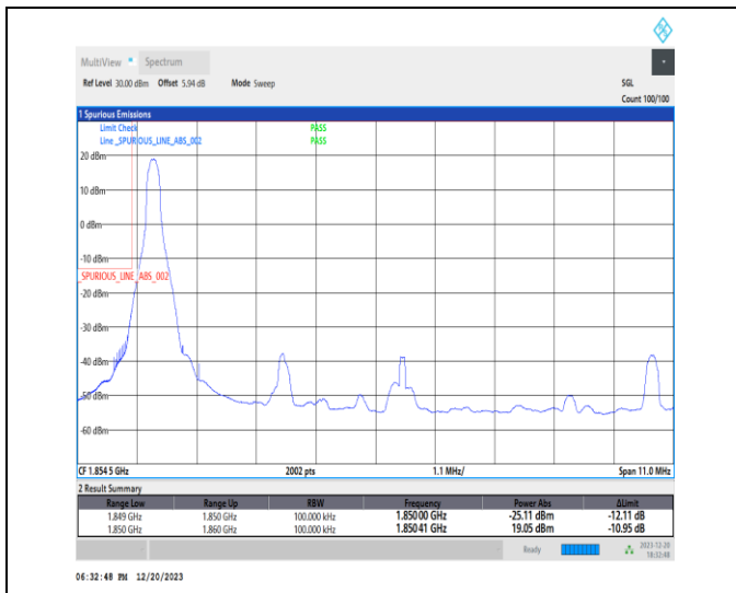
1-N25-15-10-L-1-DFT-PI2BPSK-Edge_1RB_Left-1@0-Ant1-1-seegraph-PASS-see graph
