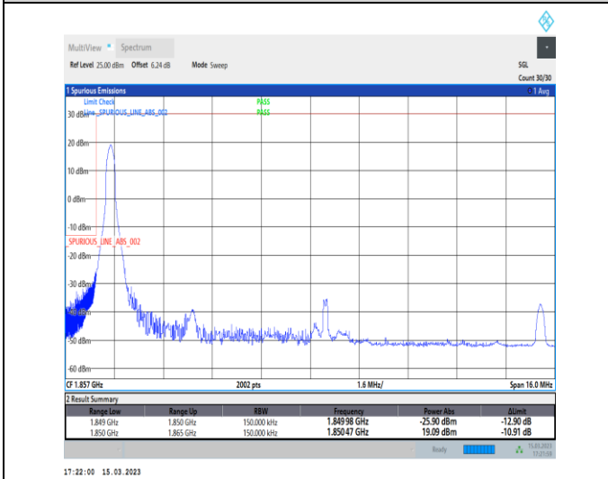
1-N25-PC3-15-15-L-4-CP-QPSK-Edge_1RB_Left-1@0-Ant1-1-seegraph-PASS-see graph
