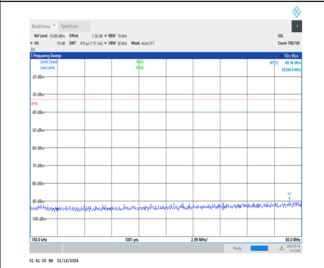
1-N25-15-20-M-1-DFT-PI2BPSK-Inner_1RB_Left-1@ 1-0.15-30-Ant1-4.54--89.36--33-PASS
