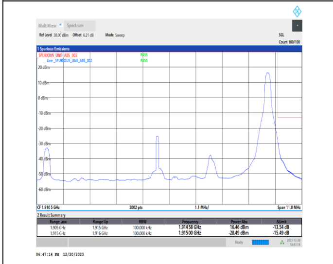
1-N25-15-10-H-5-CP-QPSK-Edge_1RB_Right-1@51-Ant1-1-seegraph-PASS-see graph
