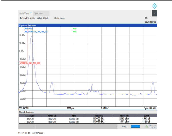
1-N25-15-15-L-4-CP-QPSK-Edge_1RB_Left-1@0-Ant1-1-seegraph-PASS-see graph
