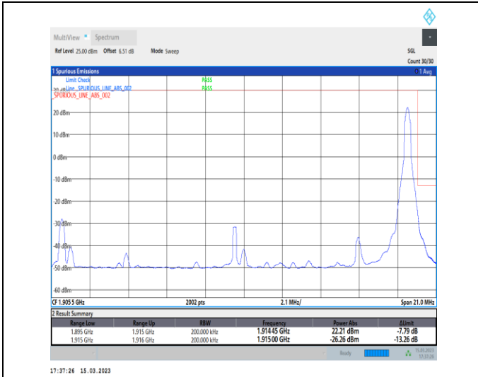
1-N25-PC3-15-20-H-2-DFT-PI2BPSK-Edge_1RB_Right-t-1@105-Ant1-1-seegraph-PASS-see graph
