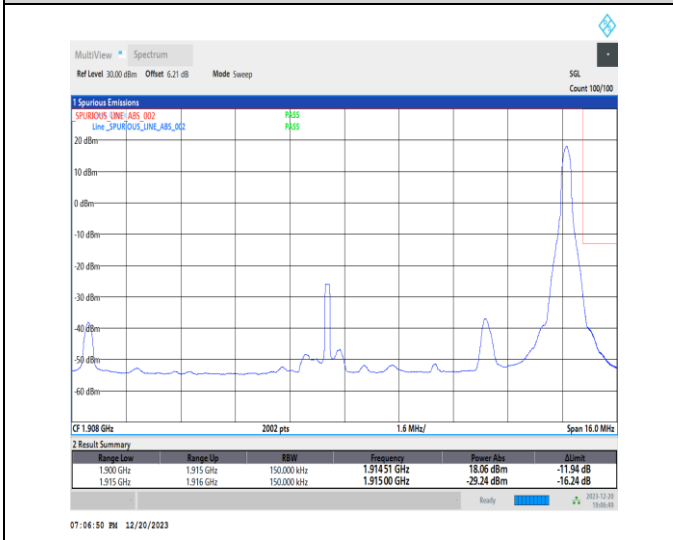
1-N25-15-15-H-5-CP-QPSK-Edge_1RB_Right-1@78-Ant1-1-seegraph-PASS-see graph
