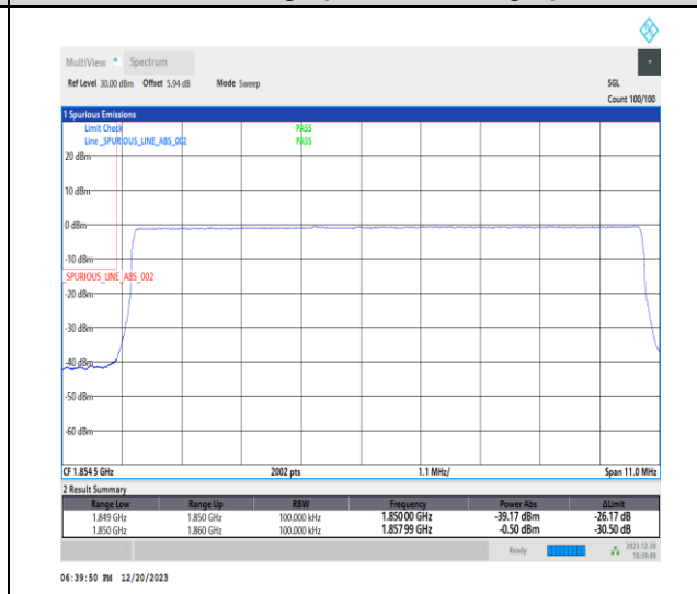
1-N25-15-10-L-6-CP-QPSK-Outer_Full-52@0-Ant1-1-seegraph-PASS-see graph
