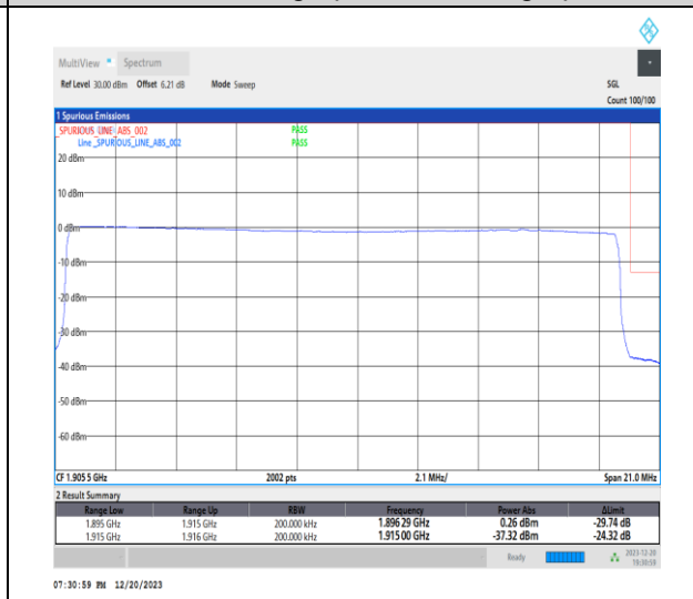
1-N25-15-20-H-6-CP-QPSK-Outer_Full-106@0-Ant1-1-seegraph-PASS-see graph
