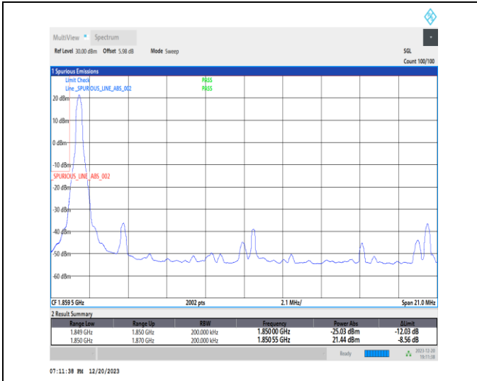
1-N25-15-20-L-1-DFT-PI2BPSK-Edge_1RB_Left-1@0-Ant1-1-seegraph-PASS-see graph
