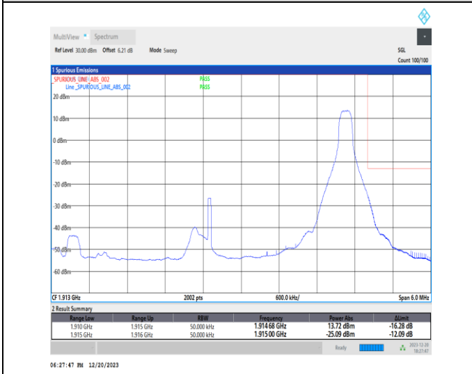
1-N25-15-5-H-5-CP-QPSK-Edge_1RB_Right-1@24-An1-1-seegraph-PASS-see graph
