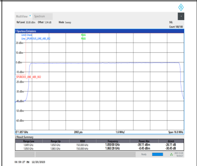
1-N25-15-15-L-6-CP-QPSK-Outer_Full-79@0-Ant1-1-seegraph-PASS-see graph
