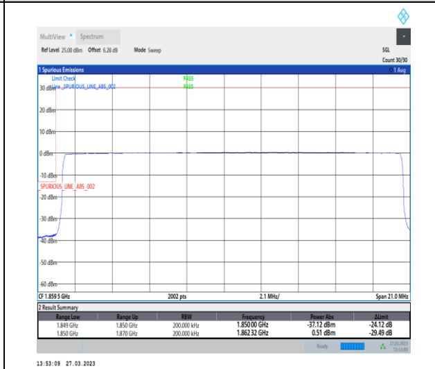
1-N25-PC3-15-20-L-6-CP-QPSK-Outer_Full-106@0-Ant1-1-seegraph-PASS-see graph
