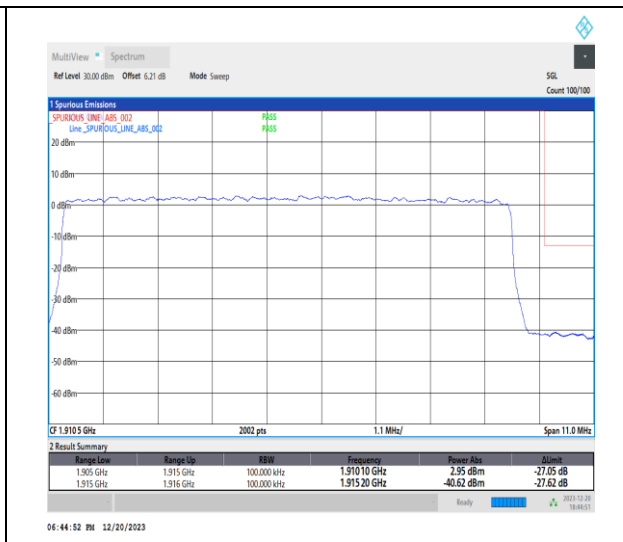
1-N25-15-10-H-3-DFT-PI2BPSK-Outer_Full-50@0-Ant1-1-seegraph-PASS-see graph
