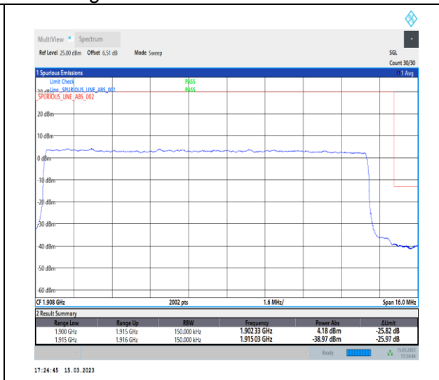
1-N25-PC3-15-15-H-3-DFT-PI2BPSK-Outer_Full-7 5@0-Ant1-1-seegraph-PASS-see graph
