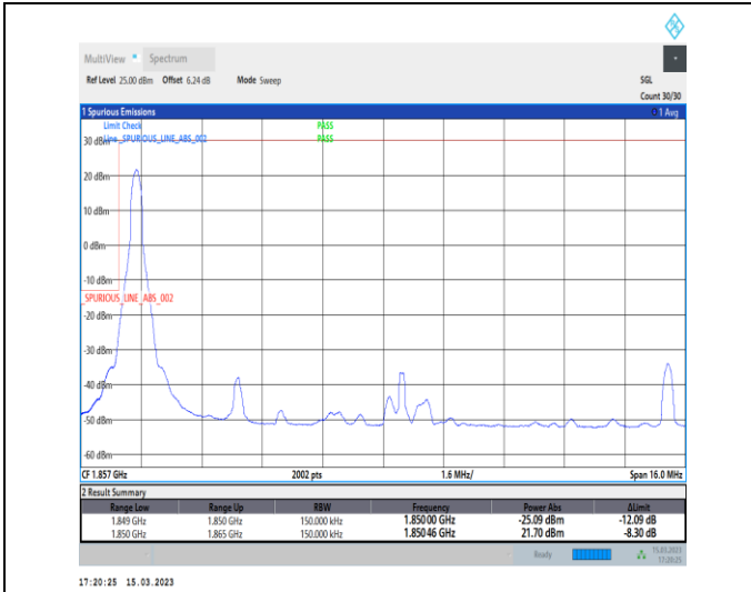
1-N25-PC3-15-15-L-1-DFT-PI2BPSK-Edge_1RB_Left-1@0-Ant1-1-seegraph-PASS-see graph
