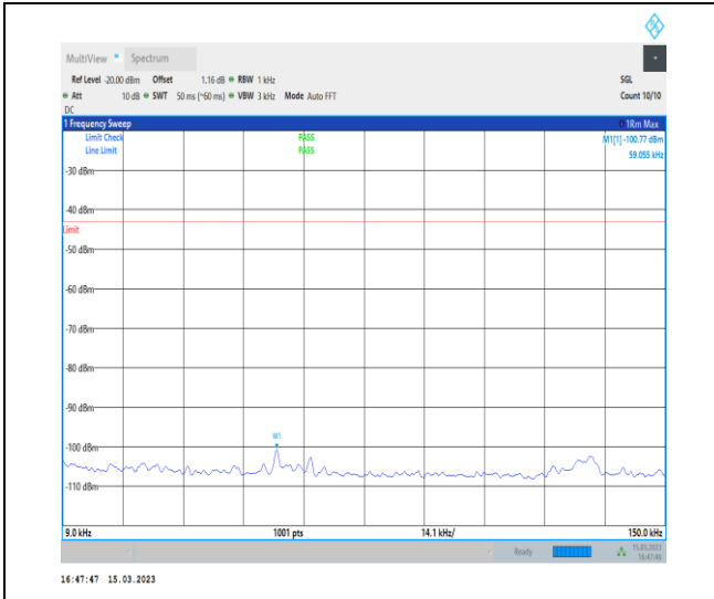
1-N25-PC3-15-20-H-1-DFT-PI2BPSK-Inner_1RB_L eft-1@1-0.009-0.15-Ant1-0.06--100.77--43-PASS
