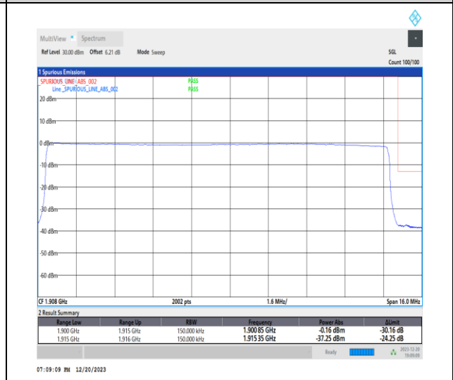
1-N25-15-15-H-6-CP-QPSK-Outer_Full-79@0-Ant1-1-seegraph-PASS-see graph
