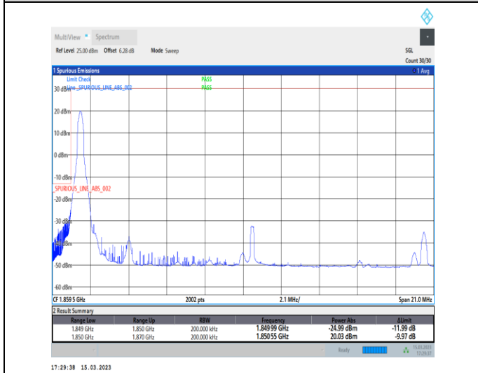
1-N25-PC3-15-20-L-4-CP-QPSK-Edge_1RB_Left-1@0-Ant1-1-seegraph-PASS-see graph
