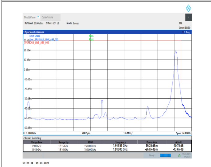
1-N25-PC3-15-15-H-5-CP-QPSK-Edge_1RB_Right-1 @78-Ant1-1-seegraph-PASS-see graph
