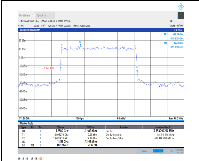
1-N25-PC3-15-20-L-2-DFT-PI2BPSK-Outer_Full-100 @0-Ant1-17.854-18.520-≤20-PASS
