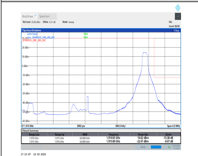
1-N25-PC3-15-5-H-5-CP-QPSK-Edge_1RB_Right-1@24-Ant1-1-seegraph-PASS-see graph
