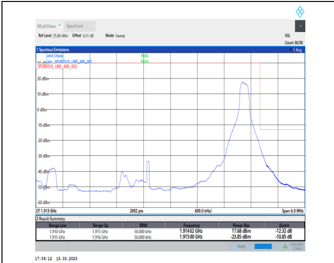
1-N25-PC3-15-5-H-2-DFT-PI2BPSK-Edge_1RB_Right-1@24-Ant1-1-seegraph-PASS-see graph
