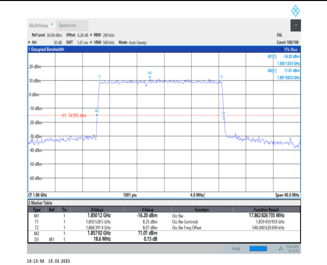
1-N25-PC3-15-20-L-3-DFT-16QAM-Outer_Full-100 @0-Ant1-17.863-18.600-≤20-PASS
