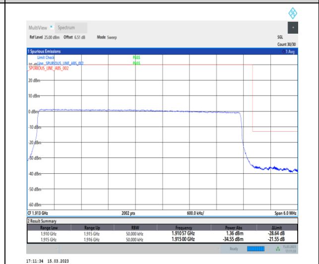
1-N25-PC3-15-5-H-6-CP-QPSK-Outer_Full-25@0-Ant1-1-seegraph-PASS-see graph
