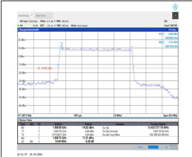
1-N25-PC3-15-15-H-5-DFT-256QAM-Outer_Full-75 @0-Ant1-13.434-14.040-≤15-PASS
