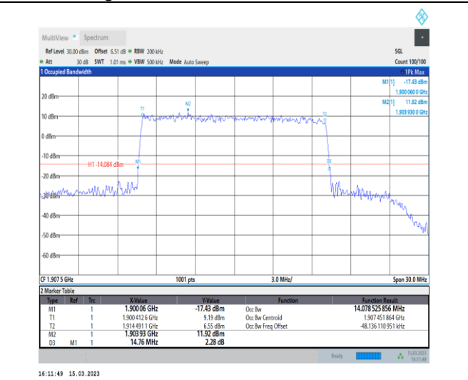
1-N25-PC3-15-15-H-6-CP-QPSK-Outer_Full-79@0-Ant1-14.079-14.760-≤15-PASS
