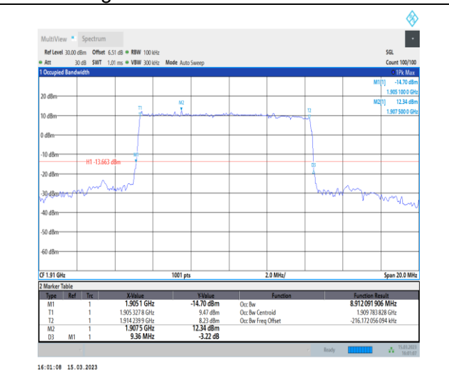
1-N25-PC3-15-10-H-1-DFT-QPSK-Outer_Full-50@0- Ant1-8.912-9.360-≤10-PASS
