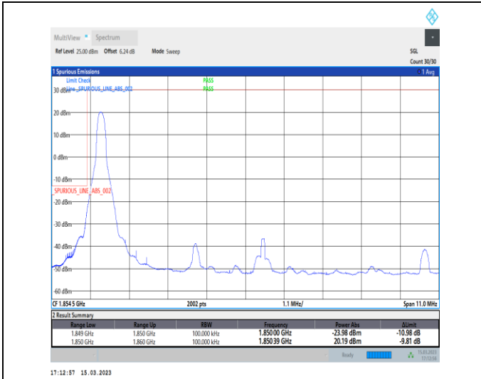
1-N25-PC3-15-10-L-1-DFT-PI2BPSK-Edge_1RB_Left-1@0-Ant1-1-seegraph-PASS-see graph
