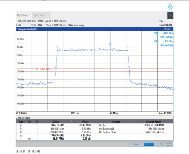
1-N25-PC3-15-20-L-5-DFT-256QAM-Outer_Full-100 @0-Ant1-17.901-18.640-≤20-PASS
