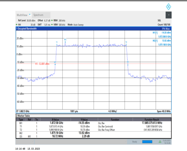
1-N25-PC3-15-20-M-2-DFT-PI2BPSK-Outer_Full-100@0-Ant1-17.885-18.720-≤20-PASS
