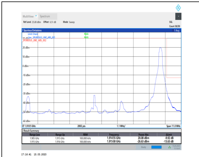
1-N25-PC3-15-10-H-2-DFT-PI2BPSK-Edge_1RB_Right-t1@51-Ant1-1-seegraph-PASS-see graph
