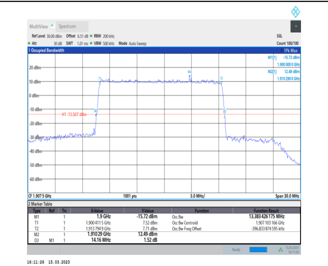
1-N25-PC3-15-15-H-4-DFT-64QAM-Outer_Full-75@ 0-Ant1-13.383-14.160-≤15-PASS
