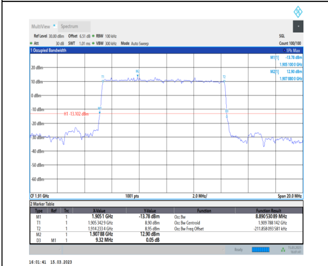
1-N25-PC3-15-10-H-2-DFT-PI2BPSK-Outer_Full-50 @0-Ant1-8.891-9.320-≤10-PASS
