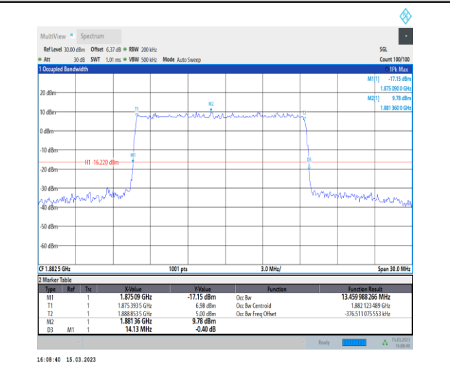
1-N25-PC3-15-15-M-5-DFT-256QAM-Outer_Full-75 @0-Ant1-13.46-14.130-≤15-PASS
