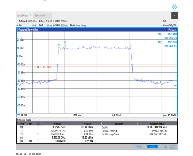
1-N25-PC3-15-20-L-1-DFT-QPSK-Outer_Full-100@0 -Ant1-17.848-18.600-≤20-PASS
