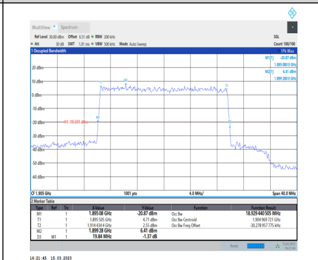
1-N25-PC3-15-20-H-9-CP-256QAM-Outer_Full-106@0 -Ant1-18.929-19.840-≤20-PASS
