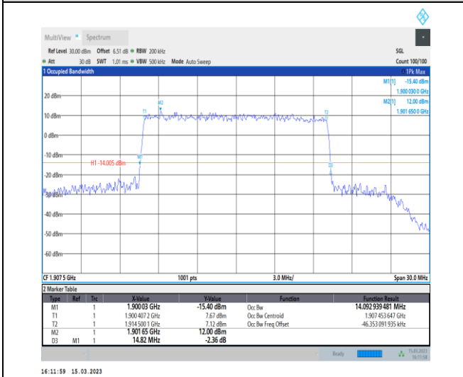
1-N25-PC3-15-15-H-7-CP-16QAM-Outer_Full-79@0 -Ant1-14.093-14.820-≤15-PASS
