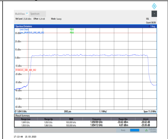
1-N25-PC3-15-10-L-3-DFT-PI2BPSK-Outer_Full-50@0-Ant1-1-seegraph-PASS-see graph
