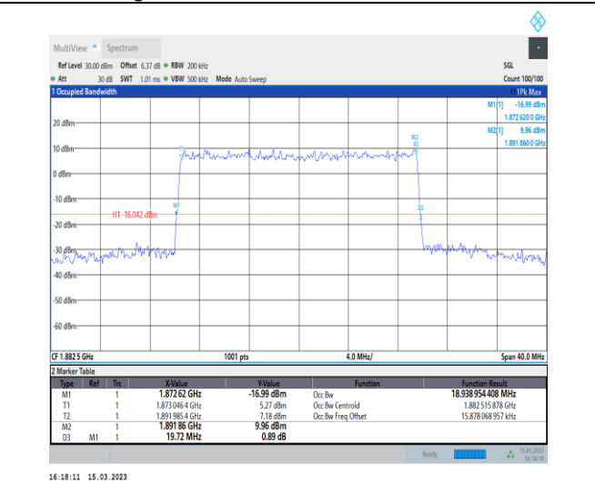
1-N25-PC3-15-20-M-8-CP-64QAM-Outer_Full-106@ 0-Ant1-18.939-19.720-≤20-PASS
