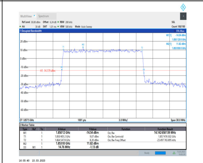
1-N25-PC3-15-15-L-6-CP-QPSK-Outer_Full-79@0-A nt1-14.143-14.760-≤15-PASS
