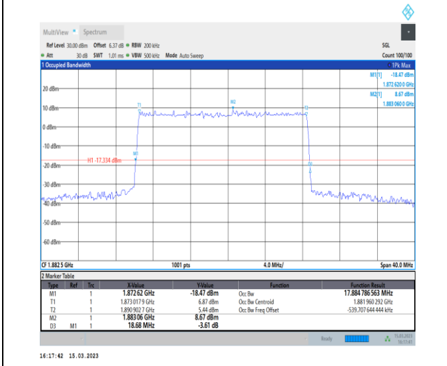
1-N25-PC3-15-20-M-5-DFT-256QAM-Outer_Full-100 @0-Ant1-17.885-18.680-≤20-PASS
