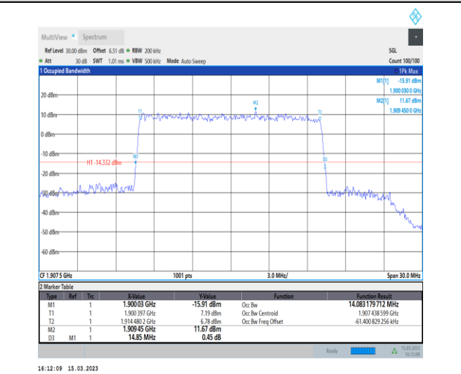
1-N25-PC3-15-15-H-8-CP-64QAM-Outer_Full-79@0 -Ant1-14.083-14.850-≤15-PASS
