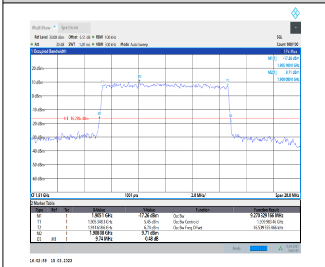
1-N25-PC3-15-10-H-6-CP-QPSK-Outer_Full-52@0- Ant1-9.27-9.740-≤10-PASS
