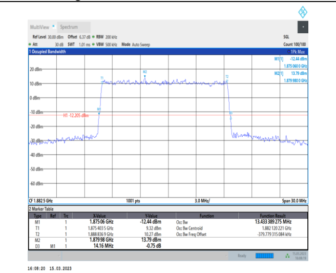
1-N25-PC3-15-15-M-3-DFT-16QAM-Outer_Full-75@ 0-Ant1-13.433-14.160-≤15-PASS
