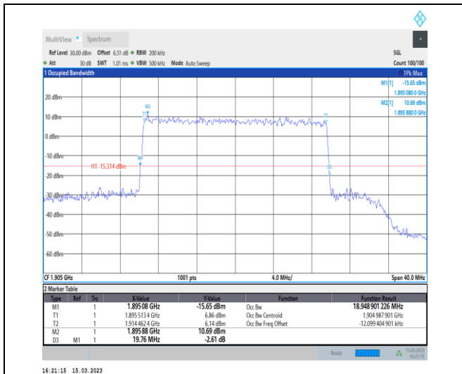
1-N25-PC3-15-20-H-6-CP-QPSK-Outer_Full-106@0 -Ant1-18.949-19.760-≤20-PASS
