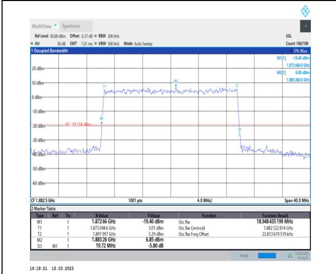
1-N25-PC3-15-20-M-9-CP-256QAM-Outer_Full-106 @0-Ant1-18.948-19.720-≤20-PASS
