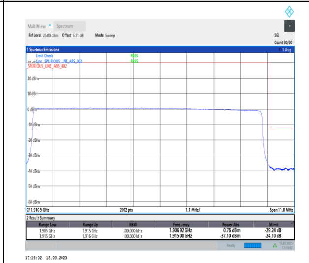
1-N25-PC3-15-10-H-6-CP-QPSK-Outer_Full-52@0-Ant1-1-seegraph-PASS-see graph
