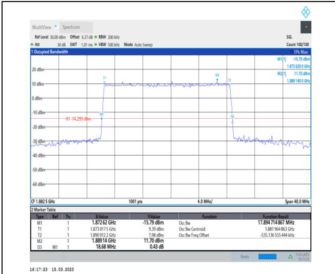
1-N25-PC3-15-20-M-3-DFT-16QAM-Outer_Full-100 @0-Ant1-17.895-18.680-≤20-PASS
