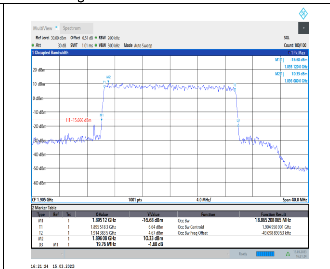
1-N25-PC3-15-20-H-7-CP-16QAM-Outer_Full-106@0 -Ant1-18.865-19.760-≤20-PASS
