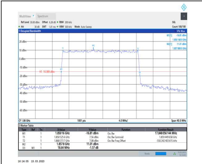
1-N25-PC3-15-20-L-4-DFT-64QAM-Outer_Full-100 @0-Ant1-17.848-18.640-≤20-PASS
