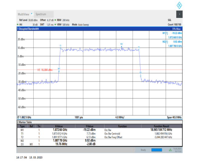
1-N25-PC3-15-20-M-6-CP-QPSK-Outer_Full-106@0 -Ant1-18.965-19.760-≤20-PASS
