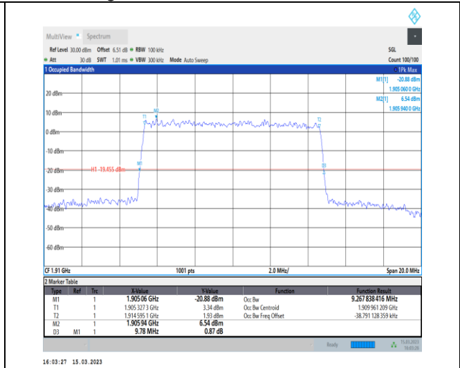
1-N25-PC3-15-10-H-9-CP-256QAM-Outer_Full-52@ 0-Ant1-9.268-9.780-≤10-PASS
