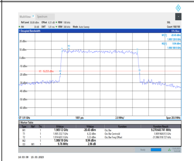
1-N25-PC3-15-10-H-7-CP-16QAM-Outer_Full-52@0 -Ant1-9.271-9.760-≤10-PASS
