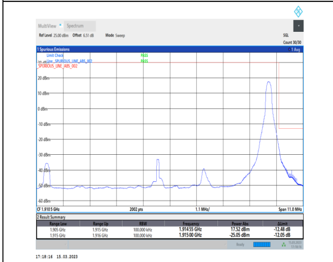
1-N25-PC3-15-10-H-5-CP-QPSK-Edge_1RB_Right-1@51-Ant1-1-seegraph-PASS-see graph
