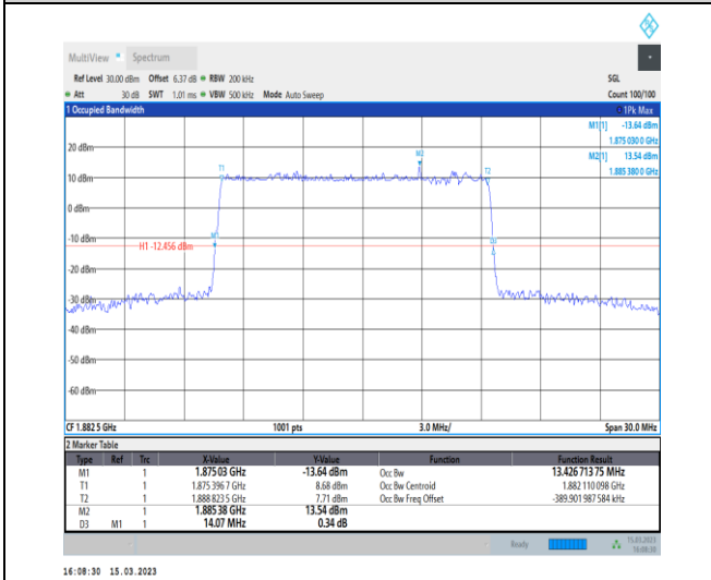
1-N25-PC3-15-15-M-4-DFT-64QAM-Outer_Full-75@ 0-Ant1-13.427-14.070-≤15-PASS
