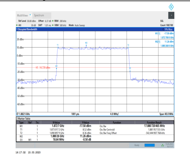
1-N25-PC3-15-20-M-4-DFT-64QAM-Outer_Full-100 @0-Ant1-17.881-18.640-≤20-PASS
