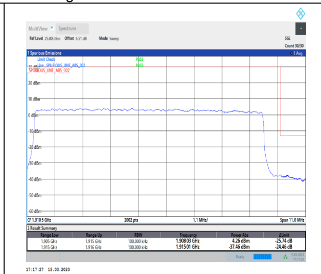
1-N25-PC3-15-10-H-3-DFT-PI2BPSK-Outer_Full-50@0-Ant1-1-seegraph-PASS-see graph
