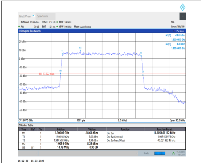
1-N25-PC3-15-15-H-9-CP-256QAM-Outer_Full-79@ 0-Ant1-14.106-14.790-≤15-PASS
