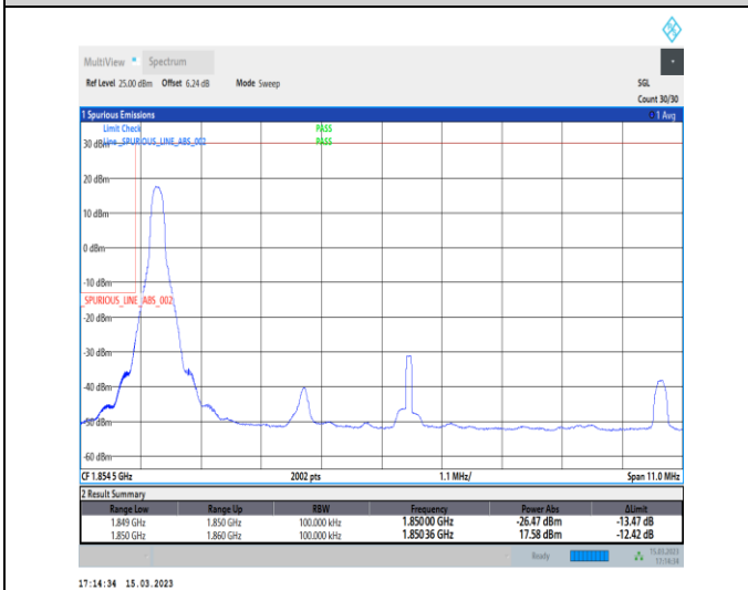
1-N25-PC3-15-10-L-4-CP-QPSK-Edge_1RB_Left-1@0-Ant1-1-seegraph-PASS-see graph
