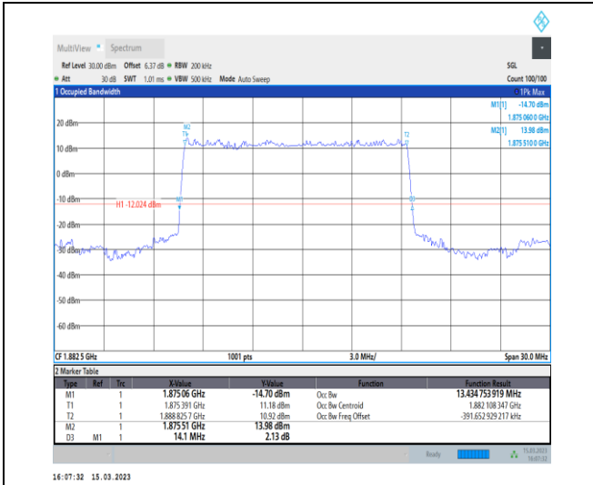
1-N25-PC3-15-15-M-2-DFT-PI2BPSK-Outer_Full-75 @0-Ant1-13.435-14.100-≤15-PASS
