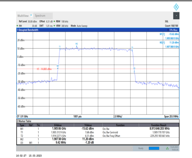
1-N25-PC3-15-10-H-3-DFT-16QAM-Outer_Full-50@ 0-Ant1-8.914-9.420-≤10-PASS
