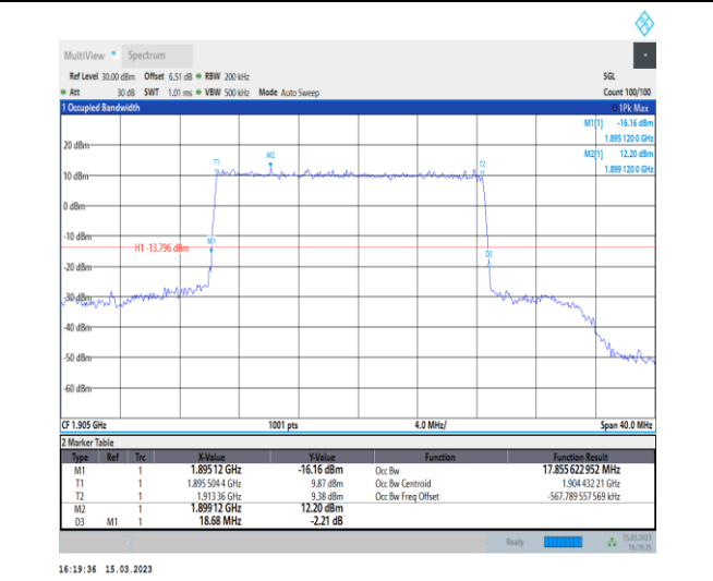
1-N25-PC3-15-20-H-1-DFT-QPSK-Outer_Full-100@ 0-Ant1-17.856-18.680-≤20-PASS
