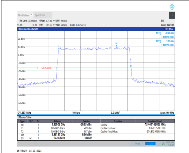
1-N25-PC3-15-15-L-5-DFT-256QAM-Outer_Full-75 @0-Ant1-13.44-14.160-≤15-PASS
