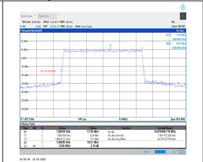
1-N25-PC3-15-15-L-8-CP-64QAM-Outer_Full-79@0-Ant1-14.078-14.850-≤15-PASS
