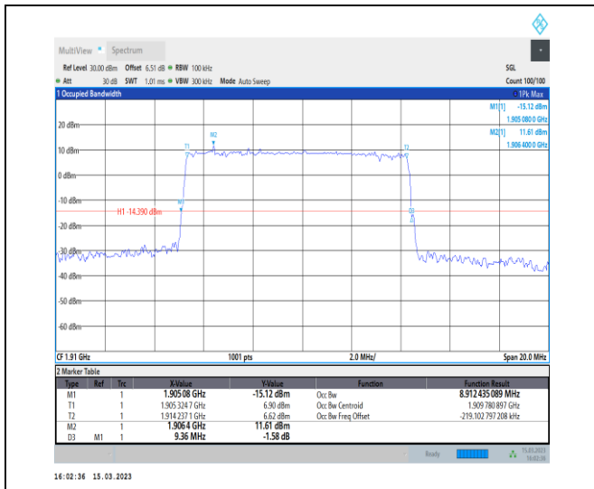
1-N25-PC3-15-10-H-4-DFT-64QAM-Outer_Full-50@ 0-Ant1-8.912-9.360-≤10-PASS
