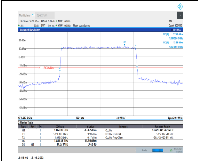
1-N25-PC3-15-15-L-1-DFT-QPSK-Outer_Full-75@0- Ant1-13.429-14.070-≤15-PASS
