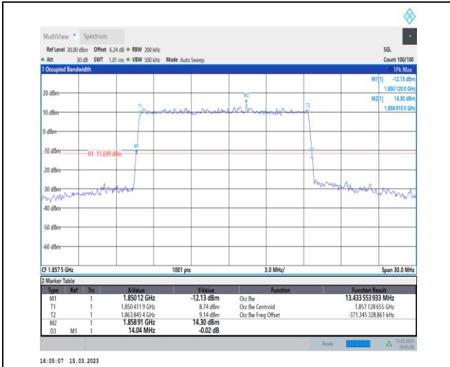
1-N25-PC3-15-15-L-3-DFT-16QAM-Outer_Full-75@ 0-Ant1-13.434-14.040-≤15-PASS
