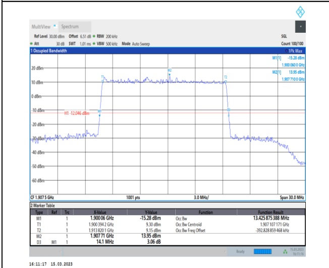
1-N25-PC3-15-15-H-3-DFT-16QAM-Outer_Full-75@ 0-Ant1-13.426-14.100-≤15-PASS
