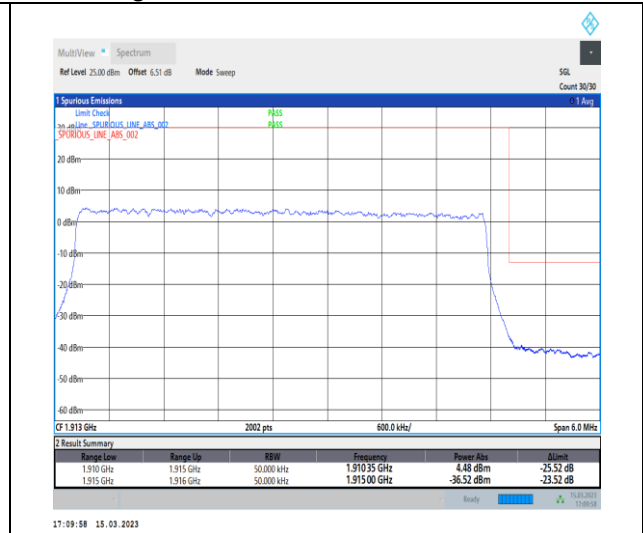
1-N25-PC3-15-5-H-3-DFT-PI2BPSK-Outer_Full-25@0-Ant1-1-seegraph-PASS-see graph
