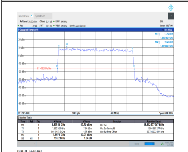
1-N25-PC3-15-20-H-8-CP-64QAM-Outer_Full-106@0 -Ant1-18.893-19.720-≤20-PASS
