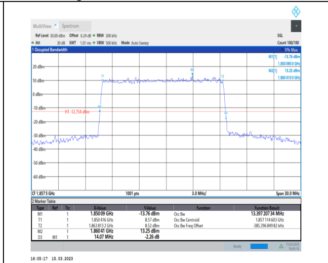
1-N25-PC3-15-15-L-4-DFT-64QAM-Outer_Full-75@ 0-Ant1-13.397-14.070-≤15-PASS
