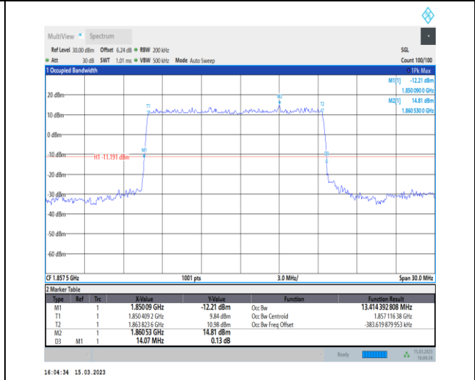
1-N25-PC3-15-15-L-2-DFT-PI2BPSK-Outer_Full-75 @0-Ant1-13.414-14.070-≤15-PASS
