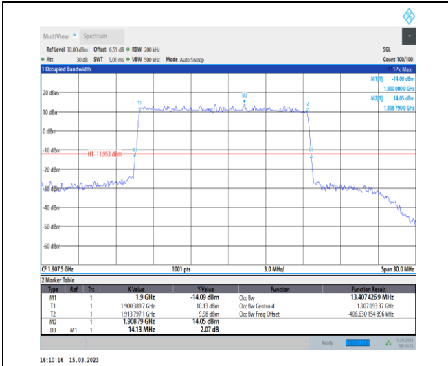
1-N25-PC3-15-15-H-1-DFT-QPSK-Outer_Full-75@0 -Ant1-13.407-14.130-≤15-PASS
