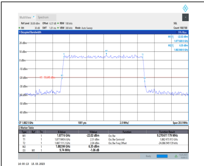
1-N25-PC3-15-10-M-9-CP-256QAM-Outer_Full-52@ 0-Ant1-9.271-9.740-≤10-PASS
