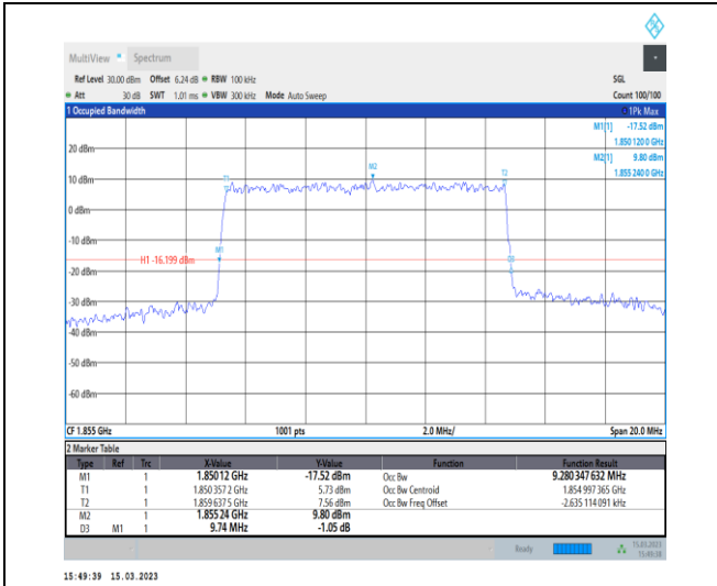
1-N25-PC3-15-10-L-6-CP-QPSK-Outer_Full-52@0-Ant1-9.28-9.740-≤10-PASS
