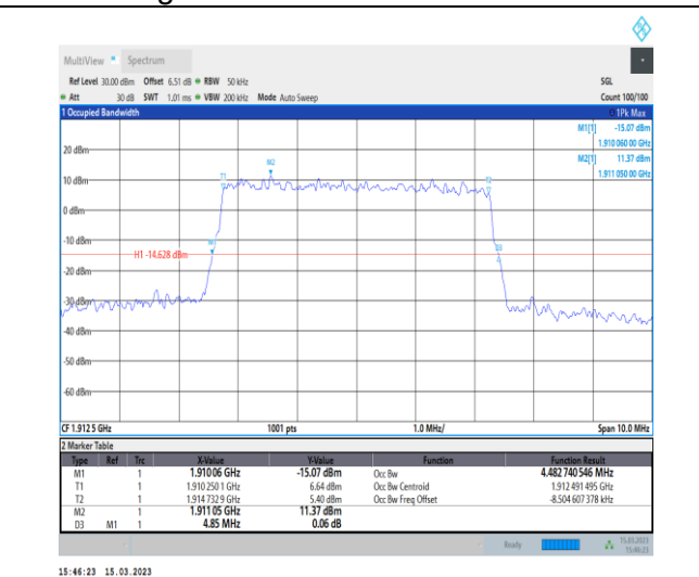
1-N25-PC3-15-5-H-4-DFT-64QAM-Outer_Full-25@0- Ant1-4.483-4.850-≤5-PASS
