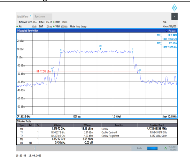
1-N25-PC3-15-5-L-6-CP-QPSK-Outer_Full-25@0-An t1-4.473-5.450-≤5-PASS
