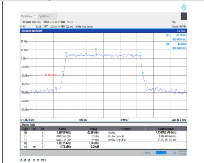
1-N25-PC3-15-5-M-9-CP-256QAM-Outer_Full-25@0-Ant1-4.459-4.780-≤5-PASS
