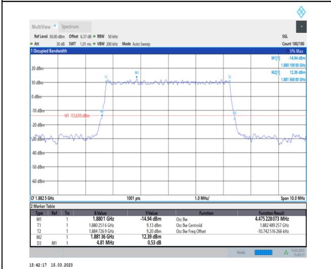
1-N25-PC3-15-5-M-2-DFT-PI2BPSK-Outer_Full-25@0-Ant1-4.475-4.810-≤5-PASS
