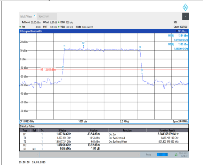
1-N25-PC3-15-10-M-2-DFT-PI2BPSK-Outer_Full-50 @0-Ant1-8.948-9.360-≤10-PASS
