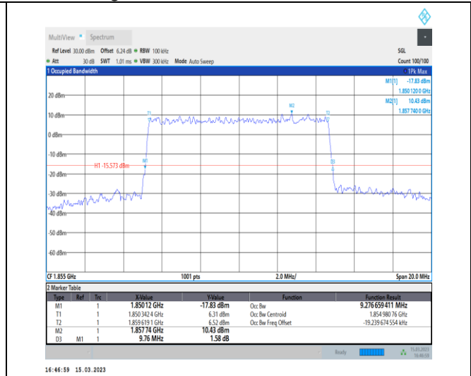
1-N25-PC3-15-10-L-7-CP-16QAM-Outer_Full-52@0-Ant1-9.277-9.760-≤10-PASS
