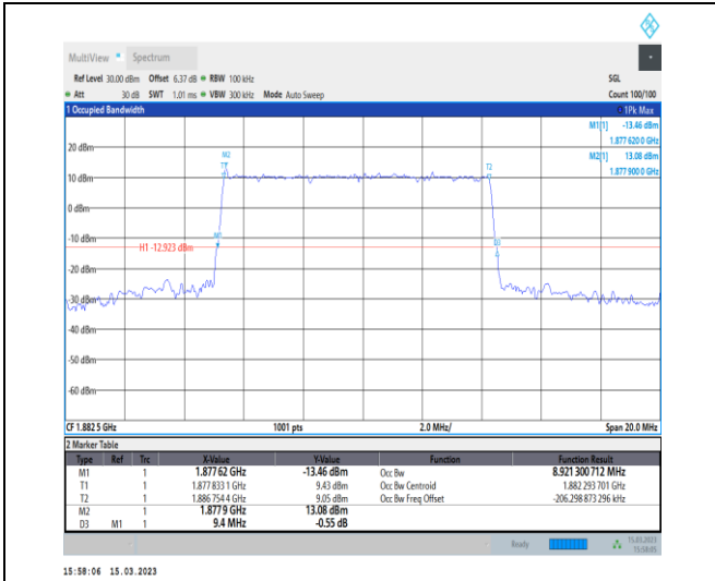
1-N25-PC3-15-10-M-1-DFT-QPSK-Outer_Full-50@0 -Ant1-8.921-9.400-≤10-PASS
