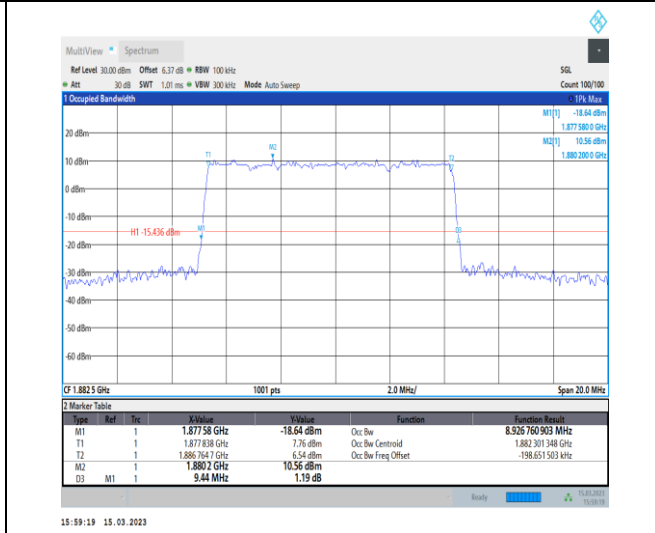
1-N25-PC3-15-10-M-4-DFT-64QAM-Outer_Full-50@ 0-Ant1-8.927-9.440-≤10-PASS
