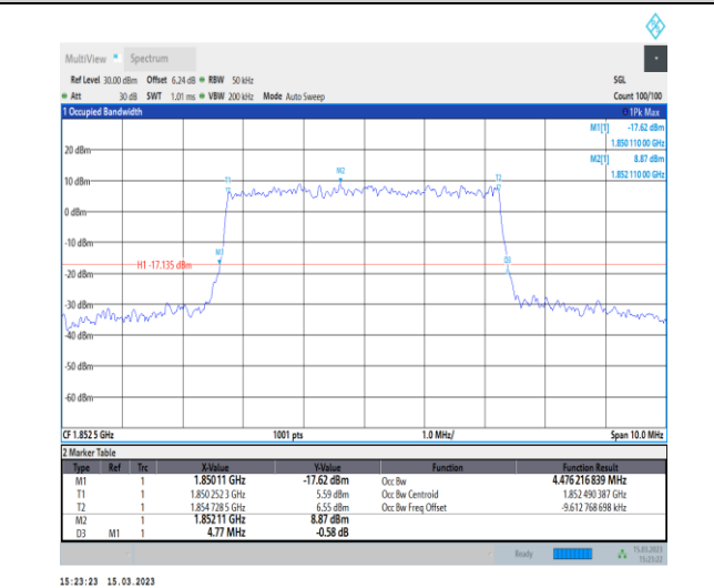
1-N25-PC3-15-5-L-8-CP-64QAM-Outer_Full-25@0-A nt1-4.476-4.770-≤5-PASS
