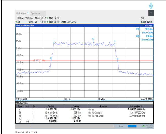
1-N25-PC3-15-5-H-5-DFT-256QAM-Outer_Full-25@ 0-Ant1-4.459-4.840-≤5-PASS
