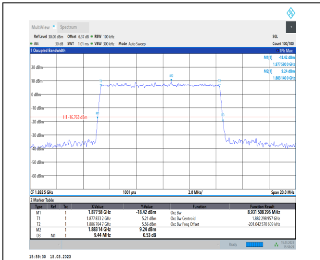
1-N25-PC3-15-10-M-5-DFT-256QAM-Outer_Full-50@0-Ant1-8.932-9.440-≤10-PASS
