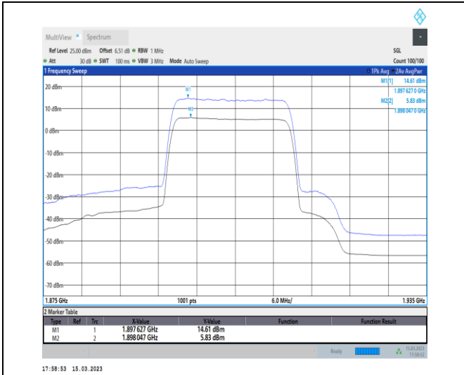
1-N25-PC3-15-20-H-1-DFT-256QAM-Outer_Full-100 @0-Ant1-8.78-100%-0.00-8.78-PASS-≤13
