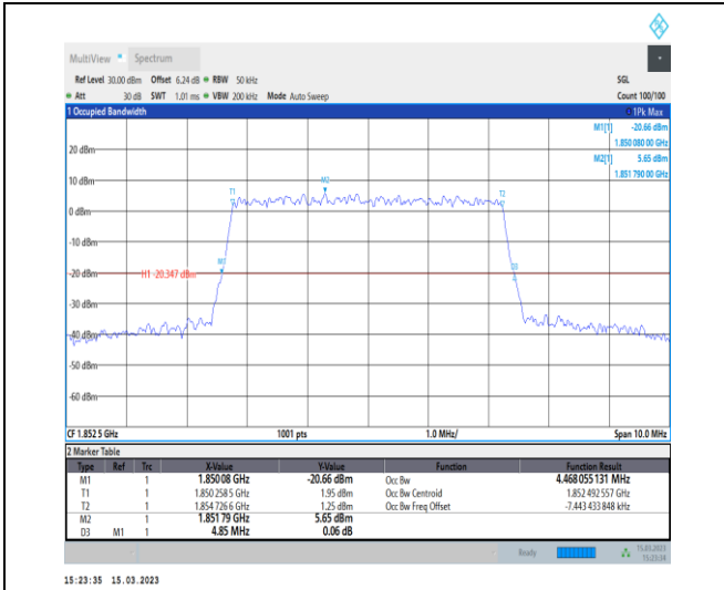
1-N25-PC3-15-5-L-9-CP-256QAM-Outer_Full-25@0-Ant1-4.468-4.850-≤5-PASS
