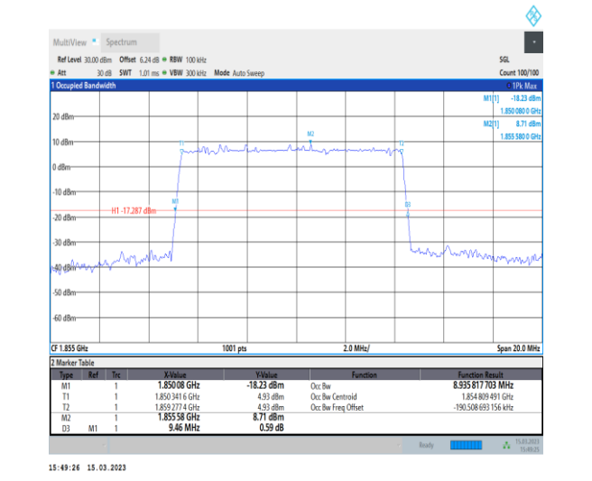
1-N25-PC3-15-10-L-5-DFT-256QAM-Outer_Full-50 @0-Ant1-8.936-9.460-≤10-PASS
