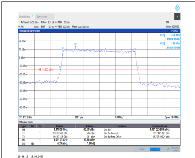
1-N25-PC3-15-5-H-3-DFT-16QAM-Outer_Full-25@0 -Ant1-4.461-4.790-≤5-PASS
