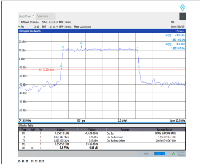
1-N25-PC3-15-10-L-2-DFT-PI2BPSK-Outer_Full-50 @0-Ant1-8.903-9.300-≤10-PASS
