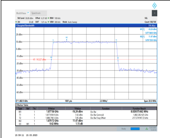
1-N25-PC3-15-10-M-3-DFT-16QAM-Outer_Full-50@ 0-Ant1-8.928-9.420-≤10-PASS
