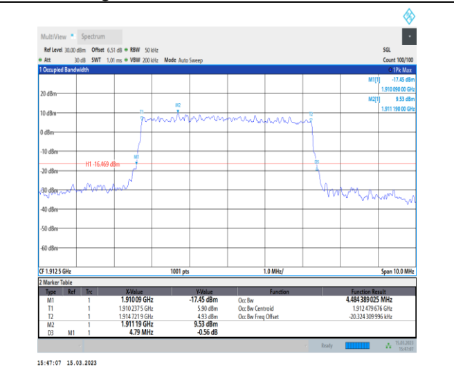
1-N25-PC3-15-5-H-8-CP-64QAM-Outer_Full-25@0-Ant1-4.484-4.790-≤5-PASS
