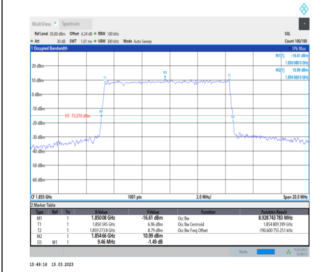
1-N25-PC3-15-10-L-4-DFT-64QAM-Outer_Full-50 @0-Ant1-8.929-9.460-≤10-PASS
