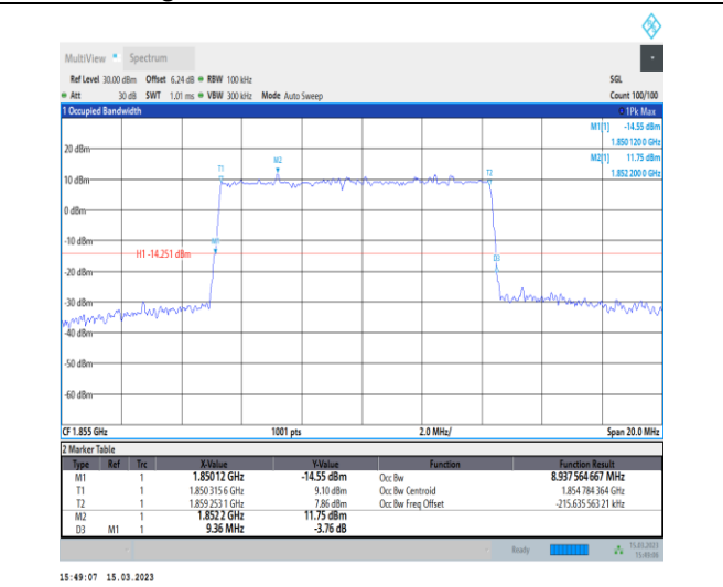
1-N25-PC3-15-10-L-3-DFT-16QAM-Outer_Full-50 @0-Ant1-8.938-9.360-≤10-PASS
