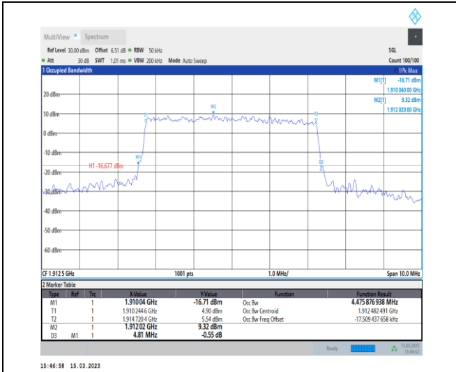
1-N25-PC3-15-5-H-7-CP-16QAM-Outer_Full-25@0-Ant1-4.476-4.810-≤5-PASS
