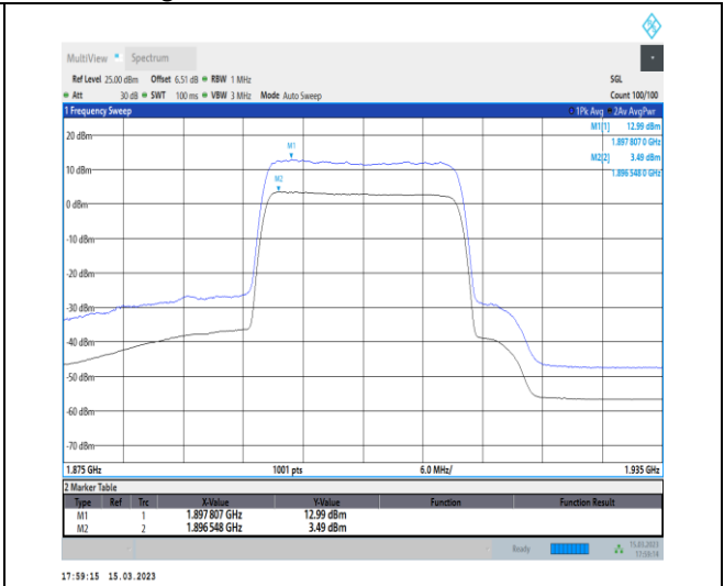
1-N25-PC3-15-20-H-2-CP-256QAM-Outer_Full-106 @0-Ant1-9.50-100%-0.00-9.50-PASS-≤13
