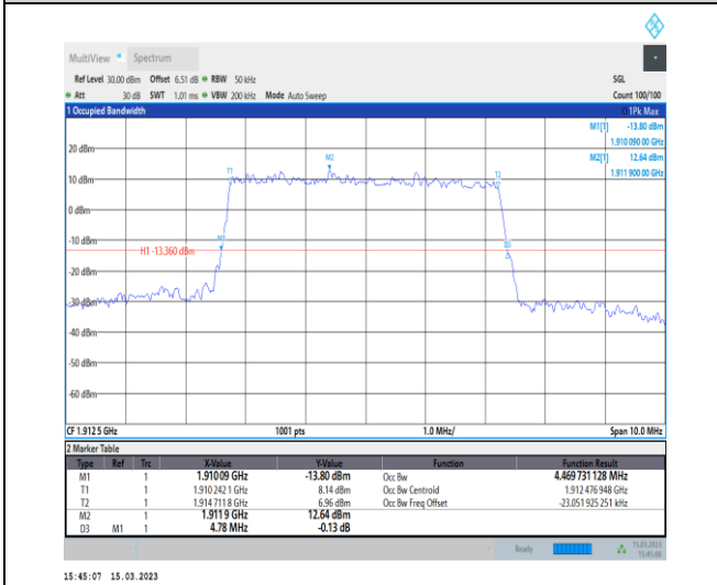
1-N25-PC3-15-5-H-1-DFT-QPSK-Outer_Full-25@0-Ant1-4.47-4.780-≤5-PASS
