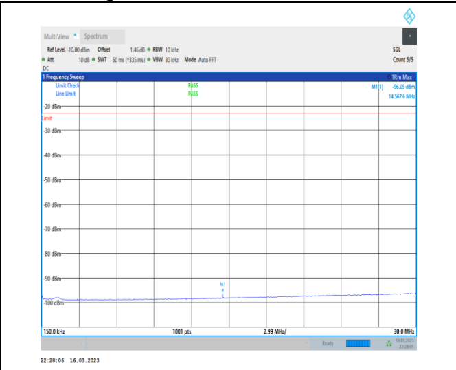
1-N14-PC3-15-10-M-1-DFT-PI2BPSK-Inner_1RB_Lef t-1@1-0.15-30-Ant7-14.57--96.05--23-PASS
