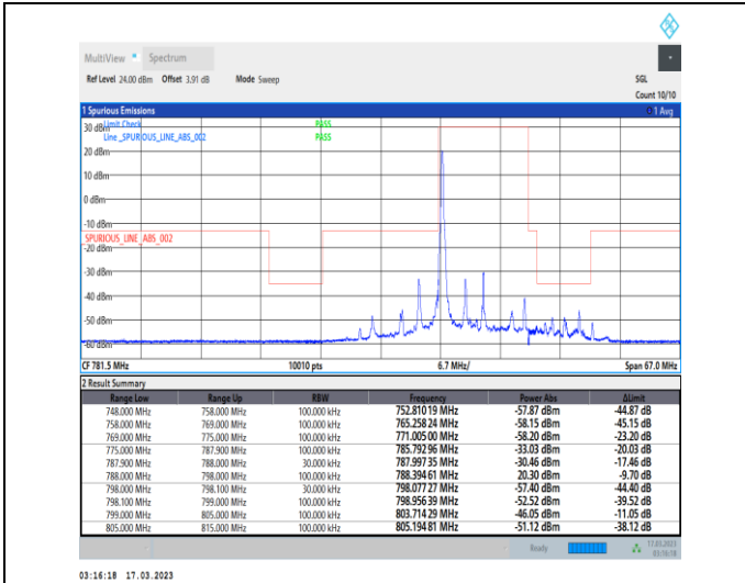
1-N14-PC3-15-10-L-1-DFT-PI2BPSK-Edge_1RB_Left-1@0-Ant7-1--PASS-see graph
