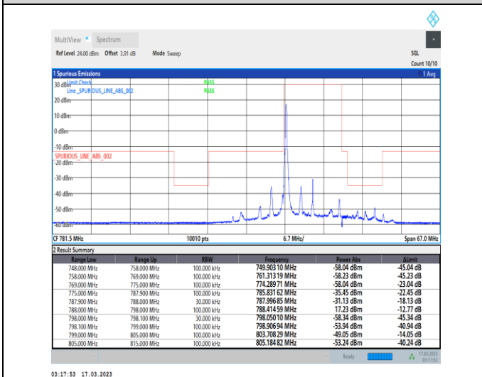
1-N14-PC3-15-10-L-4-CP-QPSK-Edge_1RB_Left-1@0-Ant7-1--PASS-see graph
