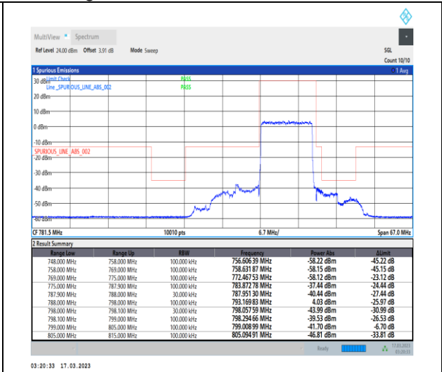
1-N14-PC3-15-10-H-3-DFT-PI2BPSK-Outer_Full-5 0@0-Ant7-1--PASS-see graph
