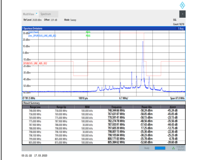
1-N14-PC3-15-10-H-5-CP-QPSK-Edge_1RB_Righ t-1@51-Ant7-1--PASS-see graph
