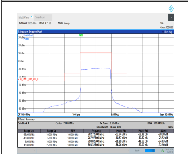
NTNV_N14_15_10_L_TID4_-25.00_-10.00_100.00_#1
