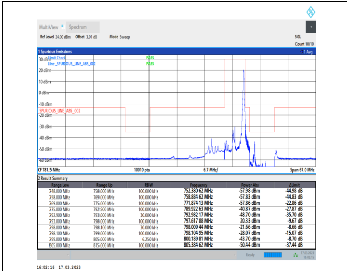
1-N14-PC3-15-5-H-2-DFT-PI2BPSK-Edge_1RB_Right-1@24-Ant7-1--PASS-see graph
