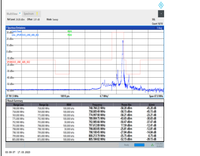
1-N14-PC3-15-5-H-5-CP-QPSK-Edge_1RB_Right-1@24-Ant7-1--PASS-see graph
