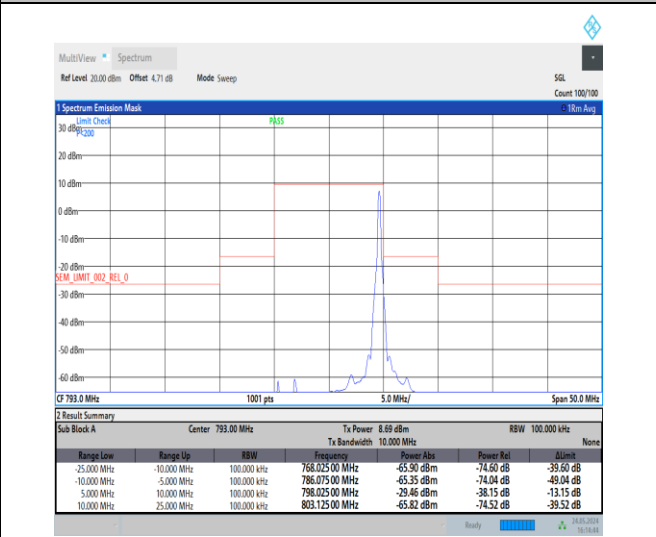
NTNV_N14_15_10_H_TID6_-25.00_-10.00_100.00_#1
