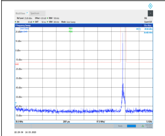
1-N14-PC3-15-10-H-1-DFT-PI2BPSK-Inner_1RB_L eft-1@1-30-1000-Ant7-30.49--59.84--13-PASS
