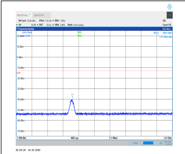
1-N14-PC3-15-10-H-1-DFT-PI2BPSK-Inner_1RB_L eft-1@1-1559-1610-Ant7-1577.30--38.91--13-PASS
