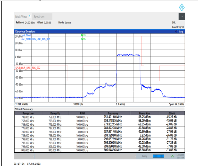
1-N14-PC3-15-10-L-3-DFT-PI2BPSK-Outer_Full-50@0-Ant7-1--PASS-see graph
