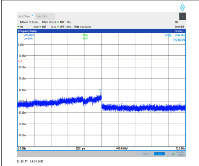
1-N14-PC3-15-10-M-1-DFT-PI2BPSK-Inner_1RB_L eft-1@1-3000-12000-Ant7-7443.30--43.64--13-PASS
