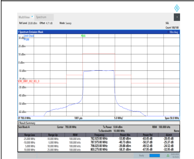
NTNV_N14_15_10_H_TID4_-25.00_-10.00_100.00_#1
