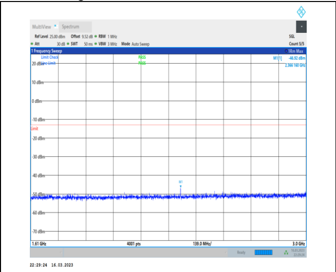
1-N14-PC3-15-10-H-1-DFT-PI2BPSK-Inner_1RB_L eft-1@1-1610-3000-Ant7-2366.16--46.92--13-PASS
