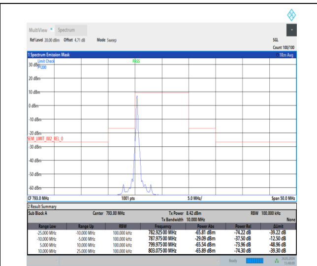
NTNV_N14_15_10_L_TID2_-25.00_-10.00_100.00_#1
