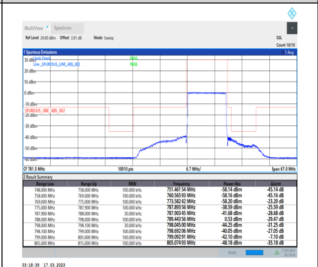
1-N14-PC3-15-10-L-6-CP-QPSK-Outer_Full-52@0-Ant7-1--PASS-see graph
