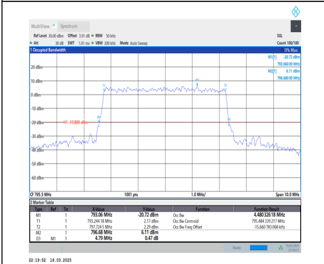
1-N14-PC3-15-5-H-9-CP-256QAM-Outer_Full-25@0-Ant7-4.48-4.790-≤5-PASS
