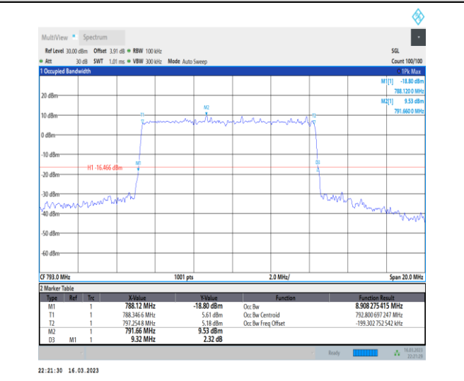
1-N14-PC3-15-10-L-5-DFT-256QAM-Outer_Full-50 @0-Ant7-8.908-9.320-≤10-PASS
