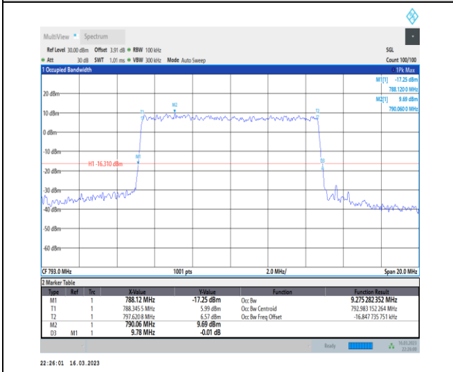
1-N14-PC3-15-10-H-6-CP-QPSK-Outer_Full-52@0- Ant7-9.275-9.780-≤10-PASS
