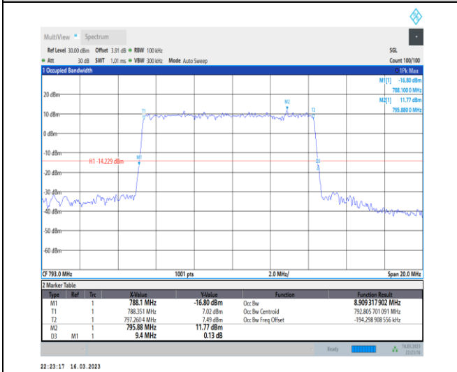
1-N14-PC3-15-10-M-3-DFT-16QAM-Outer_Full-50@0-Ant7-8.909-9.400-≤10-PASS
