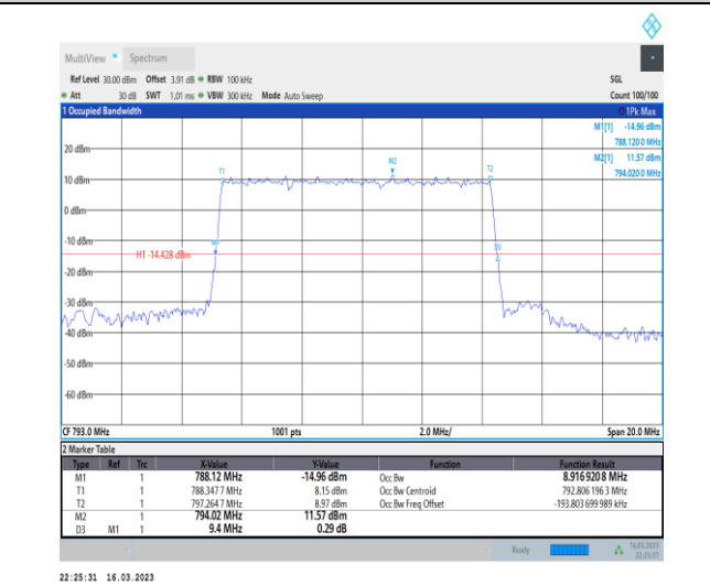
1-N14-PC3-15-10-H-3-DFT-16QAM-Outer_Full-50@ 0-Ant7-8.917-9.400-≤10-PASS
