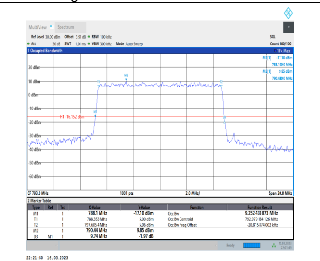
1-N14-PC3-15-10-L-7-CP-16QAM-Outer_Full-52@0-Ant7-9.252-9.740-≤10-PASS
