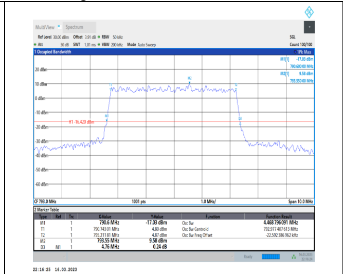
1-N14-PC3-15-5-M-5-DFT-256QAM-Outer_Full-25@0-Ant7-4.469-4.760-≤5-PASS
