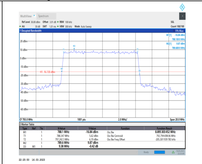
1-N14-PC3-15-10-H-5-DFT-256QAM-Outer_Full-50 @0-Ant7-8.895-9.380-≤10-PASS
