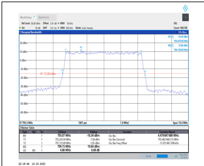
1-N14-PC3-15-5-H-3-DFT-16QAM-Outer_Full-25@0-Ant7-4.48-4.860-<math>\leq 5</math>-PASS
