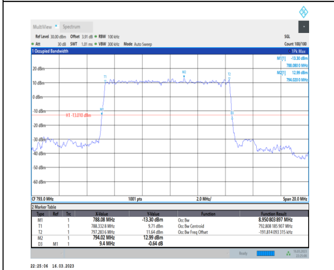
1-N14-PC3-15-10-H-2-DFT-PI2BPSK-Outer_Full-50 @0-Ant7-8.951-9.400-≤10-PASS
