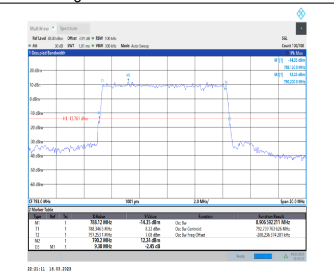
1-N14-PC3-15-10-L-3-DFT-16QAM-Outer_Full-50 @0-Ant7-8.907-9.380-≤10-PASS
