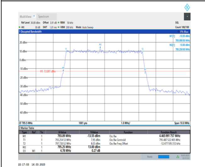
1-N14-PC3-15-5-H-1-DFT-QPSK-Outer_Full-25@0-Ant7-4.466-4.780-≤5-PASS
