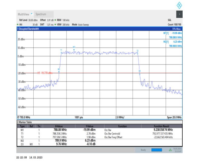
1-N14-PC3-15-10-L-9-CP-256QAM-Outer_Full-52@0-Ant7-9.238-9.760-≤10-PASS
