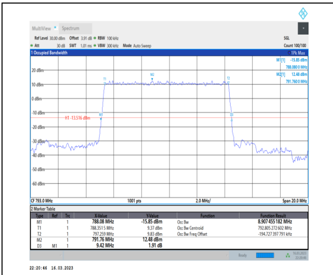
1-N14-PC3-15-10-L-2-DFT-PI2BPSK-Outer_Full-50 @0-Ant7-8.907-9.420-≤10-PASS
