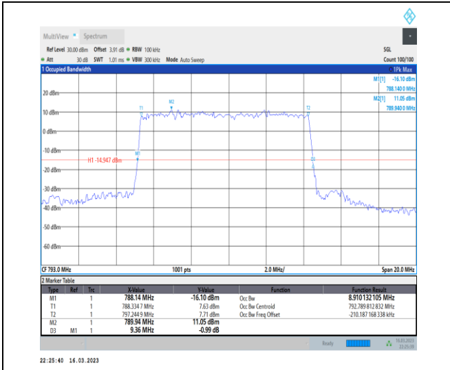
1-N14-PC3-15-10-H-4-DFT-64QAM-Outer_Full-50@ 0-Ant7-8.91-9.360-≤10-PASS
