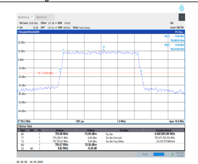
1-N14-PC3-15-5-H-4-DFT-64QAM-Outer_Full-25@0-Ant7-4.459-4.820-<math>\leq 5</math>-PASS
