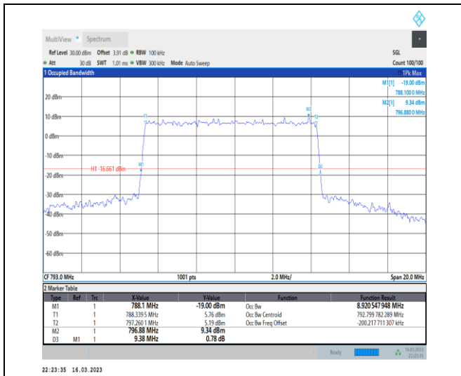
1-N14-PC3-15-10-M-5-DFT-256QAM-Outer_Full-50@0-Ant7-8.921-9.380-≤10-PASS
