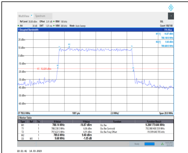
1-N14-PC3-15-10-L-6-CP-QPSK-Outer_Full-52@0-Ant7-9.284-9.680-≤10-PASS
