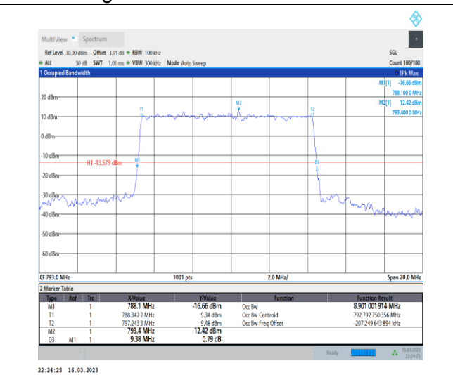
1-N14-PC3-15-10-H-1-DFT-QPSK-Outer_Full-50@0- Ant7-8.901-9.380-≤10-PASS
