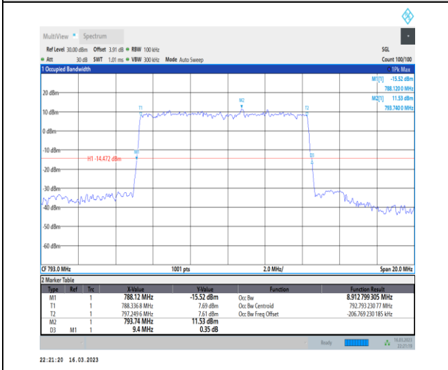
1-N14-PC3-15-10-L-4-DFT-64QAM-Outer_Full-50 @0-Ant7-8.913-9.400-≤10-PASS
