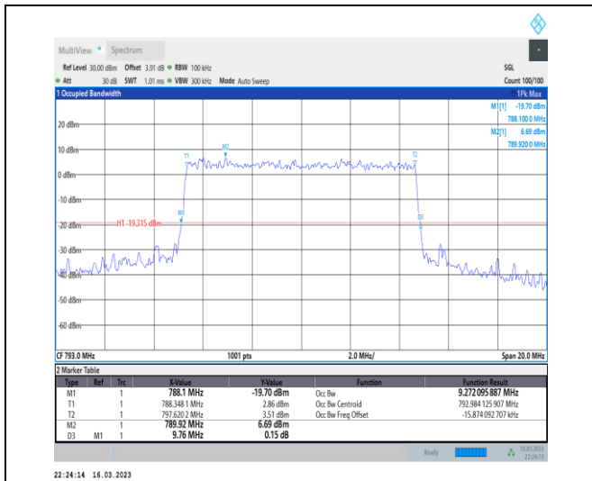
1-N14-PC3-15-10-M-9-CP-256QAM-Outer_Full-52@ 0-Ant7-9.272-9.760-≤10-PASS
