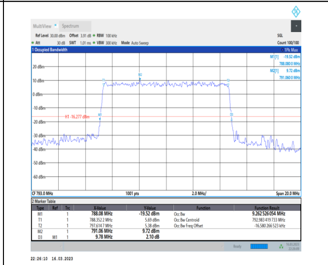
1-N14-PC3-15-10-H-7-CP-16QAM-Outer_Full-52@0 -Ant7-9.263-9.780-≤10-PASS
