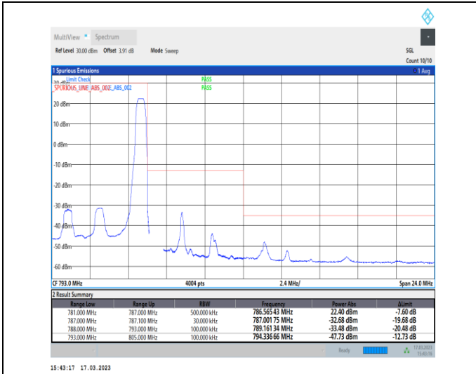
1-N13-PC3-15-10-H-2-DFT-PI2BPSK-Edge_1RB_Righ t-1@51-Ant7-1--PASS-see graph
