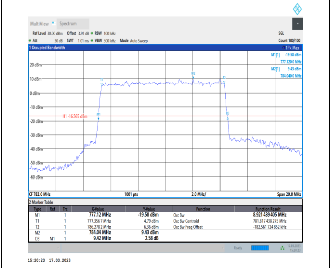
1-N13-PC3-15-10-M-5-DFT-256QAM-Outer_Full-50 @0-Ant7-8.921-9.420-≤10-PASS
