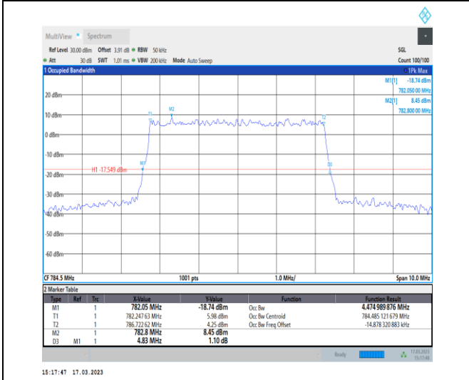
1-N13-PC3-15-5-H-5-DFT-256QAM-Outer_Full-25@0-Ant7-4.475-4.830-≤5-PASS
