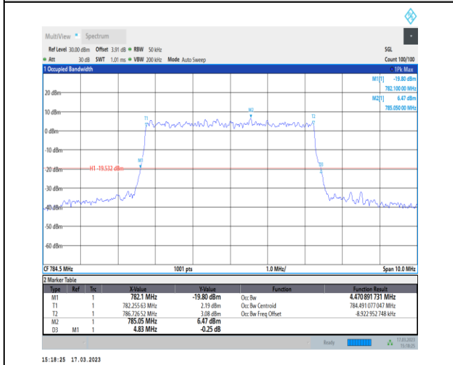
1-N13-PC3-15-5-H-9-CP-256QAM-Outer_Full-25@0-Ant7-4.471-4.830-≤5-PASS
