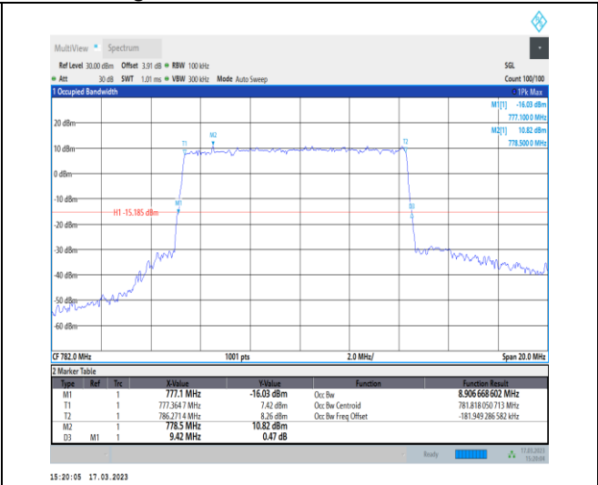
1-N13-PC3-15-10-M-3-DFT-16QAM-Outer_Full-50 @0-Ant7-8.907-9.420-≤10-PASS
