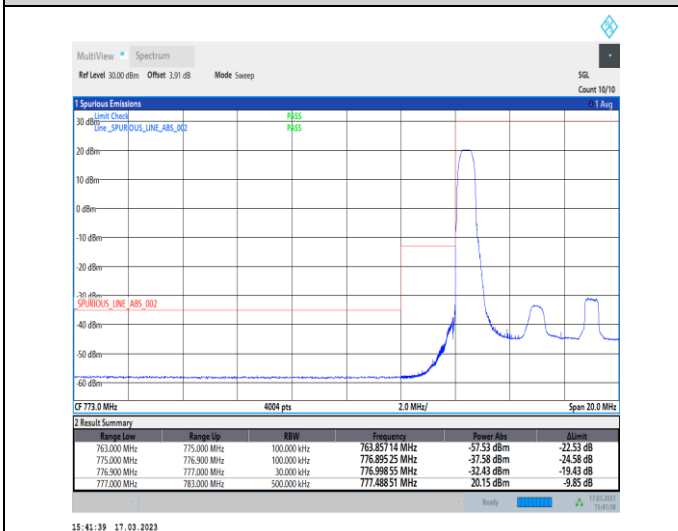
1-N13-PC3-15-10-L-4-CP-QPSK-Edge_1RB_Left-1@0-Ant7-1--PASS-see graph
