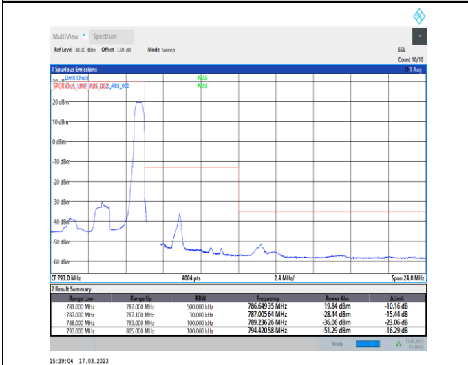
1-N13-PC3-15-5-H-5-CP-QPSK-Edge_1RB_Right-1@24-Ant7-1--PASS-see graph
