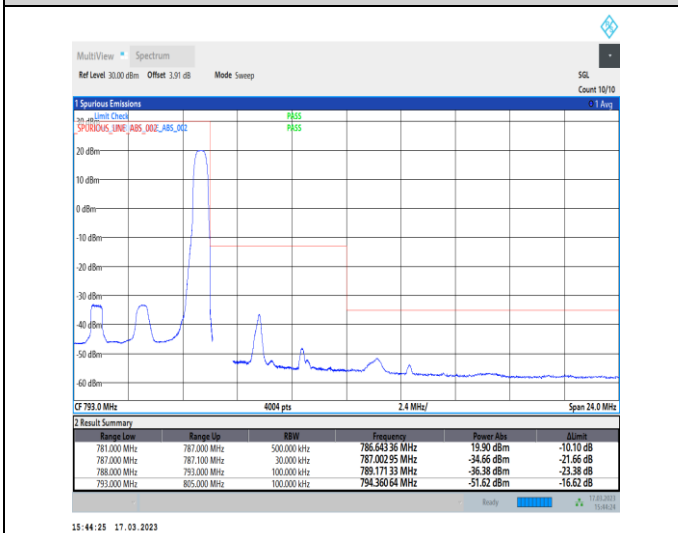
1-N13-PC3-15-10-H-5-CP-QPSK-Edge_1RB_Righ t-1 @51-Ant7-1--PASS-see graph
