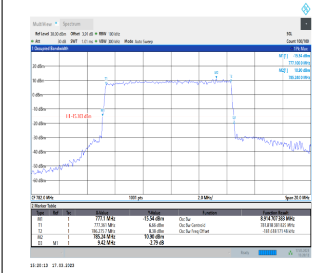
1-N13-PC3-15-10-M-4-DFT-64QAM-Outer_Full-50 @0-Ant7-8.915-9.420-≤10-PASS
