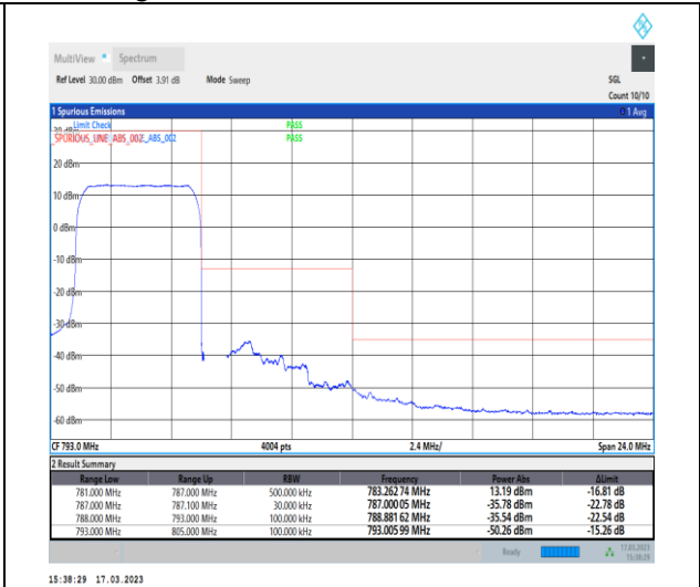
1-N13-PC3-15-5-H-3-DFT-PI2BPSK-Outer_Full-25@0-Ant7-1--PASS-see graph
