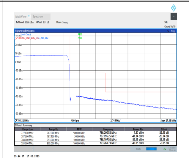
1-N13-PC3-15-10-H-6-CP-QPSK-Outer_Full-52@ 0-Ant7-1--PASS-see graph
