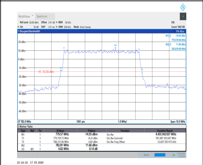
1-N13-PC3-15-5-M-3-DFT-16QAM-Outer_Full-25@0-Ant7-4.455-4.820-≤5-PASS
