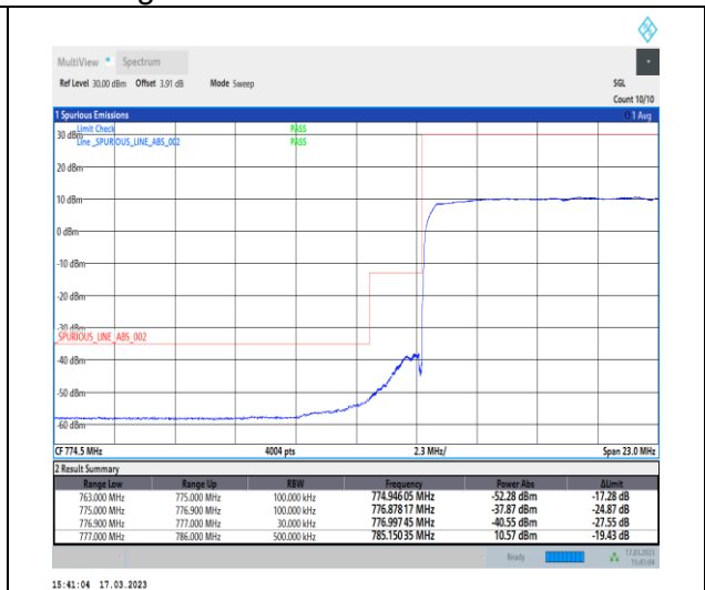
1-N13-PC3-15-10-L-3-DFT-PI2BPSK-Outer_Full-50@0-Ant7-1--PASS-see graph
