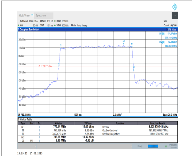
1-N13-PC3-15-10-M-2-DFT-PI2BPSK-Outer_Full-50 @0-Ant7-8.904-9.360-≤10-PASS
