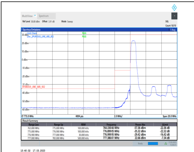
1-N13-PC3-15-10-L-1-DFT-PI2BPSK-Edge_1RB_Left-1@0-Ant7-1--PASS-see graph
