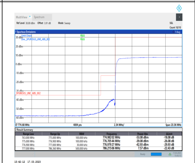
1-N13-PC3-15-10-L-6-CP-QPSK-Outer_Full-52@0-Ant7-1--PASS-see graph
