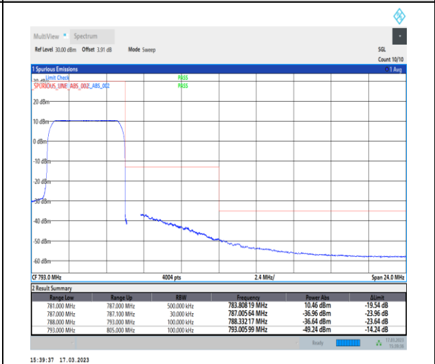
1-N13-PC3-15-5-H-6-CP-QPSK-Outer_Full-25@0-Ant7-1--PASS-see graph
