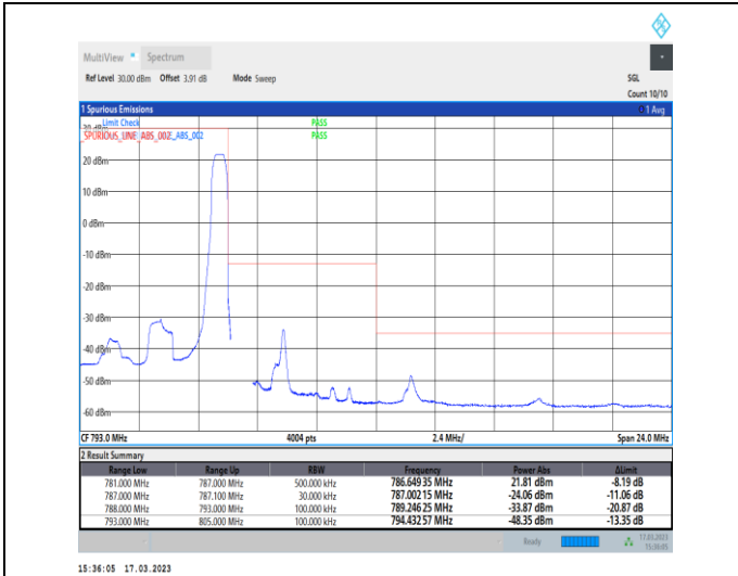
1-N13-PC3-15-5-H-2-DFT-PI2BPSK-Edge_1RB_Right-1@24-Ant7-1--PASS-see graph
