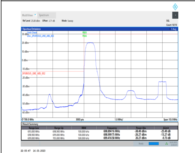
1-N12-PC3-15-10-L-4-CP-QPSK-Edge_1RB_Left-1@0-Ant7-1--PASS-see graph
