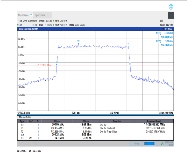
1-N12-PC3-15-15-M-4-DFT-64QAM-Outer_Full-75 @0-Ant7-13.426-14.100-≤15-PASS
