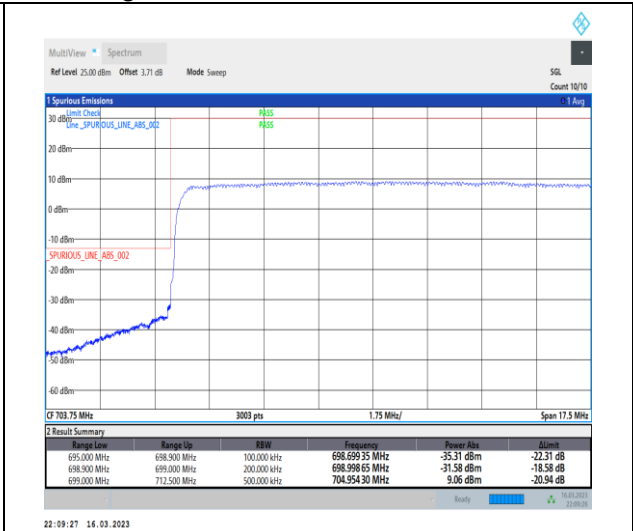
1-N12-PC3-15-15-L-3-DFT-PI2BPSK-Outer_Full-75@0-Ant7-1--PASS-see graph
