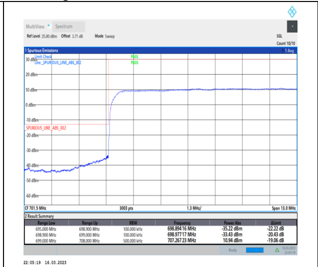
1-N12-PC3-15-10-L-3-DFT-PI2BPSK-Outer_Full-50@0-Ant7-1--PASS-see graph
