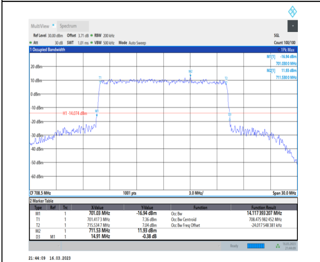
1-N12-PC3-15-15-H-7-CP-16QAM-Outer_Full-79@0 -Ant7-14.117-14.910-≤15-PASS
