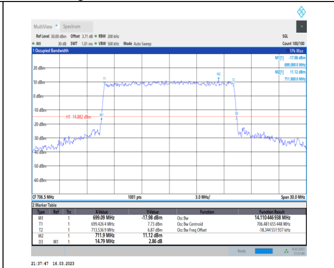
1-N12-PC3-15-15-L-8-CP-64QAM-Outer_Full-79@0-Ant7-14.11-14.790-≤15-PASS
