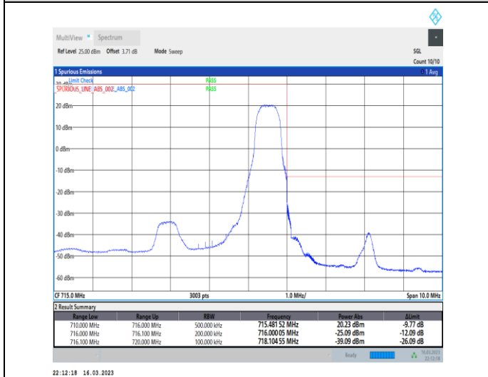
1-N12-PC3-15-15-H-5-CP-QPSK-Edge_1RB_Right-1 @78-Ant7-1--PASS-see graph
