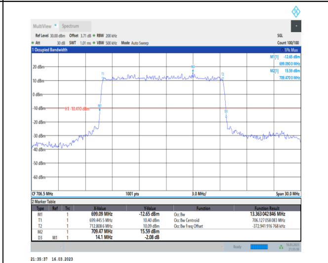
1-N12-PC3-15-15-L-2-DFT-PI2BPSK-Outer_Full-75@0- Ant7-13.363-14.100-≤15-PASS
