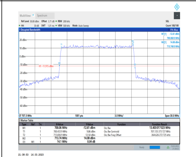
1-N12-PC3-15-15-M-1-DFT-QPSK-Outer_Full-75@0-Ant7-13.403-14.100-≤15-PASS
