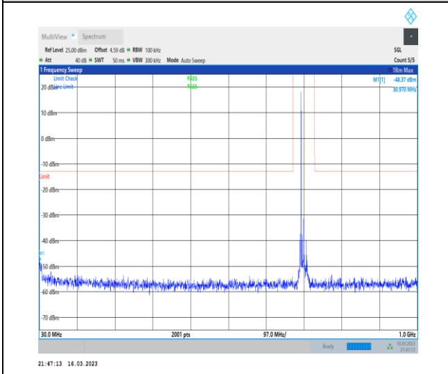
1-N12-PC3-15-15-H-1-DFT-PI2BPSK-Inner_1RB_L eft-1@1-30-1000-Ant7-30.97--48.37--13-PASS
