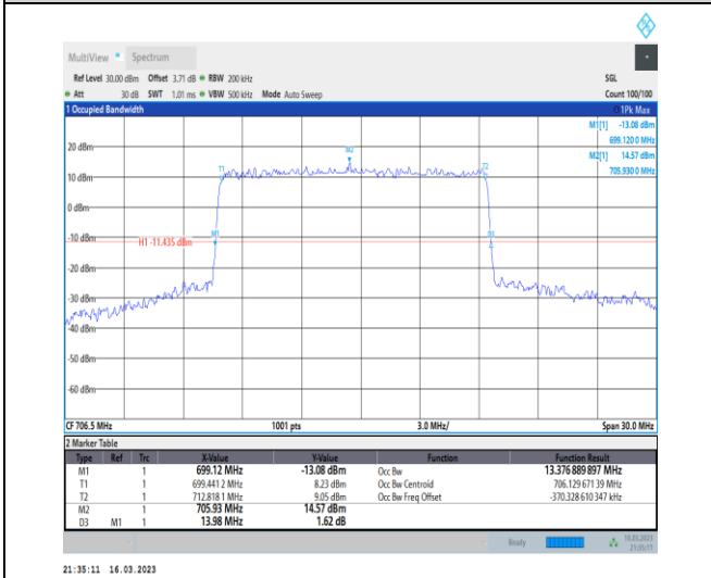
1-N12-PC3-15-15-L-1-DFT-QPSK-Outer_Full-75@0- Ant7-13.377-13.980-≤15-PASS
