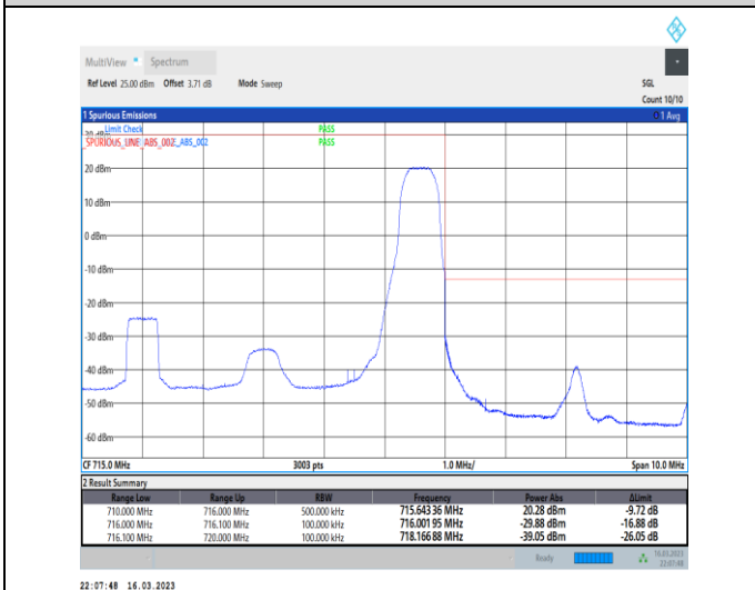
1-N12-PC3-15-10-H-5-CP-QPSK-Edge_1RB_Right-1 @51-Ant7-1--PASS-see graph
