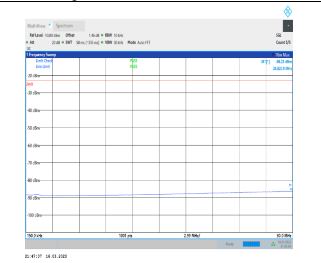
1-N12-PC3-15-15-H-1-DFT-PI2BPSK-Inner_1RB_Lef t-1@1-0.15-30-Ant7-29.82--86.23--23-PASS
