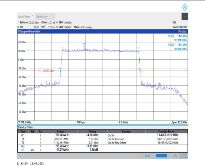
1-N12-PC3-15-15-H-4-DFT-64QAM-Outer_Full-75@0-Ant7-13.406-14.070-≤15-PASS
