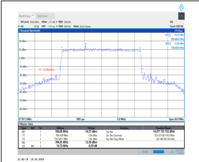
1-N12-PC3-15-15-M-6-CP-QPSK-Outer_Full-79@0-Ant7-14.072-14.730-≤15-PASS
