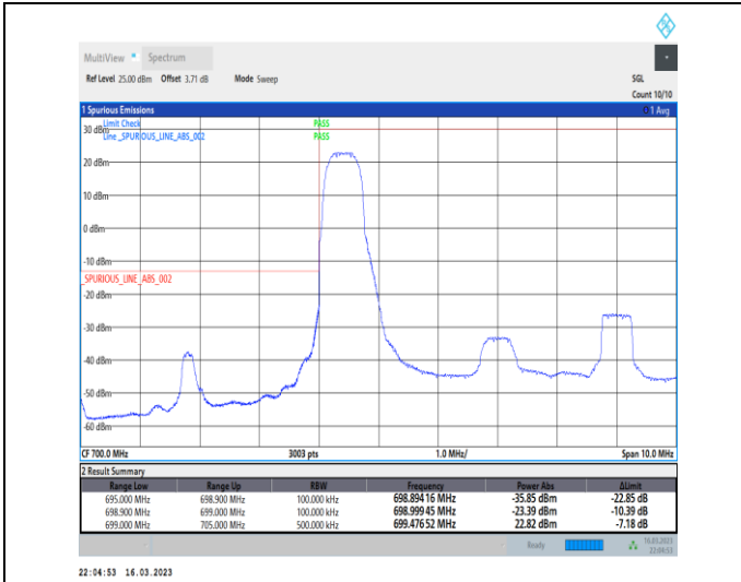
1-N12-PC3-15-10-L-1-DFT-PI2BPSK-Edge_1RB_Left-1@0-Ant7-1--PASS-see graph
