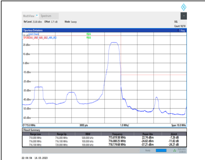
1-N12-PC3-15-10-H-2-DFT-PI2BPSK-Edge_1RB_Righ t-1@51-Ant7-1--PASS-see graph
