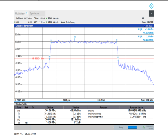
1-N12-PC3-15-15-H-6-CP-QPSK-Outer_Full-79@0-Ant7-14.08-14.760-≤15-PASS
