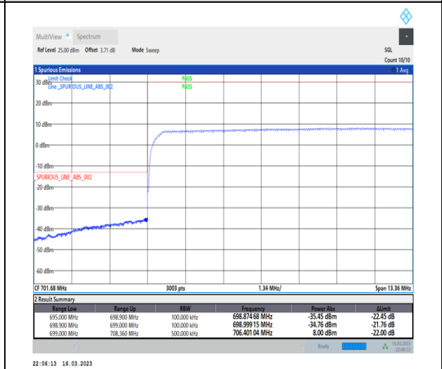
1-N12-PC3-15-10-L-6-CP-QPSK-Outer_Full-52@0-Ant7-1--PASS-see graph
