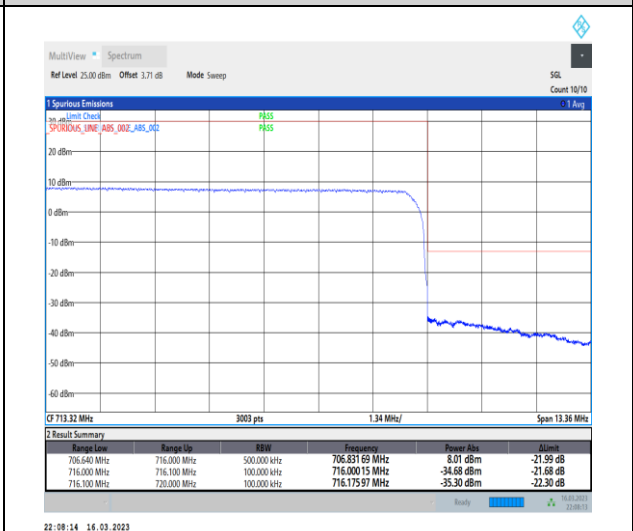
1-N12-PC3-15-10-H-6-CP-QPSK-Outer_Full-52@ 0-Ant7-1--PASS-see graph
