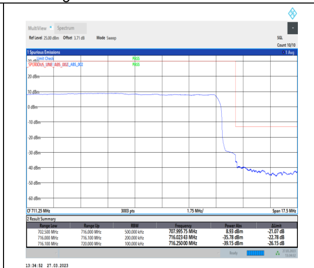
1-N12-PC3-15-15-H-3-DFT-PI2BPSK-Outer_Full-7 5@0-Ant7-1--PASS-see graph
