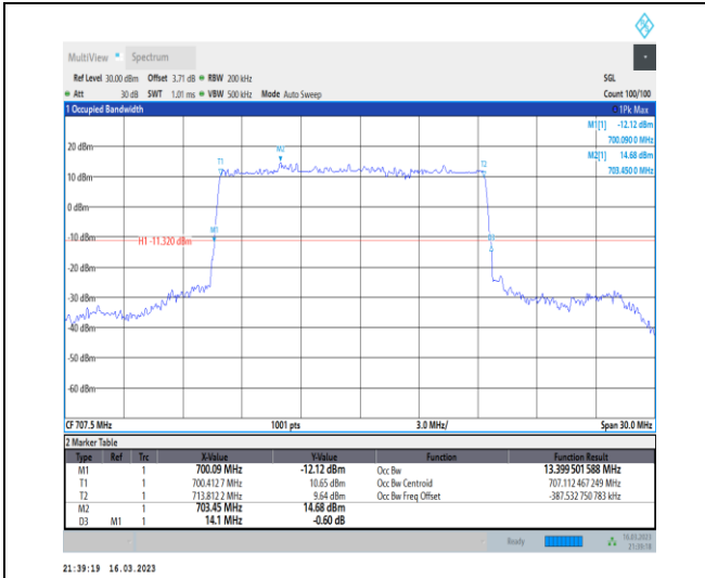
1-N12-PC3-15-15-M-2-DFT-PI2BPSK-Outer_Full-75 @0-Ant7-13.4-14.100-≤15-PASS
