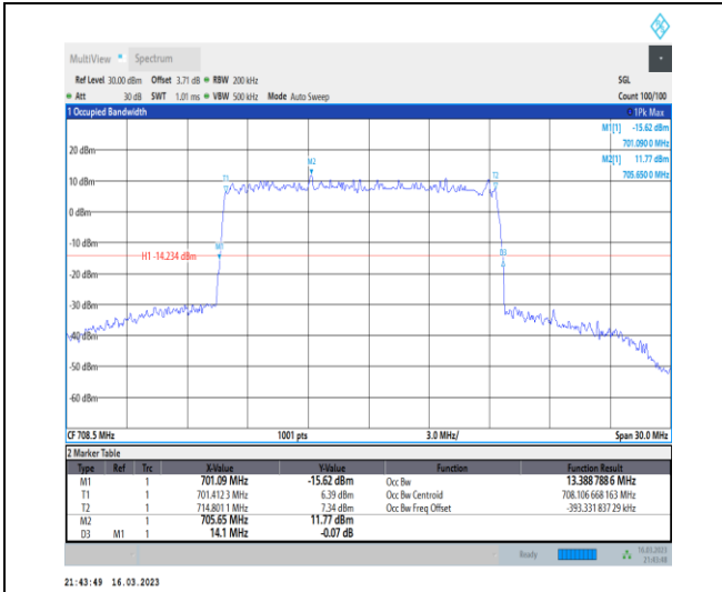
1-N12-PC3-15-15-H-5-DFT-256QAM-Outer_Full-75 @0-Ant7-13.389-14.100-≤15-PASS
