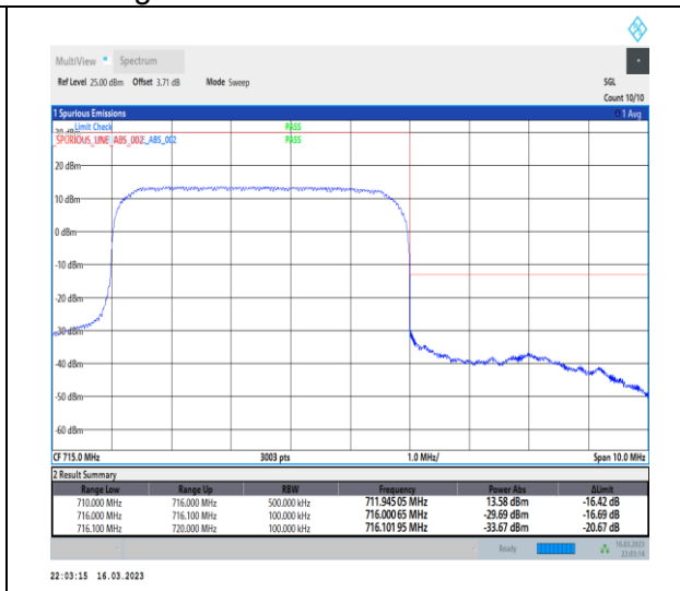
1-N12-PC3-15-5-H-3-DFT-PI2BPSK-Outer_Full-25@0-Ant7-1--PASS-see graph
