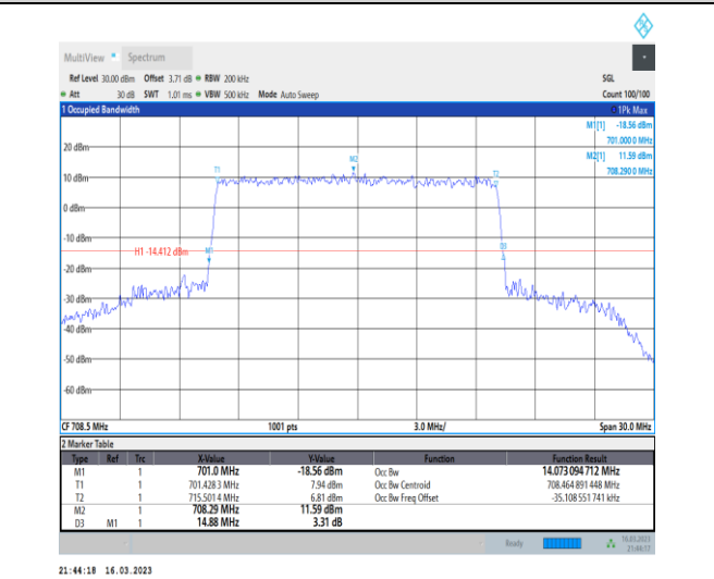
1-N12-PC3-15-15-H-8-CP-64QAM-Outer_Full-79@0 -Ant7-14.073-14.880-≤15-PASS
