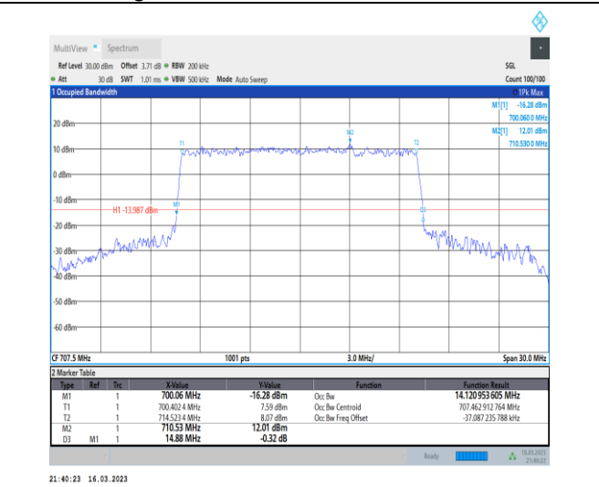
1-N12-PC3-15-15-M-7-CP-16QAM-Outer_Full-79@0-Ant7-14.121-14.880-≤15-PASS
