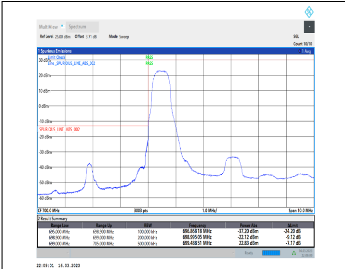
1-N12-PC3-15-15-L-1-DFT-PI2BPSK-Edge_1RB_Left-1@0-Ant7-1--PASS-see graph
