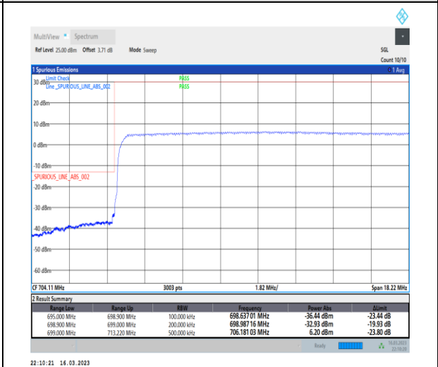
1-N12-PC3-15-15-L-6-CP-QPSK-Outer_Full-79@0-Ant7-1--PASS-see graph
