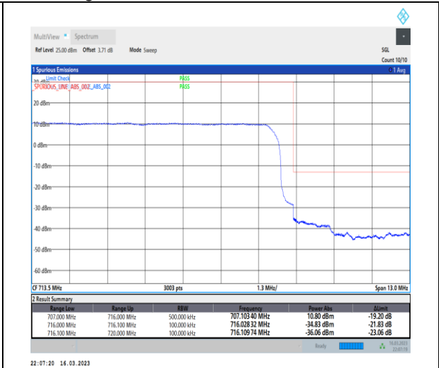
1-N12-PC3-15-10-H-3-DFT-PI2BPSK-Outer_Full-5 0@0-Ant7-1--PASS-see graph
