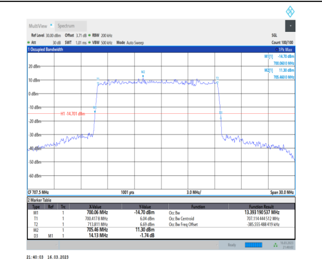
1-N12-PC3-15-15-M-5-DFT-256QAM-Outer_Full-75 @0-Ant7-13.393-14.130-≤15-PASS
