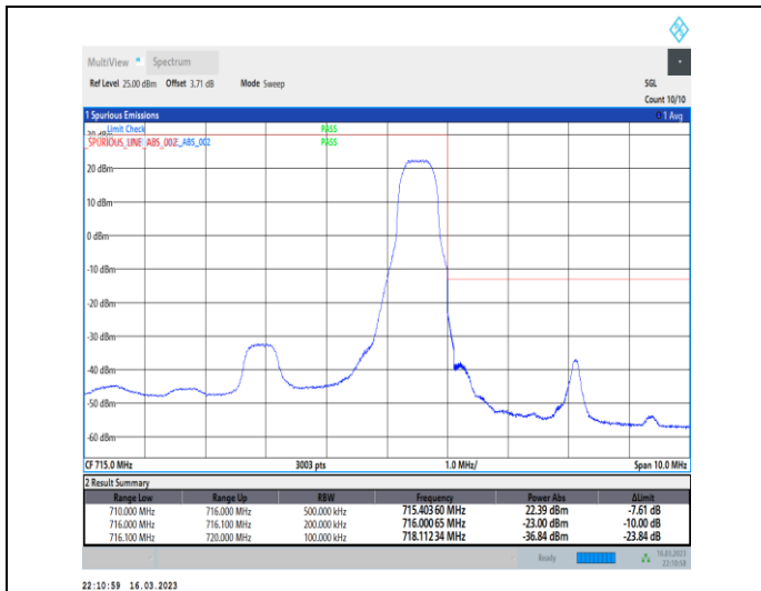
1-N12-PC3-15-15-H-2-DFT-PI2BPSK-Edge_1RB_Righ t-1@78-Ant7-1--PASS-see graph
