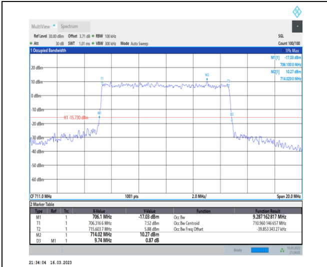
1-N12-PC3-15-10-H-8-CP-64QAM-Outer_Full-52@0 -Ant7-9.287-9.740-≤10-PASS
