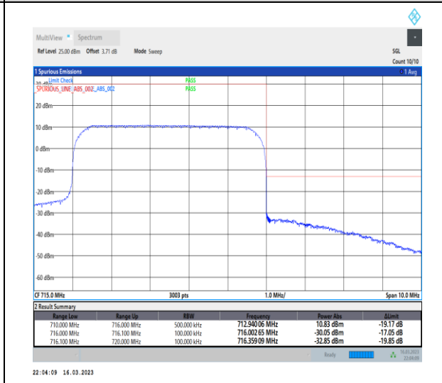
1-N12-PC3-15-5-H-6-CP-QPSK-Outer_Full-25@0-Ant7-1--PASS-see graph
