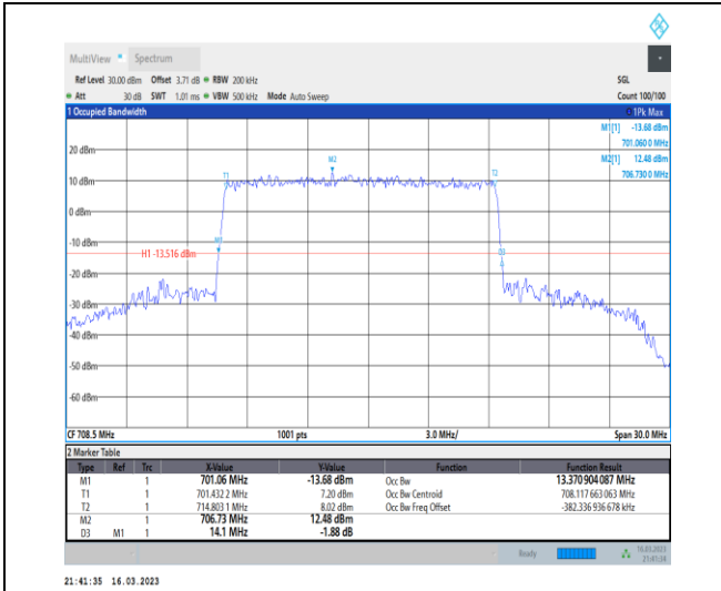
1-N12-PC3-15-15-H-1-DFT-QPSK-Outer_Full-75@0-Ant7-13.371-14.100-≤15-PASS
