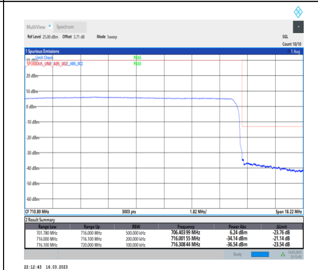
1-N12-PC3-15-15-H-6-CP-QPSK-Outer_Full-79@ 0-Ant7-1--PASS-see graph
