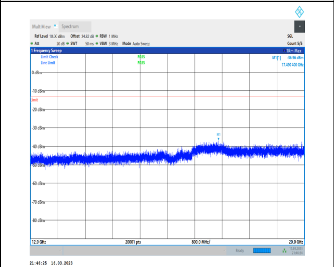
1-N12-PC3-15-15-M-1-DFT-PI2BPSK-Inner_1RB_L eft-1@1-12000-20000-Ant7-17490.40--36.96--13-PASS
