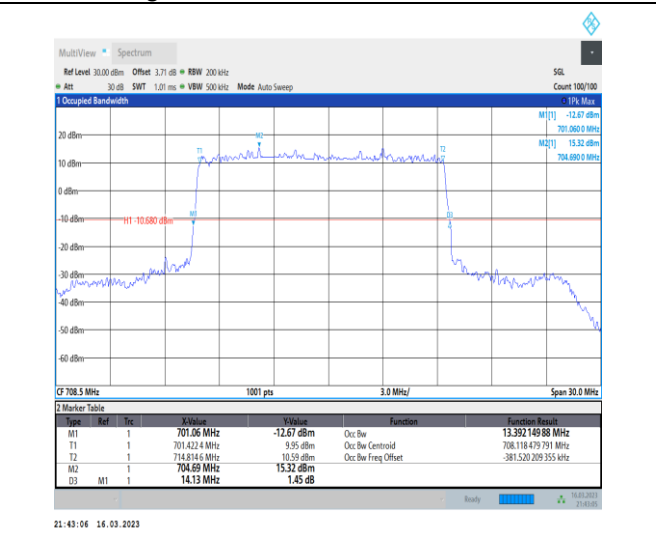
1-N12-PC3-15-15-H-2-DFT-PI2BPSK-Outer_Full-75@0-Ant7-13.392-14.130-≤15-PASS
