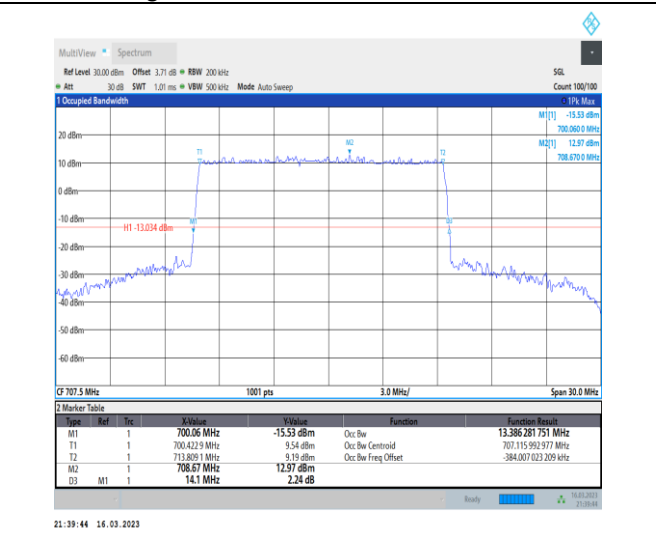
1-N12-PC3-15-15-M-3-DFT-16QAM-Outer_Full-75 @0-Ant7-13.386-14.100-≤15-PASS
