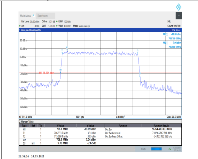
1-N12-PC3-15-10-H-9-CP-256QAM-Outer_Full-52@0 -Ant7-9.264-9.760-≤10-PASS
