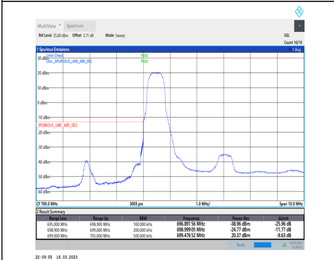
1-N12-PC3-15-15-L-4-CP-QPSK-Edge_1RB_Left-1@0-Ant7-1--PASS-see graph
