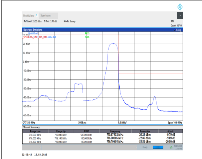
1-N12-PC3-15-5-H-5-CP-QPSK-Edge_1RB_Right-1@24-Ant7-1--PASS-see graph
