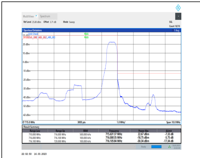
1-N12-PC3-15-5-H-2-DFT-PI2BPSK-Edge_1RB_Right-1@24-Ant7-1--PASS-see graph
