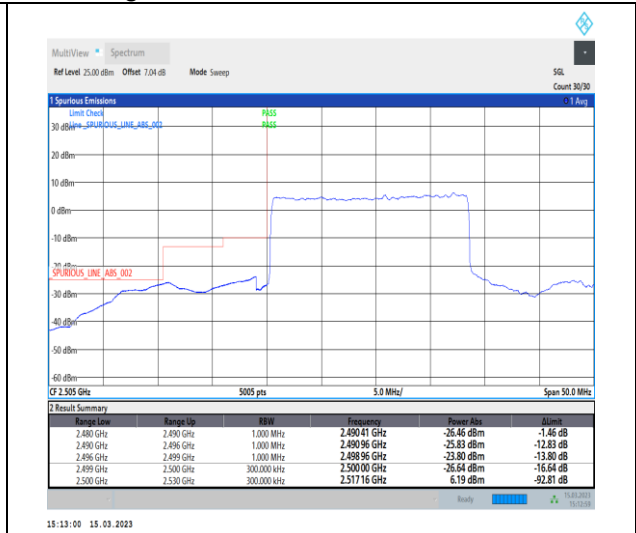
1-N7-PC3-15-20-L-3-DFT-PI2BPSK-Outer_Full-10 @0-Ant1-1--PASS-see graph
