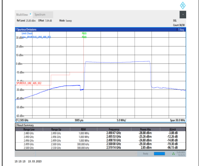
1-N7-PC3-15-20-L-6-CP-QPSK-Outer_Full-106@0-Ant1-1--PASS-see graph
