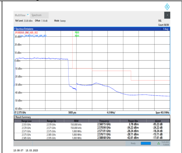
1-N7-PC3-15-15-H-3-DFT-PI2BPSK-Outer_Full-75@0-Ant1-1--PASS-see graph
