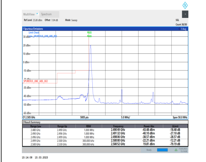
1-N7-PC3-15-20-L-4-CP-QPSK-Edge_1RB_Left-1@0-Ant1-1--PASS-see graph
