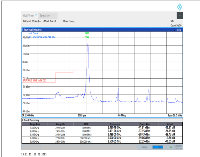
1-N7-PC3-15-20-L-1-DFT-PI2BPSK-Edge_1RB_Left-1 @0-Ant1-1--PASS-see graph
