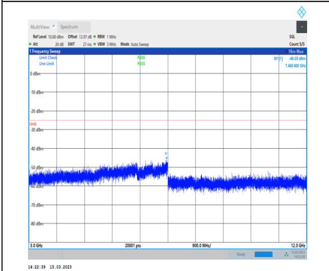
1-N7-PC3-15-20-M-1-DFT-PI2BPSK-Inner_1RB_Lef t-1@1-3000-12000-Ant1-7460.40--46.03--25-PASS
