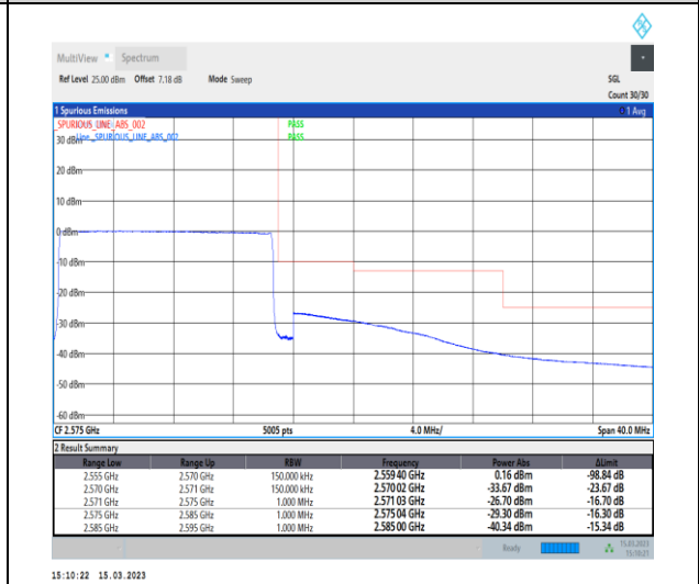
1-N7-PC3-15-15-H-6-CP-QPSK-Outer_Full-79@0-Ant1-1--PASS-see graph
