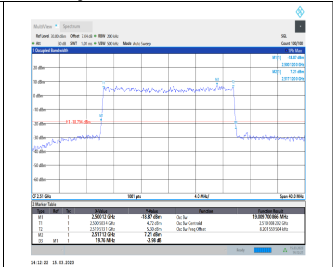
1-N7-PC3-15-20-L-9-CP-256QAM-Outer_Full-106@0-Ant1-19.01-19.760-≤20-PASS
