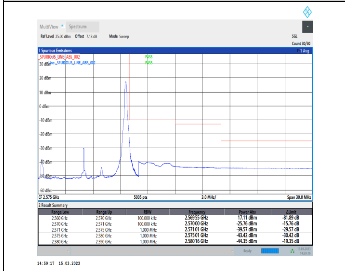
1-N7-PC3-15-10-H-5-CP-QPSK-Edge_1RB_Right-1@51-Ant1-1--PASS-see graph
