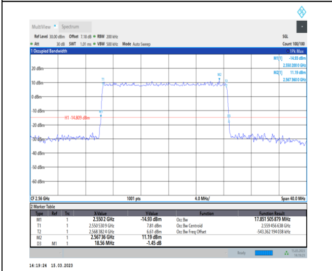
1-N7-PC3-15-20-H-4-DFT-64QAM-Outer_Full-100 @0-Ant1-17.852-18.560-≤20-PASS
