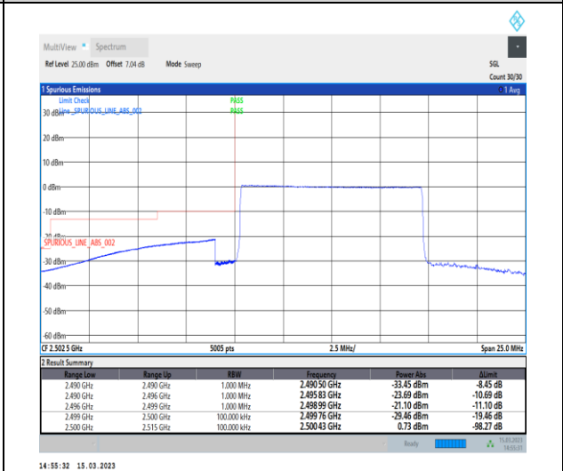
1-N7-PC3-15-10-L-6-CP-QPSK-Outer_Full-52@0-Ant1-1--PASS-see graph
