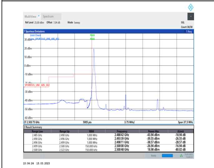
1-N7-PC3-15-15-L-4-CP-QPSK-Edge_1RB_Left-1@0-Ant1-1--PASS-see graph
