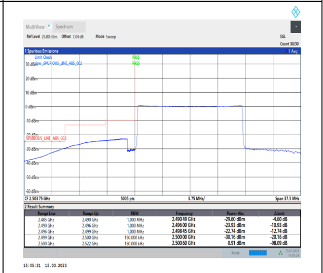
1-N7-PC3-15-15-L-6-CP-QPSK-Outer_Full-79@0-Ant1-1--PASS-see graph
