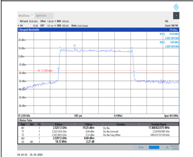
1-N7-PC3-15-20-M-5-DFT-256QAM-Outer_Full-100 @0-Ant1-17.869-18.720-≤20-PASS
