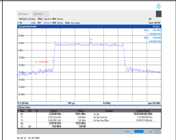
1-N7-PC3-15-20-M-6-CP-QPSK-Outer_Full-106@0- Ant1-18.875-19.800-≤20-PASS
