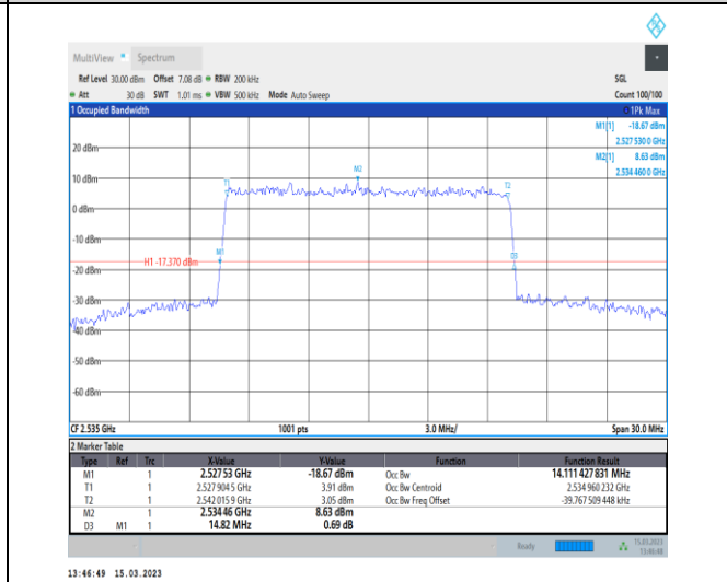
1-N7-PC3-15-15-M-9-CP-256QAM-Outer_Full-79@0- -Ant1-14.111-14.820-≤15-PASS
