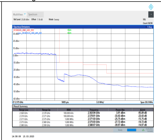
1-N7-PC3-15-10-H-3-DFT-PI2BPSK-Outer_Full-50@0-Ant1-1--PASS-see graph
