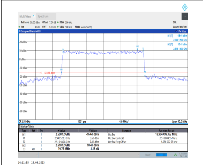
1-N7-PC3-15-20-L-6-CP-QPSK-Outer_Full-106@0- Ant1-18.964-19.760-≤20-PASS
