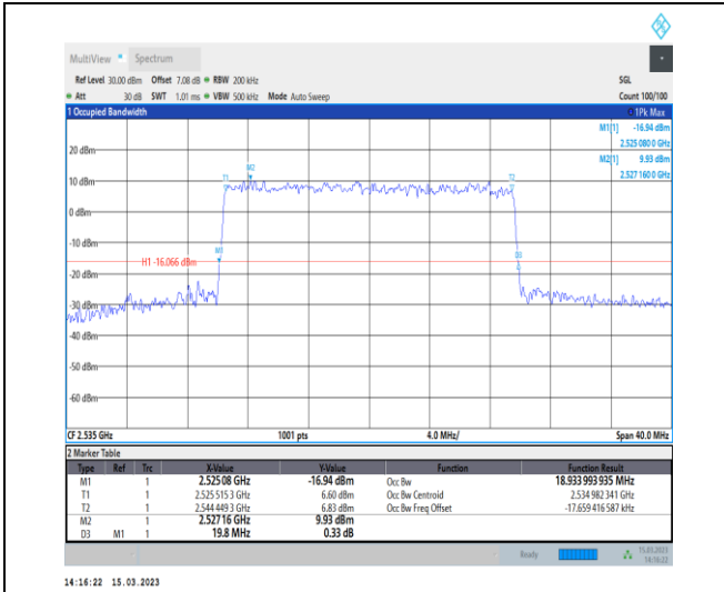
1-N7-PC3-15-20-M-7-CP-16QAM-Outer_Full-106@0 -Ant1-18.934-19.800-≤20-PASS
