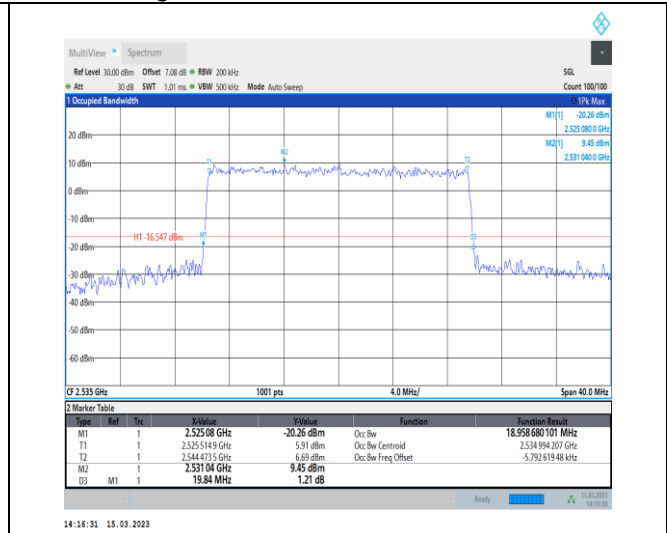
1-N7-PC3-15-20-M-8-CP-64QAM-Outer_Full-106@0 -Ant1-18.959-19.840-≤20-PASS
