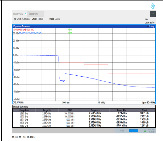
1-N7-PC3-15-10-H-6-CP-QPSK-Outer_Full-52@0-Ant1-1--PASS-see graph
