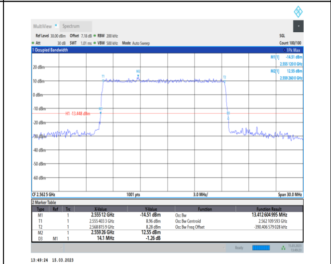
1-N7-PC3-15-15-H-4-DFT-64QAM-Outer_Full-75@0-Ant1-13.413-14.100-≤15-PASS
