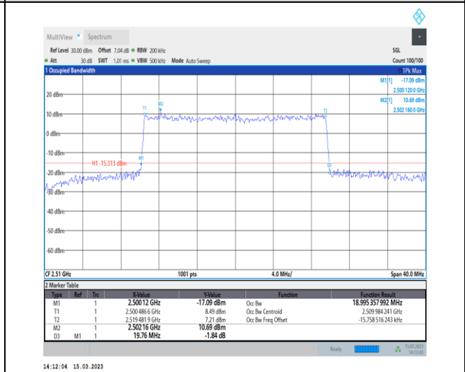
1-N7-PC3-15-20-L-7-CP-16QAM-Outer_Full-106@0- Ant1-18.995-19.760-≤20-PASS
