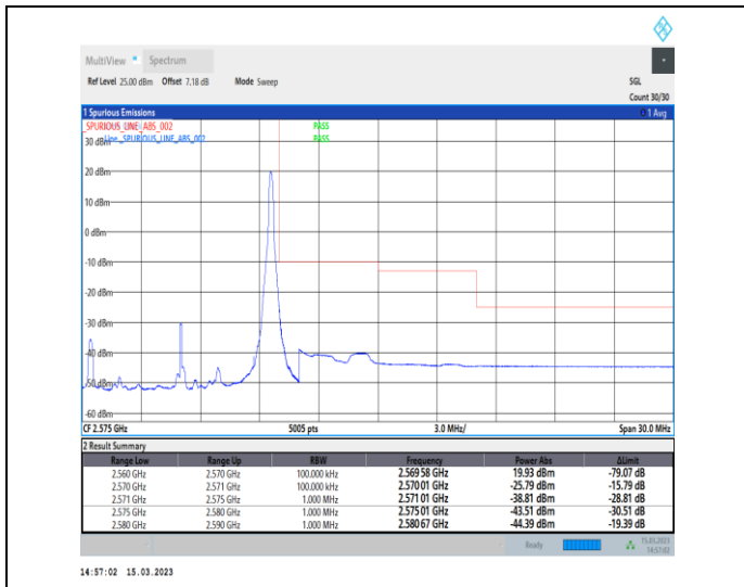
1-N7-PC3-15-10-H-2-DFT-PI2BPSK-Edge_1RB_Right-1@51-Ant1-1--PASS-see graph
