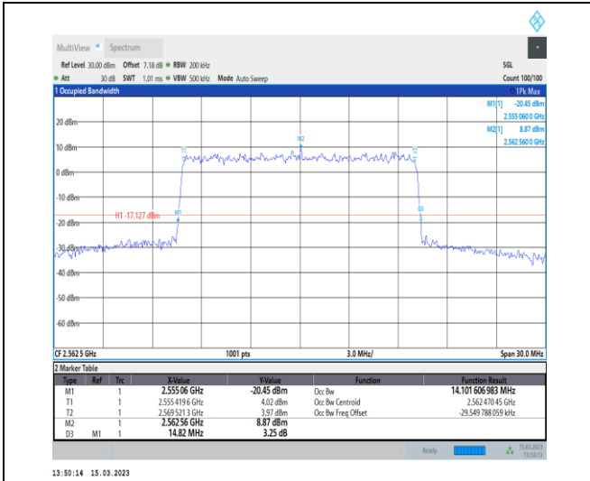
1-N7-PC3-15-15-H-9-CP-256QAM-Outer_Full-79@0 -Ant1-14.102-14.820-≤15-PASS
