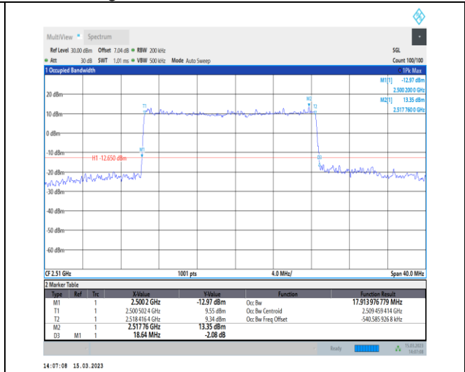
1-N7-PC3-15-20-L-1-DFT-QPSK-Outer_Full-100@0 -Ant1-17.914-18.640-≤20-PASS
