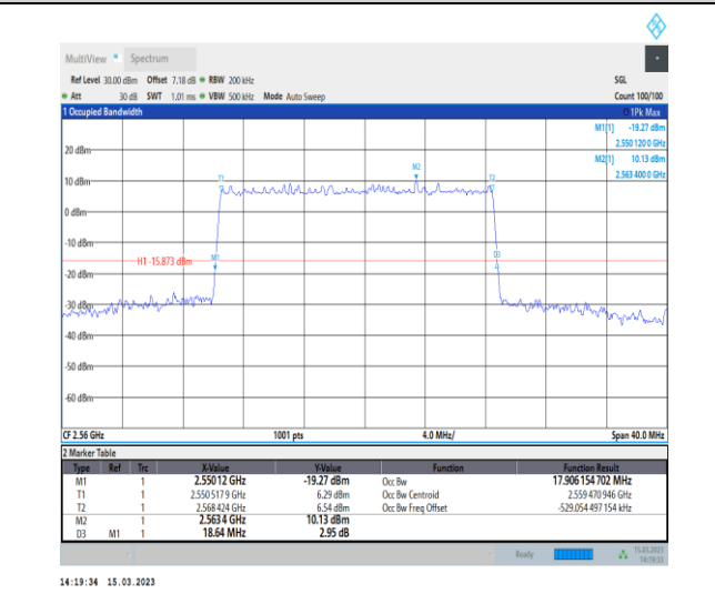
1-N7-PC3-15-20-H-5-DFT-256QAM-Outer_Full-100 @0-Ant1-17.906-18.640-≤20-PASS
