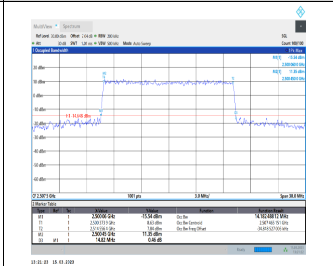
1-N7-PC3-15-15-L-6-CP-QPSK-Outer_Full-79@0-An t1-14.182-14.820-≤15-PASS
