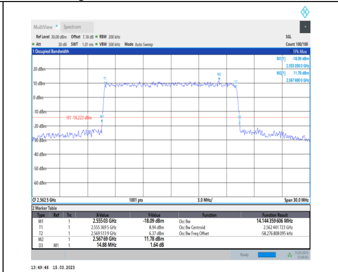
1-N7-PC3-15-15-H-6-CP-QPSK-Outer_Full-79@0-A nt1-14.144-14.880-≤15-PASS
