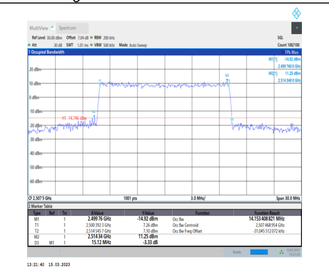
1-N7-PC3-15-15-L-8-CP-64QAM-Outer_Full-79@0-Ant1-14.153-15.120-≤15-PASS
