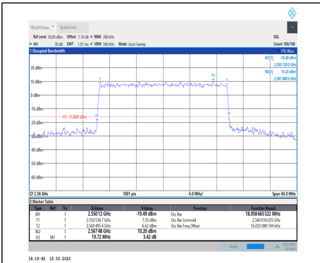
1-N7-PC3-15-20-H-6-CP-QPSK-Outer_Full-106@0-Ant1-18.959-19.720-≤20-PASS
