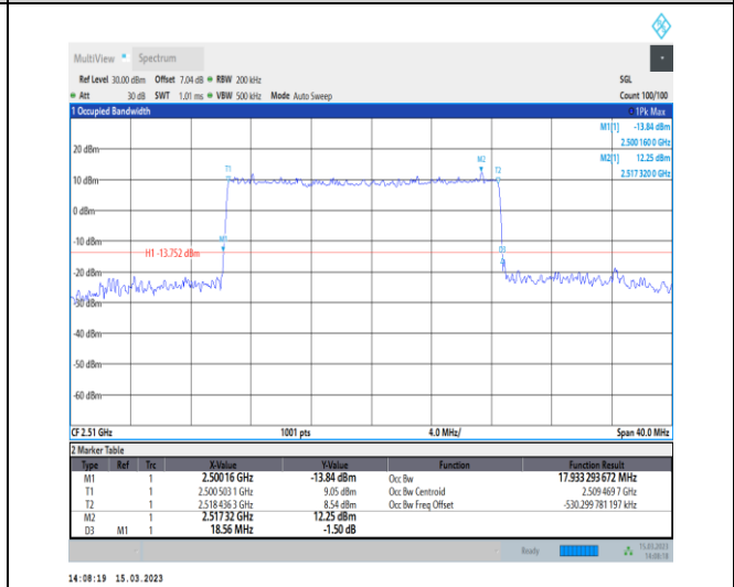
1-N7-PC3-15-20-L-3-DFT-16QAM-Outer_Full-100@0-Ant1-17.933-18.560-≤20-PASS
