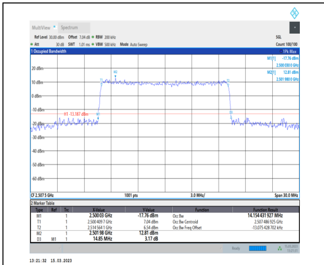
1-N7-PC3-15-15-L-7-CP-16QAM-Outer_Full-79@0-Ant1-14.154-14.850-≤15-PASS
