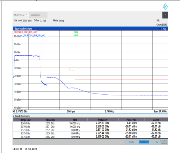
1-N7-PC3-15-5-H-3-DFT-PI2BPSK-Outer_Full-25@0-Ant1-1--PASS-see graph
