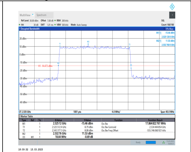
1-N7-PC3-15-20-M-4-DFT-64QAM-Outer_Full-100@ 0-Ant1-17.865-18.640-≤20-PASS
