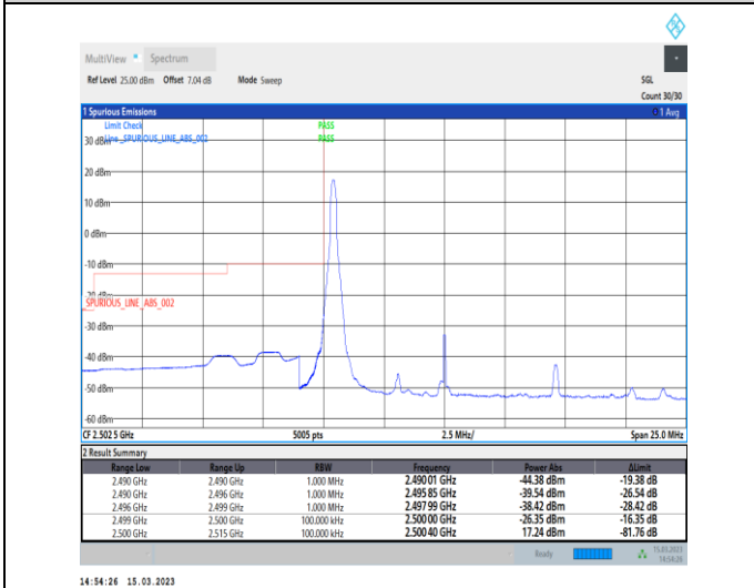
1-N7-PC3-15-10-L-4-CP-QPSK-Edge_1RB_Left-1@0-Ant1-1--PASS-see graph
