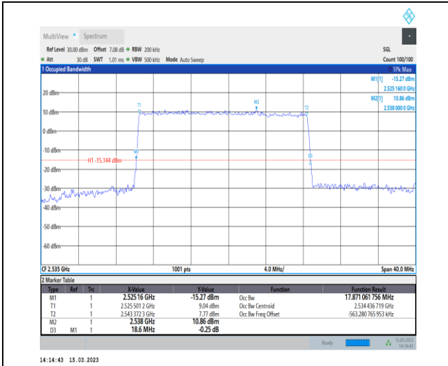
1-N7-PC3-15-20-M-3-DFT-16QAM-Outer_Full-100@ 0-Ant1-17.871-18.600-≤20-PASS
