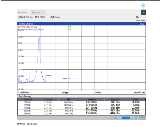
1-N7-PC3-15-5-H-2-DFT-PI2BPSK-Edge_1RB_Right-1@24-Ant1-1--PASS-see graph
