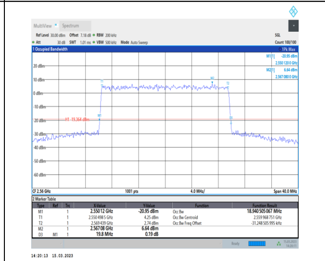
1-N7-PC3-15-20-H-9-CP-256QAM-Outer_Full-106@0-Ant1-18.941-19.800-≤20-PASS
