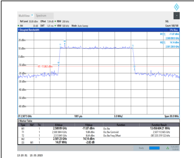
1-N7-PC3-15-15-L-3-DFT-16QAM-Outer_Full-75@0-Ant1-13.457-14.070-≤15-PASS
