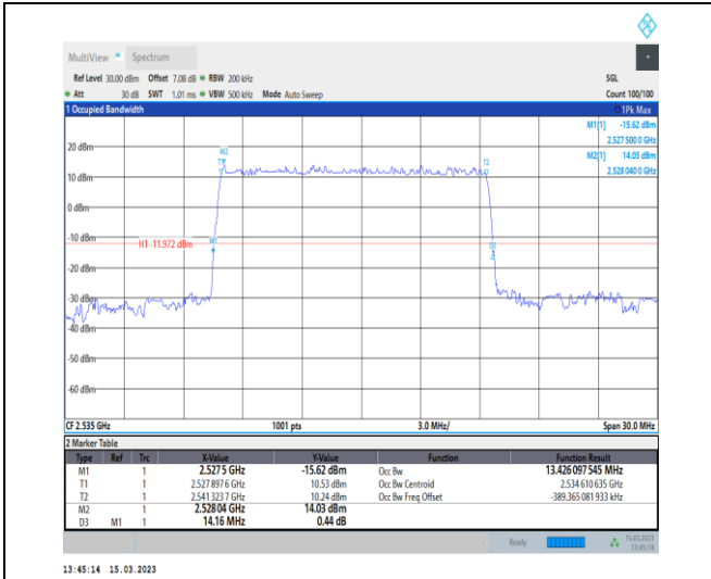
1-N7-PC3-15-15-M-2-DFT-PI2BPSK-Outer_Full-75 @0-Ant1-13.426-14.160-≤15-PASS
