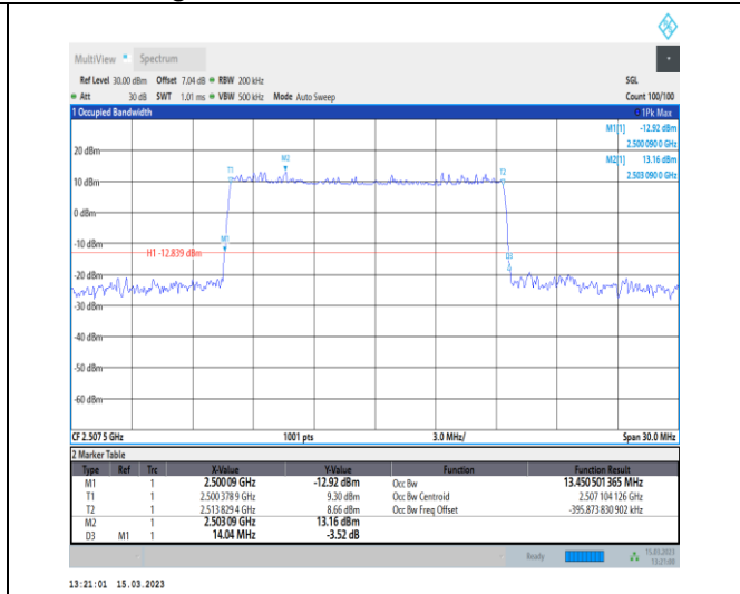
1-N7-PC3-15-15-L-4-DFT-64QAM-Outer_Full-75@0-Ant1-13.451-14.040-≤15-PASS
