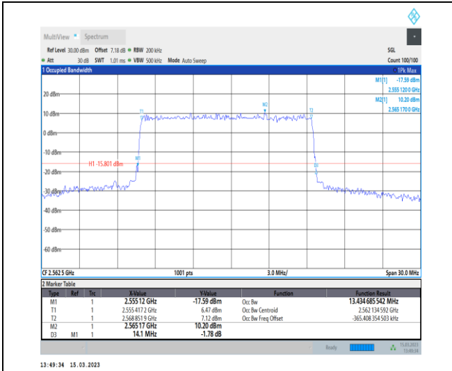
1-N7-PC3-15-15-H-5-DFT-256QAM-Outer_Full-75@ 0-Ant1-13.435-14.100-≤15-PASS
