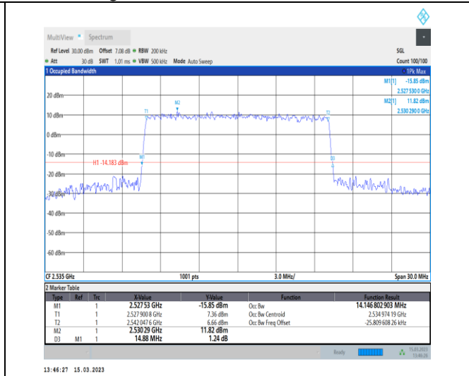
1-N7-PC3-15-15-M-7-CP-16QAM-Outer_Full-79@0- Ant1-14.147-14.880-≤15-PASS
