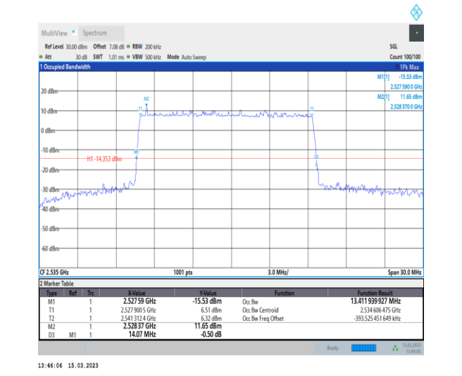
1-N7-PC3-15-15-M-5-DFT-256QAM-Outer_Full-75@0-Ant1-13.412-14.070-≤15-PASS
