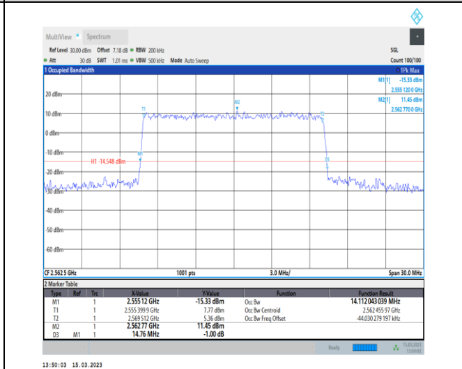
1-N7-PC3-15-15-H-8-CP-64QAM-Outer_Full-79@0- Ant1-14.112-14.760-≤15-PASS
