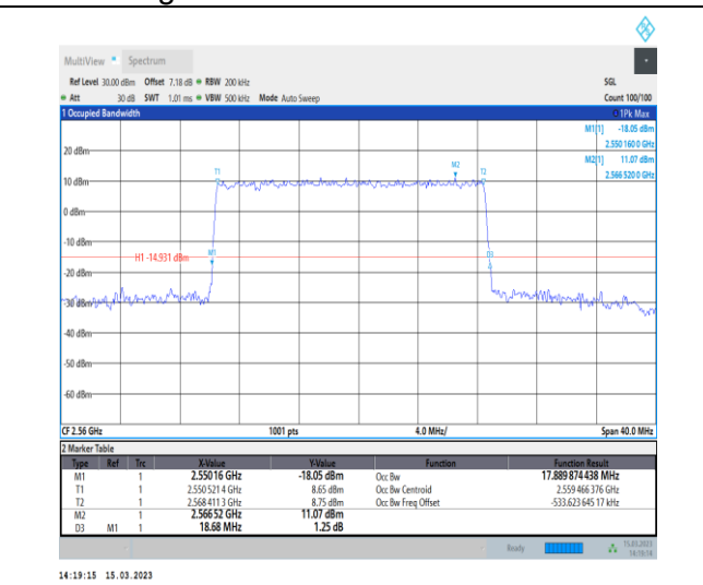
1-N7-PC3-15-20-H-3-DFT-16QAM-Outer_Full-100 @0-Ant1-17.89-18.680-≤20-PASS
