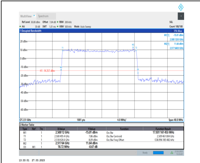
1-N7-PC3-15-20-L-4-DFT-64QAM-Outer_Full-100@ 0-Ant1-39.617-40.000-≤20-PASS
