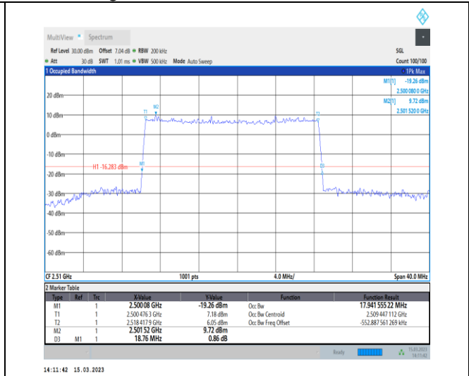
1-N7-PC3-15-20-L-5-DFT-256QAM-Outer_Full-100 @0-Ant1-17.942-18.760-≤20-PASS
