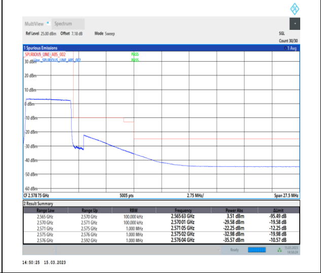
1-N7-PC3-15-5-H-6-CP-QPSK-Outer_Full-25@0-Ant1-1--PASS-see graph
