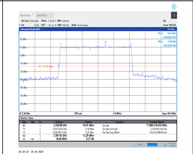
1-N7-PC3-15-20-H-1-DFT-QPSK-Outer_Full-100@0- Ant1-17.885-18.680-≤20-PASS
