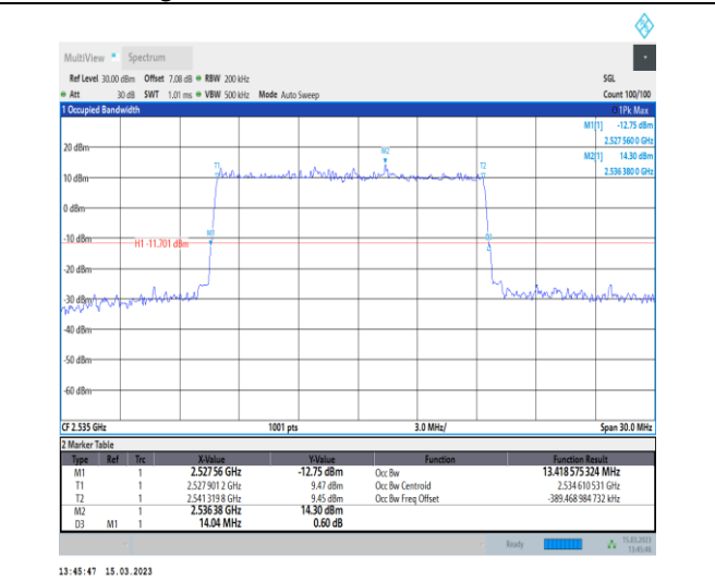
1-N7-PC3-15-15-M-3-DFT-16QAM-Outer_Full-75@0-Ant1-13.419-14.040-≤15-PASS
