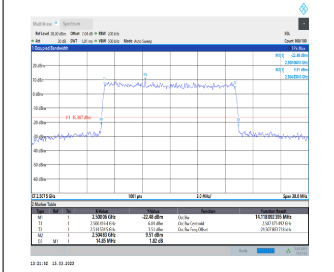
1-N7-PC3-15-15-L-9-CP-256QAM-Outer_Full-79@0-Ant1-14.118-14.850-≤15-PASS
