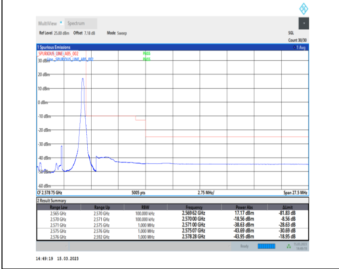
1-N7-PC3-15-5-H-5-CP-QPSK-Edge_1RB_Right-1@24-Ant1-1--PASS-see graph
