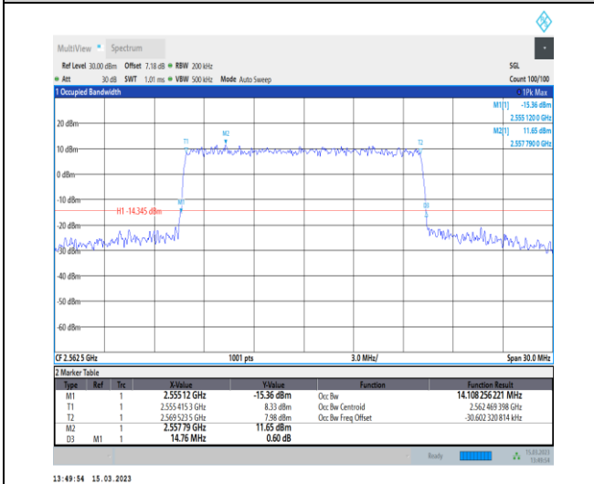
1-N7-PC3-15-15-H-7-CP-16QAM-Outer_Full-79@0- Ant1-14.108-14.760-≤15-PASS
