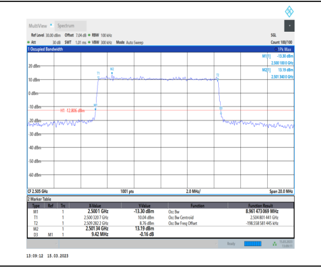
1-N7-PC3-15-10-L-1-DFT-QPSK-Outer_Full-50@0-A nt1-8.961-9.420-≤10-PASS
