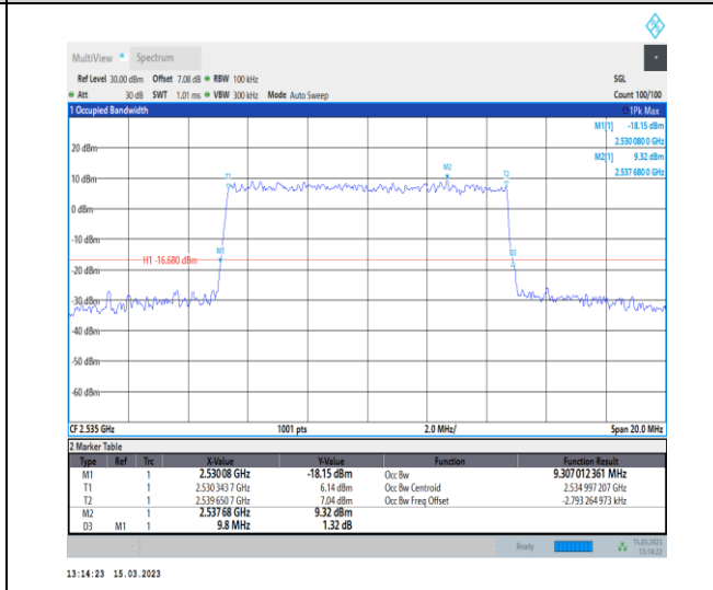
1-N7-PC3-15-10-M-8-CP-64QAM-Outer_Full-52@0-Ant1-9.307-9.800-≤10-PASS
