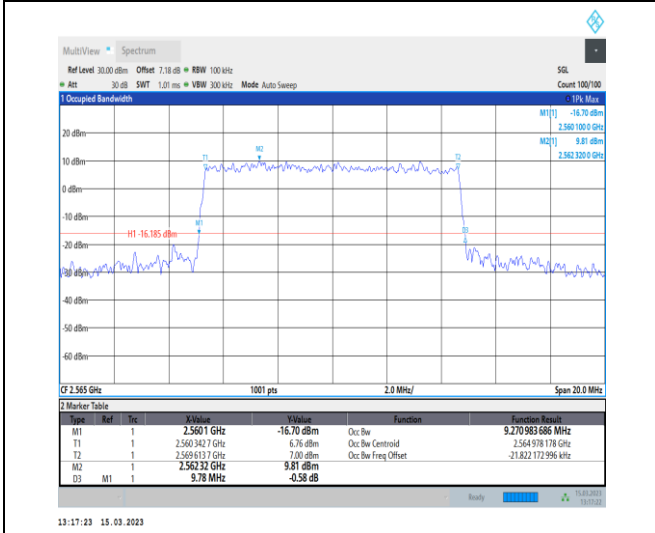
1-N7-PC3-15-10-H-6-CP-QPSK-Outer_Full-52@0-Ant1-9.271-9.780-≤10-PASS
