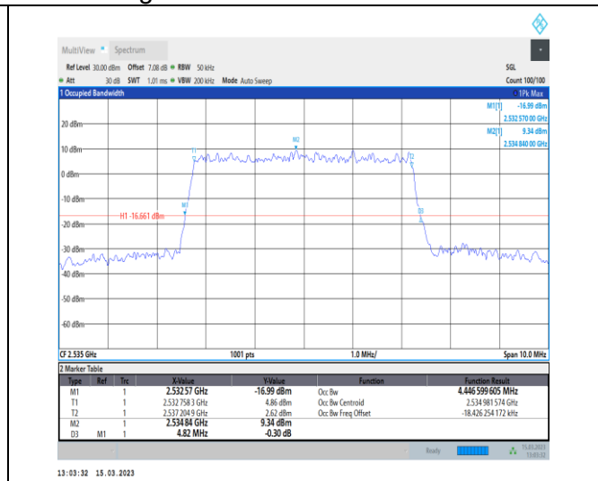
1-N7-PC3-15-5-M-5-DFT-256QAM-Outer_Full-25@0-Ant1-4.447-4.820-≤5-PASS
