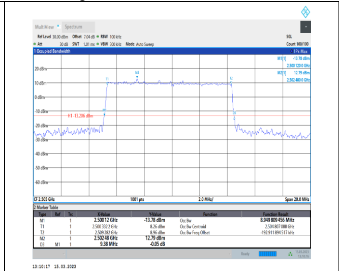
1-N7-PC3-15-10-L-3-DFT-16QAM-Outer_Full-50@0-Ant1-8.95-9.380-≤10-PASS
