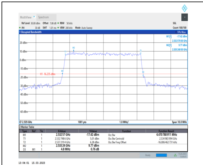
1-N7-PC3-15-5-M-8-CP-64QAM-Outer_Full-25@0-A nt1-4.471-4.800-≤5-PASS
