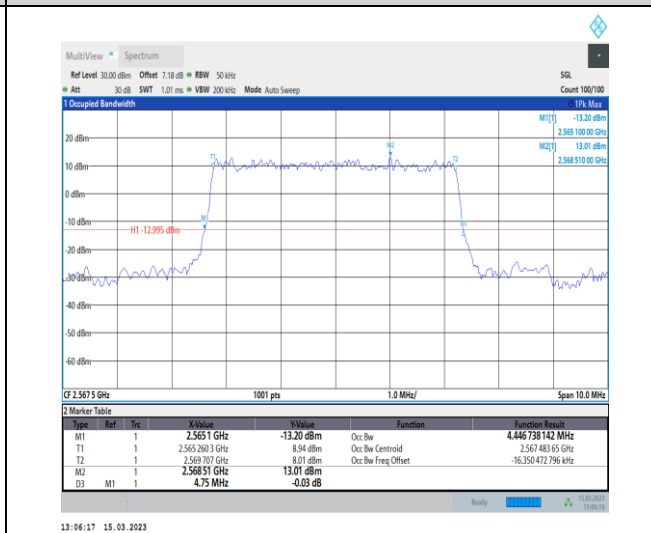
1-N7-PC3-15-5-H-2-DFT-PI2BPSK-Outer_Full-25@0- -Ant1-4.447-4.750-≤5-PASS
