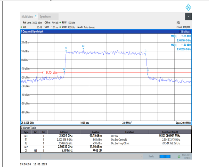
1-N7-PC3-15-10-L-7-CP-16QAM-Outer_Full-52@0-A nt1-9.307-9.780-≤10-PASS
