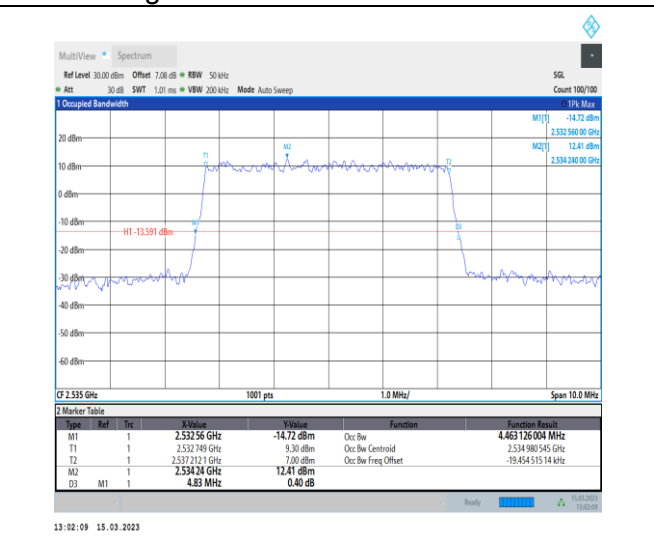
1-N7-PC3-15-5-M-1-DFT-QPSK-Outer_Full-25@0-Ant1-4.463-4.830-≤5-PASS
