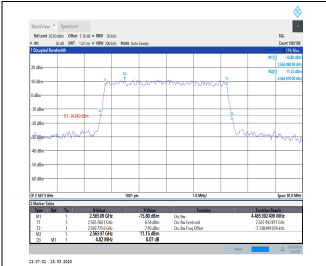
1-N7-PC3-15-5-H-3-DFT-16QAM-Outer_Full-25@0-Ant1-4.465-4.820-≤5-PASS
