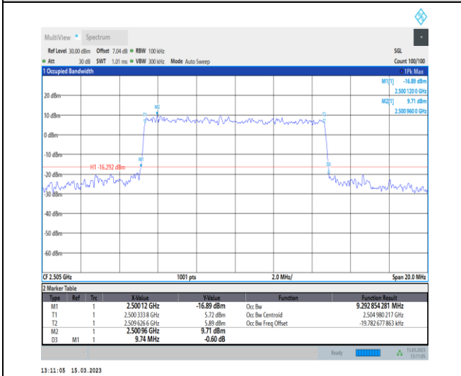
1-N7-PC3-15-10-L-8-CP-64QAM-Outer_Full-52@0-A Ant1-9.293-9.740-≤10-PASS
