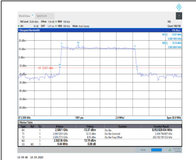
1-N7-PC3-15-10-L-2-DFT-PI2BPSK-Outer_Full-50@0-Ant1-8.953-9.440-≤10-PASS
