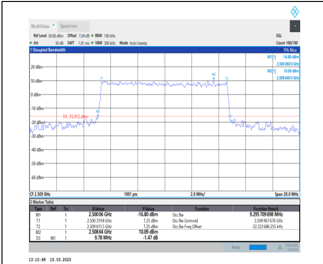
1-N7-PC3-15-10-L-6-CP-QPSK-Outer_Full-52@0-A nt1-9.296-9.780-≤10-PASS
