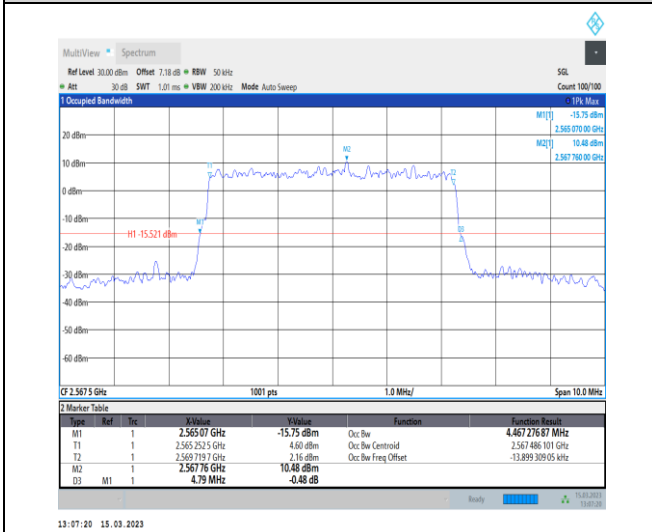
1-N7-PC3-15-5-H-5-DFT-256QAM-Outer_Full-25@0-Ant1-4.467-4.790-≤5-PASS
