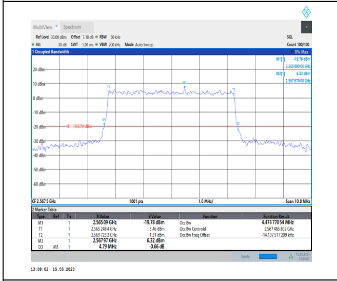
1-N7-PC3-15-5-H-9-CP-256QAM-Outer_Full-25@0-A Ant1-4.475-4.790-≤5-PASS
