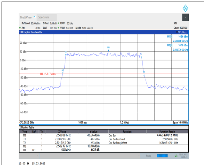
1-N7-PC3-15-5-L-5-DFT-256QAM-Outer_Full-25@0-Ant1-4.465-4.800-≤5-PASS
