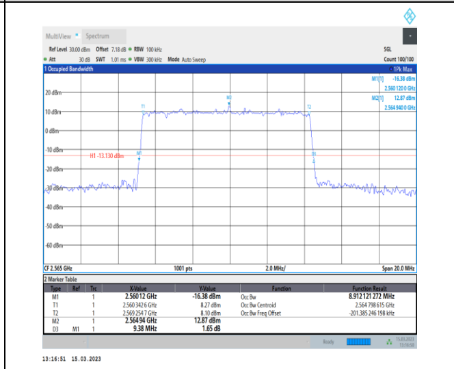
1-N7-PC3-15-10-H-3-DFT-16QAM-Outer_Full-50@0- Ant1-8.912-9.380-≤10-PASS
