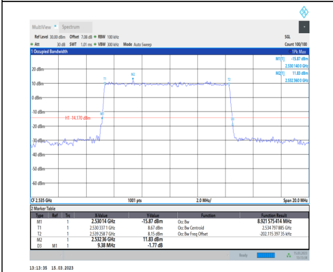
1-N7-PC3-15-10-M-3-DFT-16QAM-Outer_Full-50@0-Ant1-8.922-9.380-≤10-PASS
