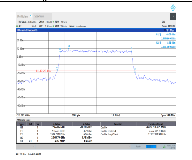
1-N7-PC3-15-5-H-8-CP-64QAM-Outer_Full-25@0-A nt1-4.479-4.870-≤5-PASS
