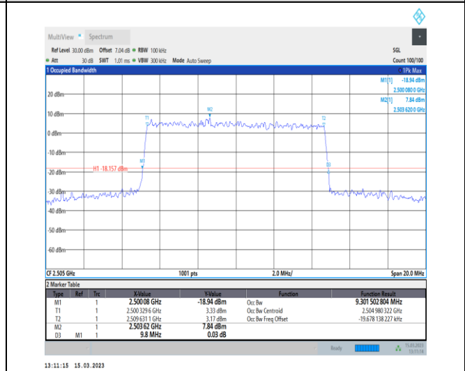
1-N7-PC3-15-10-L-9-CP-256QAM-Outer_Full-52@0-A Ant1-9.302-9.800-≤10-PASS
