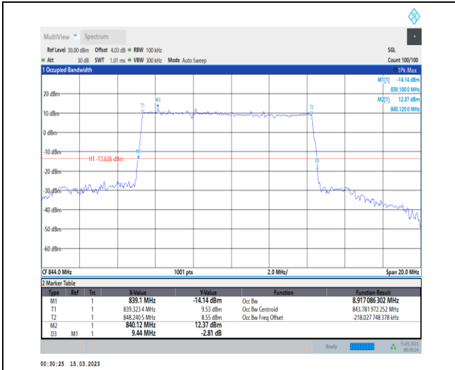
1-N5-PC3-15-10-H-4-DFT-64QAM-Outer_Full-50@0 -Ant1-8.917-9.440-≤10-PASS
