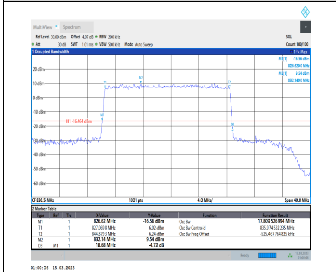
1-N5-PC3-15-20-M-5-DFT-256QAM-Outer_Full-100 @0-Ant1-17.81-18.680-≤20-PASS
