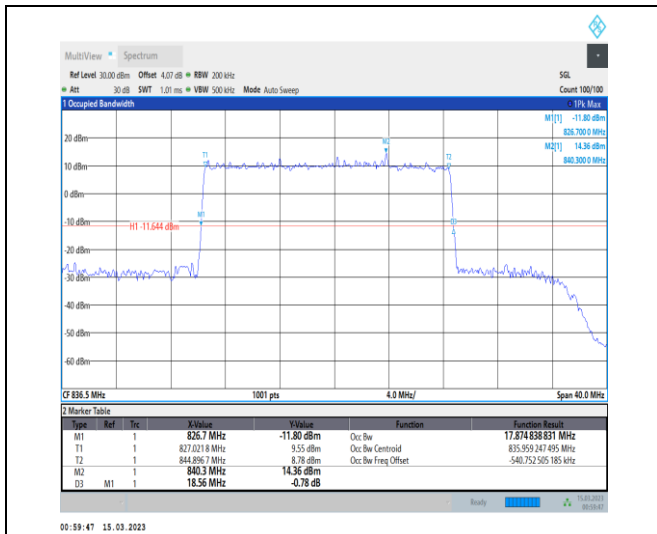
1-N5-PC3-15-20-M-3-DFT-16QAM-Outer_Full-100@ 0-Ant1-17.875-18.560-≤20-PASS
