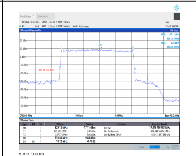
1-N5-PC3-15-20-H-5-DFT-256QAM-Outer_Full-100 @0-Ant1-17.849-18.720-≤20-PASS
