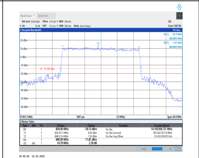
1-N5-PC3-15-15-H-8-CP-64QAM-Outer_Full-79@0- Ant1-14.102-14.790-≤15-PASS
