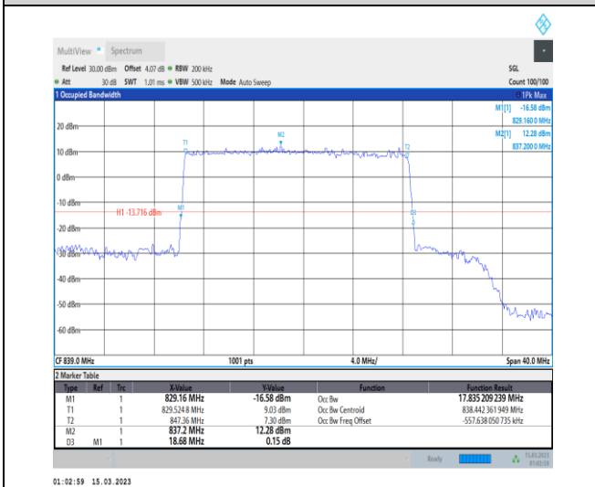
1-N5-PC3-15-20-H-4-DFT-64QAM-Outer_Full-100 @0-Ant1-17.835-18.680-≤20-PASS
