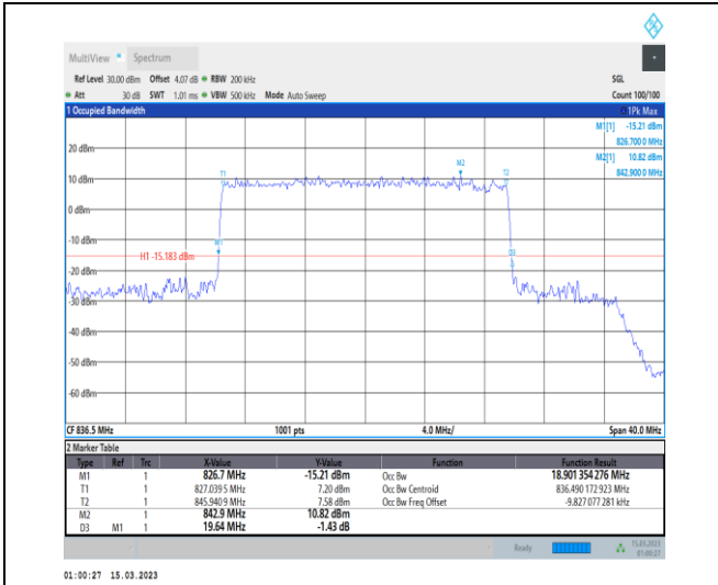
1-N5-PC3-15-20-M-7-CP-16QAM-Outer_Full-106@0 -Ant1-18.901-19.640-≤20-PASS
