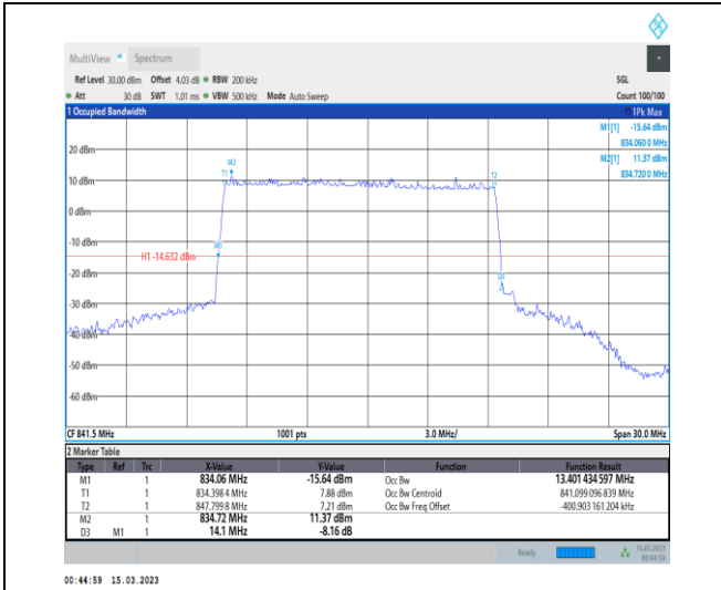
1-N5-PC3-15-15-H-5-DFT-256QAM-Outer_Full-75@ 0-Ant1-13.401-14.100-≤15-PASS
