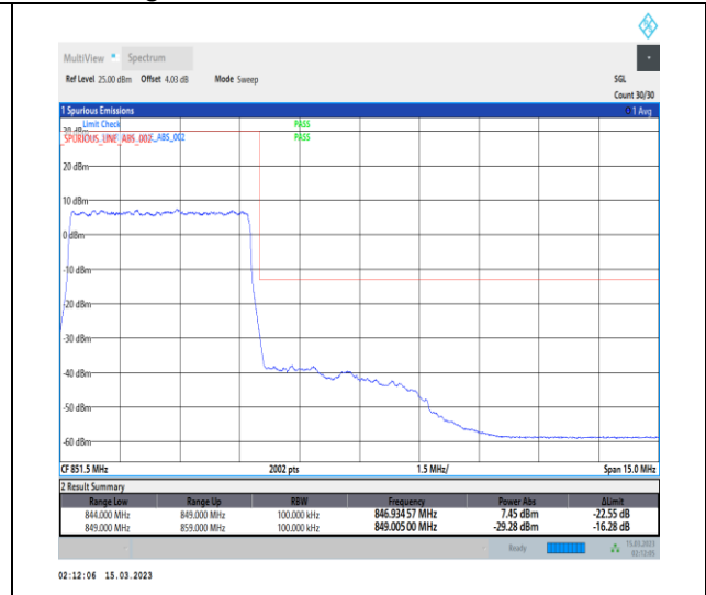
1-N5-PC3-15-5-H-3-DFT-PI2BPSK-Outer_Full-25 @0-Ant1-1-seegraph-PASS-see graph
