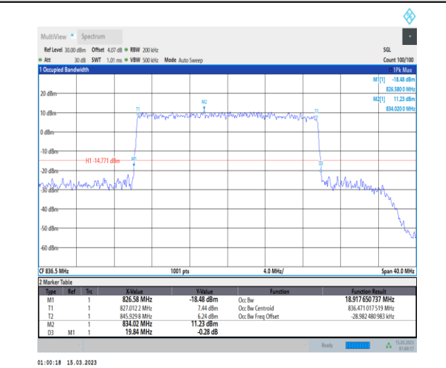
1-N5-PC3-15-20-M-6-CP-QPSK-Outer_Full-106@0- Ant1-18.918-19.840-≤20-PASS
