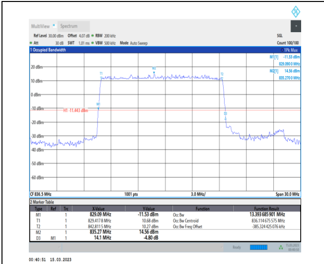
1-N5-PC3-15-15-M-2-DFT-PI2BPSK-Outer_Full-75 @0-Ant1-13.394-14.100-≤15-PASS
