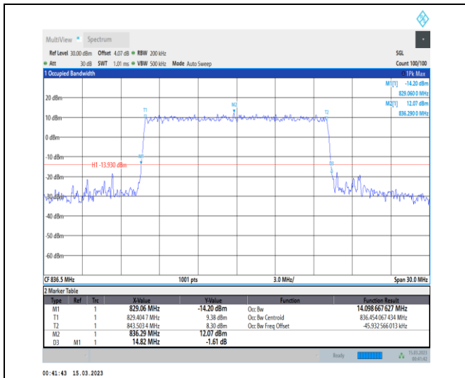
1-N5-PC3-15-15-M-6-CP-QPSK-Outer_Full-79@0-A Ant1-14.099-14.820-≤15-PASS
