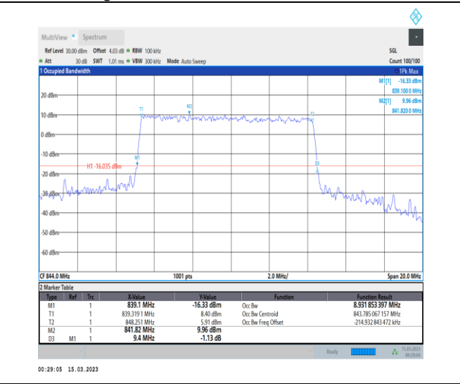
1-N5-PC3-15-10-H-1-DFT-QPSK-Outer_Full-50@0- Ant1-8.932-9.400-≤10-PASS
