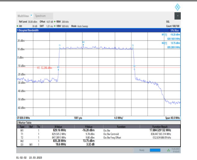
1-N5-PC3-15-20-H-1-DFT-QPSK-Outer_Full-100@0- Ant1-17.884-18.600-≤20-PASS
