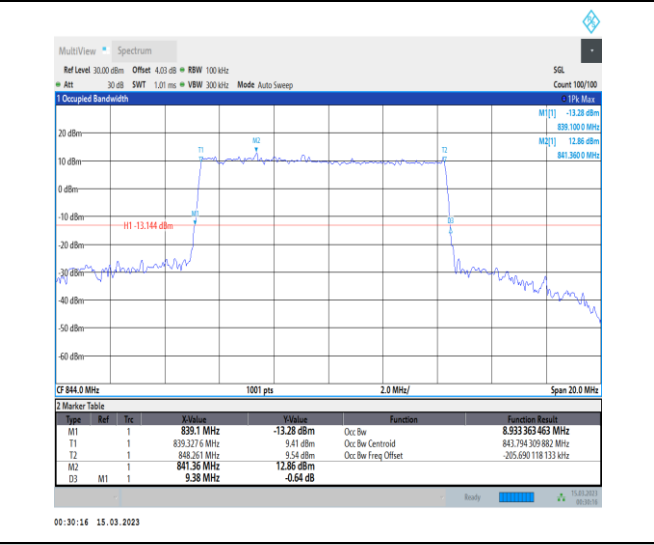
1-N5-PC3-15-10-H-3-DFT-16QAM-Outer_Full-50@0- Ant1-8.933-9.380-≤10-PASS
