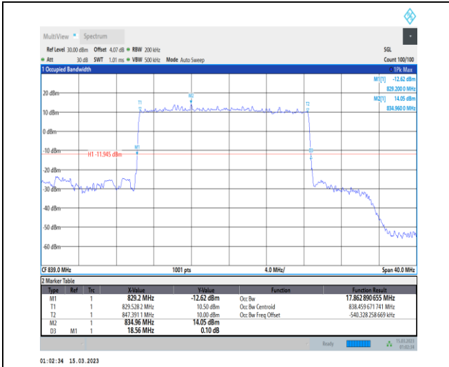
1-N5-PC3-15-20-H-2-DFT-PI2BPSK-Outer_Full-100 @0-Ant1-17.863-18.560-≤20-PASS
