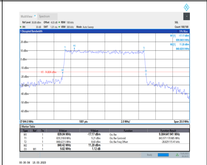
1-N5-PC3-15-10-H-7-CP-16QAM-Outer_Full-52@0- Ant1-9.305-9.820-≤10-PASS
