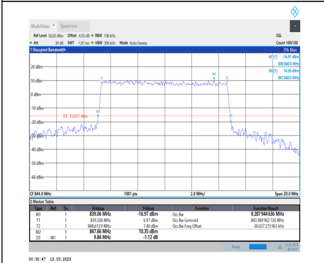
1-N5-PC3-15-10-H-6-CP-QPSK-Outer_Full-52@0-A nt1-9.288-9.840-≤10-PASS
