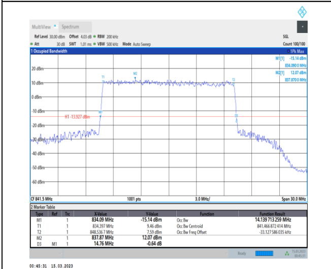
1-N5-PC3-15-15-H-7-CP-16QAM-Outer_Full-79@0- Ant1-14.14-14.760-≤15-PASS
