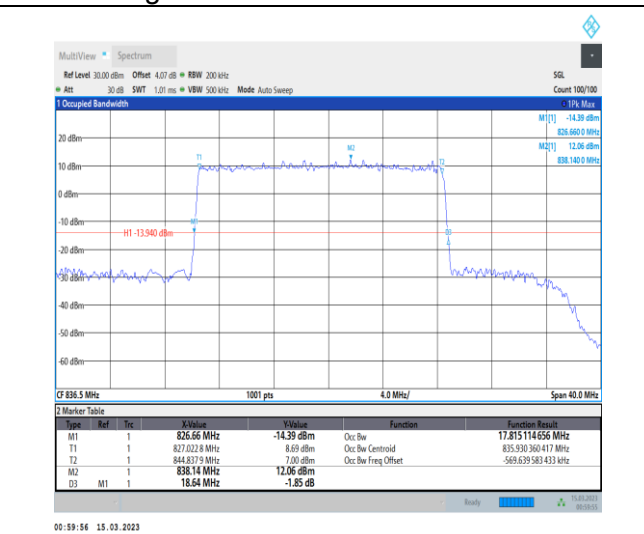
1-N5-PC3-15-20-M-4-DFT-64QAM-Outer_Full-100@ 0-Ant1-17.815-18.640-≤20-PASS
