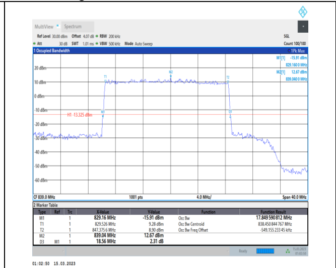
1-N5-PC3-15-20-H-3-DFT-16QAM-Outer_Full-100 @0-Ant1-17.85-18.560-≤20-PASS
