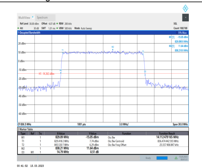
1-N5-PC3-15-15-M-7-CP-16QAM-Outer_Full-79@0- Ant1-14.112-14.790-≤15-PASS
