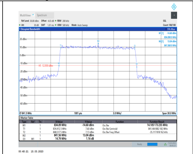
1-N5-PC3-15-15-H-6-CP-QPSK-Outer_Full-79@0-A nt1-14.105-14.790-≤15-PASS
