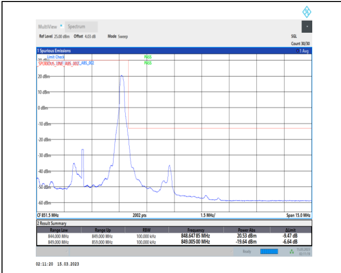
1-N5-PC3-15-5-H-2-DFT-PI2BPSK-Edge_1RB_Right-1 @24-Ant1-1-seegraph-PASS-see graph
