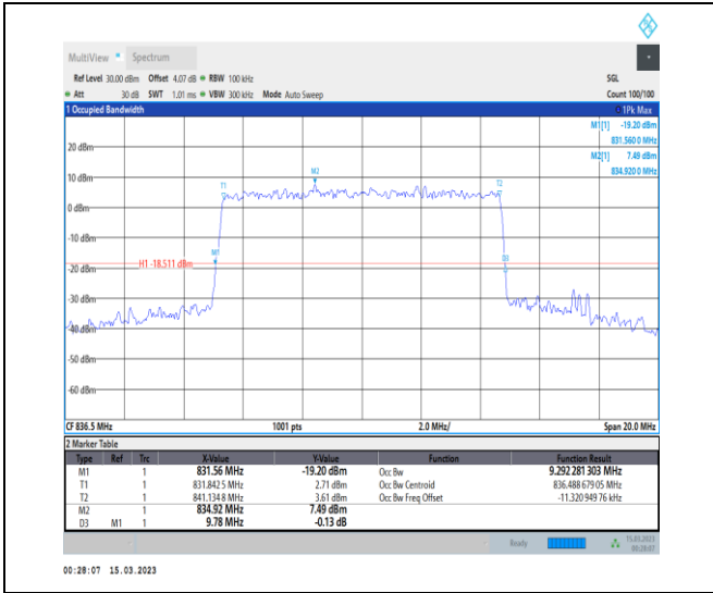
1-N5-PC3-15-10-M-9-CP-256QAM-Outer_Full-52@0 -Ant1-9.292-9.780-≤10-PASS
