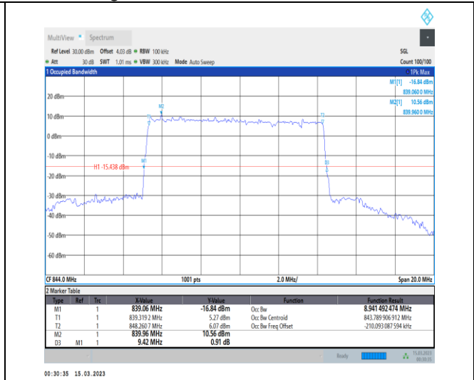
1-N5-PC3-15-10-H-5-DFT-256QAM-Outer_Full-50@0 -Ant1-8.941-9.420-≤10-PASS
