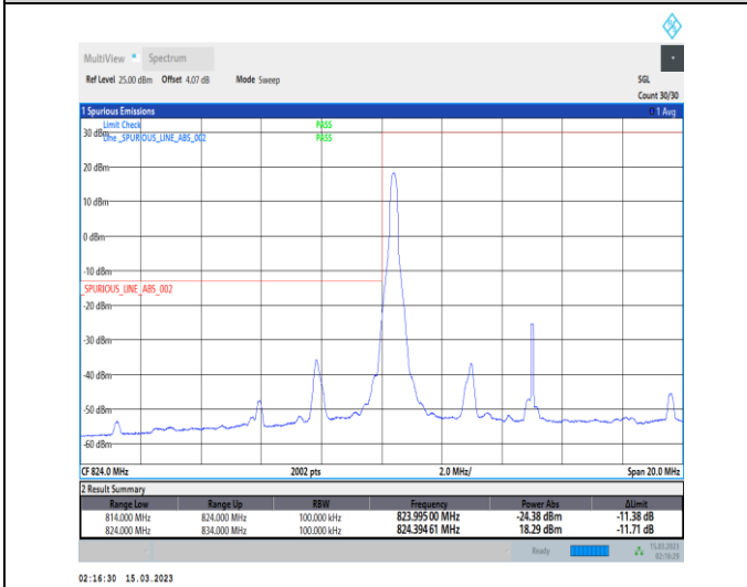
1-N5-PC3-15-10-L-4-CP-QPSK-Edge_1RB_Left-1@0-Ant1-1-seegraph-PASS-see graph
