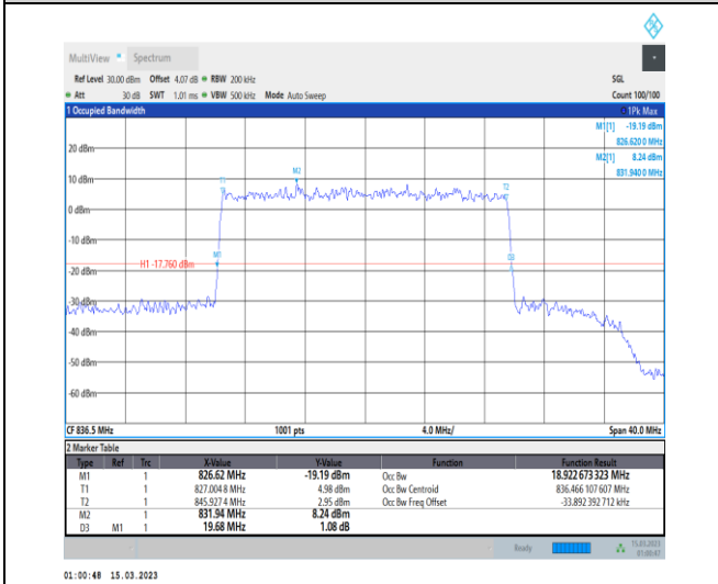
1-N5-PC3-15-20-M-9-CP-256QAM-Outer_Full-106@0 -Ant1-18.923-19.680-≤20-PASS
