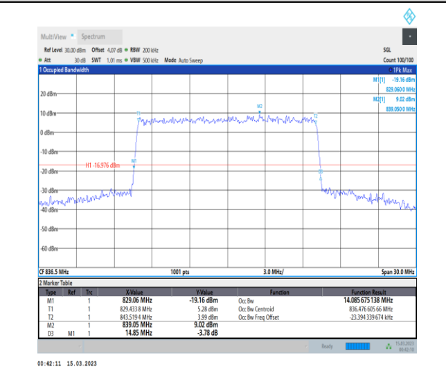
1-N5-PC3-15-15-M-9-CP-256QAM-Outer_Full-79@0- -Ant1-14.086-14.850-≤15-PASS
