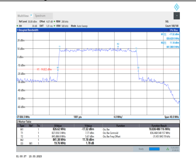
1-N5-PC3-15-20-M-8-CP-64QAM-Outer_Full-106@0 -Ant1-18.836-19.760-≤20-PASS
