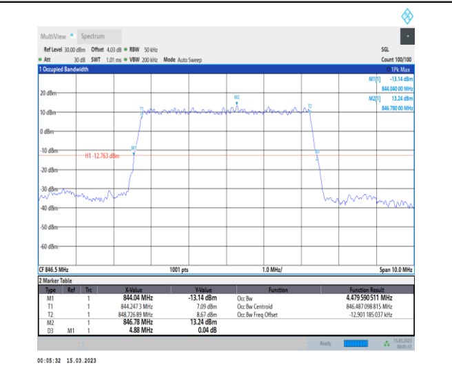
1-N5-PC3-15-5-H-2-DFT-PI2BPSK-Outer_Full-25@0- -Ant1-4.48-4.880-≤5-PASS
