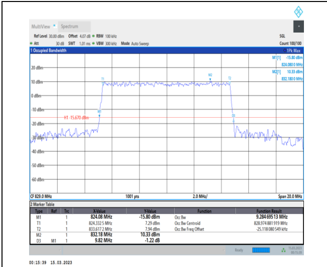
1-N5-PC3-15-10-L-6-CP-QPSK-Outer_Full-52@0-A nt1-9.285-9.820-≤10-PASS
