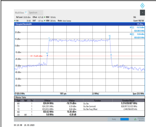
1-N5-PC3-15-10-L-8-CP-64QAM-Outer_Full-52@0-A Ant1-9.316-9.800-≤10-PASS
