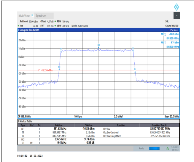
1-N5-PC3-15-10-M-5-DFT-256QAM-Outer_Full-50@0-Ant1-8.921-9.400-≤10-PASS
