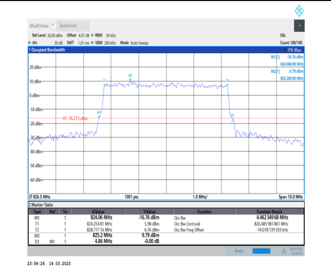
1-N5-PC3-15-5-L-8-CP-64QAM-Outer_Full-25@0-Ant1-4.462-4.840-≤5-PASS
