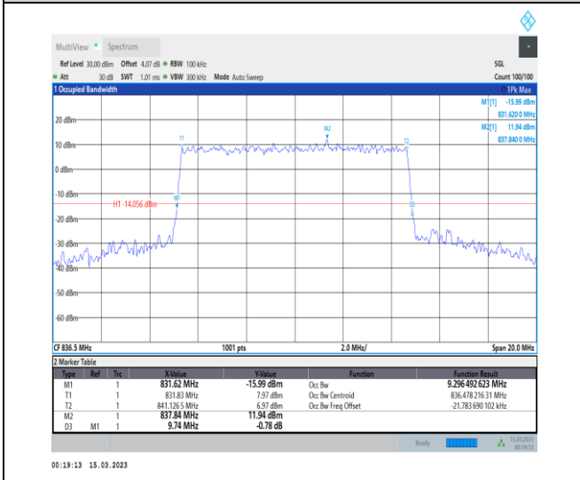
1-N5-PC3-15-10-M-7-CP-16QAM-Outer_Full-52@0-Ant1-9.296-9.740-≤10-PASS
