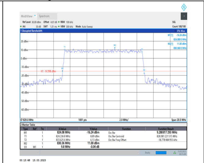
1-N5-PC3-15-10-L-7-CP-16QAM-Outer_Full-52@0-A nt1-9.289-9.800-≤10-PASS
