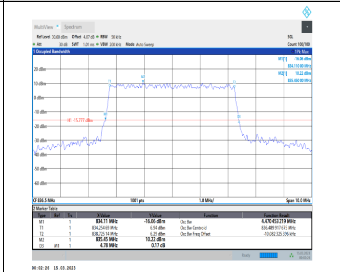
1-N5-PC3-15-5-M-7-CP-16QAM-Outer_Full-25@0-Ant1-4.47-4.780-≤5-PASS
