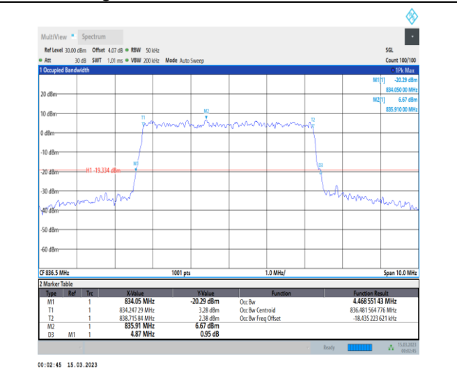
1-N5-PC3-15-5-M-9-CP-256QAM-Outer_Full-25@0- Ant1-4.469-4.870-≤5-PASS
