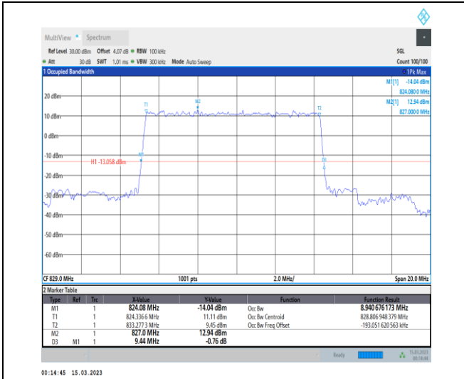
1-N5-PC3-15-10-L-2-DFT-PI2BPSK-Outer_Full-50@0-Ant1-8.941-9.440-≤10-PASS
