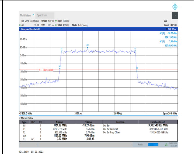
1-N5-PC3-15-10-L-9-CP-256QAM-Outer_Full-52@0-A Ant1-9.306-9.720-≤10-PASS
