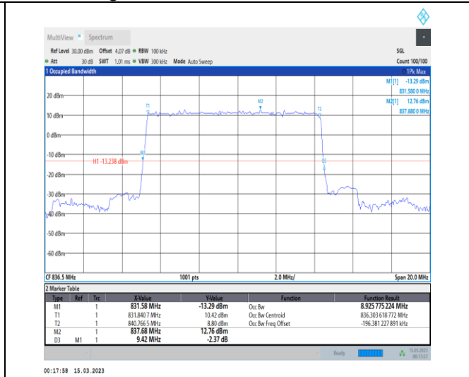
1-N5-PC3-15-10-M-2-DFT-PI2BPSK-Outer_Full-50@0-Ant1-8.926-9.420-≤10-PASS
