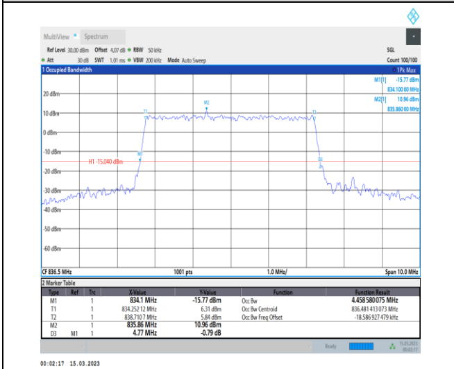
1-N5-PC3-15-5-M-6-CP-QPSK-Outer_Full-25@0-Ant1-4.459-4.770-≤5-PASS
