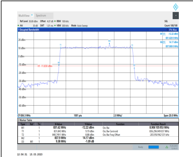
1-N5-PC3-15-10-M-1-DFT-QPSK-Outer_Full-50@0-Ant1-8.906-9.380-≤10-PASS
