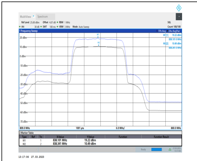
1-N5-PC3-15-20-H-1-DFT-256QAM-Outer_Full-100 @0-Ant1-8.73-100%-0.00-8.73-PASS-≤13
