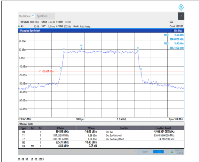
1-N5-PC3-15-5-M-8-CP-64QAM-Outer_Full-25@0-A nt1-4.466-4.830-≤5-PASS
