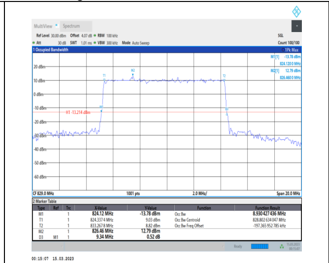
1-N5-PC3-15-10-L-3-DFT-16QAM-Outer_Full-50@0-Ant1-8.93-9.340-≤10-PASS
