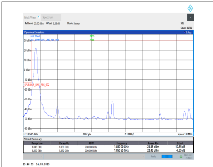
1-N2-PC3-15-20-L-1-DFT-PI2BPSK-Edge_1RB_Left-1 @0-Ant1-1-seegraph-PASS-see graph
