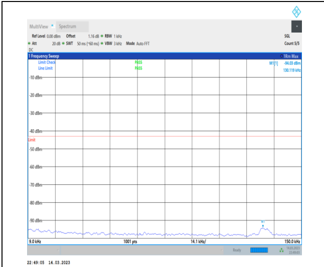
1-N2-PC3-15-20-H-1-DFT-PI2BPSK-Inner_1RB_Lef t-1@1-0.009-0.15-Ant1-0.13--94.03--43-PASS
