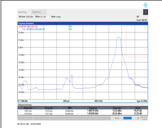
1-N2-15-5-H-5-CP-QPSK-Edge_1RB_Right-1@24-Ant1-1-seegraph-PASS-see graph
