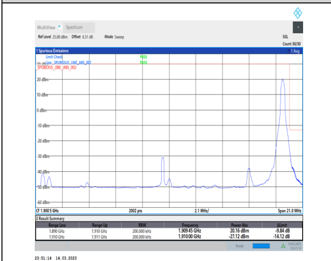
1-N2-PC3-15-20-H-5-CP-QPSK-Edge_1RB_Right-1@105-Ant1-1-seegraph-PASS-see graph
