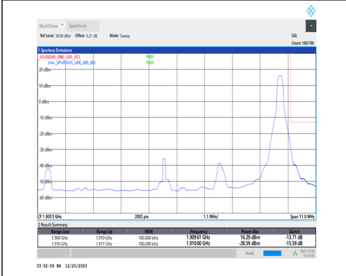
1-N2-15-10-H-5-CP-QPSK-Edge_1RB_Right-1@51-Ant1-1-seegraph-PASS-see graph
