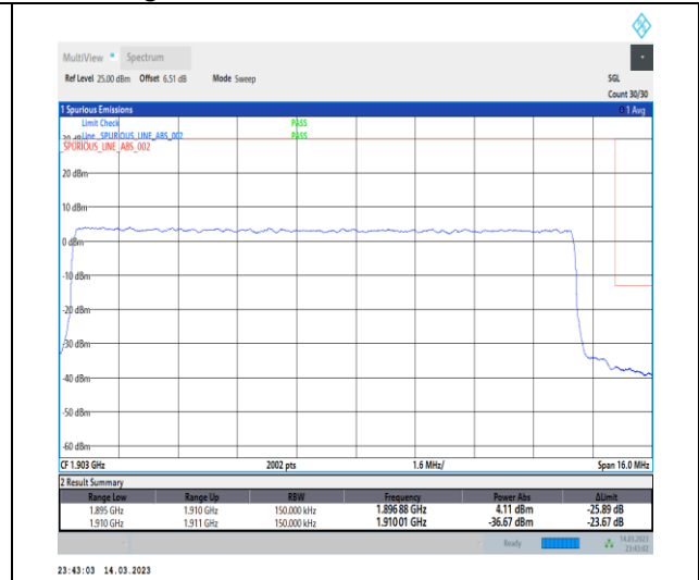
1-N2-PC3-15-15-H-3-DFT-PI2BPSK-Outer_Full-75@0-Ant1-1-seegraph-PASS-see graph
