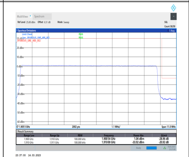
1-N2-PC3-15-10-H-6-CP-QPSK-Outer_Full-52@0-Ant1-1-seegraph-PASS-see graph
