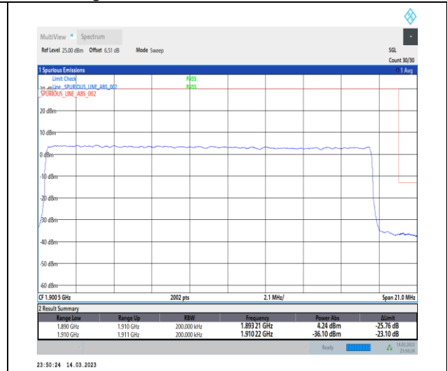
1-N2-PC3-15-20-H-3-DFT-PI2BPSK-Outer_Full-100@0-Ant1-1-seegraph-PASS-see graph
