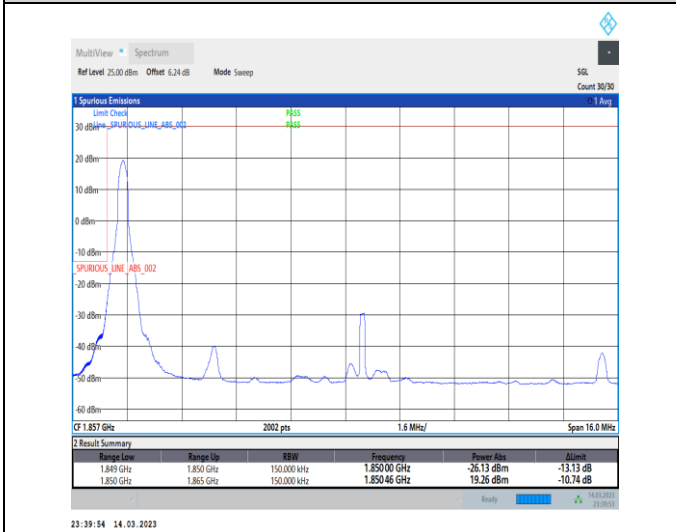
1-N2-PC3-15-15-L-4-CP-QPSK-Edge_1RB_Left-1@0-Ant1-1-seegraph-PASS-see graph
