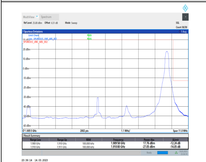
1-N2-PC3-15-10-H-5-CP-QPSK-Edge_1RB_Right-1@51-Ant1-1-seegraph-PASS-see graph
