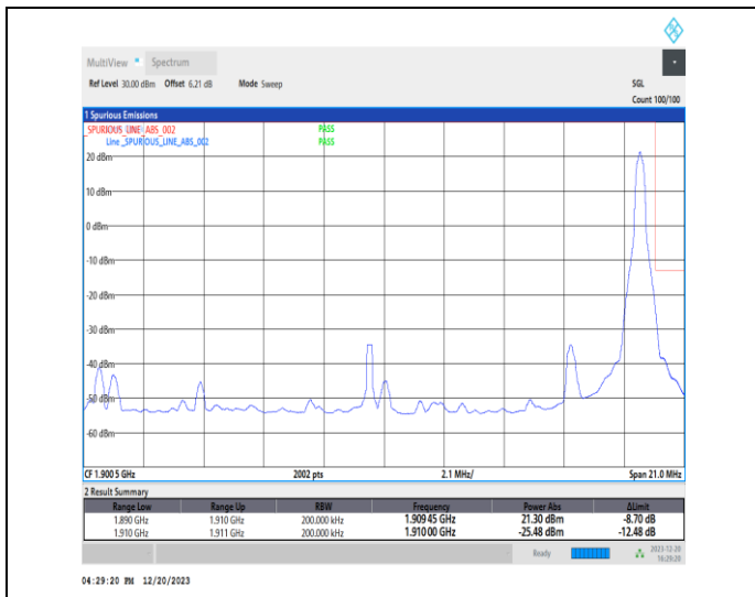
1-N2-15-20-H-2-DFT-PI2BPSK-Edge_1RB_Right-1@105-Ant1-1-seegraph-PASS-see graph
