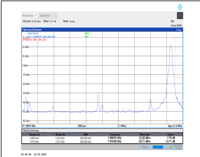
1-N2-PC3-15-20-H-2-DFT-PI2BPSK-Edge_1RB_Right-1@105-Ant1-1-seegraph-PASS-see graph
