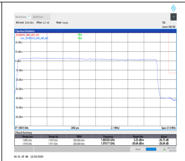
1-N2-15-20-H-3-DFT-PI2BPSK-Outer_Full-100@0-Ant1-1-seegraph-PASS-see graph
