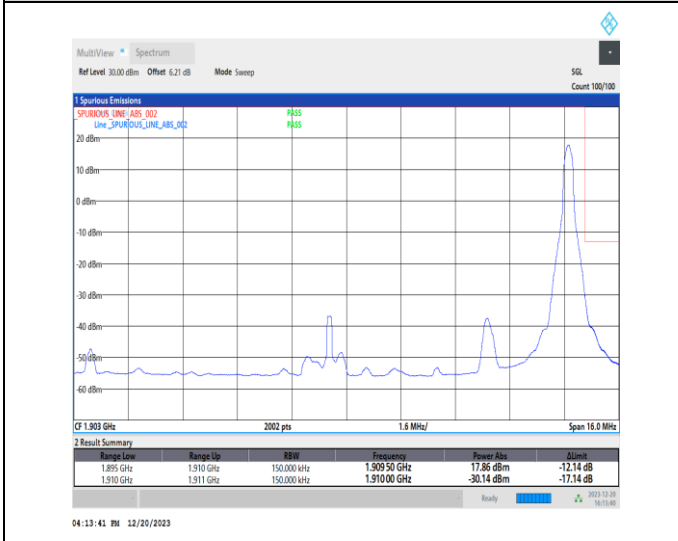
1-N2-15-15-H-5-CP-QPSK-Edge_1RB_Right-1@78-Ant1-1-seegraph-PASS-see graph
