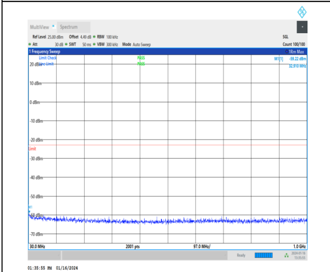
1-N2-15-20-H-1-DFT-PI2BPSK-Inner_1RB_Left-1@ 1-30-1000-Ant1-34.37--59.22--23-PASS
