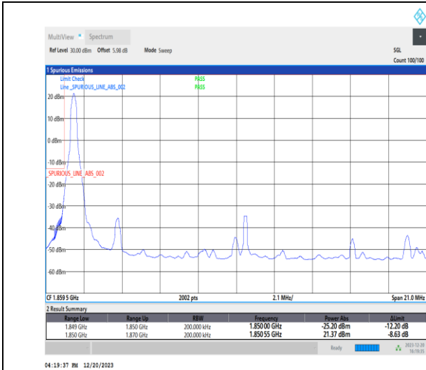
1-N2-15-20-L-1-DFT-PI2BPSK-Edge_1RB_Left-1@0-Ant1-1-seegraph-PASS-see graph
