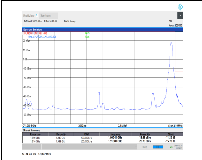
1-N2-15-20-H-5-CP-QPSK-Edge_1RB_Right-1@105-Ant1-1-seegraph-PASS-see graph
