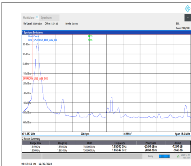
1-N2-15-15-L-1-DFT-PI2BPSK-Edge_1RB_Left-1@0-Ant1-1-seegraph-PASS-see graph
