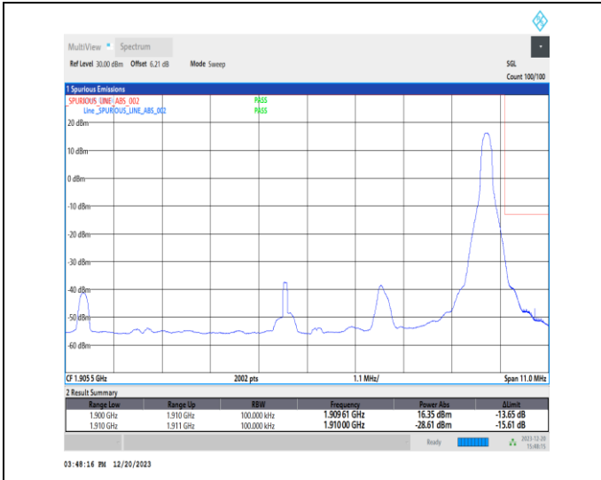
1-N2-15-10-H-2-DFT-PI2BPSK-Edge_1RB_Right-1@5-Ant1-1-seegraph-PASS-see graph
