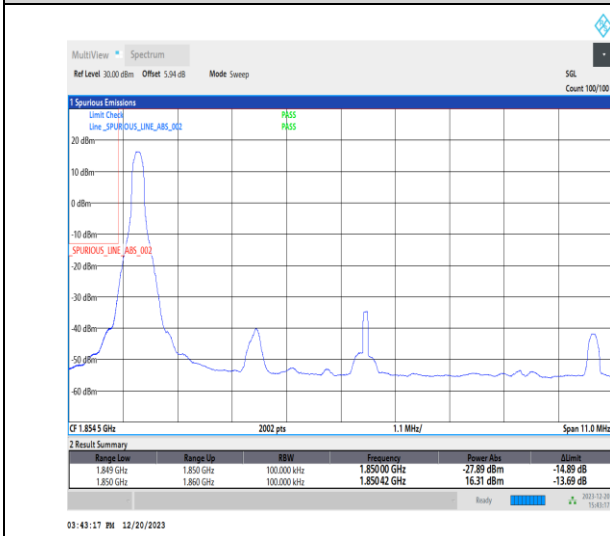
1-N2-15-10-L-4-CP-QPSK-Edge_1RB_Left-1@0-Ant1-1-seegraph-PASS-see graph
