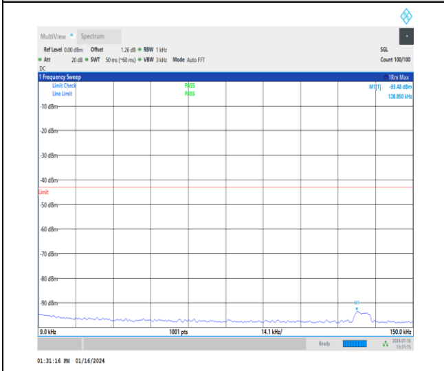
1-N2-15-20-M-1-DFT-PI2BPSK-Inner_1RB_Left-1@ 1-0.009-0.15-Ant1-0.13--93.48--43-PASS
