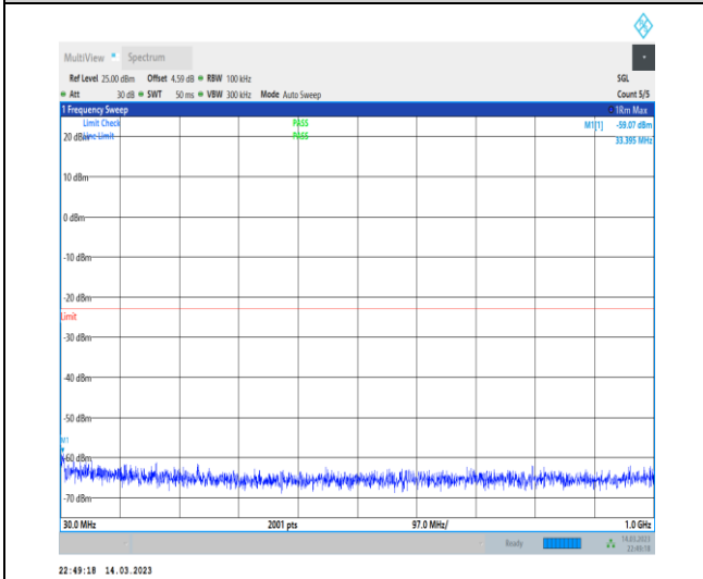
1-N2-PC3-15-20-H-1-DFT-PI2BPSK-Inner_1RB_Lef t-1@1-30-1000-Ant1-33.40--59.07--23-PASS
