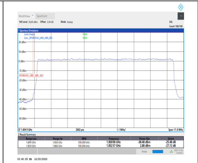
1-N2-15-10-L-3-DFT-PI2BPSK-Outer_Full-50@0-Ant1-1-seegraph-PASS-see graph
