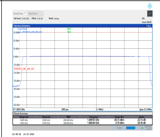
1-N2-PC3-15-20-L-6-CP-QPSK-Outer_Full-106@0-Ant1-1-seegraph-PASS-see graph
