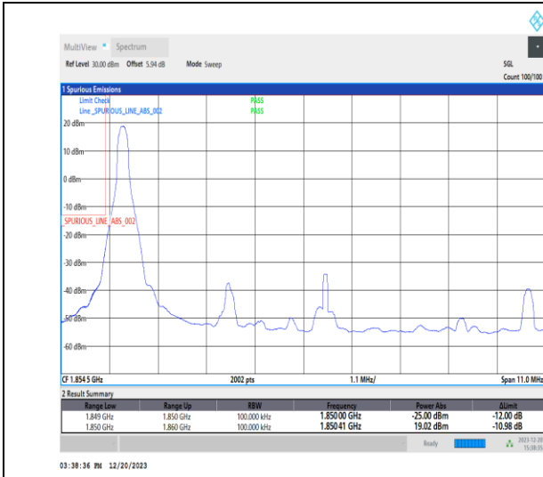
1-N2-15-10-L-1-DFT-PI2BPSK-Edge_1RB_Left-1@0-Ant1-1-seegraph-PASS-see graph
