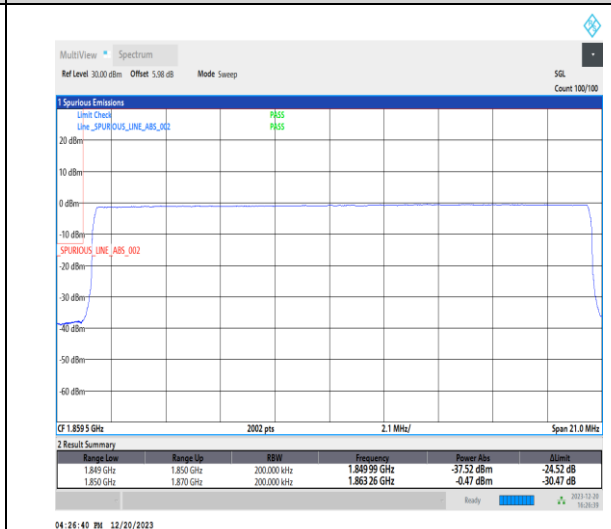
1-N2-15-20-L-6-CP-QPSK-Outer_Full-106@0-Ant1-1-seegraph-PASS-see graph
