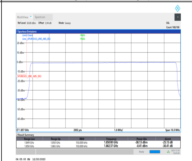
1-N2-15-15-L-6-CP-QPSK-Outer_Full-79@0-Ant1-1-seegraph-PASS-see graph
