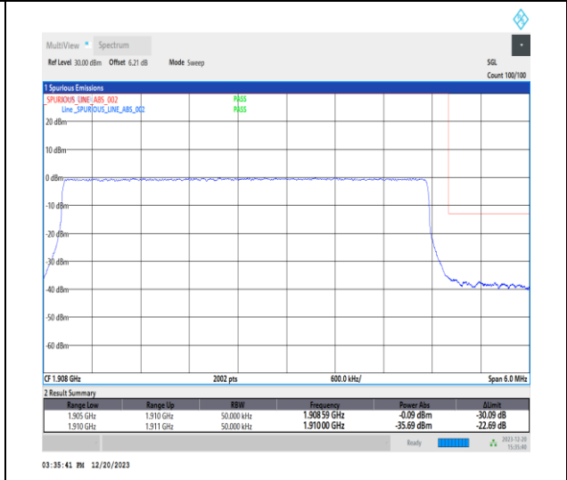
1-N2-15-5-H-6-CP-QPSK-Outer_Full-25@0-Ant1-1-seegraph-PASS-see graph
