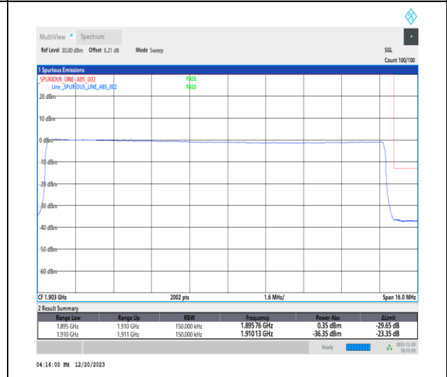
1-N2-15-15-H-6-CP-QPSK-Outer_Full-79@0-Ant1-1-seegraph-PASS-see graph
