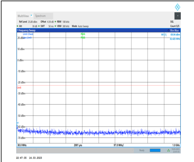
1-N2-PC3-15-20-M-1-DFT-PI2BPSK-Inner_1RB_Lef t-1@1-30-1000-Ant1-32.43--59.94--23-PASS
