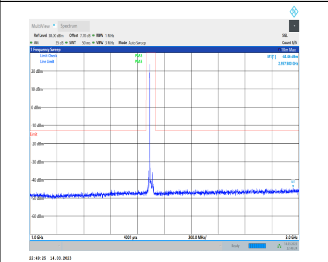
1-N2-PC3-15-20-H-1-DFT-PI2BPSK-Inner_1RB_Left- 1@1-1000-3000-Ant1-2957.50--44.46--13-PASS
