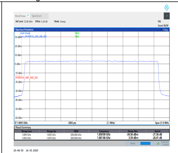
1-N2-PC3-15-20-L-3-DFT-PI2BPSK-Outer_Full-10 @0-Ant1-1-seegraph-PASS-see graph
