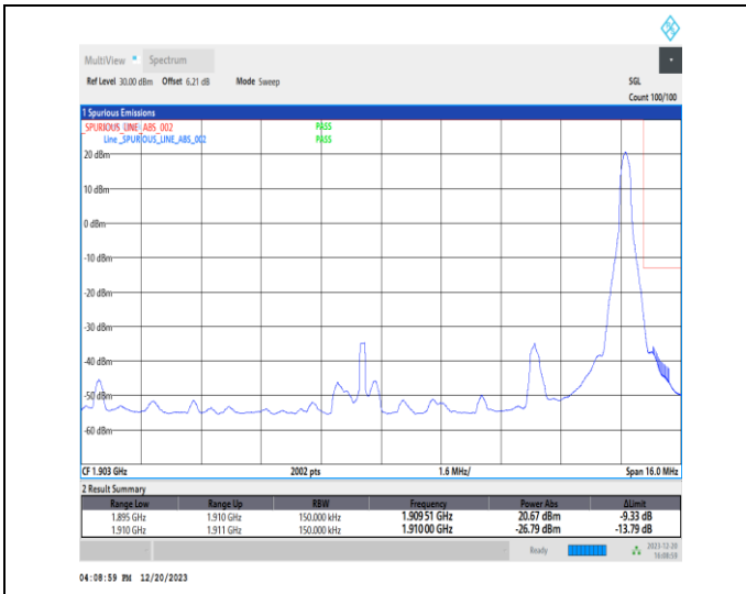
1-N2-15-15-H-2-DFT-PI2BPSK-Edge_1RB_Right-1@7-8-Ant1-1-seegraph-PASS-see graph
