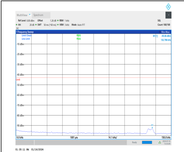
1-N2-15-20-H-1-DFT-PI2BPSK-Inner_1RB_Left-1@ 1-0.009-0.15-Ant1-0.13--93.06--43-PASS
