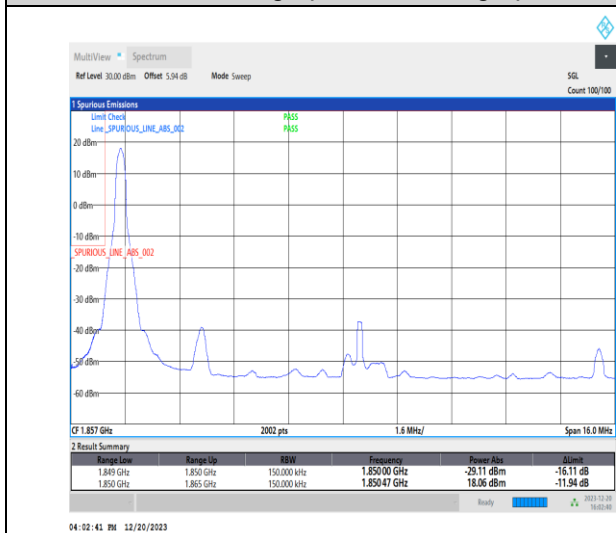
1-N2-15-15-L-4-CP-QPSK-Edge_1RB_Left-1@0-Ant1-1-seegraph-PASS-see graph
