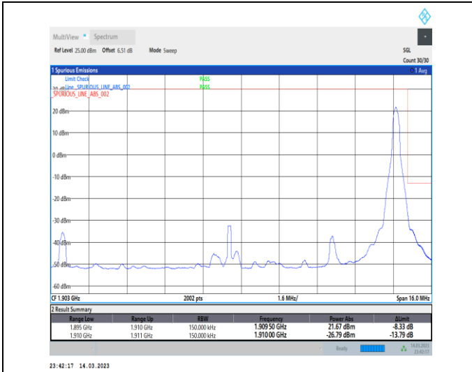
1-N2-PC3-15-15-H-2-DFT-PI2BPSK-Edge_1RB_Right-1@78-Ant1-1-seegraph-PASS-see graph
