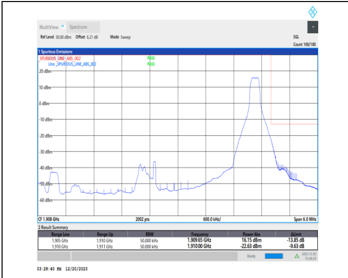
1-N2-15-5-H-2-DFT-PI2BPSK-Edge_1RB_Right-1@24-Ant1-1-seegraph-PASS-see graph
