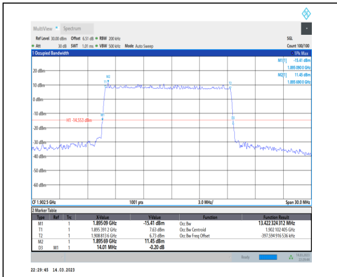
1-N2-PC3-15-15-H-5-DFT-256QAM-Outer_Full-75@ 0-Ant1-13.422-14.010-≤15-PASS
