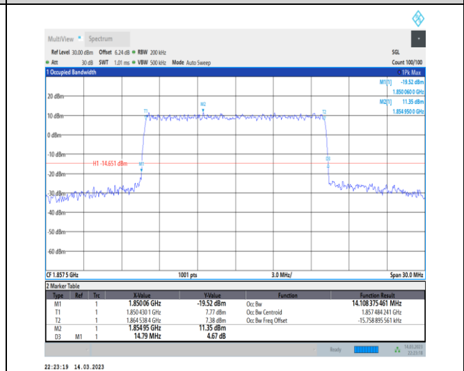
1-N2-PC3-15-15-L-6-CP-QPSK-Outer_Full-79@0-Ant1-14.108-14.790-≤15-PASS
