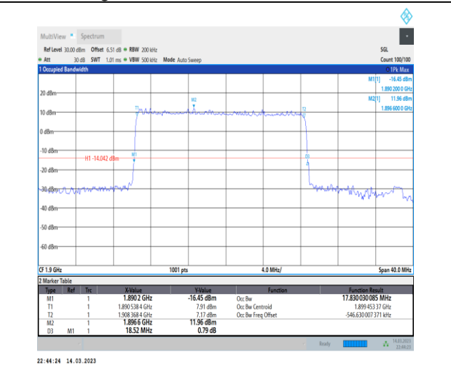
1-N2-PC3-15-20-H-3-DFT-16QAM-Outer_Full-100 @0-Ant1-17.83-18.520-≤20-PASS
