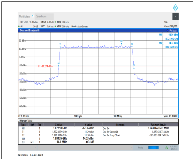
1-N2-PC3-15-15-M-2-DFT-PI2BPSK-Outer_Full-75 @0-Ant1-13.434-14.100-≤15-PASS
