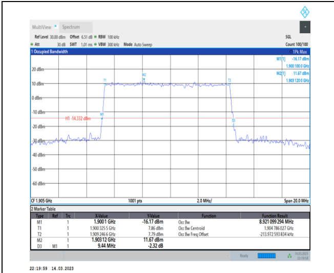
1-N2-PC3-15-10-H-4-DFT-64QAM-Outer_Full-50@0 -Ant1-8.921-9.440-≤10-PASS
