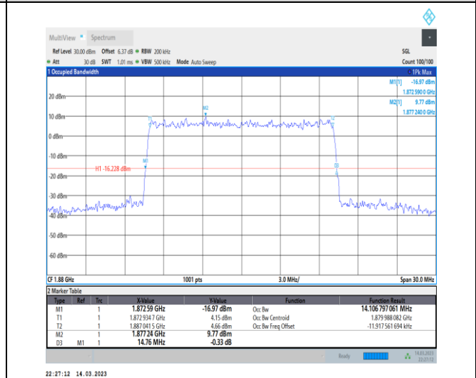
1-N2-PC3-15-15-M-9-CP-256QAM-Outer_Full-79@0-A Ant1-14.107-14.760-≤15-PASS
