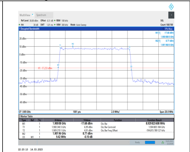
1-N2-PC3-15-10-H-5-DFT-256QAM-Outer_Full-50@0 0-Ant1-8.93-9.420-≤10-PASS
