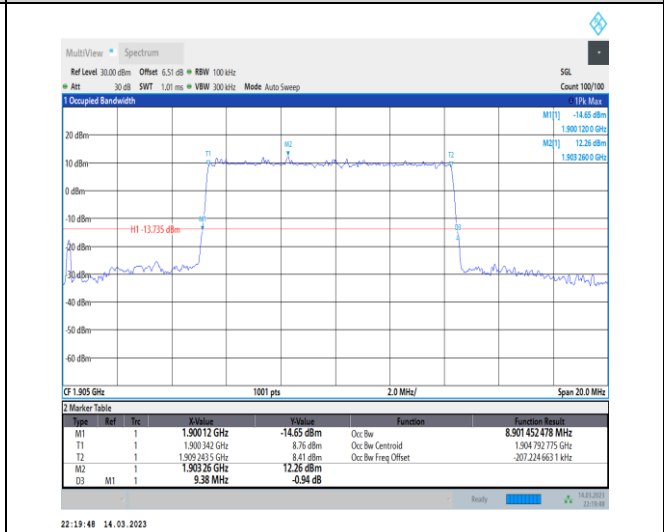
1-N2-PC3-15-10-H-3-DFT-16QAM-Outer_Full-50@0- Ant1-8.901-9.380-≤10-PASS
