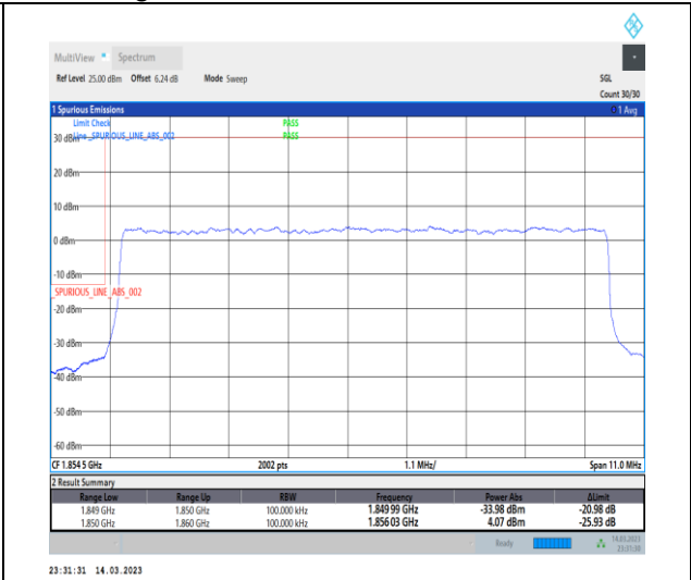
1-N2-PC3-15-10-L-3-DFT-PI2BPSK-Outer_Full-50 @0-Ant1-1-seegraph-PASS-see graph
