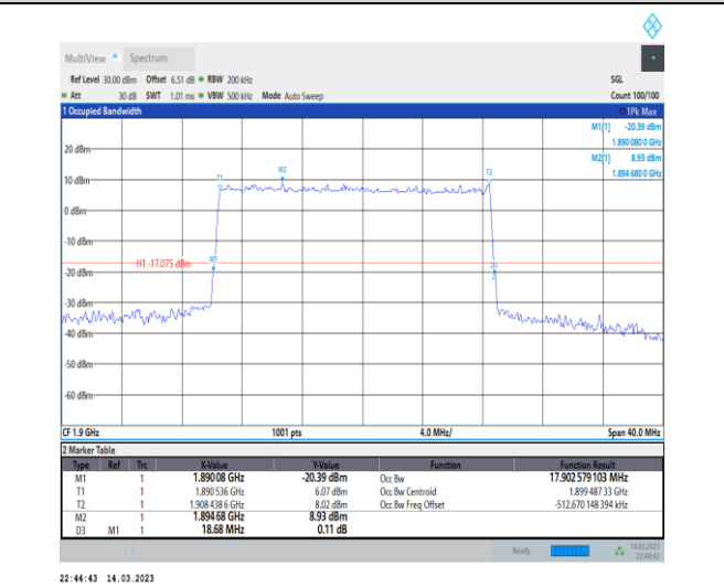
1-N2-PC3-15-20-H-5-DFT-256QAM-Outer_Full-100 @0-Ant1-17.903-18.680-≤20-PASS
