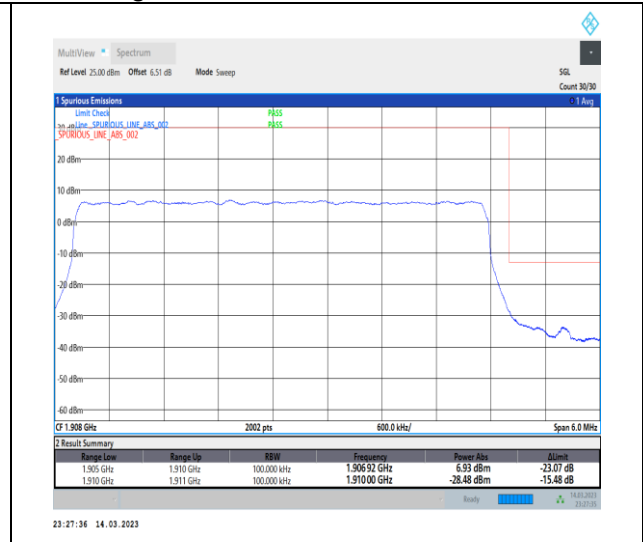
1-N2-PC3-15-5-H-3-DFT-PI2BPSK-Outer_Full-25 @0-Ant1-1-seegraph-PASS-see graph
