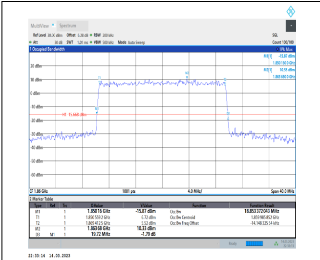
1-N2-PC3-15-20-L-8-CP-64QAM-Outer_Full-106@0-Ant1-18.853-19.720-≤20-PASS
