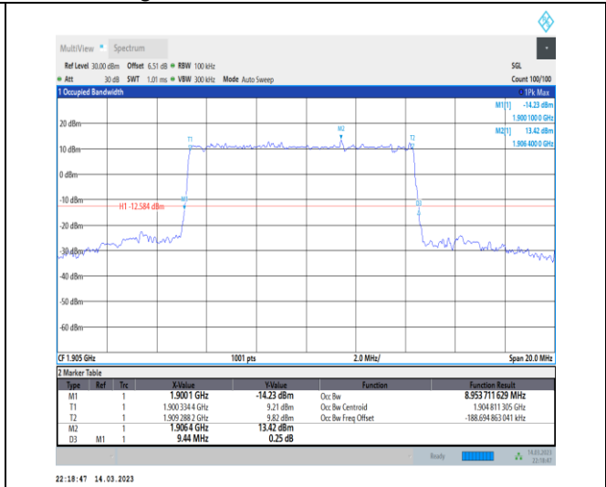
1-N2-PC3-15-10-H-1-DFT-QPSK-Outer_Full-50@0- Ant1-8.954-9.440-≤10-PASS
