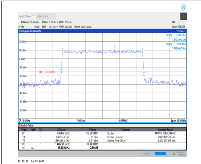
1-N2-PC3-15-20-M-7-CP-16QAM-Outer_Full-106@0 -Ant1-18.915-19.680-≤20-PASS
