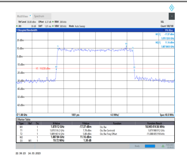
1-N2-PC3-15-20-M-6-CP-QPSK-Outer_Full-106@0-Ant1-18.945-19.720-≤20-PASS
