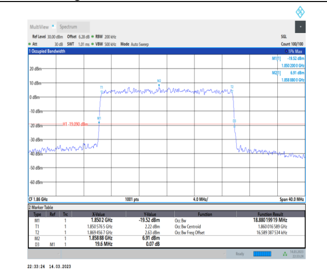
1-N2-PC3-15-20-L-9-CP-256QAM-Outer_Full-106@0-Ant1-18.88-19.600-≤20-PASS
