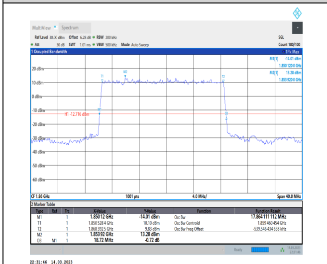
1-N2-PC3-15-20-L-2-DFT-PI2BPSK-Outer_Full-100 @0-Ant1-17.864-18.720-≤20-PASS
