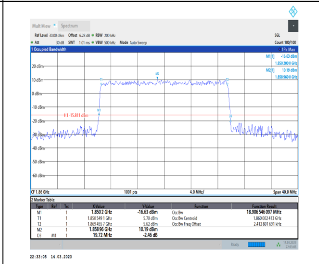
1-N2-PC3-15-20-L-7-CP-16QAM-Outer_Full-106@0-Ant1-18.907-19.720-≤20-PASS
