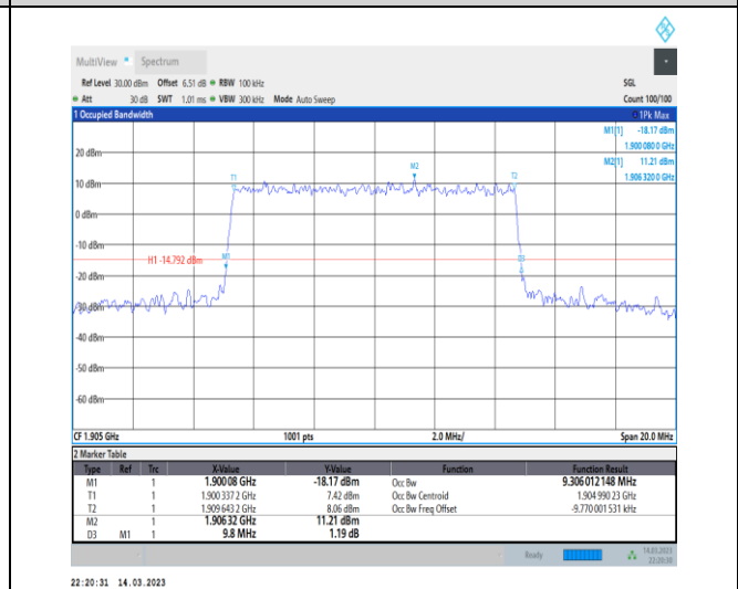
1-N2-PC3-15-10-H-7-CP-16QAM-Outer_Full-52@0- Ant1-9.306-9.800-≤10-PASS
