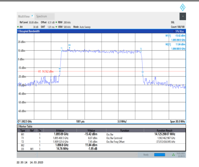
1-N2-PC3-15-15-H-8-CP-64QAM-Outer_Full-79@0- Ant1-14.125-14.760-≤15-PASS
