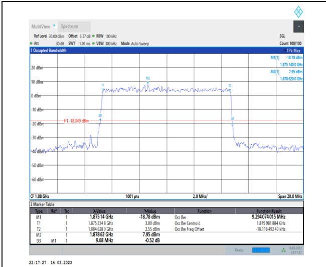
1-N2-PC3-15-10-M-9-CP-256QAM-Outer_Full-52@0 -Ant1-9.294-9.680-≤10-PASS
