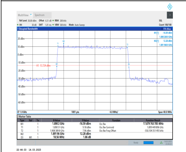
1-N2-PC3-15-20-H-4-DFT-64QAM-Outer_Full-100 @0-Ant1-17.88-18.560-≤20-PASS
