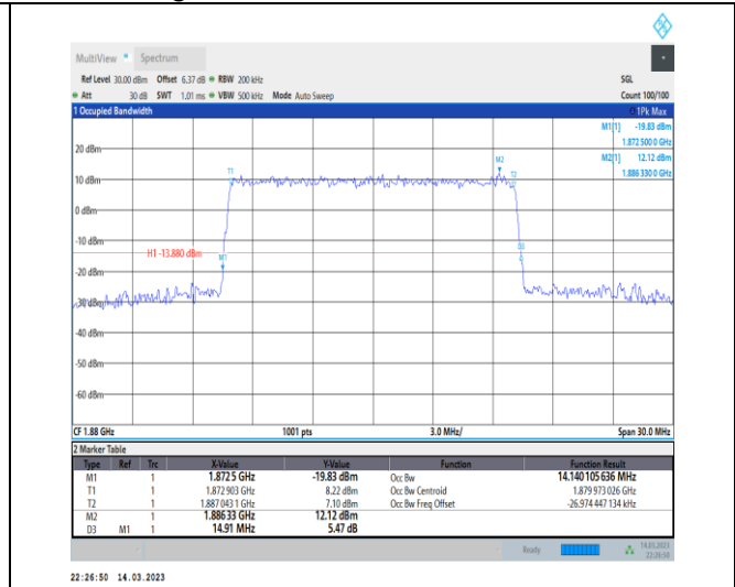
1-N2-PC3-15-15-M-7-CP-16QAM-Outer_Full-79@0-A Ant1-14.14-14.910-≤15-PASS
