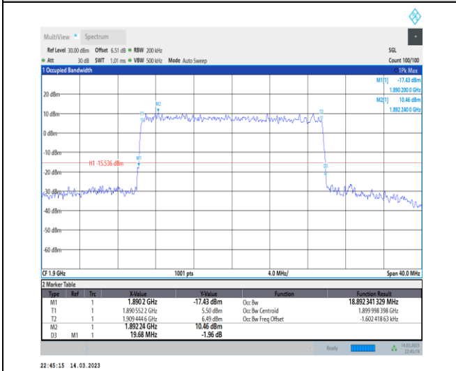
1-N2-PC3-15-20-H-8-CP-64QAM-Outer_Full-106@0-Ant1-18.892-19.680-≤20-PASS
