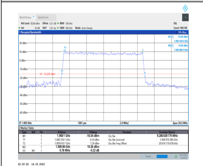
1-N2-PC3-15-10-H-6-CP-QPSK-Outer_Full-52@0-A nt1-9.281-9.780-≤10-PASS
