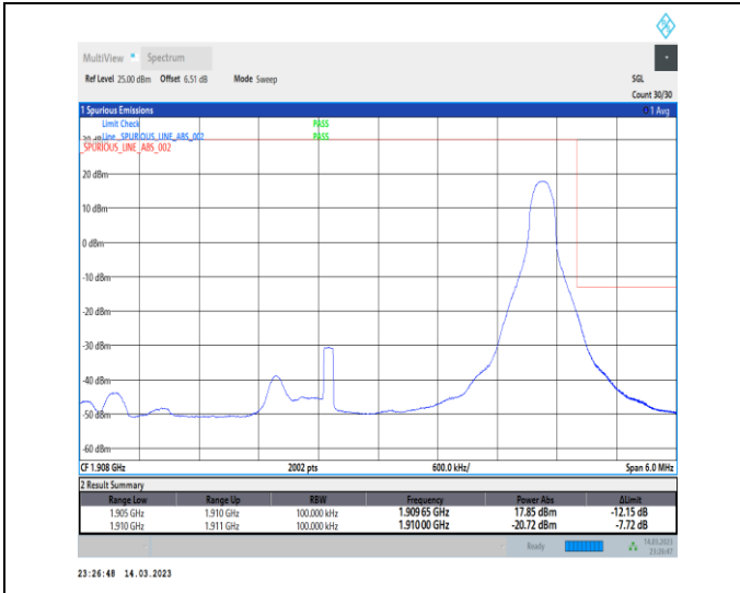
1-N2-PC3-15-5-H-2-DFT-PI2BPSK-Edge_1RB_Right-1 @24-Ant1-1-seegraph-PASS-see graph
