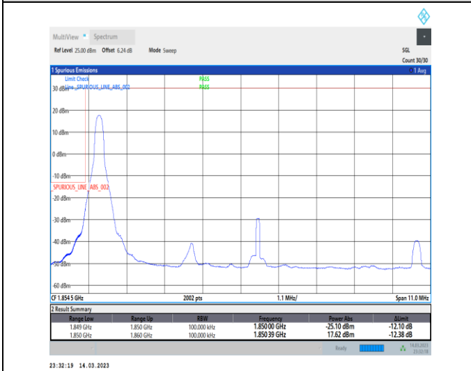
1-N2-PC3-15-10-L-4-CP-QPSK-Edge_1RB_Left-1@0-Ant1-1-seegraph-PASS-see graph
