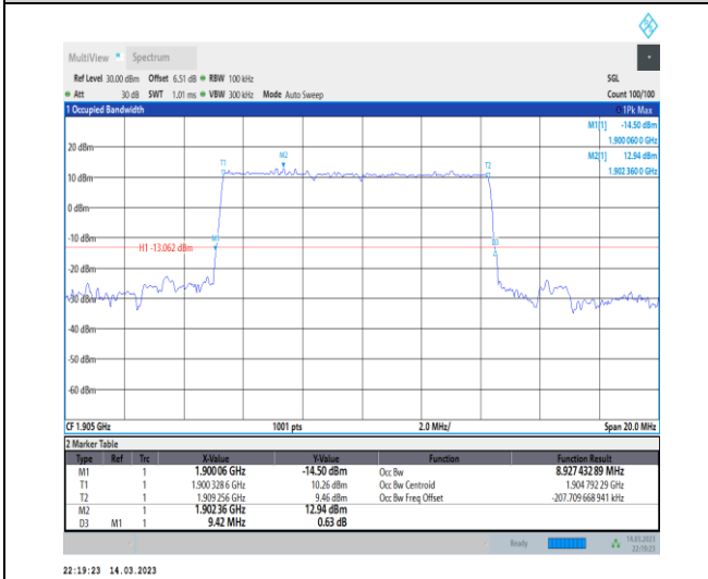
1-N2-PC3-15-10-H-2-DFT-PI2BPSK-Outer_Full-50@0- Ant1-8.927-9.420-≤10-PASS
