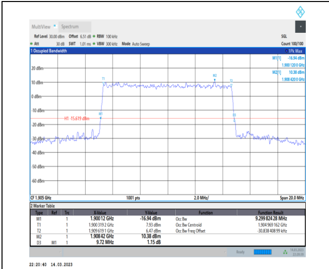
1-N2-PC3-15-10-H-8-CP-64QAM-Outer_Full-52@0-Ant1-9.3-9.720-≤10-PASS
