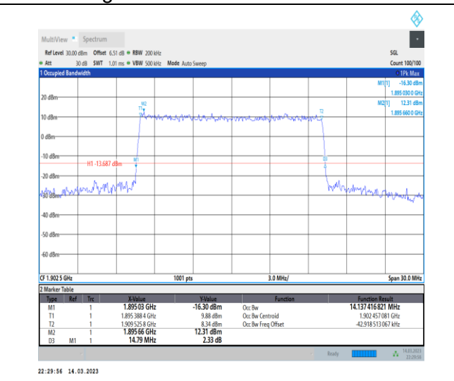
1-N2-PC3-15-15-H-6-CP-QPSK-Outer_Full-79@0-A nt1-14.137-14.790-≤15-PASS
