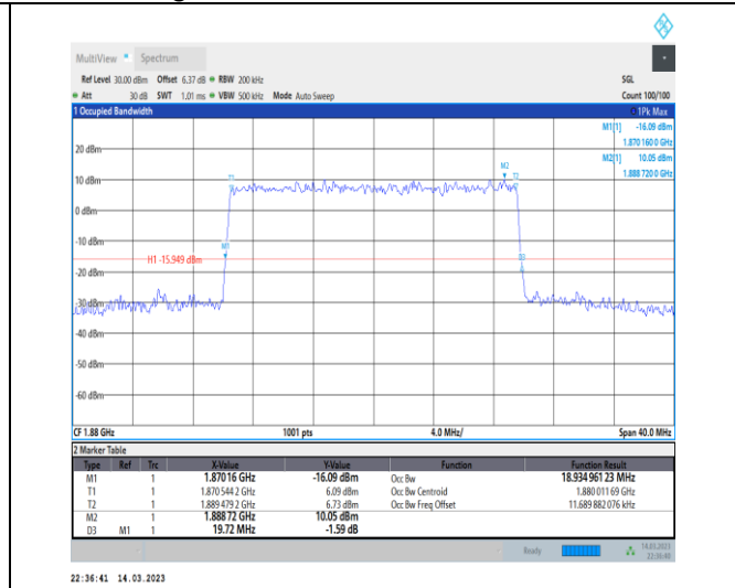
1-N2-PC3-15-20-M-8-CP-64QAM-Outer_Full-106@0 -Ant1-18.935-19.720-≤20-PASS
