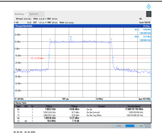
1-N2-PC3-15-20-L-3-DFT-16QAM-Outer_Full-100@ 0-Ant1-17.87-18.600-≤20-PASS
