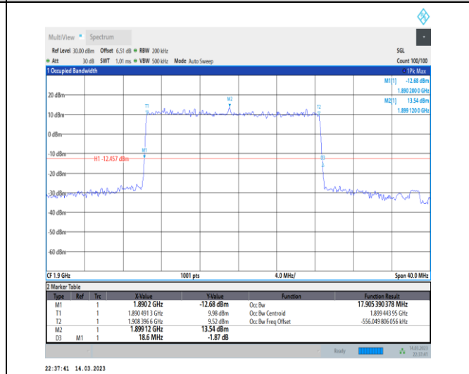
1-N2-PC3-15-20-H-1-DFT-QPSK-Outer_Full-100@0- Ant1-17.905-18.600-≤20-PASS
