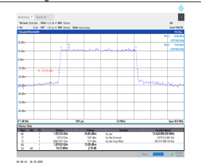
1-N2-PC3-15-15-M-3-DFT-16QAM-Outer_Full-75@0-Ant1-13.424-14.130-≤15-PASS
