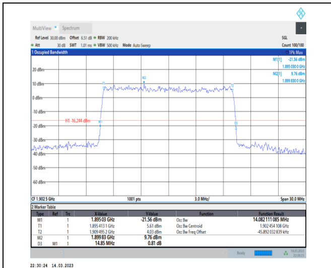
1-N2-PC3-15-15-H-9-CP-256QAM-Outer_Full-79@0 -Ant1-14.082-14.850-≤15-PASS
