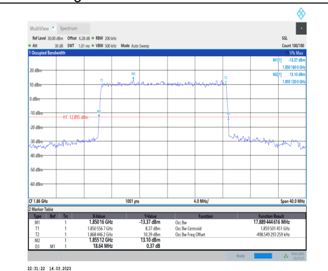
1-N2-PC3-15-20-L-1-DFT-QPSK-Outer_Full-100@0 Ant1-17.889-18.640-≤20-PASS
