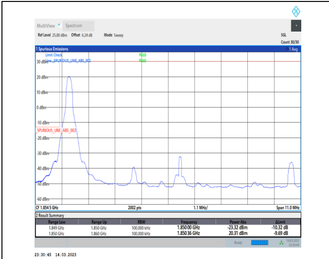
1-N2-PC3-15-10-L-1-DFT-PI2BPSK-Edge_1RB_Left-1 @0-Ant1-1-seegraph-PASS-see graph
