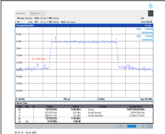
1-N2-PC3-15-15-M-8-CP-64QAM-Outer_Full-79@0-A Ant1-14.098-14.790-≤15-PASS
