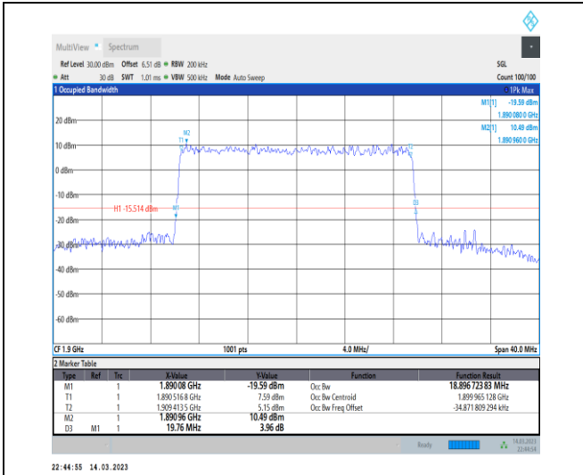
1-N2-PC3-15-20-H-6-CP-QPSK-Outer_Full-106@0-Ant1-18.897-19.760-≤20-PASS
