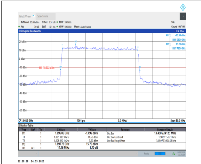
1-N2-PC3-15-15-H-1-DFT-QPSK-Outer_Full-75@0-Ant1-13.45-14.160-≤15-PASS
