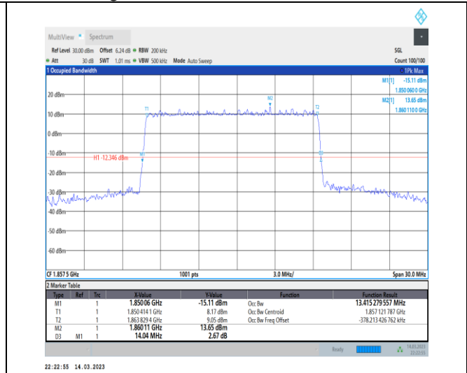
1-N2-PC3-15-15-L-4-DFT-64QAM-Outer_Full-75@0-Ant1-13.415-14.040-≤15-PASS
