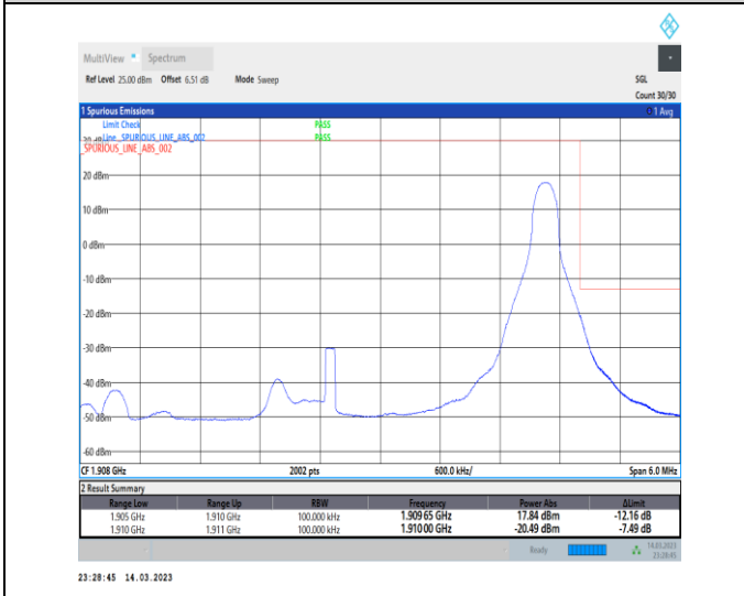
1-N2-PC3-15-5-H-5-CP-QPSK-Edge_1RB_Right-1@24-Ant1-1-seegraph-PASS-see graph
