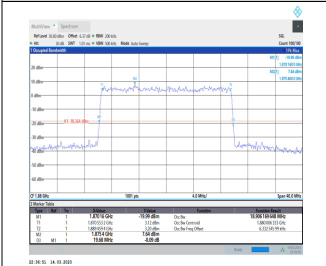
1-N2-PC3-15-20-M-9-CP-256QAM-Outer_Full-106@0 0-Ant1-18.906-19.680-≤20-PASS
