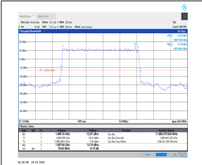
1-N2-PC3-15-20-H-2-DFT-PI2BPSK-Outer_Full-100 @0-Ant1-17.885-18.640-≤20-PASS
