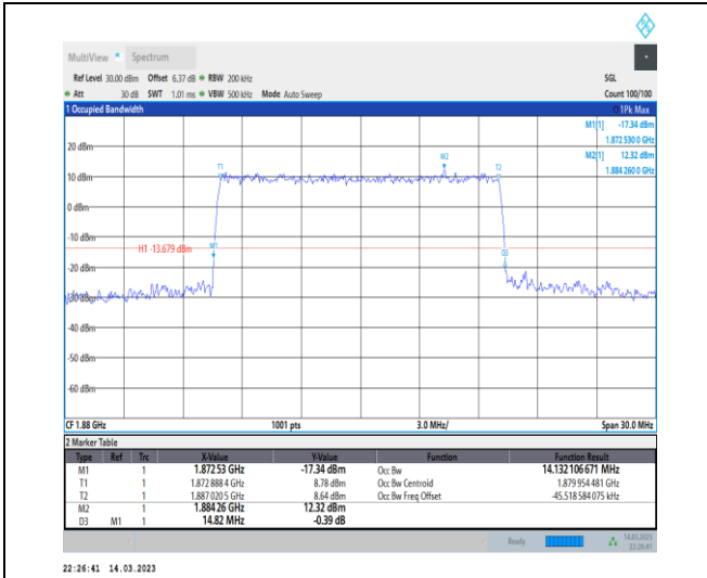
1-N2-PC3-15-15-M-6-CP-QPSK-Outer_Full-79@0-A Ant1-14.132-14.820-≤15-PASS
