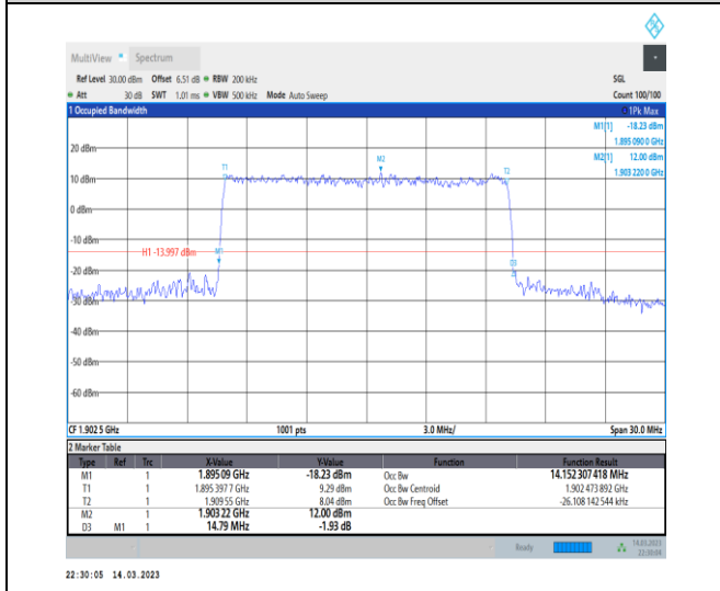
1-N2-PC3-15-15-H-7-CP-16QAM-Outer_Full-79@0- Ant1-14.152-14.790-≤15-PASS
