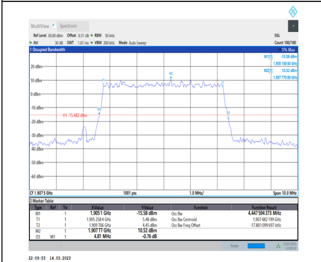
1-N2-PC3-15-5-H-5-DFT-256QAM-Outer_Full-25@0-Ant1-4.448-4.810-≤5-PASS
