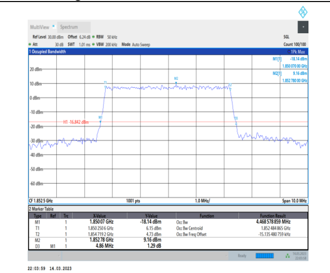
1-N2-PC3-15-5-L-6-CP-QPSK-Outer_Full-25@0-Ant 1-4.469-4.860-≤5-PASS
