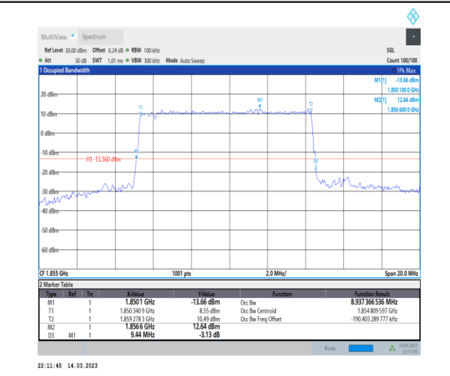
1-N2-PC3-15-10-L-1-DFT-QPSK-Outer_Full-50@0-A nt1-8.937-9.440-≤10-PASS
