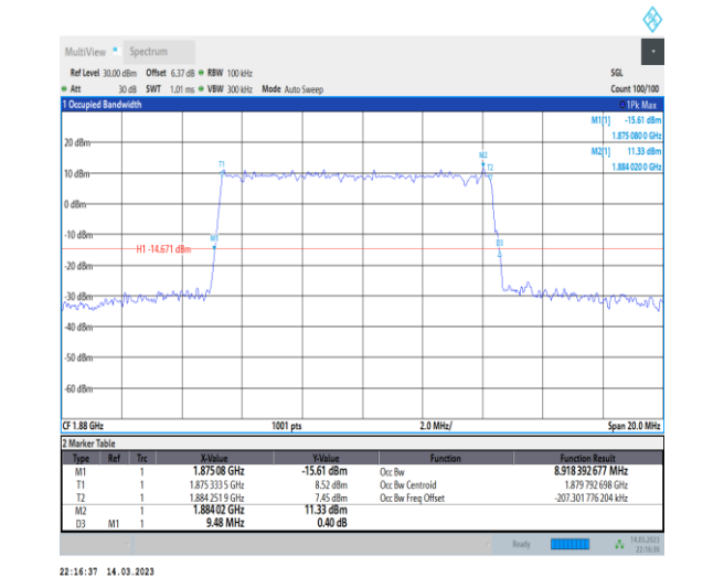
1-N2-PC3-15-10-M-4-DFT-64QAM-Outer_Full-50@0-Ant1-8.918-9.480-≤10-PASS
