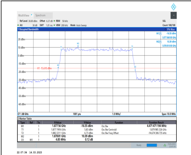
1-N2-PC3-15-5-M-8-CP-64QAM-Outer_Full-25@0-A nt1-4.471-4.850-≤5-PASS
