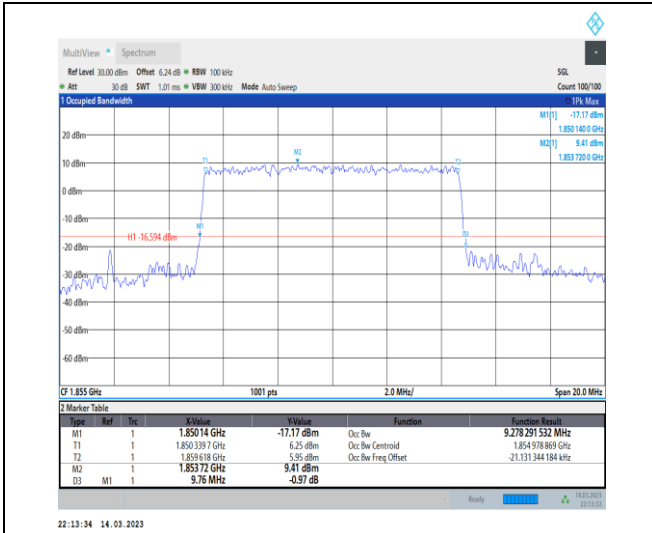
1-N2-PC3-15-10-L-6-CP-QPSK-Outer_Full-52@0-A nt1-9.278-9.760-≤10-PASS
