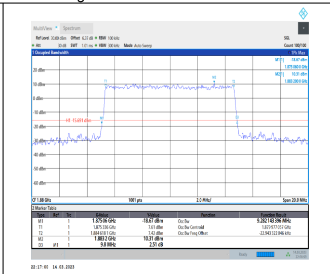
1-N2-PC3-15-10-M-6-CP-QPSK-Outer_Full-52@0-Ant1-9.282-9.800-≤10-PASS
