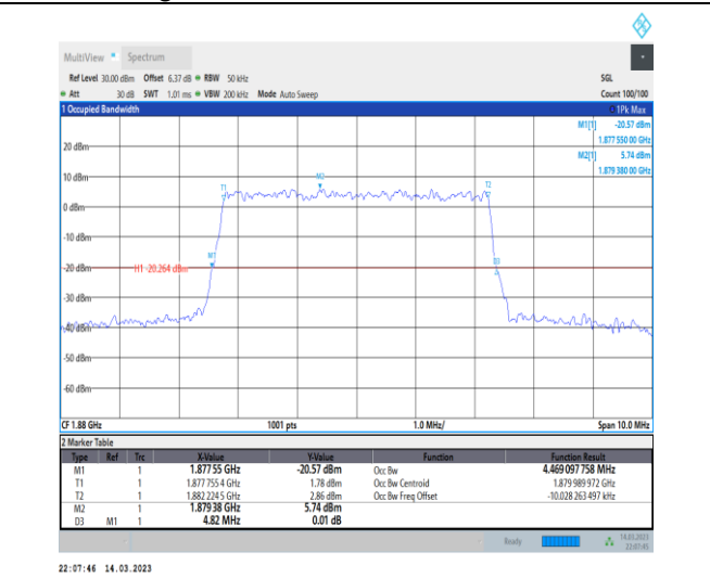
1-N2-PC3-15-5-M-9-CP-256QAM-Outer_Full-25@0- Ant1-4.469-4.820-≤5-PASS
