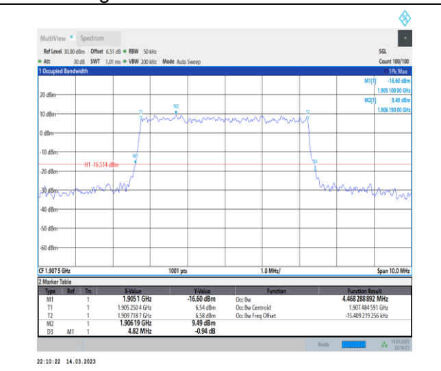
1-N2-PC3-15-5-H-8-CP-64QAM-Outer_Full-25@0-A nt1-4.468-4.820-≤5-PASS
