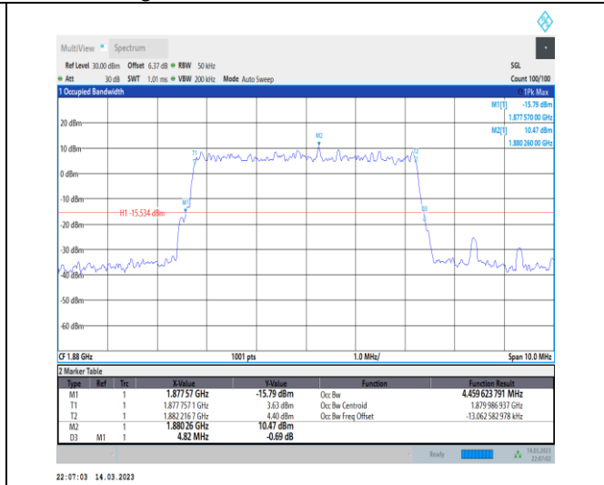
1-N2-PC3-15-5-M-5-DFT-256QAM-Outer_Full-25@0-Ant1-4.46-4.820-≤5-PASS
