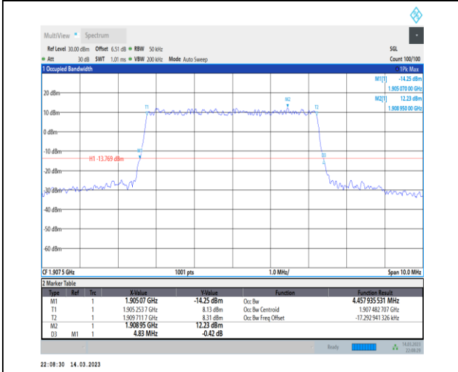
1-N2-PC3-15-5-H-1-DFT-QPSK-Outer_Full-25@0-A nt1-4.458-4.830-≤5-PASS
