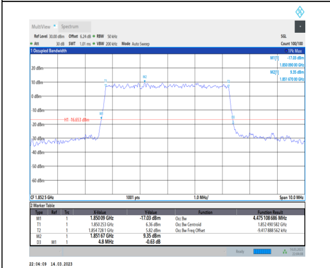
1-N2-PC3-15-5-L-7-CP-16QAM-Outer_Full-25@0-Ant1-4.475-4.800-≤5-PASS
