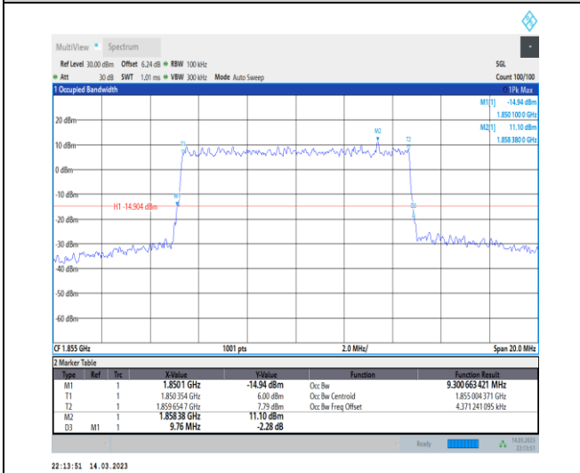
1-N2-PC3-15-10-L-8-CP-64QAM-Outer_Full-52@0-A Ant1-9.301-9.760-≤10-PASS
