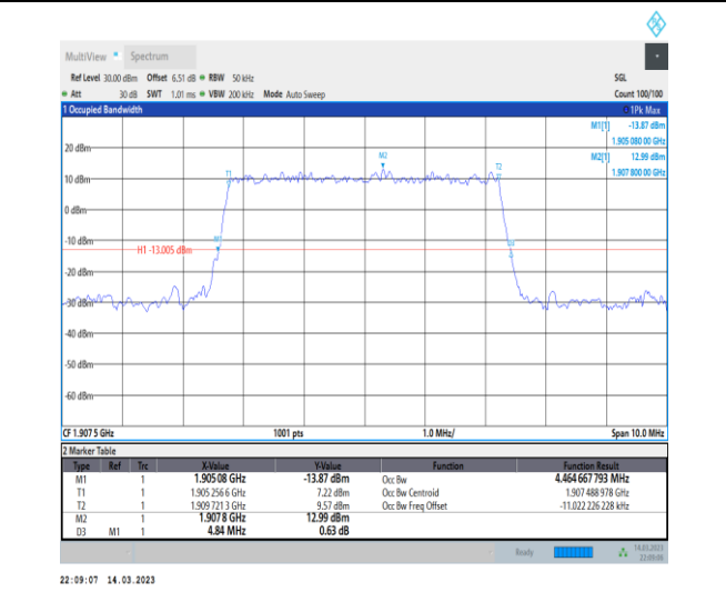
1-N2-PC3-15-5-H-2-DFT-PI2BPSK-Outer_Full-25@0- -Ant1-4.465-4.840-≤5-PASS
