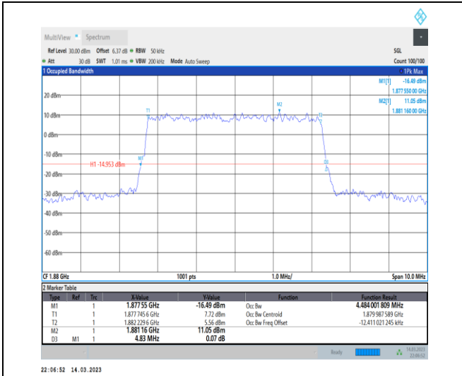
1-N2-PC3-15-5-M-4-DFT-64QAM-Outer_Full-25@0-Ant1-4.484-4.830-≤5-PASS
