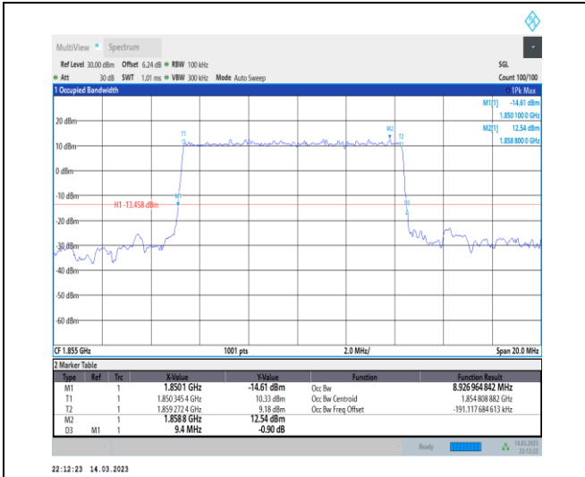
1-N2-PC3-15-10-L-2-DFT-PI2BPSK-Outer_Full-50@0-Ant1-8.927-9.400-≤10-PASS
