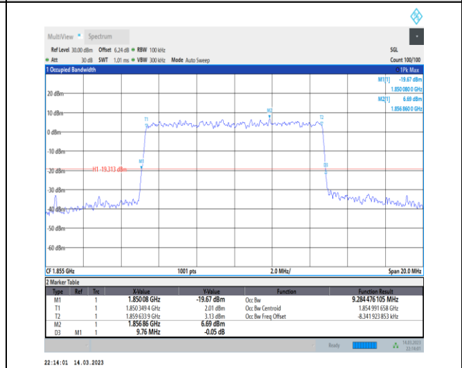
1-N2-PC3-15-10-L-9-CP-256QAM-Outer_Full-52@0-A Ant1-9.284-9.760-≤10-PASS
