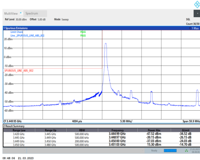
42-42-10MHz-20MHz-QPSK-QPSK-42145-42289-50RB#0-100RB#0
