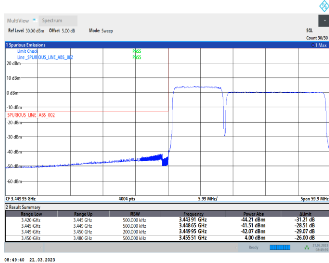
42-42-10MHz-20MHz-QPSK-QPSK-42145-42289-50RB#0-100RB#0
