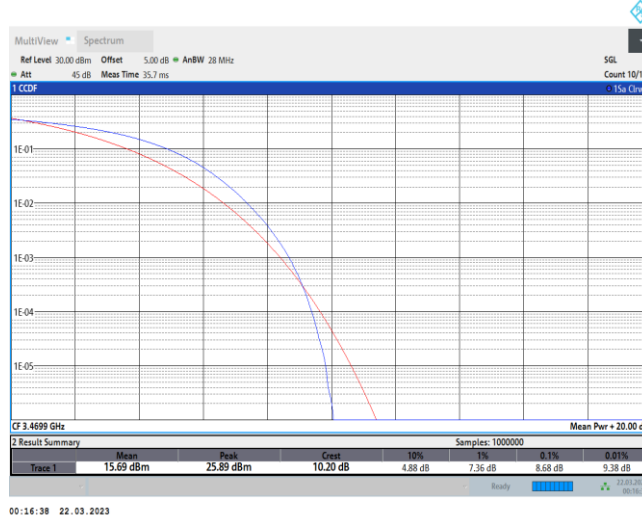
42-42-20MHz-20MHz-QPSK-QPSK-42491-42689-100RB#0-100RB#0
