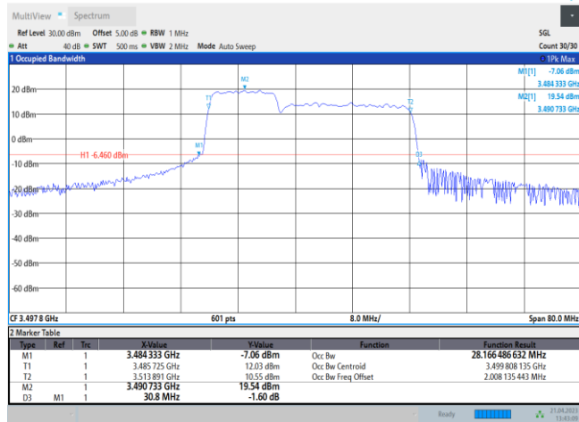
42-42-10MHz-20MHz-QPSK-QPSK-42496-42640-50RB#0-100RB#0
