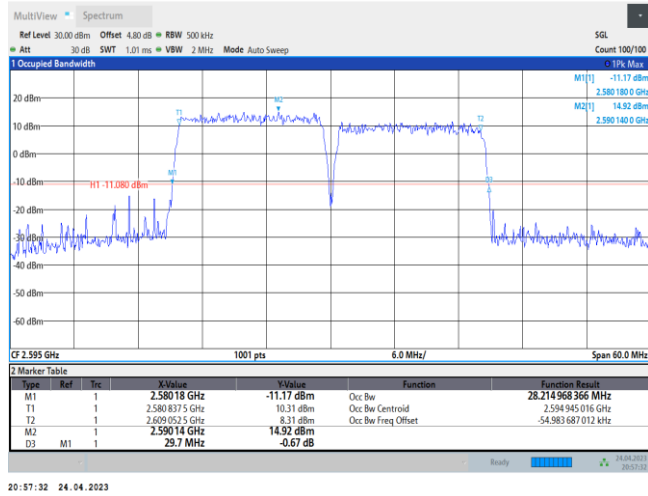
38-38-15MHz-15MHz-QPSK-QPSK-37925-38075-75RB#0-75RB#0
