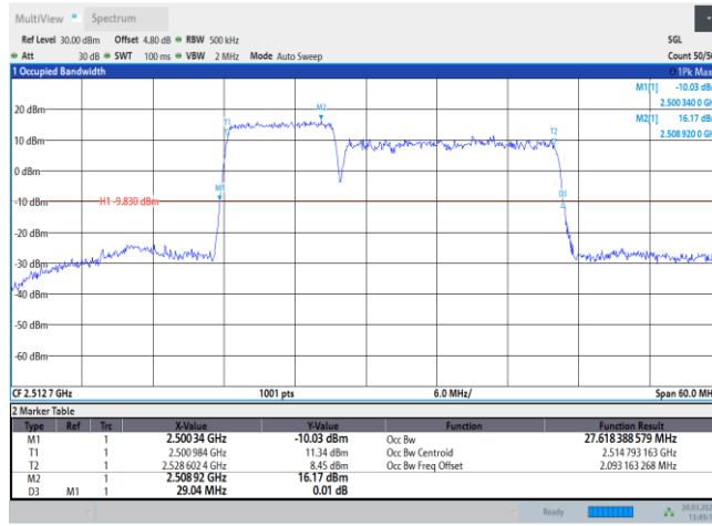
7-7-10MHz-20MHz-QPSK-QPSK-21006-21150-50RB#0-100RB#0
