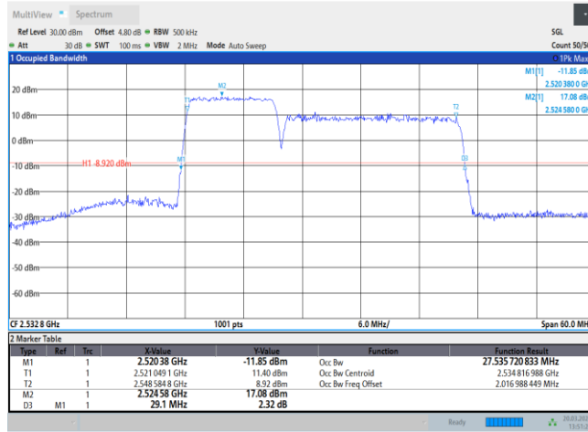
7-7-10MHz-20MHz-QPSK-QPSK-21006-21150-50RB#0-100RB#0
