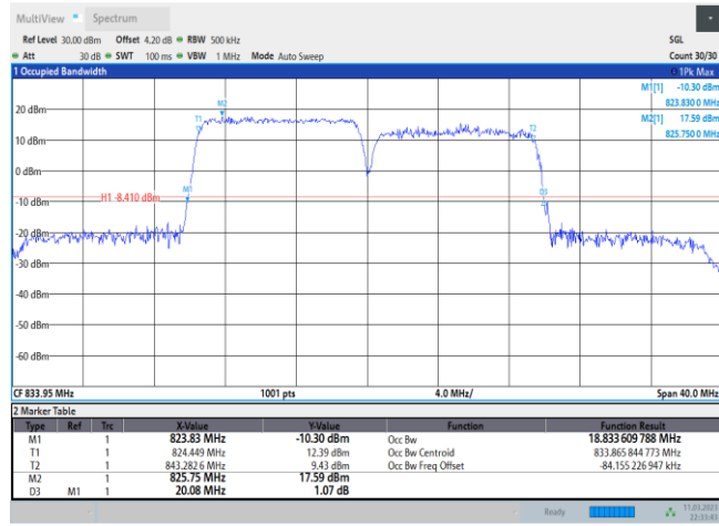
5-5-10MHz-10MHz-QPSK-QPSK-20476-20575-50RB#0-50RB#0
