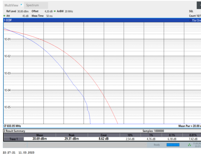
5-5-10MHz-10MHz-QPSK-QPSK-20476-20575-50RB#0-50RB#0
