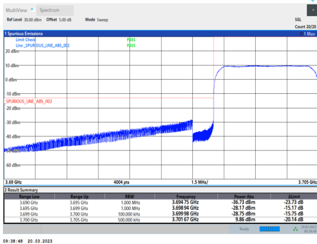
Band43-5MHz-QPSK-44615-25RB#0
