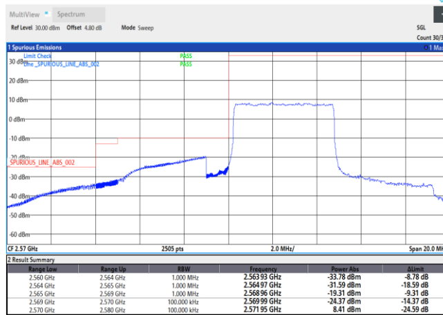
Band38-5MHz-QPSK-37775-25RB#0
