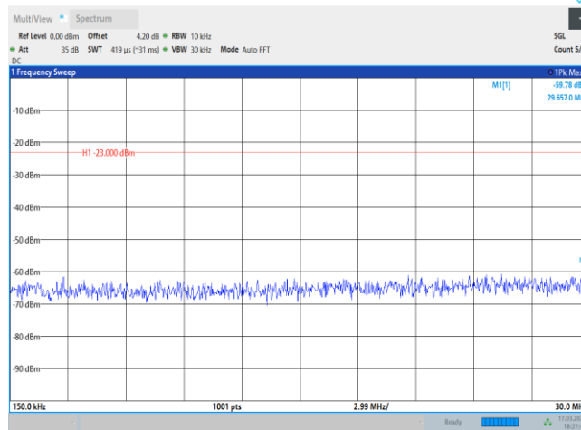
Band17-10MHz-QPSK-23780-1RB#0-Range2:0.15~30MHz
