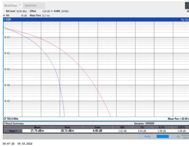
Band14-10MHz-16QAM-23330-50RB#0
