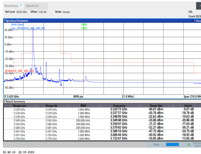
48-48-10MHz-20MHz-QPSK-QPSK-55295-55439-50RB#0-100RB#0
