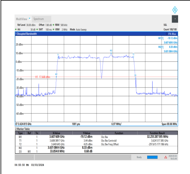
NTNV_CA_n48B_PC3_30+30_20+15_M+M_Ant0_TID8_1_#1
