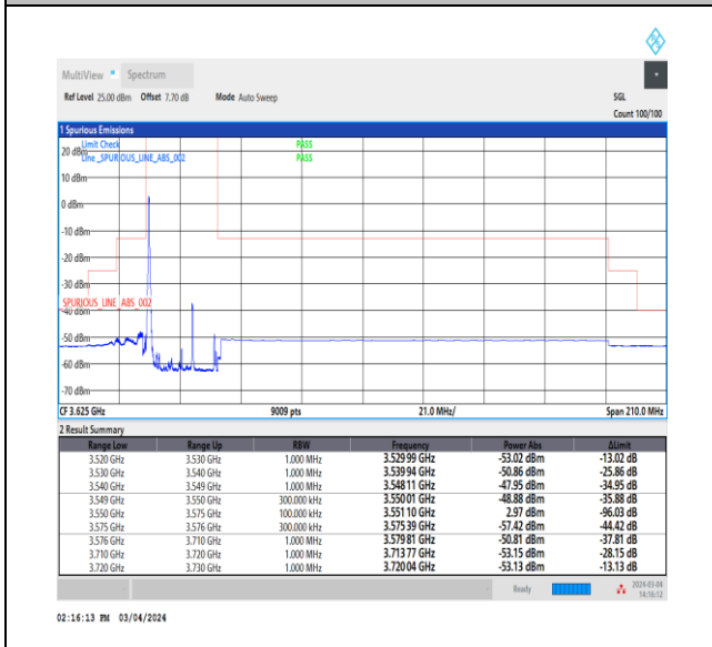
NTNV_CA_n48B_PC3_30+30_15+10_L+L_TID4_1_#1
