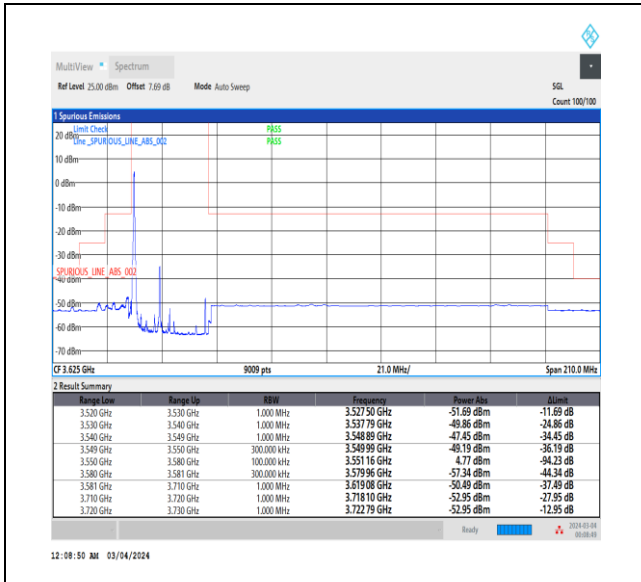
NTNV_CA_n48B_PC3_30+30_10+20_L+L_TID1_1_#1
