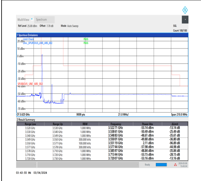
NTNV_CA_n48B_PC3_30+30_15+15_L+L_TID4_1_#1
