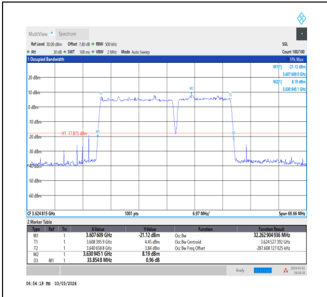
NTNV_CA_n48B_PC3_30+30_20+15_M+M_Ant0_TID2_1_#1
