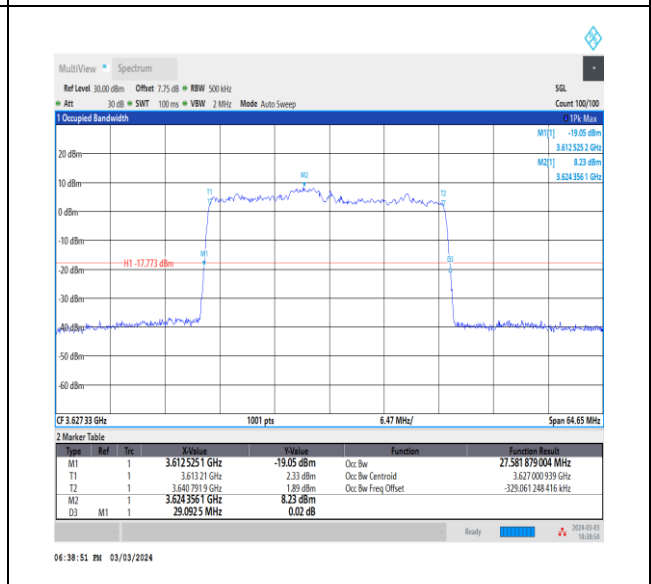
NTNV_CA_n48B_PC3_30+30_15+20_M+M_Ant0_TID7_1_#1
