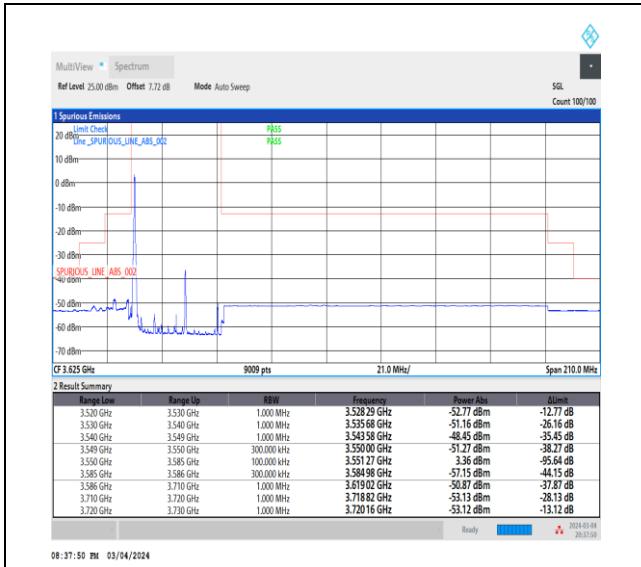
NTNV_CA_n48B_PC3_30+30_20+15_L+L_TID1_1_#1
