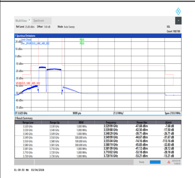
NTNV_CA_n48B_PC3_30+30_10+20_L+L_TID6_1_#1
