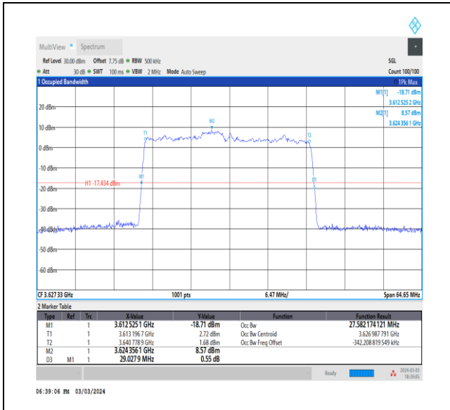
NTVN_CA_n48B_PC3_30+30_15+20_M+M_Ant0_TID8_1_#1
