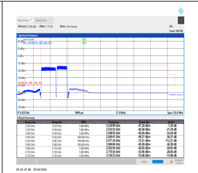
NTNV_CA_n48B_PC3_30+30_20+15_L+L_TID3_1_#1
