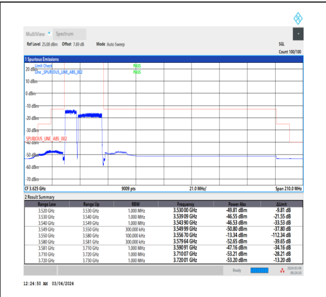
NTNV_CA_n48B_PC3_30+30_10+20_L+L_TID3_1_#1
