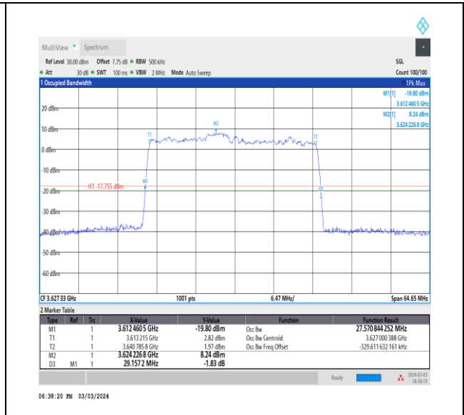
NTNV_CA_n48B_PC3_30+30_15+20_M+M_Ant0_TID5_1_#1
