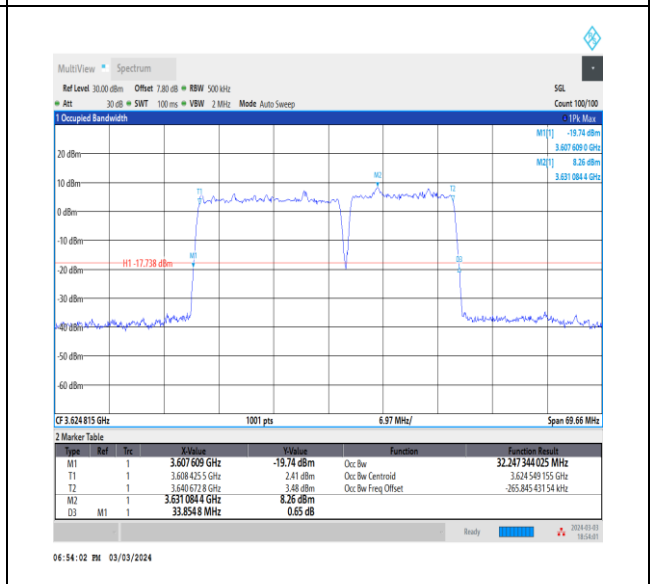
NTNV_CA_n48B_PC3_30+30_20+15_M+M_Ant0_TID1_1_#1
