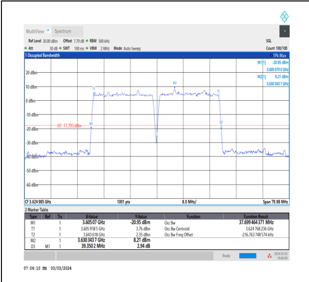
NTNV_CA_n48B_PC3_30+30_20+20_M+M_Ant0_TID5_1_#1
