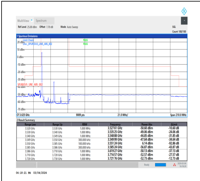
NTNV_CA_n48B_PC3_30+30_15+20_L+L_TID1_1_#1
