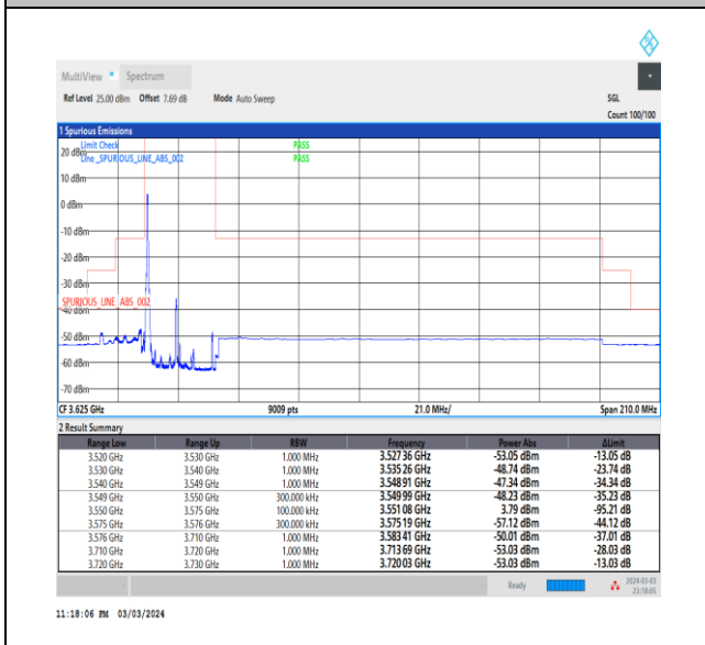
NTNV_CA_n48B_PC3_30+30_10+15_L+L_TID4_1_#1
