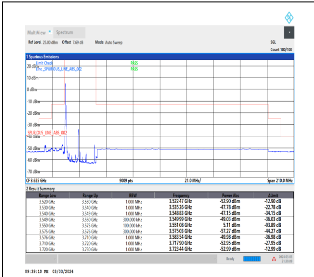
NTNV_CA_n48B_PC3_30+30_10+15_L+L_TID1_1_#1
