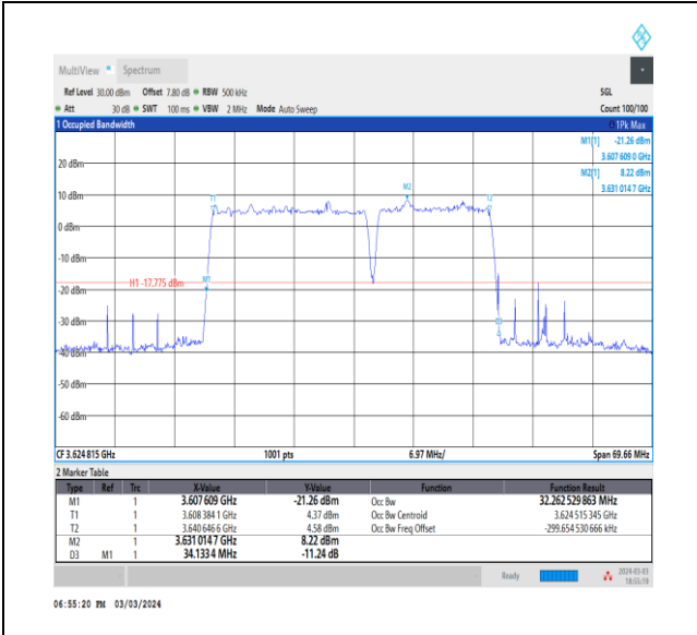
NTNV_CA_n48B_PC3_30+30_20+15_M+M_Ant0_TID6_1_#1
