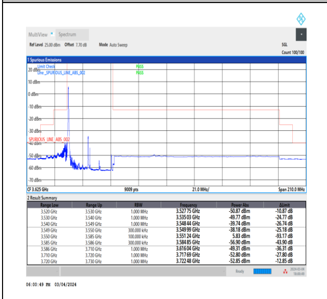
NTNV_CA_n48B_PC3_30+30_15+20_L+L_TID4_1_#1
