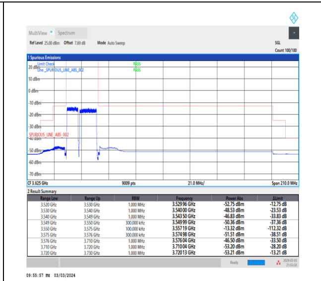
NTNV_CA_n48B_PC3_30+30_10+15_L+L_TID3_1_#1
