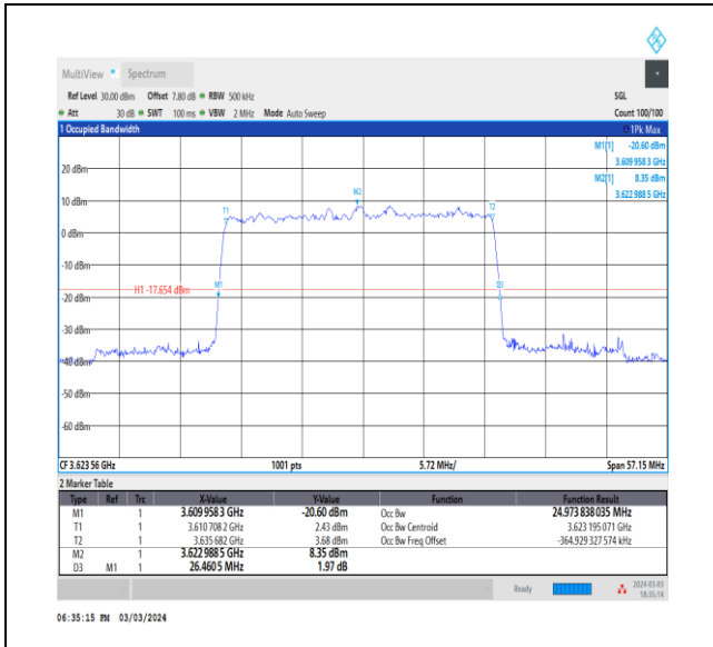
NTNV_CA_n48B_PC3_30+30_15+15_M+M_Ant0_TID9_1_#1
