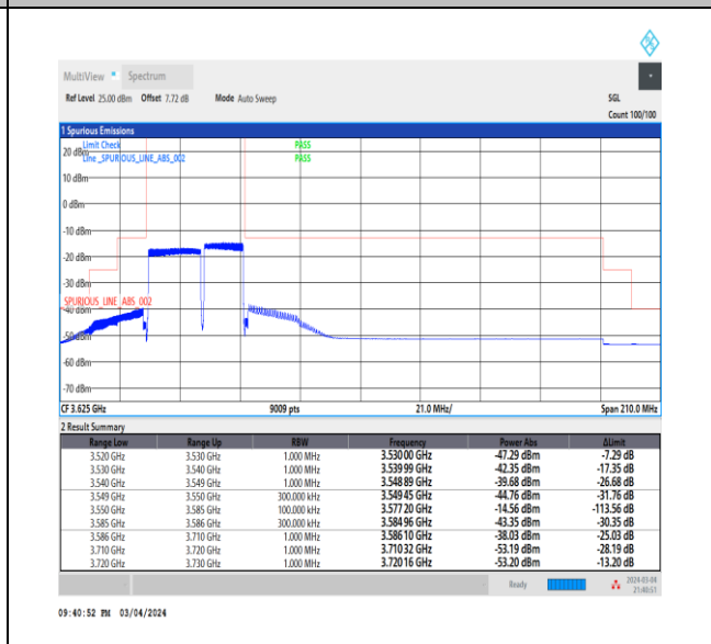
NTNV_CA_n48B_PC3_30+30_20+15_L+L_TID6_1_#1
