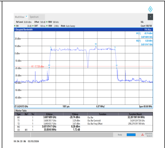
NTNV_CA_n48B_PC3_30+30_20+15_M+M_Ant0_TID3_1_#1
