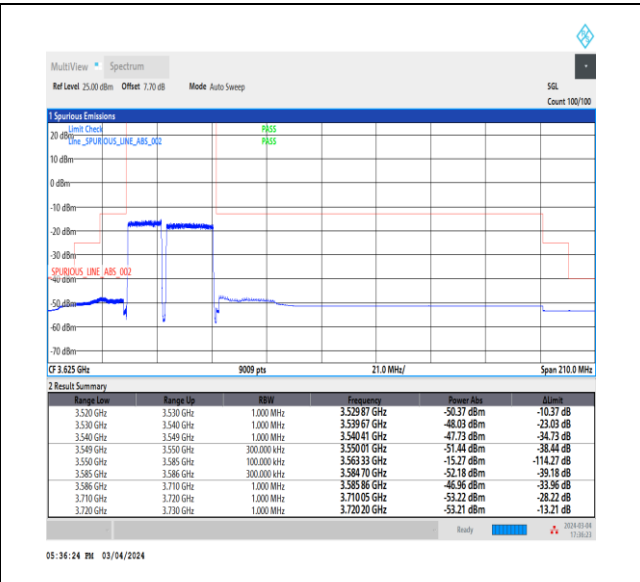
NTNV_CA_n48B_PC3_30+30_15+20_L+L_TID3_1_#1
