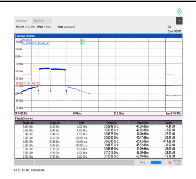
NTNV_CA_n48B_PC3_30+30_15+20_L+L_TID6_1_#1
