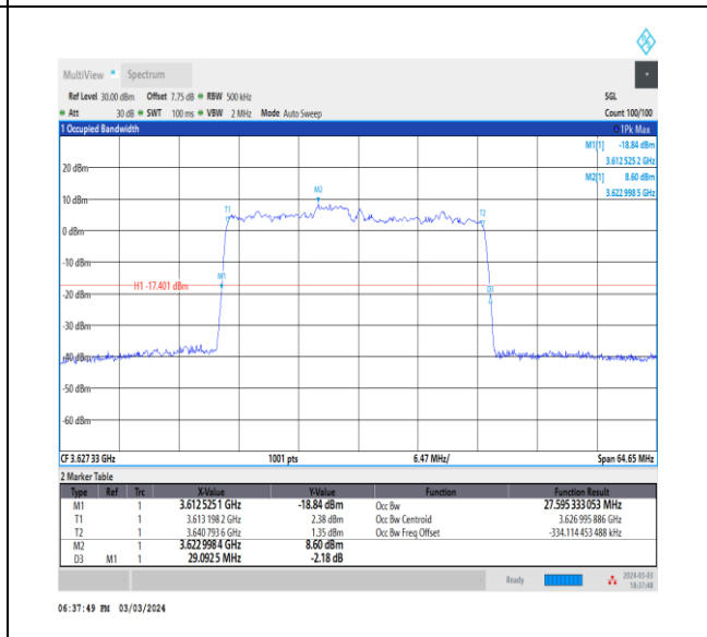
NTNV_CA_n48B_PC3_30+30_15+20_M+M_Ant0_TID3_1_#1
