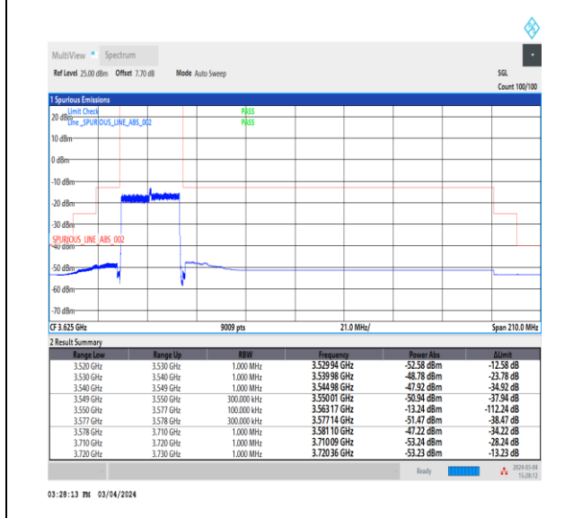
NTNV_CA_n48B_PC3_30+30_15+15_L+L_TID3_1_#1
