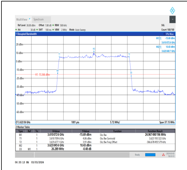
NTNV_CA_n48B_PC3_30+30_15+15_M+M_Ant0_TID1_1_#1
