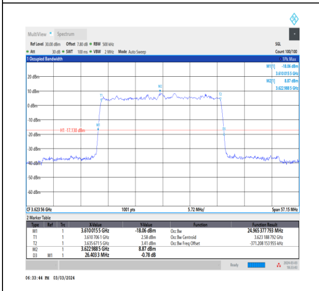
NTNV_CA_n48B_PC3_30+30_15+15_M+M_Ant0_TID3_1_#1
