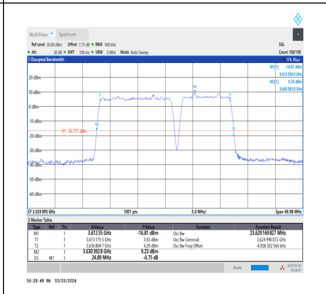
NTNV_CA_n48B_PC3_30+30_15+10_M+M_Ant0_TID5_1_#1
