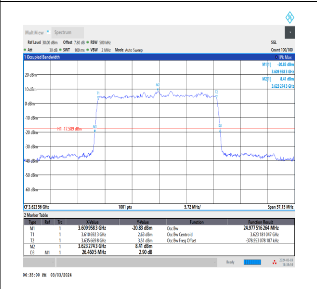
NTNV_CA_n48B_PC3_30+30_15+15_M+M_Ant0_TID8_1_#1
