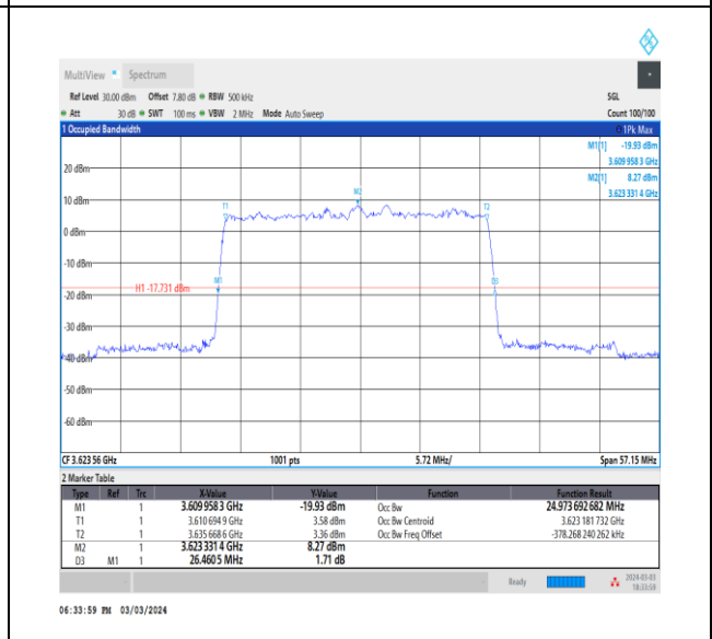
NTNV_CA_n48B_PC3_30+30_15+15_M+M_Ant0_TID4_1_#1
