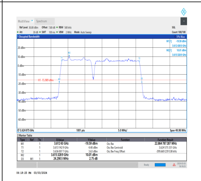
NTNV_CA_n48B_PC3_30+30_10+15_M+M_Ant0_TID3_1_#1
