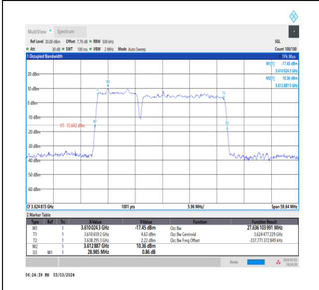
NTNV_CA_n48B_PC3_30+30_10+20_M+M_Ant0_TID5_1_#1
