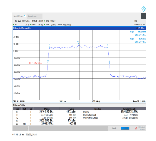
NTNV_CA_n48B_PC3_30+30_15+15_M+M_Ant0_TID5_1_#1
