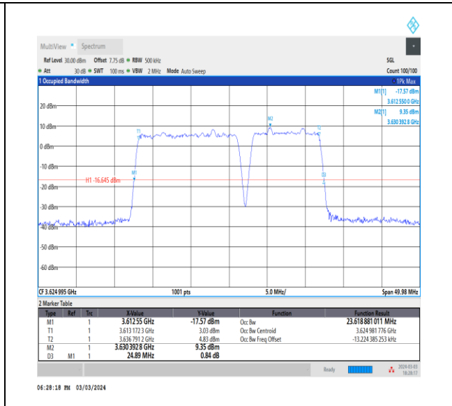
NTNV_CA_n48B_PC3_30+30_15+10_M+M_Ant0_TID3_1_#1
