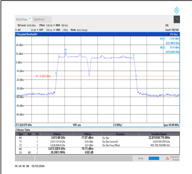
NTNV_CA_n48B_PC3_30+30_10+15_M+M_Ant0_TID4_1_#1
