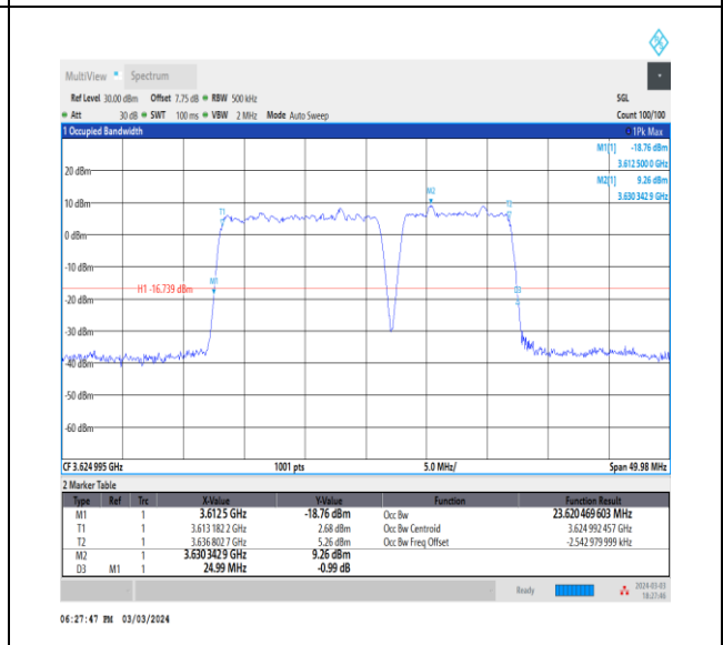
NTNV_CA_n48B_PC3_30+30_15+10_M+M_Ant0_TID1_1_#1
