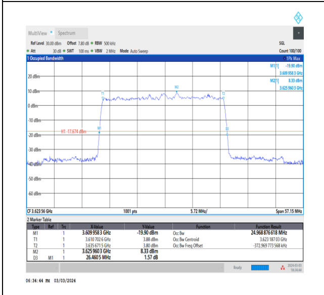
NTNV_CA_n48B_PC3_30+30_15+15_M+M_Ant0_TID7_1_#1
