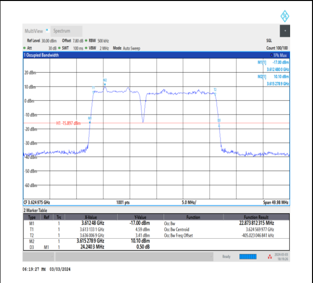
NTNV_CA_n48B_PC3_30+30_10+15_M+M_Ant0_TID7_1_#1
