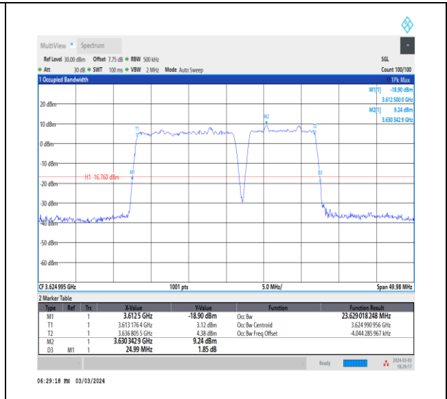
NTNV_CA_n48B_PC3_30+30_15+10_M+M_Ant0_TID7_1_#1
