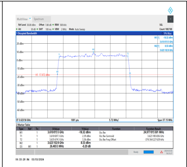
NTNV_CA_n48B_PC3_30+30_15+15_M+M_Ant0_TID2_1_#1
