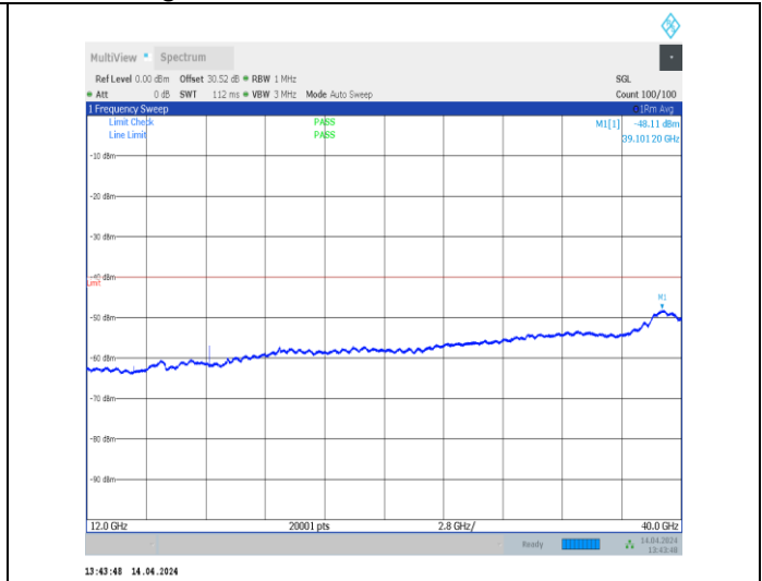
1-N48-PC3-30-40-L-1-DFT-PI2BPSK-Inner_1RB_Left-1 @1-12000-40000-Ant0-12000.00--48.12--40-PASS
