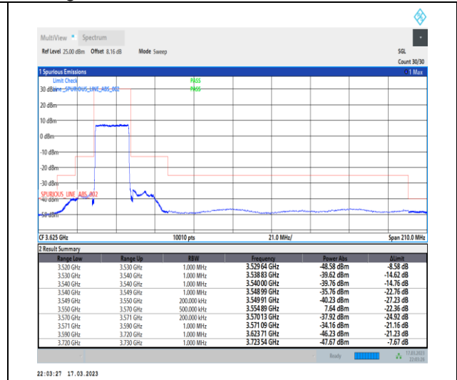
1-N48-PC3-30-20-L-3-DFT-PI2BPSK-Outer_Full-50@0-Ant0-1--PASS-see graph
