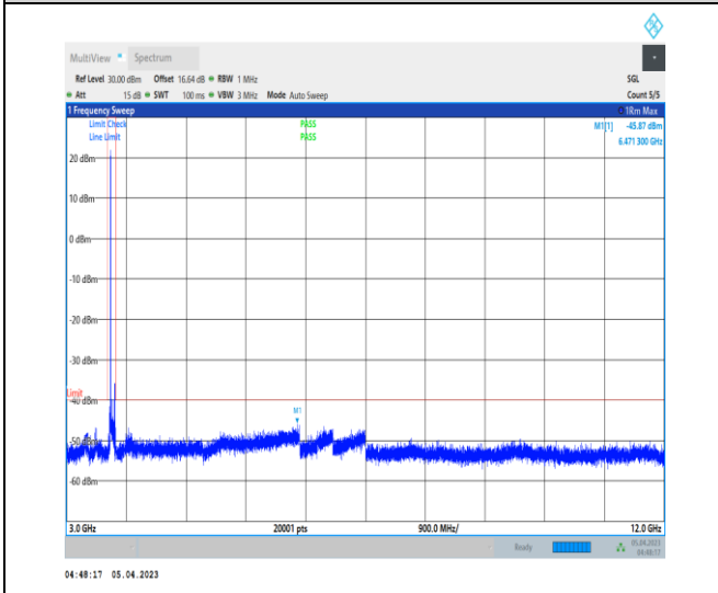
1-N48-PC3-30-40-H-1-DFT-PI2BPSK-Inner_1RB_Le ft-1@1-3000-12000-Ant0-3368.55--45.87--40-PASS
