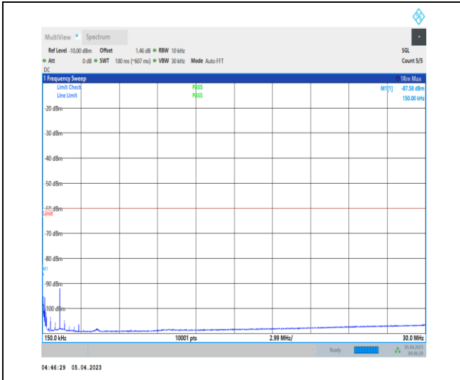
1-N48-PC3-30-40-M-1-DFT-PI2BPSK-Inner_1RB_Le ft-1@1-0.15-30-Ant0-0.15--87.58--60-PASS
