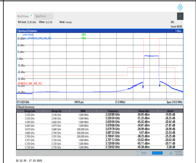
1-N48-PC3-30-20-H-6-CP-QPSK-Outer_Full-51@0-Ant0-1--PASS-see graph
