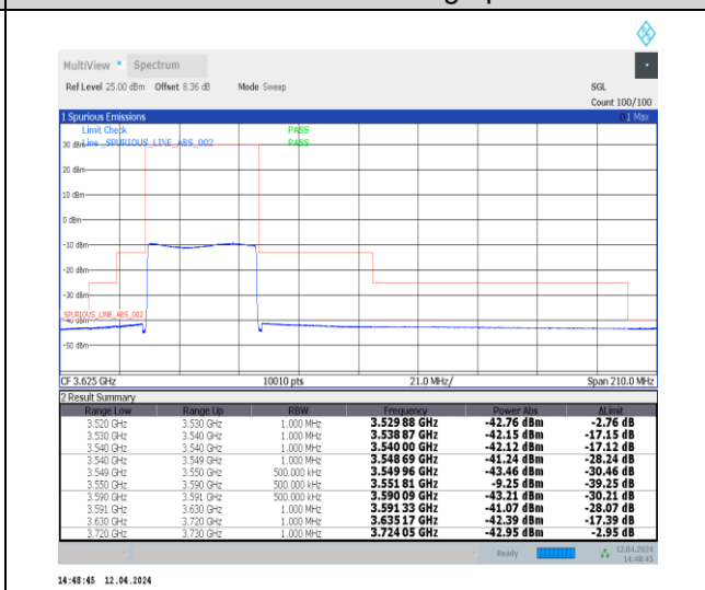
1-N48-30-40-L-6-CP-QPSK-Outer_Full-106@0-Ant0-1--PASS-see graph
