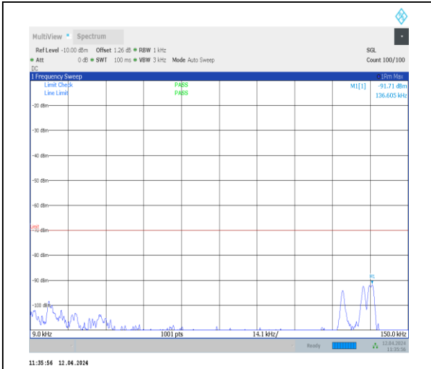
1-N48-30-40-H-1-DFT-QPSK-Edge_1RB_Left-1@ 0-0.009-0.15-Ant0-0.02--91.71--70-PASS
