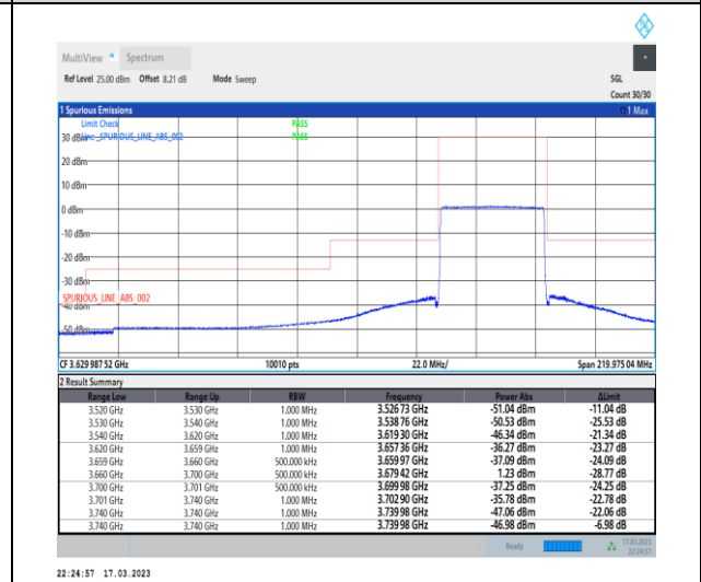
1-N48-PC3-30-40-H-6-CP-QPSK-Outer_Full-106 @0-Ant0-1--PASS-see graph
