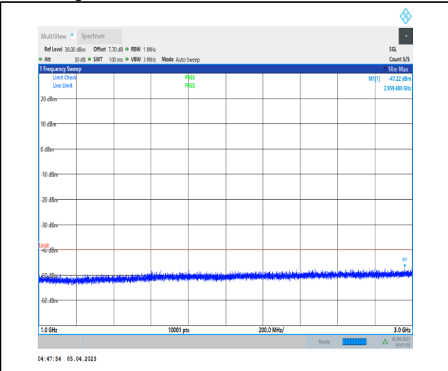
1-N48-PC3-30-40-H-1-DFT-PI2BPSK-Inner_1RB_Le ft-1@1-1000-3000-Ant0-2996.80--47.22--40-PASS
