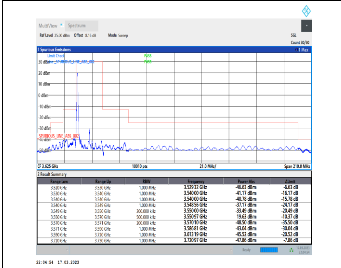
1-N48-PC3-30-20-L-4-CP-QPSK-Edge_1RB_Left-1@0-Ant0-1--PASS-see graph
