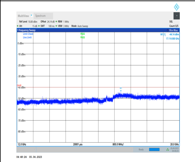
1-N48-PC3-30-40-H-1-DFT-PI2BPSK-Inner_1RB_Le ft-1@1-12000-20000-Ant0-17080.40--44.14--40-PASS
