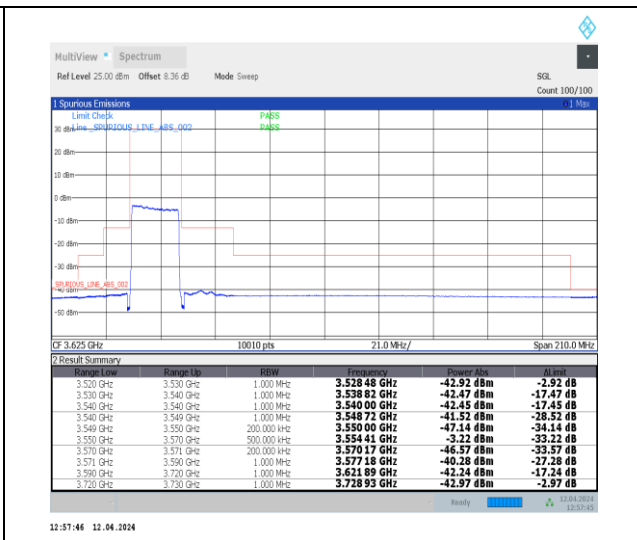
1-N48-30-20-L-3-DFT-PI2BPSK-Outer_Full-50@0-Ant0-1--PASS-see graph
