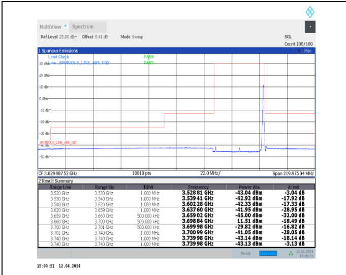
1-N48-30-40-H-2-DFT-PI2BPSK-Edge_1RB_Right-1@105-Ant0-1--PASS-see graph
