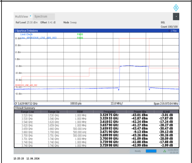
1-N48-30-40-H-6-CP-QPSK-Outer_Full-106@0-Ant0-1--PASS-see graph
