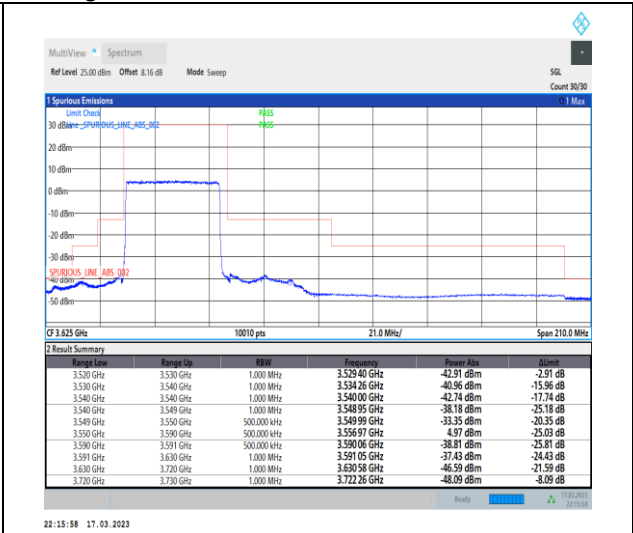
1-N48-PC3-30-40-L-3-DFT-PI2BPSK-Outer_Full-100@0-Ant0-1--PASS-see graph
