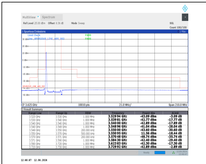
1-N48-30-20-L-1-DFT-PI2BPSK-Edge_1RB_Left-1@0-Ant0-1--PASS-see graph
