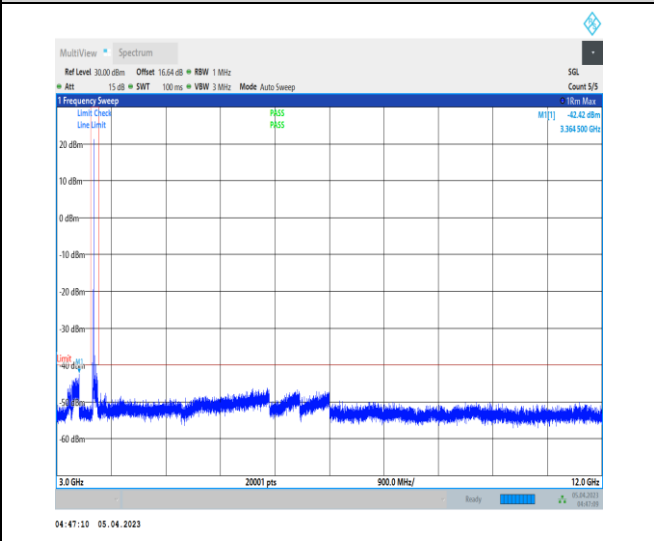
1-N48-PC3-30-40-M-1-DFT-PI2BPSK-Inner_1RB_Le ft-1@1-3000-12000-Ant0-3322.20--42.42--40-PASS
