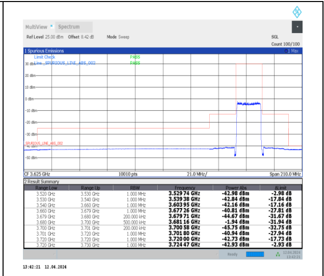
1-N48-30-20-H-3-DFT-PI2BPSK-Outer_Full-50@0-Ant0-1--PASS-see graph
