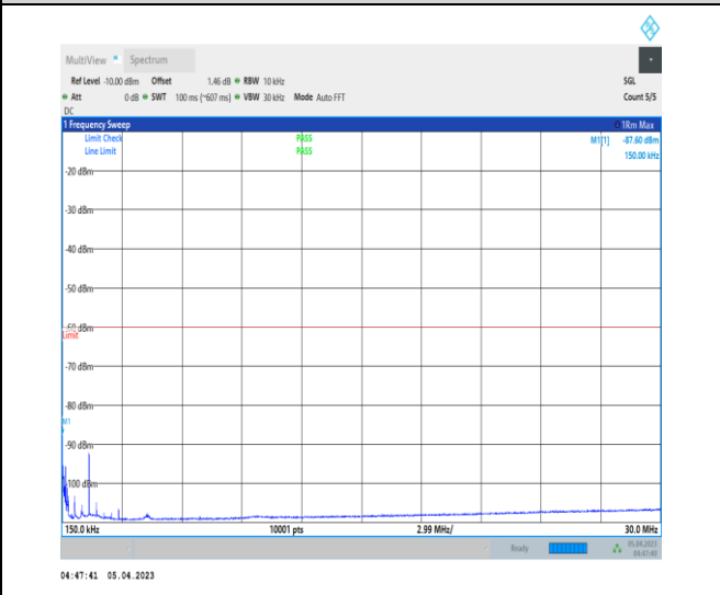
1-N48-PC3-30-40-H-1-DFT-PI2BPSK-Inner_1RB_Le ft-1@1-0.15-30-Ant0-0.15--87.60--60-PASS
