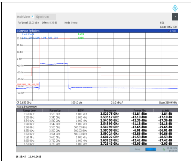
1-N48-30-40-L-3-DFT-PI2BPSK-Outer_Full-100@0-Ant0-1--PASS-see graph
