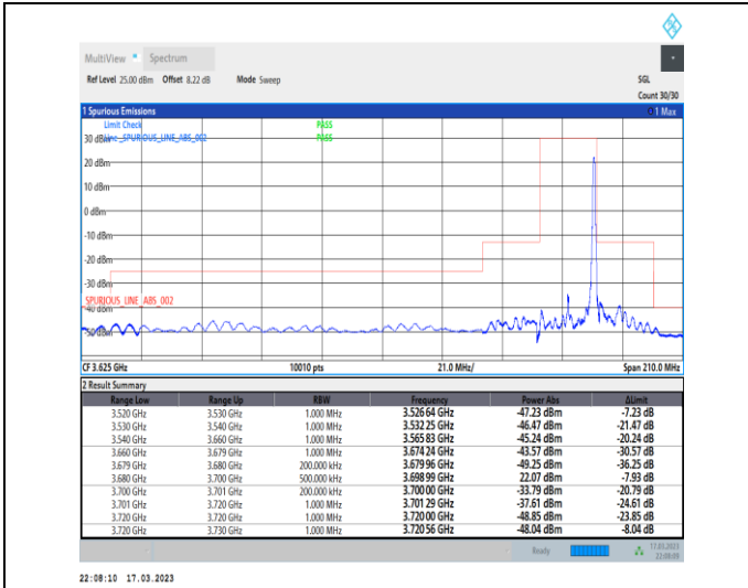
1-N48-PC3-30-20-H-2-DFT-PI2BPSK-Edge_1RB_Right-t-1@50-Ant0-1--PASS-see graph
