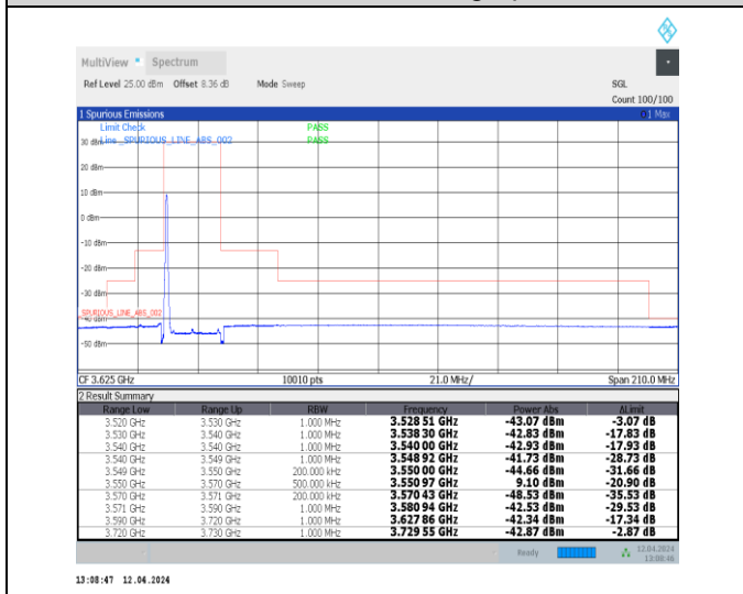
1-N48-30-20-L-4-CP-QPSK-Edge_1RB_Left-1@0-Ant0-1--PASS-see graph
