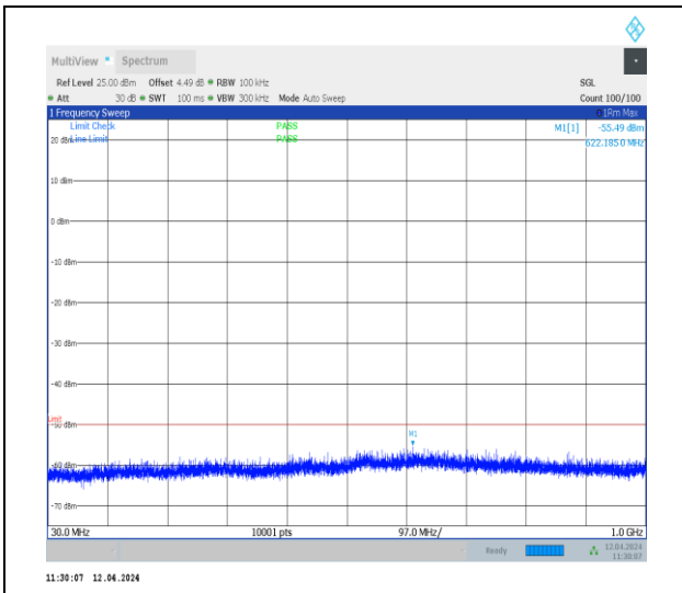
1-N48-30-40-M-1-DFT-QPSK-Edge_1RB_Left-1@ 0-30-1000-Ant0-33.88--55.49--50-PASS
