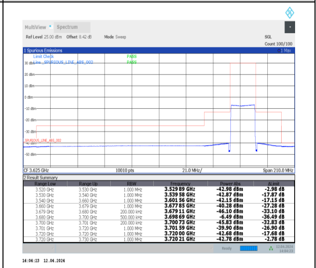
1-N48-30-20-H-6-CP-QPSK-Outer_Full-51@0-Ant0-1--PASS-see graph
