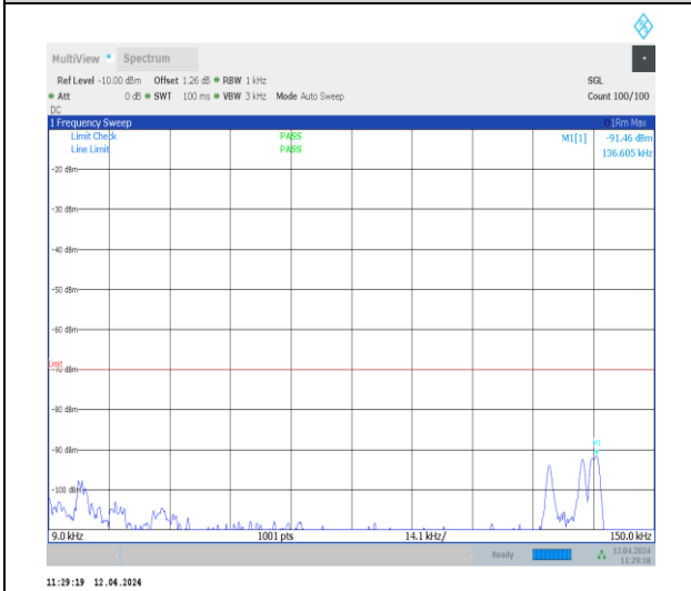
1-N48-30-40-M-1-DFT-QPSK-Edge_1RB_Left-1@ 0-0.009-0.15-Ant0-0.02--91.46--70-PASS
