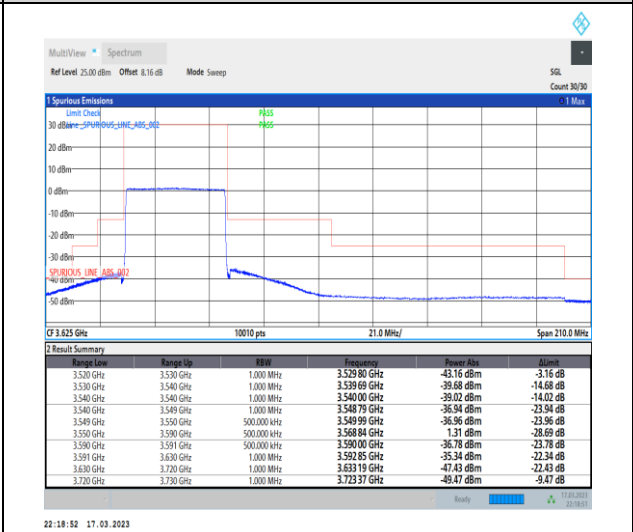
1-N48-PC3-30-40-L-6-CP-QPSK-Outer_Full-106@0-Ant0-1--PASS-see graph
