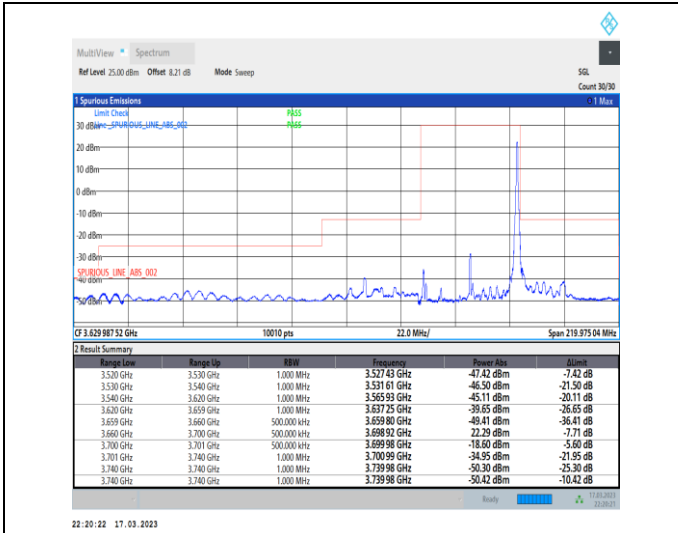
1-N48-PC3-30-40-H-2-DFT-PI2BPSK-Edge_1RB_Righ t-1@105-Ant0-1--PASS-see graph
