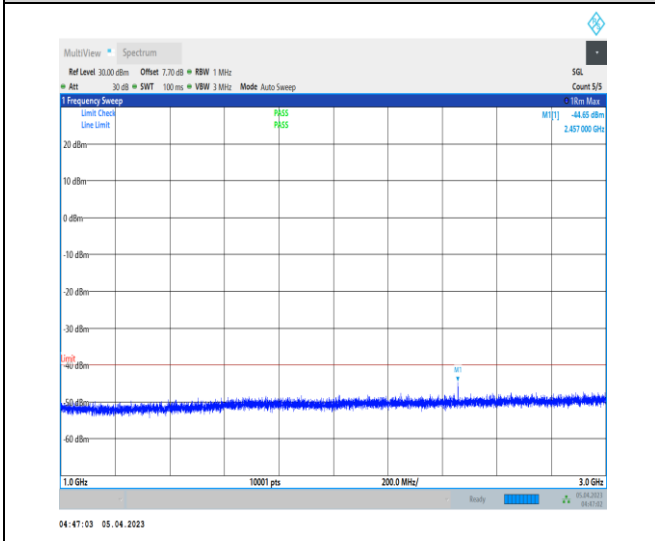
1-N48-PC3-30-40-M-1-DFT-PI2BPSK-Inner_1RB_Le ft-1@1-1000-3000-Ant0-2634.20--44.65--40-PASS
