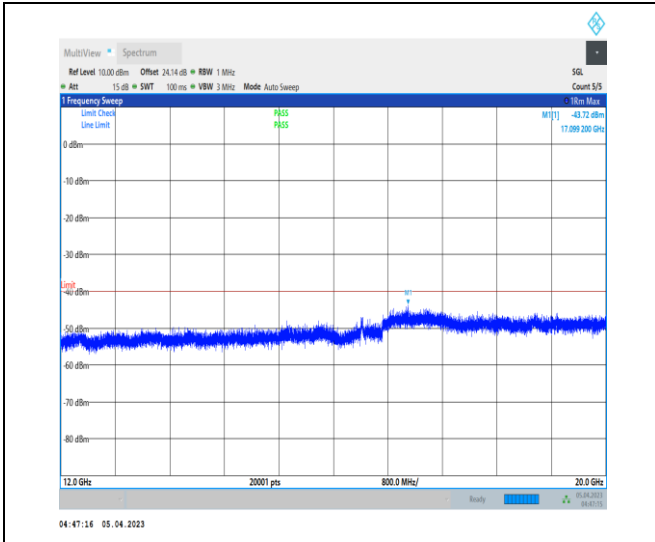
1-N48-PC3-30-40-M-1-DFT-PI2BPSK-Inner_1RB_Le ft-1@1-12000-20000-Ant0-17286.80--43.72--40-PASS S
