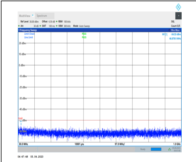
1-N48-PC3-30-40-H-1-DFT-PI2BPSK-Inner_1RB_Le ft-1@1-30-1000-Ant0-61.62--54.53--50-PASS
