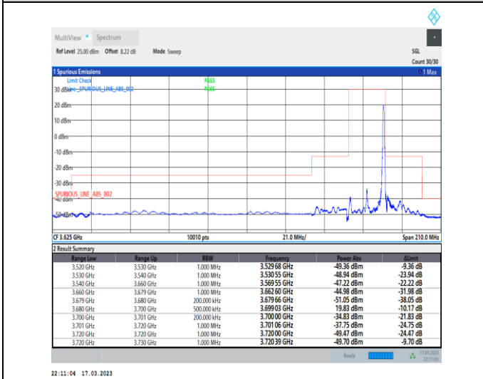
1-N48-PC3-30-20-H-5-CP-QPSK-Edge_1RB_Right-1@50-Ant0-1--PASS-see graph
