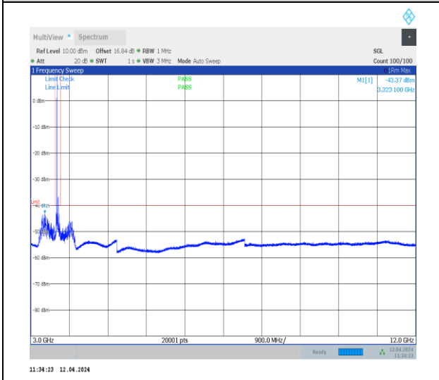
1-N48-30-40-M-1-DFT-QPSK-Edge_1RB_Left-1@ 0-3000-12000-Ant0-3317.25--43.37--40-PASS
