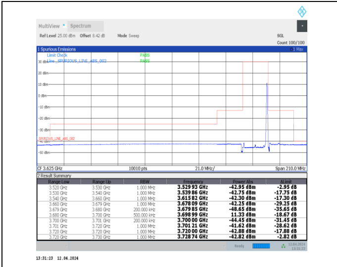
1-N48-30-20-H-2-DFT-PI2BPSK-Edge_1RB_Right-1@50-Ant0-1--PASS-see graph
