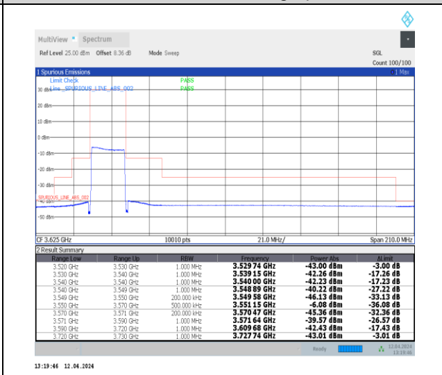
1-N48-30-20-L-6-CP-QPSK-Outer_Full-51@0-Ant0-1--PASS-see graph
