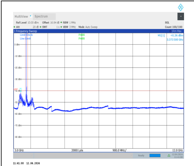
1-N48-30-40-H-1-DFT-QPSK-Edge_1RB_Left-1@ 0-3000-12000-Ant0-3373.95--41.36--40-PASS
