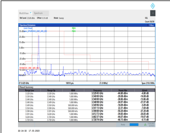
1-N48-PC3-30-40-L-1-DFT-PI2BPSK-Edge_1RB_Left-1@0-Ant0-1--PASS-see graph
