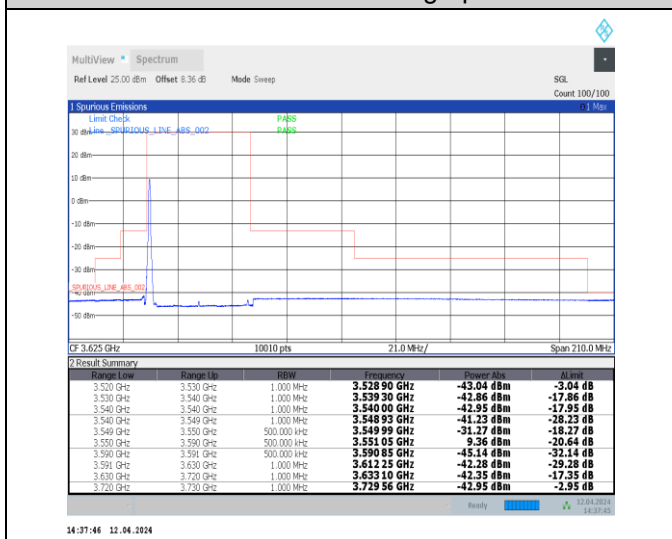
1-N48-30-40-L-4-CP-QPSK-Edge_1RB_Left-1@0-Ant0-1--PASS-see graph
