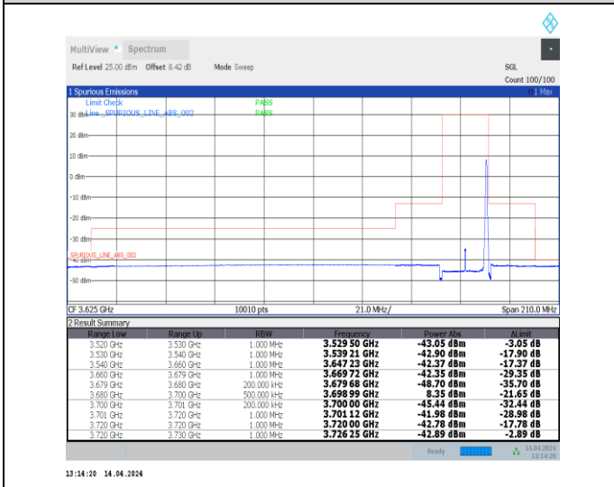
1-N48-30-20-H-5-CP-QPSK-Edge_1RB_Right-1@50-Ant0-1--PASS-see graph
