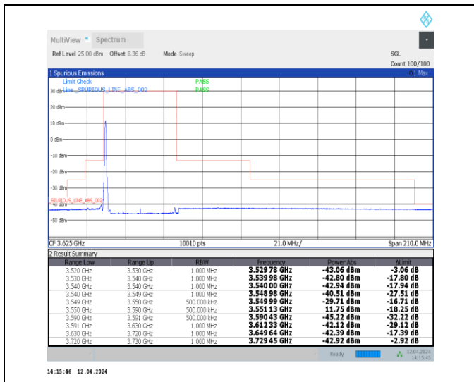
1-N48-30-40-L-1-DFT-PI2BPSK-Edge_1RB_Left-1@0 -Ant0-1--PASS-see graph
