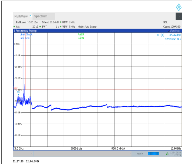
1-N48-30-40-L-1-DFT-QPSK-Edge_1RB_Left-1@ 0-3000-12000-Ant0-3359.10--45.26--40-PASS
