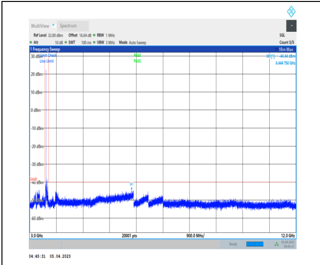
1-N48-PC3-30-40-L-1-DFT-PI2BPSK-Inner_1RB_Lef t-1@1-3000-12000-Ant0-3197.55--44.44--40-PASS
