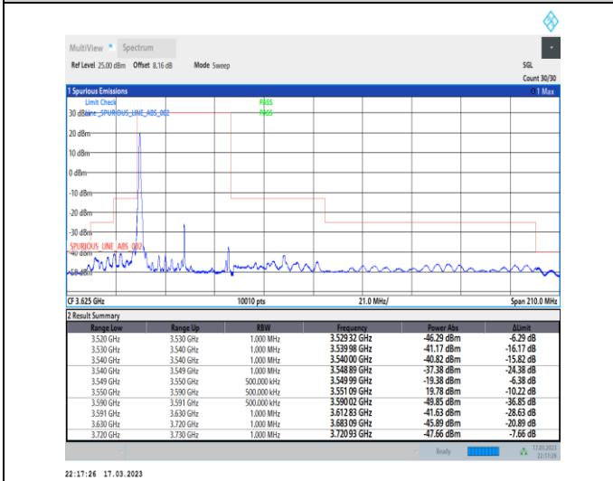
1-N48-PC3-30-40-L-4-CP-QPSK-Edge_1RB_Left-1@0-Ant0-1--PASS-see graph
