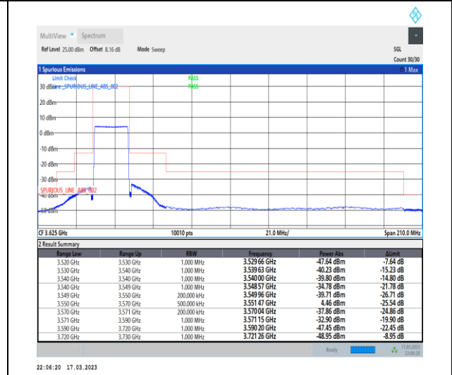
1-N48-PC3-30-20-L-6-CP-QPSK-Outer_Full-51@0-Ant0-1--PASS-see graph
