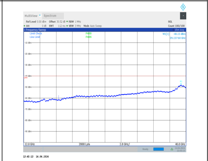
1-N48-PC3-30-40-M-1-DFT-PI2BPSK-Inner_1RB_Left- 1@1-12000-40000-Ant0-12000.00--48.12--40-PASS
