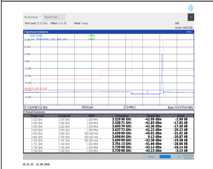
1-N48-30-40-H-5-CP-QPSK-Edge_1RB_Right-1@105-Ant0-1--PASS-see graph
