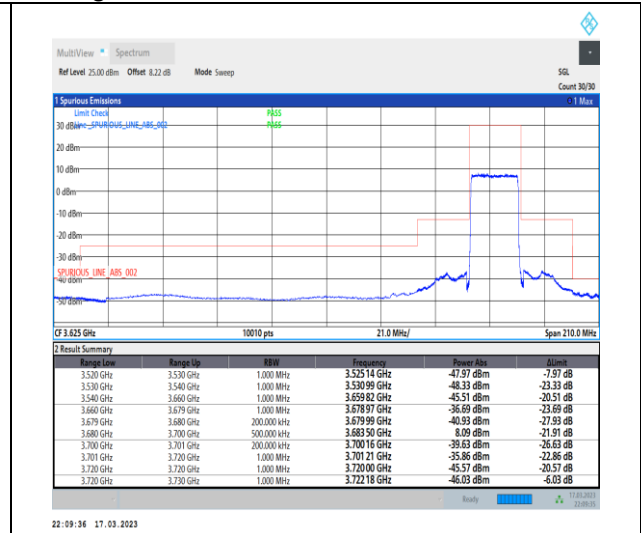
1-N48-PC3-30-20-H-3-DFT-PI2BPSK-Outer_Full-50@0-Ant0-1--PASS-see graph
