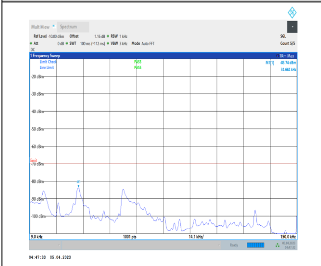
1-N48-PC3-30-40-H-1-DFT-PI2BPSK-Inner_1RB_Le ft-1@1-0.009-0.15-Ant0-0.06--83.74--70-PASS
