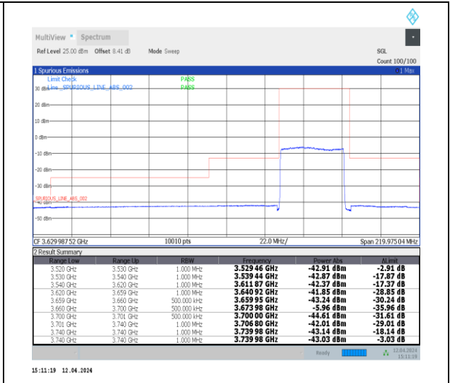
1-N48-30-40-H-3-DFT-PI2BPSK-Outer_Full-100@0-Ant0-1--PASS-see graph
