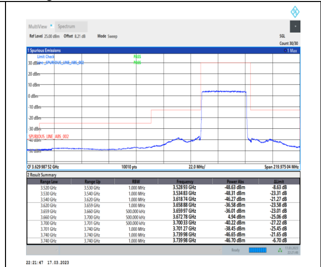
1-N48-PC3-30-40-H-3-DFT-PI2BPSK-Outer_Full-1 00@0-Ant0-1--PASS-see graph
