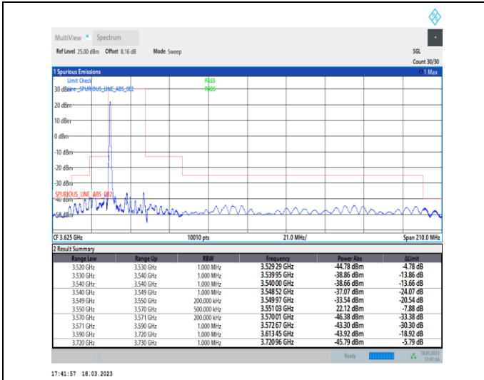
1-N48-PC3-30-20-L-1-DFT-PI2BPSK-Edge_1RB_Left-1@0-Ant0-1--PASS-see graph
