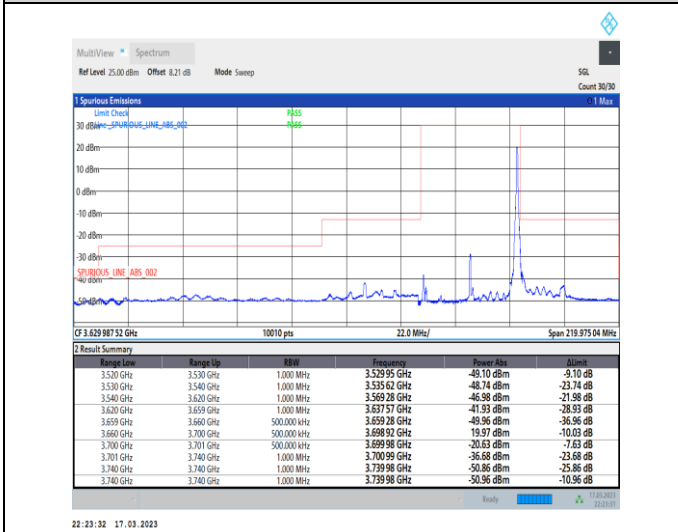
1-N48-PC3-30-40-H-5-CP-QPSK-Edge_1RB_Righ t-1@105-Ant0-1--PASS-see graph
