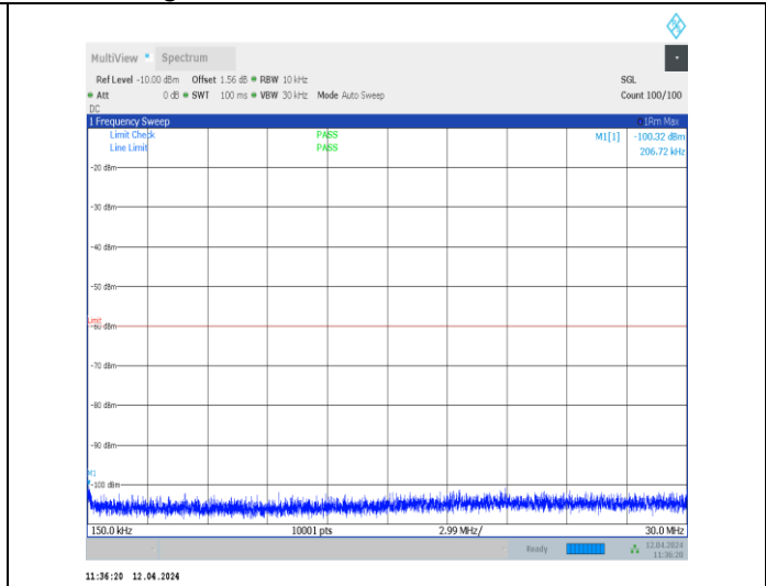
1-N48-30-40-H-1-DFT-QPSK-Edge_1RB_Left-1@0-0.1 5-30-Ant0-29.97--100.32--60-PASS
