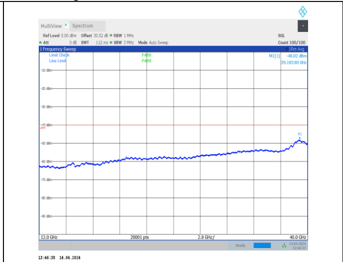
1-N48-PC3-30-40-H-1-DFT-PI2BPSK-Inner_1RB_Left-1@ 1-12000-40000-Ant0-12000.00--48.00--40-PASS
