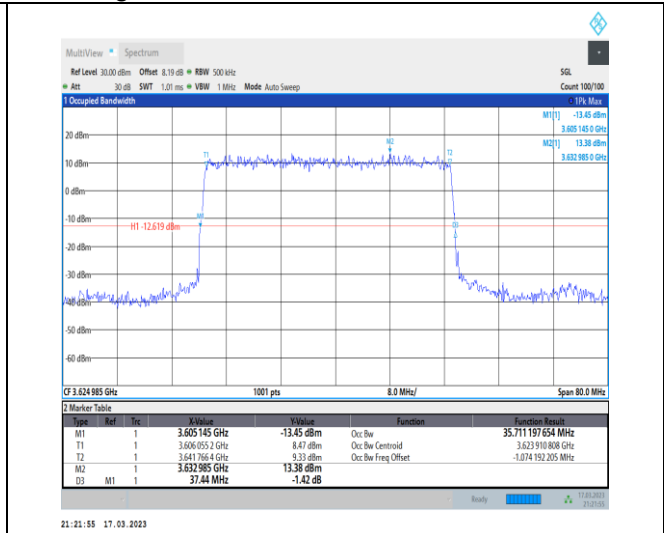
1-N48-PC3-30-40-M-2-DFT-PI2BPSK-Outer_Full-100@0-Ant0-35.711-37.440-≤40-PASS
