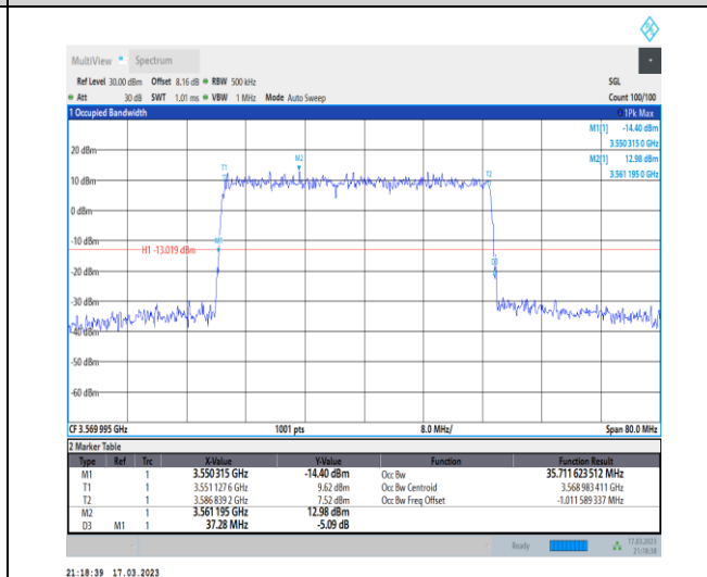
1-N48-PC3-30-40-L-1-DFT-QPSK-Outer_Full-100@0 -Ant0-35.712-37.280-≤40-PASS
