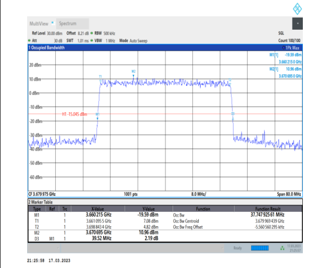
1-N48-PC3-30-40-H-7-CP-16QAM-Outer_Full-106@0 -Ant0-37.748-39.520-≤40-PASS
