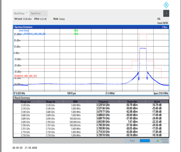
1-N48-PC3-30-10-H-6-CP-QPSK-Outer_Full-24@ 0-Ant0-1--PASS-see graph
