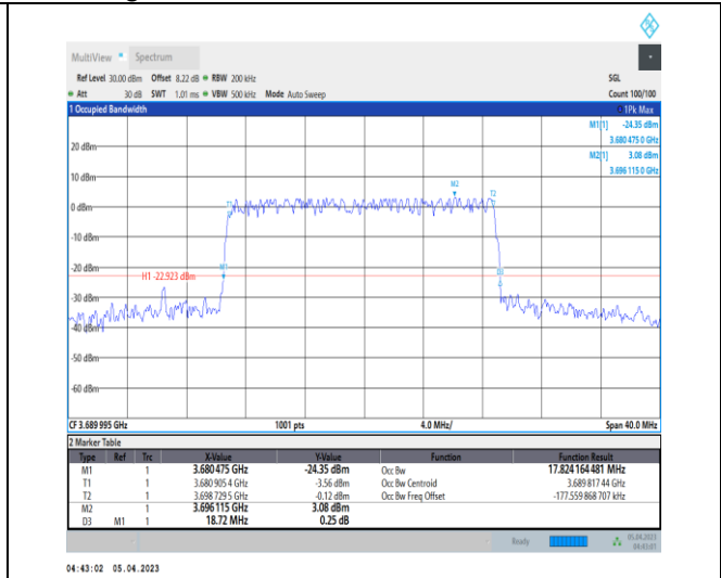
1-N48-PC3-30-20-H-4-DFT-64QAM-Outer_Full-50@ 0-Ant0-7.442-7.720-≤20-PASS
