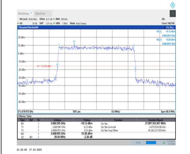
1-N48-PC3-30-40-H-6-CP-QPSK-Outer_Full-106@0 -Ant0-37.897-39.440-≤40-PASS
