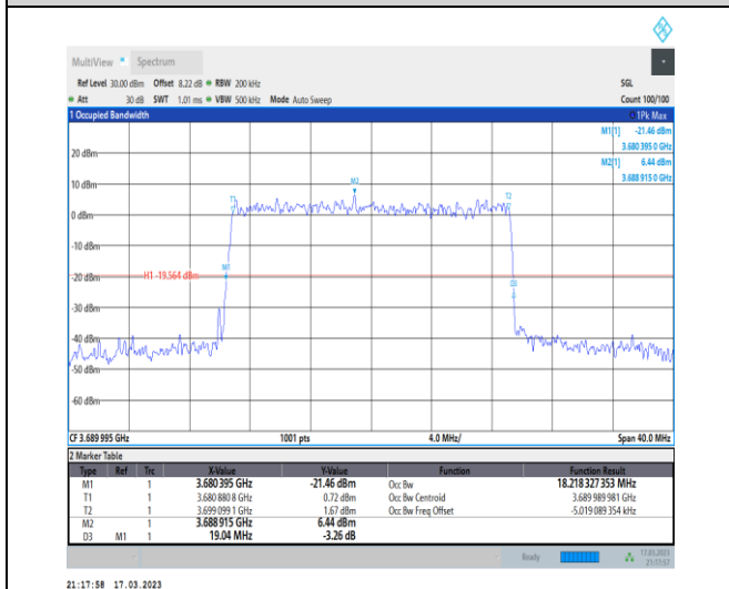
1-N48-PC3-30-20-H-9-CP-256QAM-Outer_Full-51@0 -Ant0-18.218-19.040-≤20-PASS
