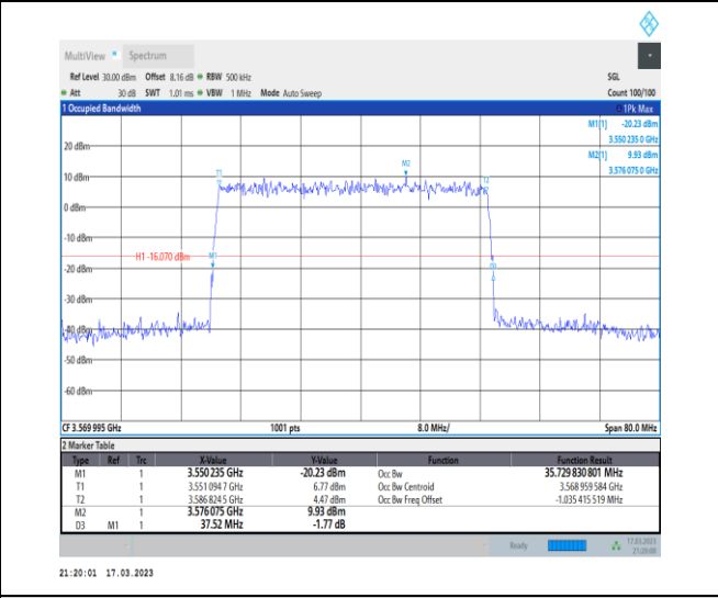
1-N48-PC3-30-40-L-5-DFT-256QAM-Outer_Full-100 @0-Ant0-35.73-37.520-≤40-PASS
