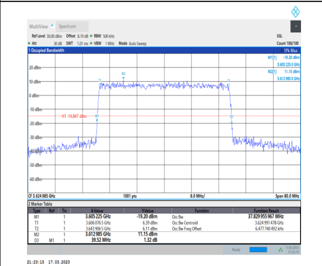
1-N48-PC3-30-40-M-8-CP-64QAM-Outer_Full-106@0-Ant0-37.83-39.520-≤40-PASS
