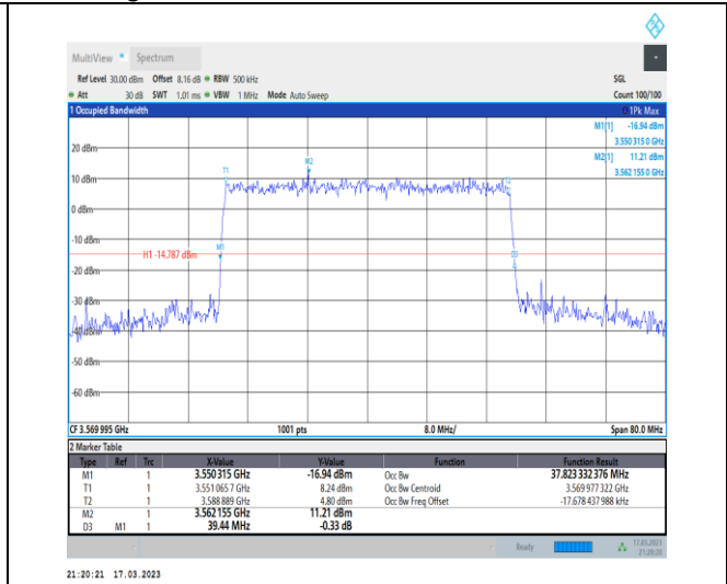
1-N48-PC3-30-40-L-7-CP-16QAM-Outer_Full-106@0-Ant0-37.823-39.440-≤40-PASS
