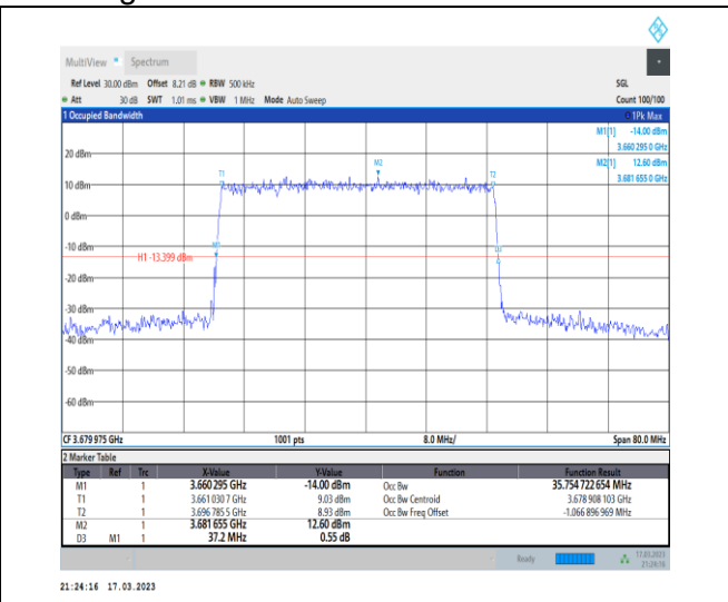
1-N48-PC3-30-40-H-1-DFT-QPSK-Outer_Full-100 @0-Ant0-35.755-37.200-≤40-PASS
