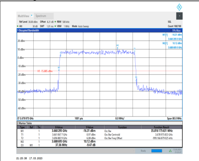
1-N48-PC3-30-40-H-5-DFT-256QAM-Outer_Full-100 @0-Ant0-35.816-37.360-≤40-PASS
