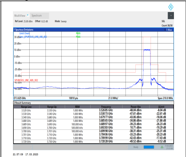
1-N48-PC3-30-10-H-3-DFT-PI2BPSK-Outer_Full-2 4@0-Ant0-1--PASS-see graph
