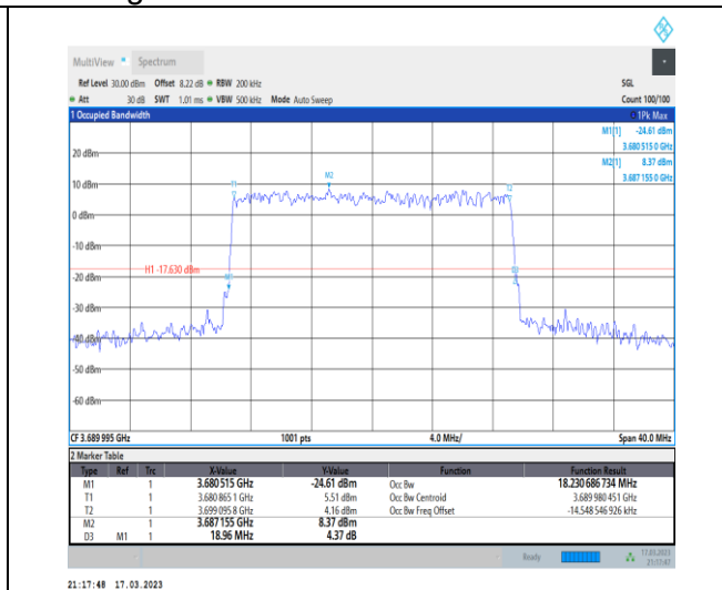
1-N48-PC3-30-20-H-8-CP-64QAM-Outer_Full-51@0 -Ant0-18.231-18.960-≤20-PASS
