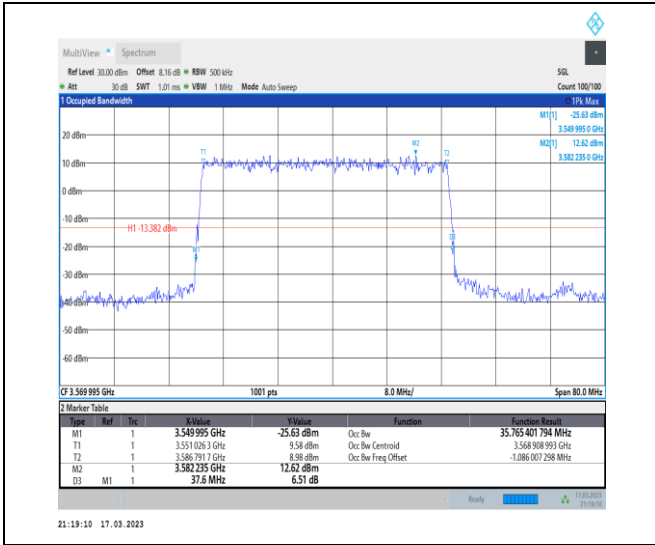
1-N48-PC3-30-40-L-2-DFT-PI2BPSK-Outer_Full-100 @0-Ant0-35.765-37.600-≤40-PASS
