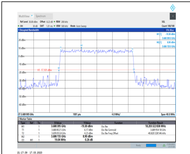
1-N48-PC3-30-20-H-7-CP-16QAM-Outer_Full-51@0 -Ant0-18.203-19.040-≤20-PASS
