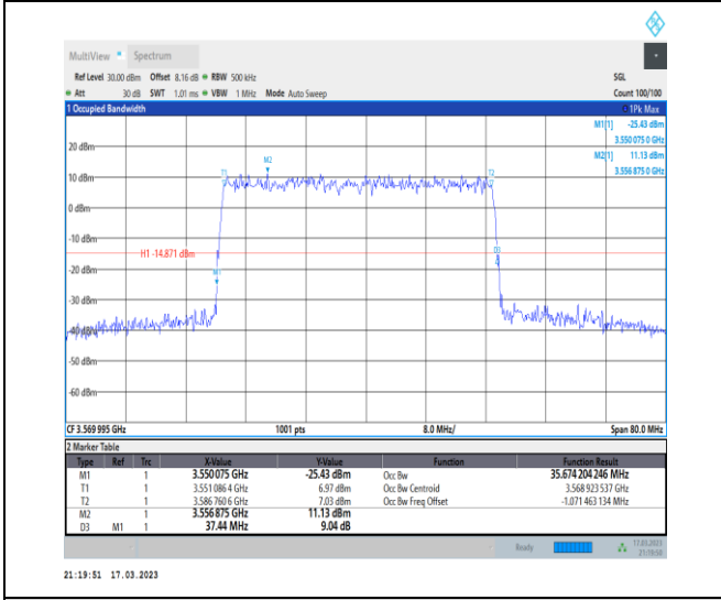
1-N48-PC3-30-40-L-4-DFT-64QAM-Outer_Full-100 @0-Ant0-35.674-37.440-≤40-PASS
