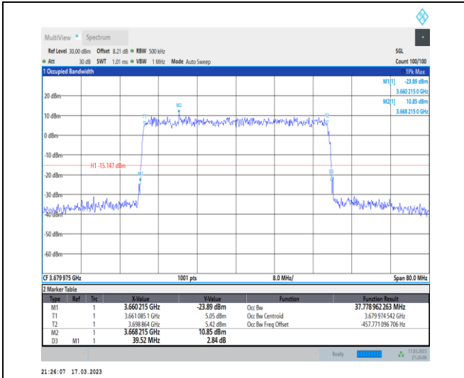
1-N48-PC3-30-40-H-8-CP-64QAM-Outer_Full-106@ 0-Ant0-37.779-39.520-≤40-PASS
