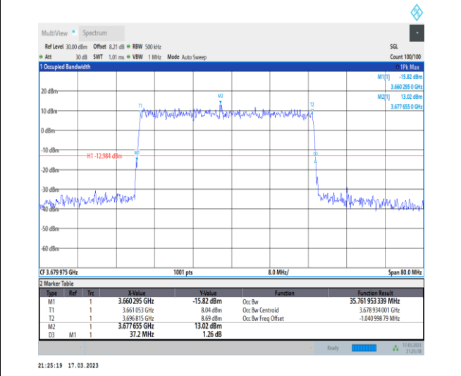
1-N48-PC3-30-40-H-3-DFT-16QAM-Outer_Full-100 @0-Ant0-35.762-37.200-≤40-PASS
