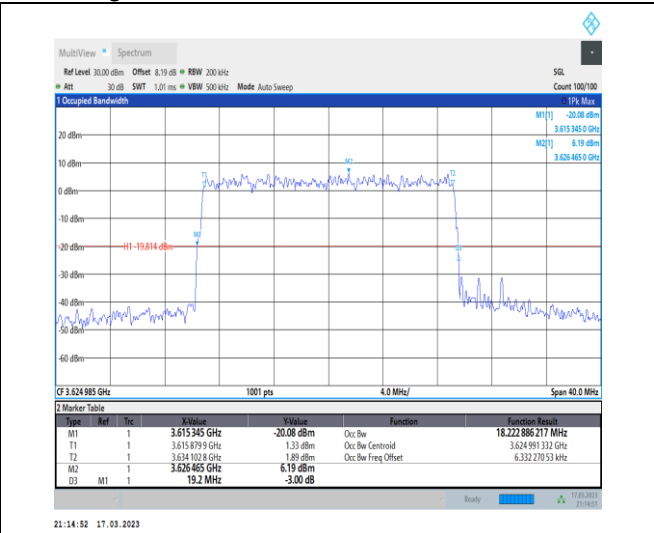
1-N48-PC3-30-20-M-9-CP-256QAM-Outer_Full-51@0 -Ant0-18.223-19.200-≤20-PASS
