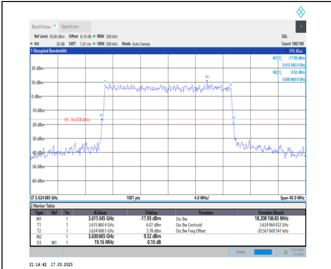
1-N48-PC3-30-20-M-8-CP-64QAM-Outer_Full-51@0 -Ant0-18.208-19.160-≤20-PASS
