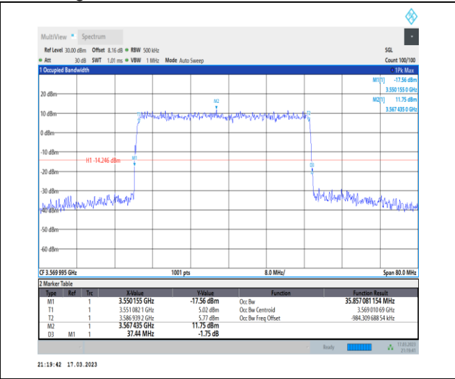
1-N48-PC3-30-40-L-3-DFT-16QAM-Outer_Full-100 @0-Ant0-35.857-37.440-≤40-PASS
