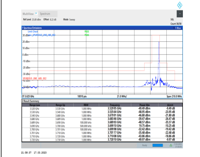
1-N48-PC3-30-10-H-5-CP-QPSK-Edge_1RB_Righ t-1@23-Ant0-1--PASS-see graph
