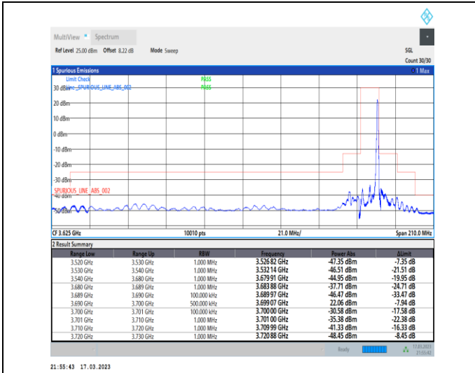
1-N48-PC3-30-10-H-2-DFT-PI2BPSK-Edge_1RB_Righ t-1@23-Ant0-1--PASS-see graph
