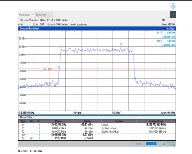
1-N48-PC3-30-20-H-6-CP-QPSK-Outer_Full-51@0- Ant0-18.2-19.120-≤20-PASS
