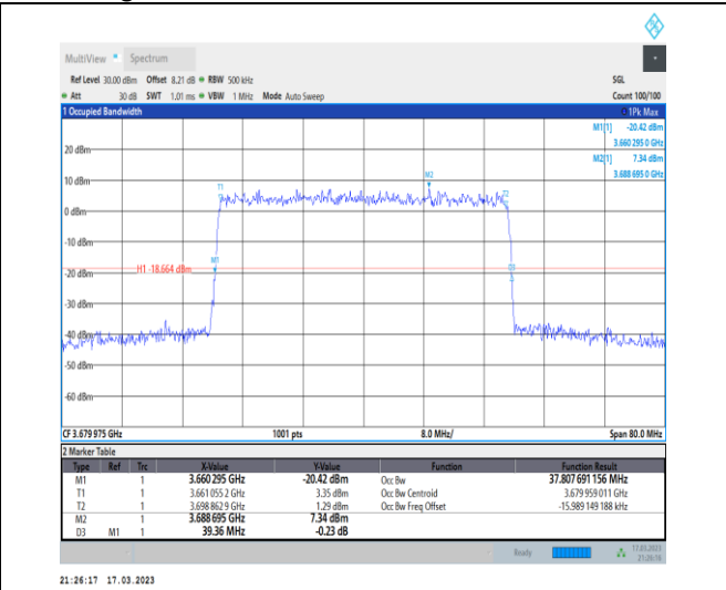
1-N48-PC3-30-40-H-9-CP-256QAM-Outer_Full-106 @0-Ant0-37.808-39.360-≤40-PASS
