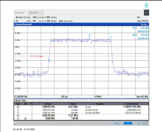
1-N48-PC3-30-20-H-2-DFT-PI2BPSK-Outer_Full-50 @0-Ant0-17.845-18.680-≤20-PASS
