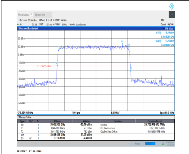
1-N48-PC3-30-40-M-3-DFT-16QAM-Outer_Full-100@0-Ant0-35.703-37.360-≤40-PASS
