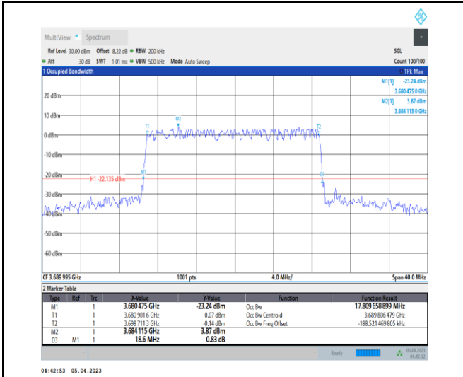
1-N48-PC3-30-20-H-3-DFT-16QAM-Outer_Full-50@ 0-Ant0-3.071-3.320-≤20-PASS
