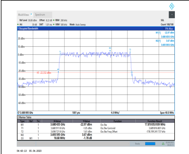
1-N48-PC3-30-20-H-5-DFT-256QAM-Outer_Full-50@ 0-Ant0-12.67-13.160-≤20-PASS
