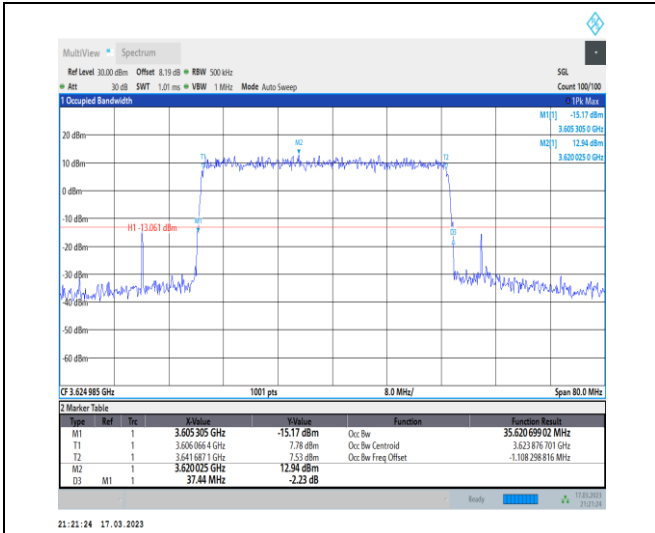
1-N48-PC3-30-40-M-1-DFT-QPSK-Outer_Full-100@0-Ant0-35.621-37.440-≤40-PASS
