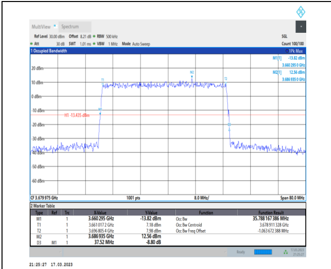
1-N48-PC3-30-40-H-4-DFT-64QAM-Outer_Full-100 @0-Ant0-35.788-37.520-≤40-PASS
