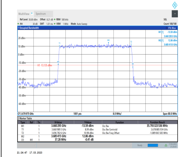
1-N48-PC3-30-40-H-2-DFT-PI2BPSK-Outer_Full-10 @0-Ant0-35.793-37.280-≤40-PASS
