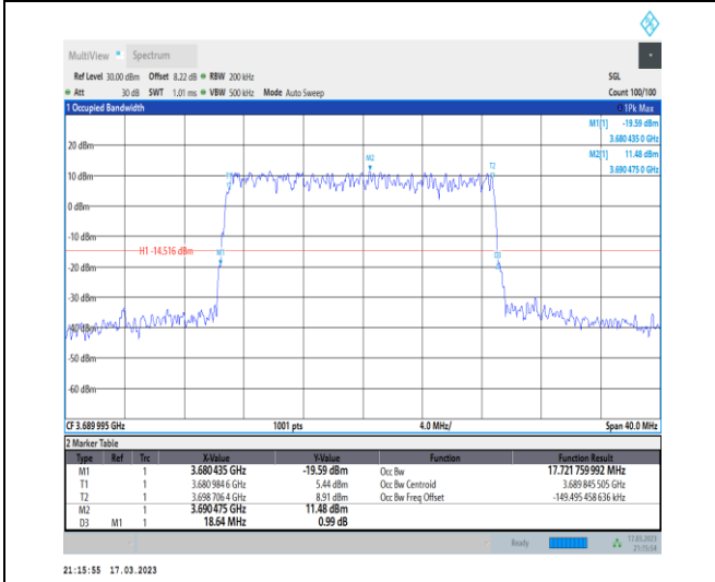
1-N48-PC3-30-20-H-1-DFT-QPSK-Outer_Full-50@0- Ant0-17.722-18.640-≤20-PASS
