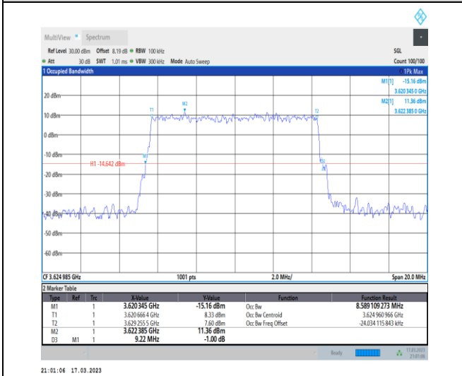
1-N48-PC3-30-10-M-2-DFT-PI2BPSK-Outer_Full-24 @0-Ant0-8.589-9.220-≤10-PASS
