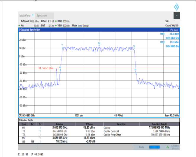
1-N48-PC3-30-20-M-1-DFT-QPSK-Outer_Full-50@ 0-Ant0-17.81-18.720-<=20-PASS
