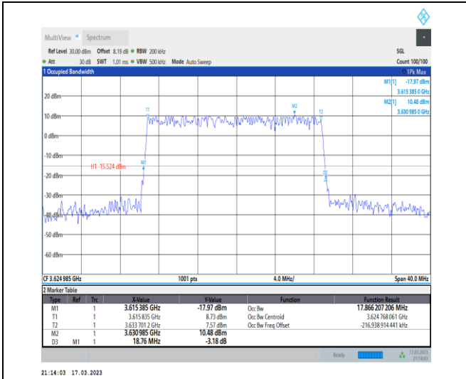
1-N48-PC3-30-20-M-4-DFT-64QAM-Outer_Full-50@ 0-Ant0-17.866-18.760-≤20-PASS
