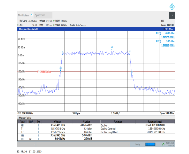
1-N48-PC3-30-10-L-9-CP-256QAM-Outer_Full-24@ 0-Ant0-8.556-9.040-≤10-PASS
