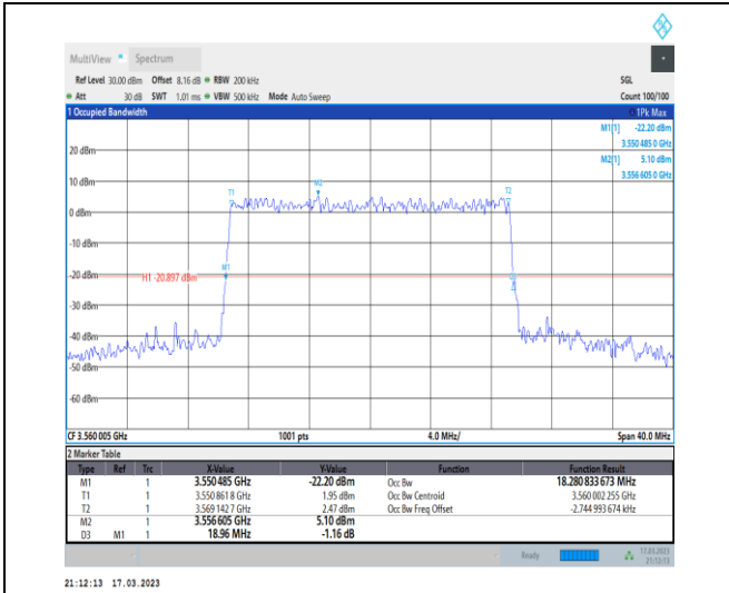
1-N48-PC3-30-20-L-9-CP-256QAM-Outer_Full-51@ 0-Ant0-18.281-18.960-<=20-PASS
