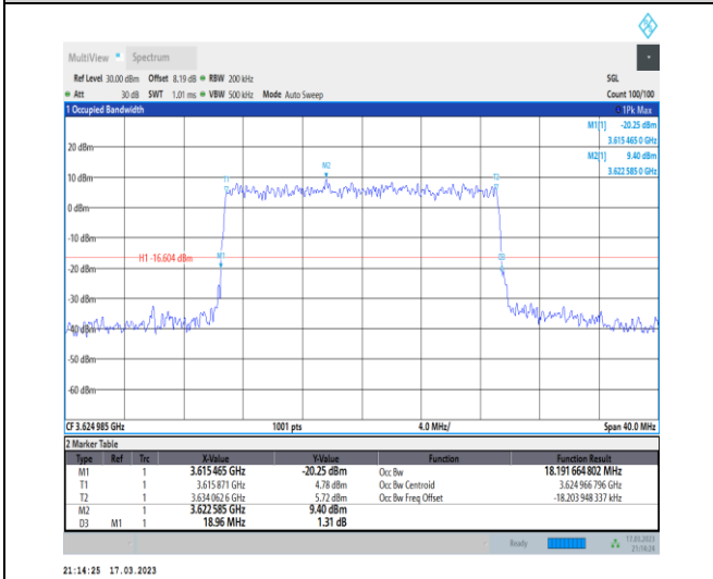
1-N48-PC3-30-20-M-6-CP-QPSK-Outer_Full-51@0- Ant0-18.192-18.960-≤20-PASS
