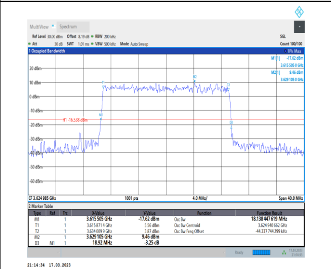
1-N48-PC3-30-20-M-7-CP-16QAM-Outer_Full-51@0 -Ant0-18.138-18.920-≤20-PASS
