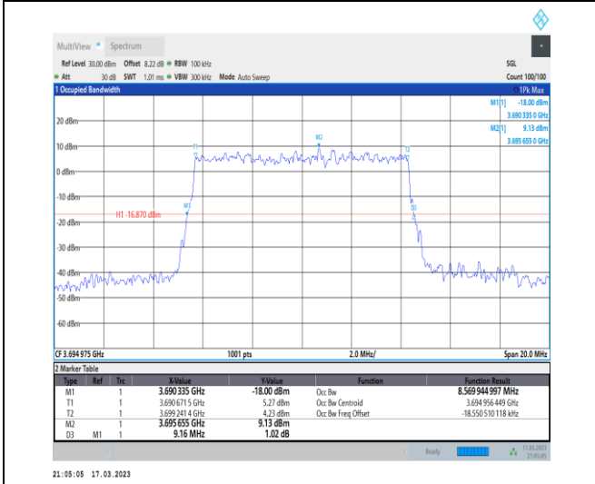
1-N48-PC3-30-10-H-5-DFT-256QAM-Outer_Full-24 @0-Ant0-8.57-9.160-≤10-PASS
