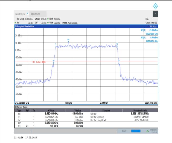
1-N48-PC3-30-10-M-5-DFT-256QAM-Outer_Full-24@0-Ant0-8.598-9.100-≤10-PASS
