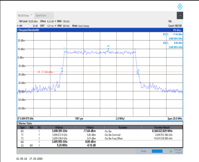
1-N48-PC3-30-10-H-6-CP-QPSK-Outer_Full-24@0- Ant0-8.566-9.240-≤10-PASS
