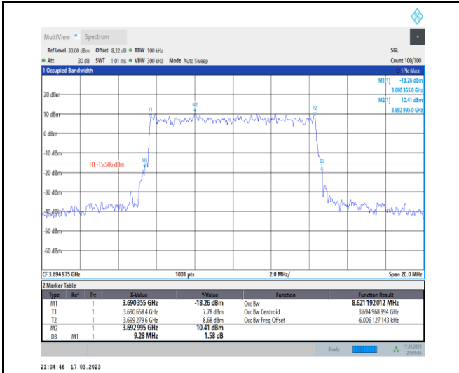
1-N48-PC3-30-10-H-3-DFT-16QAM-Outer_Full-24@ 0-Ant0-8.621-9.280-≤10-PASS
