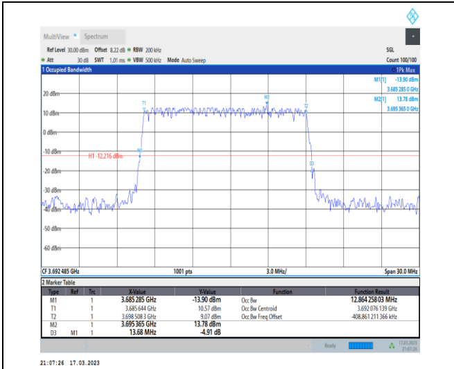
1-N48-PC3-30-15-H-2-DFT-PI2BPSK-Outer_Full-36@0-Ant0-12.864-13.680-≤15-PASS
