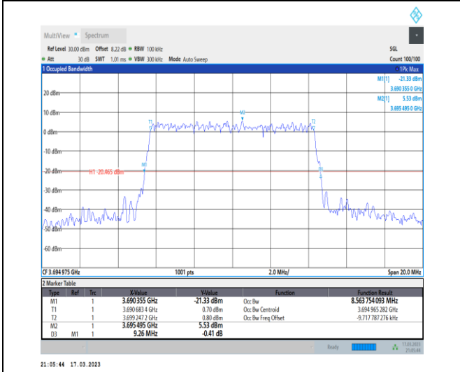
1-N48-PC3-30-10-H-9-CP-256QAM-Outer_Full-24@0 0-Ant0-8.564-9.260-≤10-PASS
