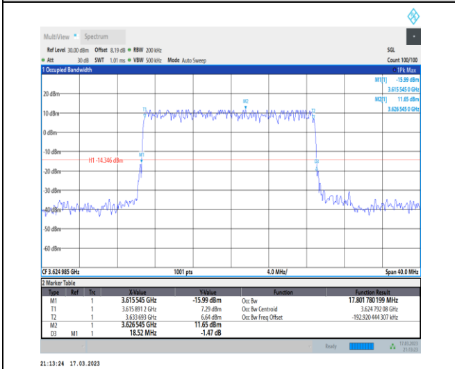
1-N48-PC3-30-20-M-2-DFT-PI2BPSK-Outer_Full-50 @0-Ant0-17.802-18.520-<=20-PASS
