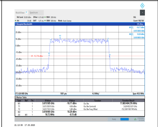
1-N48-PC3-30-20-M-3-DFT-16QAM-Outer_Full-50@ 0-Ant0-17.803-18.720-<=20-PASS
