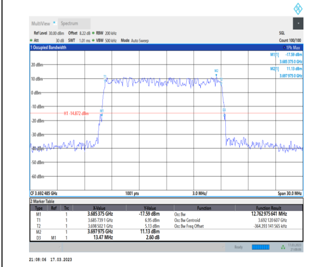
1-N48-PC3-30-15-H-4-DFT-64QAM-Outer_Full-36@0-Ant0-12.763-13.470-≤15-PASS
