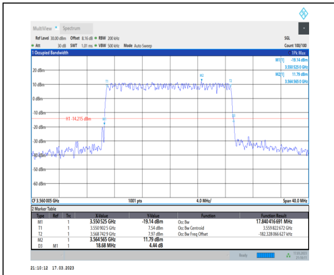
1-N48-PC3-30-20-L-1-DFT-QPSK-Outer_Full-50@0-Ant0-17.84-18.680-≤20-PASS
