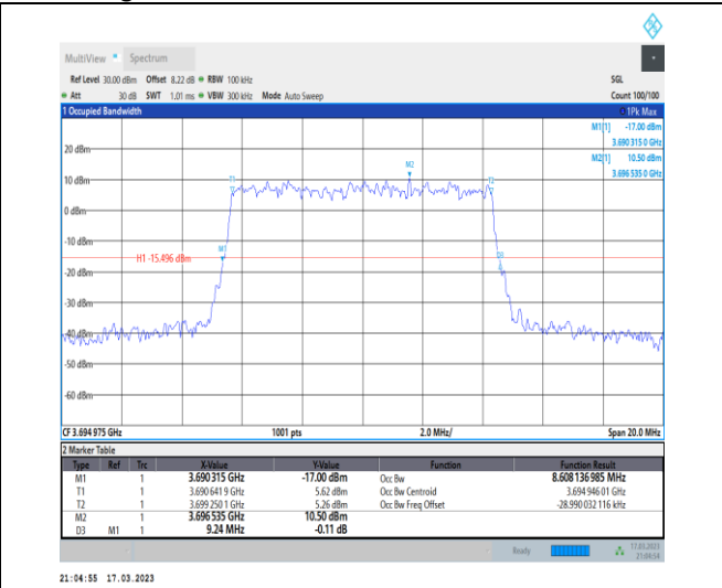
1-N48-PC3-30-10-H-4-DFT-64QAM-Outer_Full-24@ 0-Ant0-8.608-9.240-≤10-PASS
