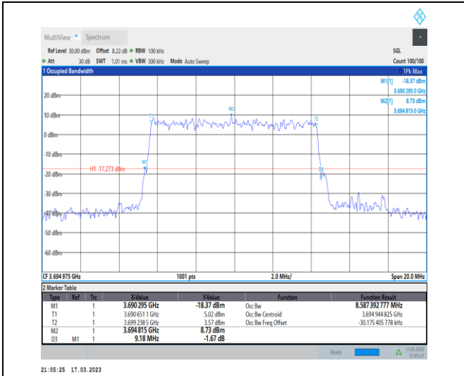
1-N48-PC3-30-10-H-7-CP-16QAM-Outer_Full-24@0 -Ant0-8.587-9.180-≤10-PASS
