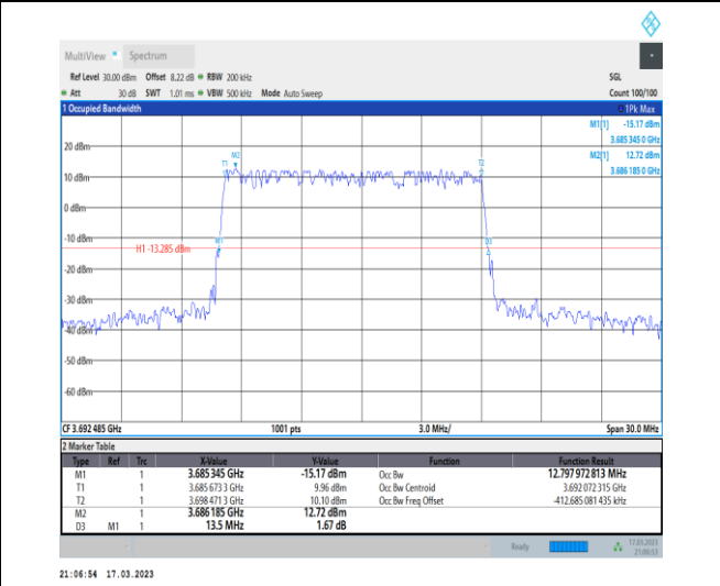
1-N48-PC3-30-15-H-1-DFT-QPSK-Outer_Full-36@0- Ant0-12.798-13.500-≤15-PASS
