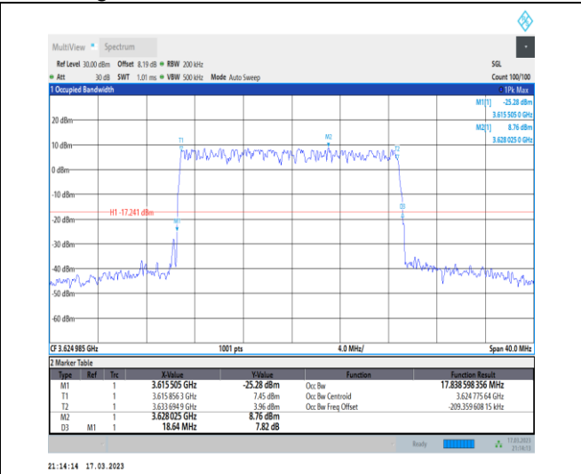
1-N48-PC3-30-20-M-5-DFT-256QAM-Outer_Full-50 @0-Ant0-17.839-18.640-≤20-PASS
