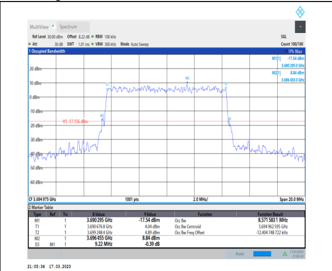
1-N48-PC3-30-10-H-8-CP-64QAM-Outer_Full-24@0 -Ant0-8.572-9.220-≤10-PASS
