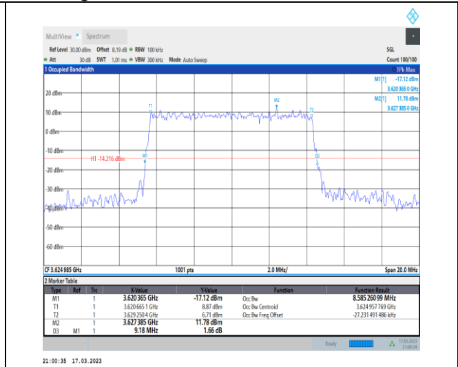
1-N48-PC3-30-10-M-1-DFT-QPSK-Outer_Full-24@ 0-Ant0-8.585-9.180-≤10-PASS
