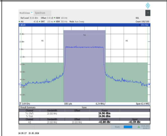
Band48-20MHz-QPSK-56640-100RB#0-PASS
