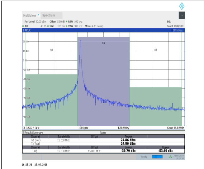
Band48-15MHz-QPSK-55315-1RB#0-PASS
