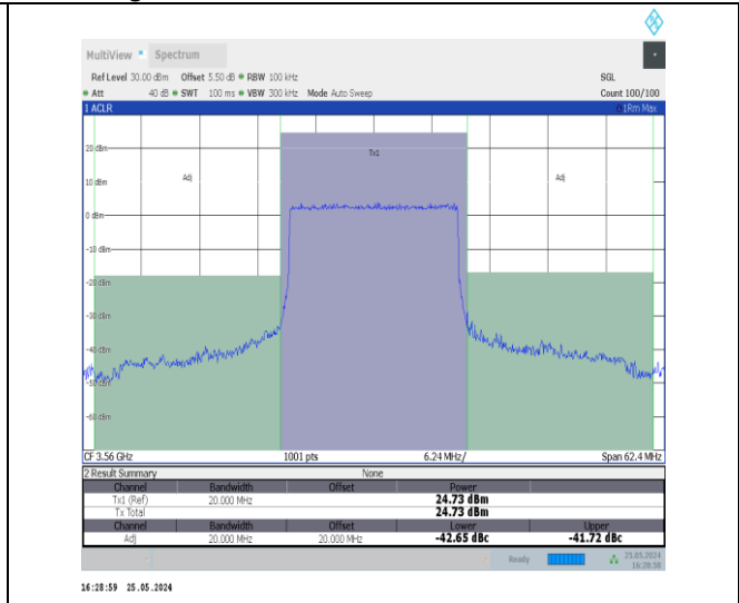
Band48-20MHz-QPSK-55340-100RB#0-PASS
