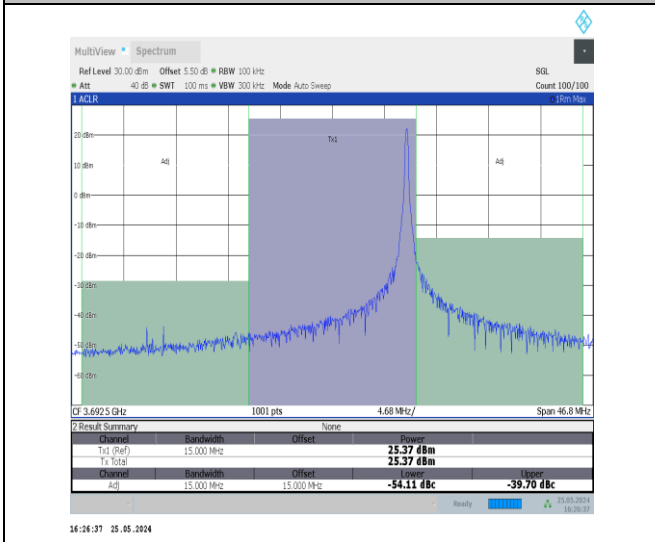
Band48-15MHz-QPSK-56665-1RB#74-PASS
