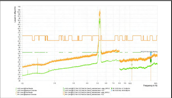
Wi-Fi 5G-11AC80_5530_High
