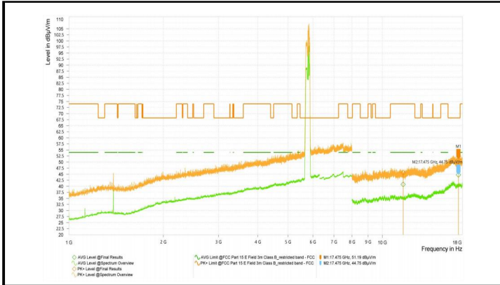
Wi-Fi 5G-11AC80_5290_High
