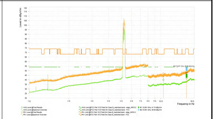
Wi-Fi 5G-11AX40_5310_High
