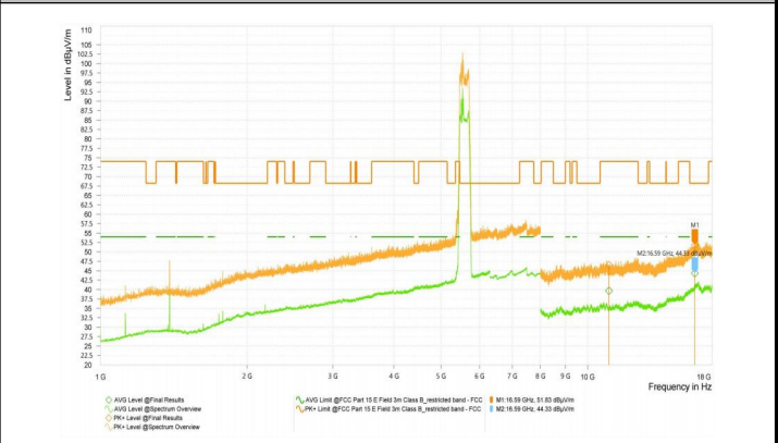
Wi-Fi 5G-11AC80_5690_High
