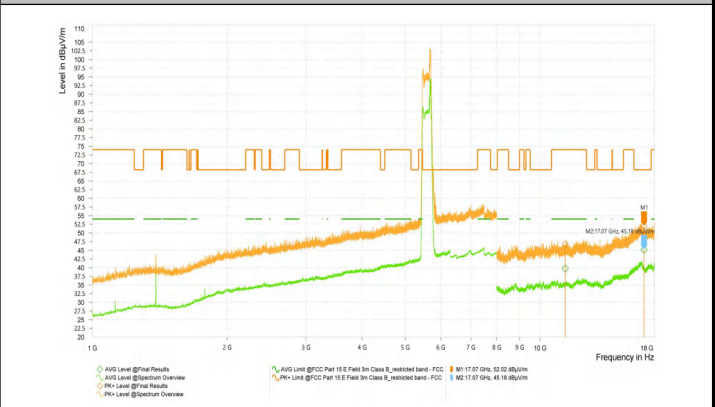
Wi-Fi 5G-11AX20_5180_High
