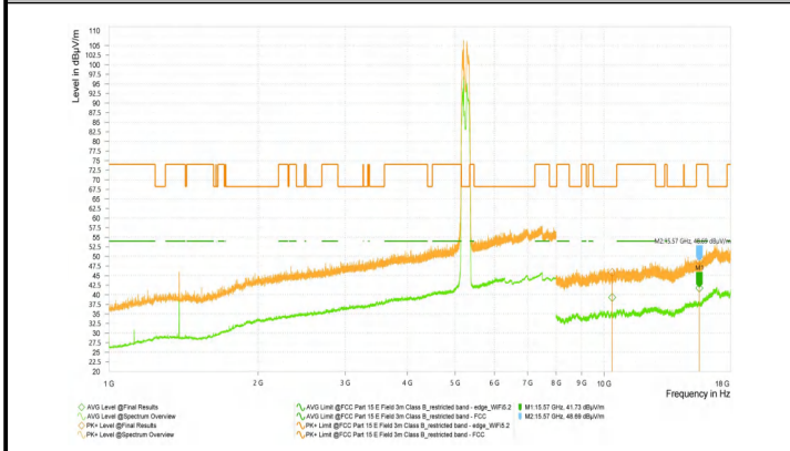
Wi-Fi 5G-11AX40_5270_High
