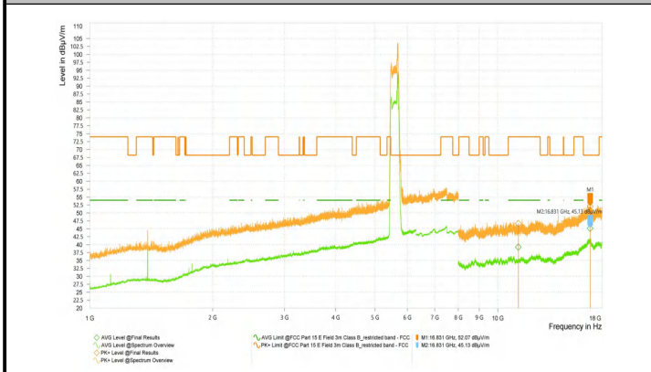
Wi-Fi 5G-11AC80_5775_High
