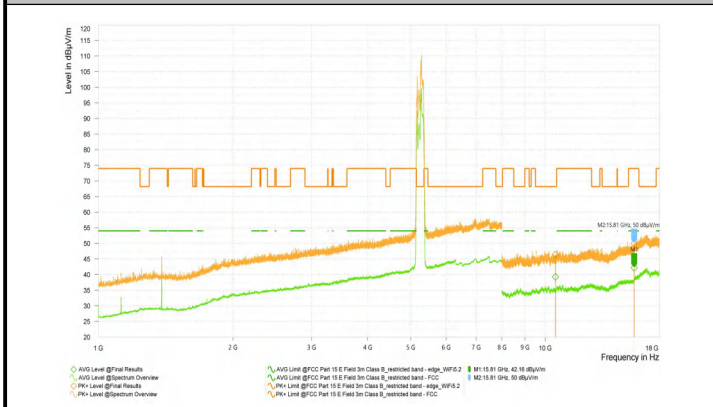
Wi-Fi 5G-11AX40_5510_High
