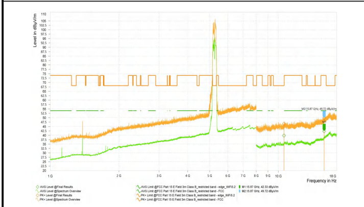
Wi-Fi 5G-11AC80_5610_High
