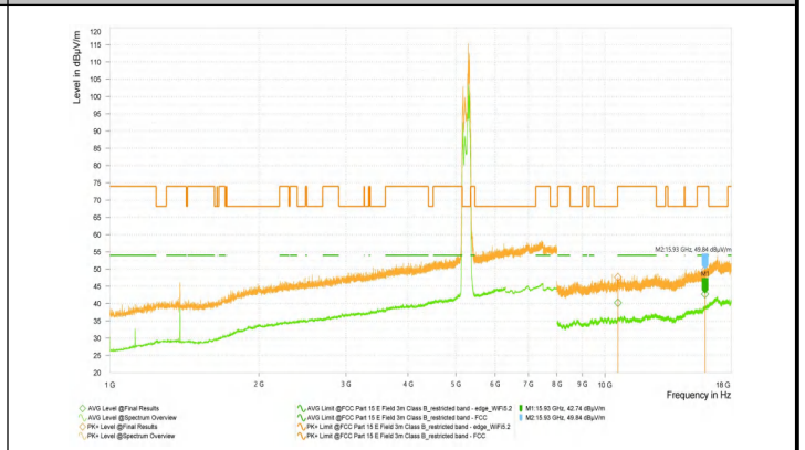
Wi-Fi 5G-11AX40_5550_High
