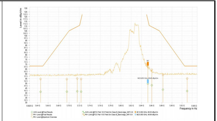
Wi-Fi 5G_11AX20_5825_52Tone_RU40
