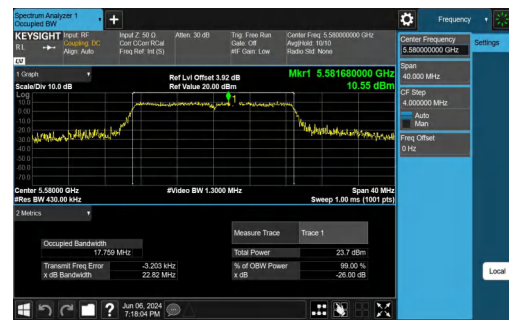
11AC20SISO-Ant1-5580
