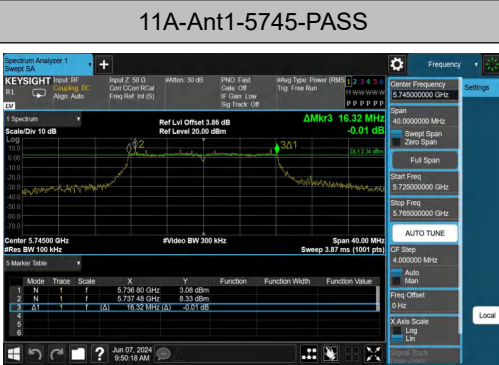
11A-Ant1-5745-PASS
