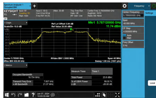
11A-Ant1-5785
