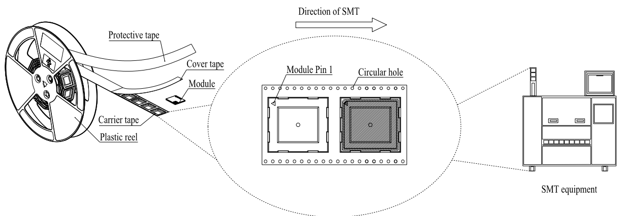
Figure 20: Mounting Direction
