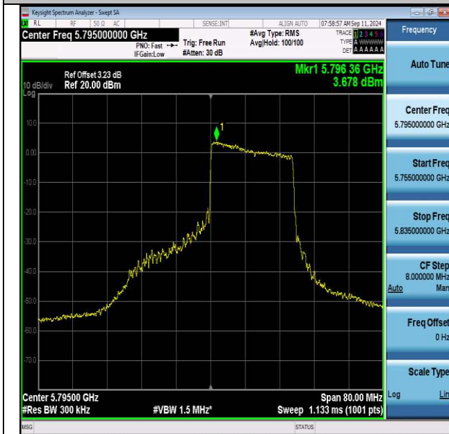
11be40MIMO-Ant1-5795-242Tone-RU62-PASS
