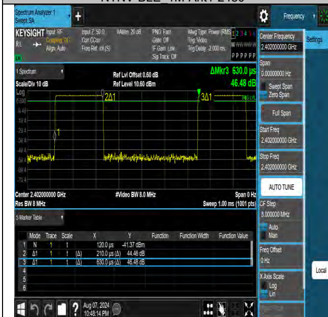
NTNV-BLE 2M-Ant1-2402
