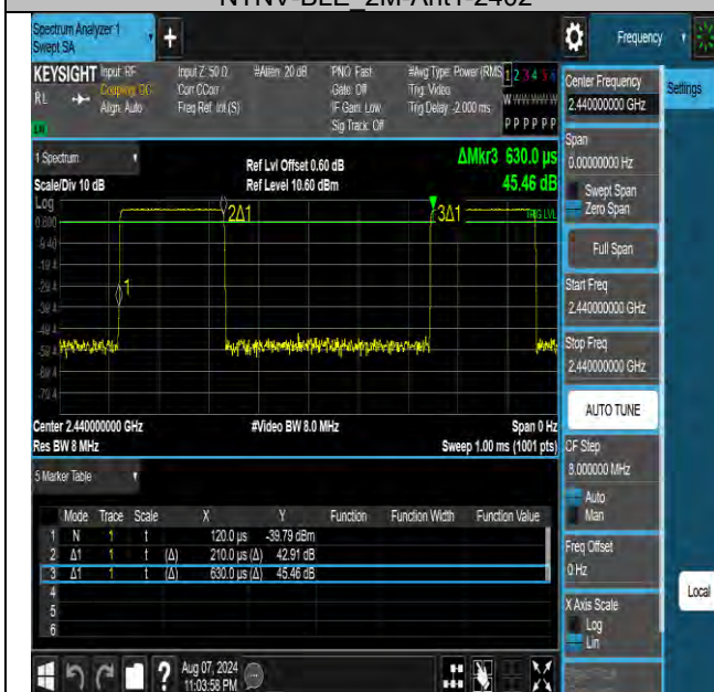
NTNV-BLE 2M-Ant1-2440
