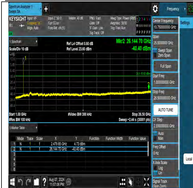
BLE_2M-Ant1-2480-1000~26500-PASS
