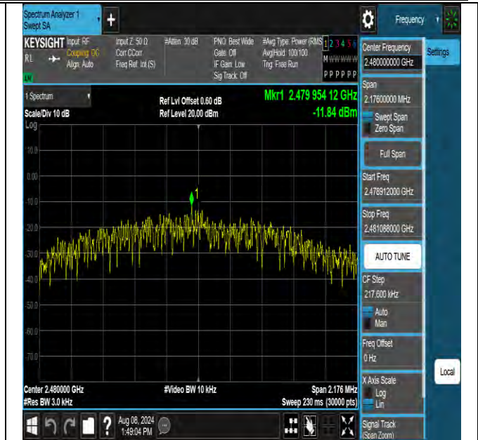
BLE_2M-Ant2-2480-PASS
