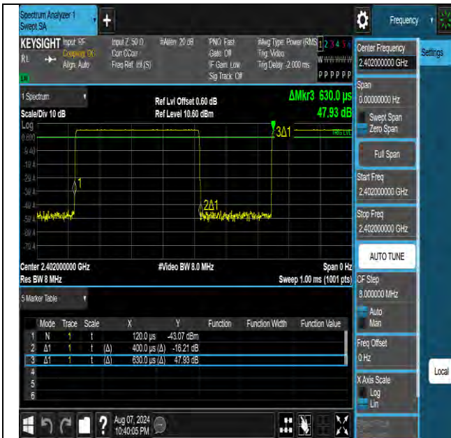
NTVN-BLE_1M-Ant1-2402
