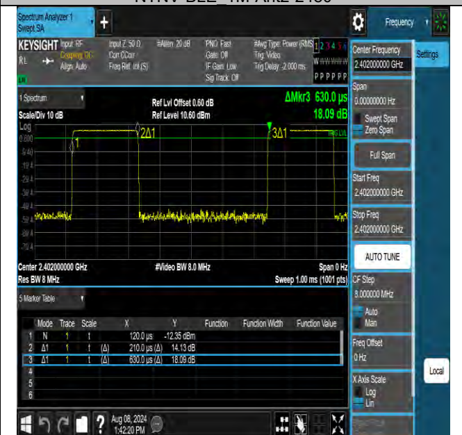
NTNV-BLE 2M-Ant2-2402
