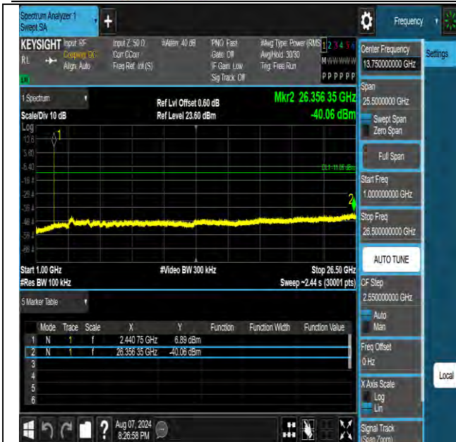
3DH5-Ant1-2441-1000~26500-PASS
