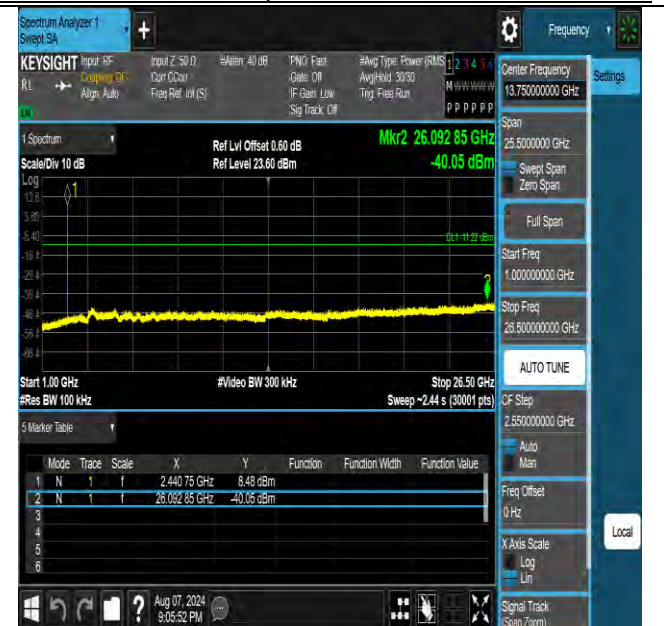
3DH5-Ant2-2441-1000~26500-PASS
