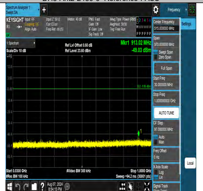
DH5-Ant2-2480-30~1000-PASS
