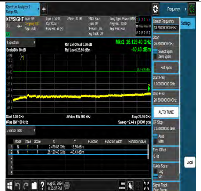
DH5-Ant2-2480-1000~26500-PASS
