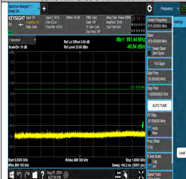
3DH5-Ant1-2480-30~1000-PASS
