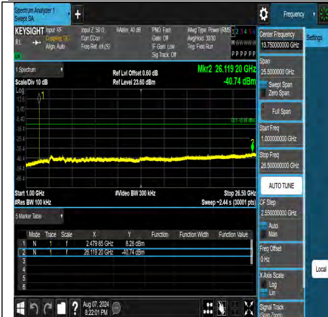
2DH5-Ant1-2480-1000~26500-PASS
