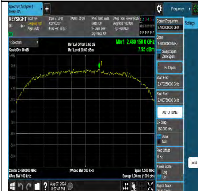
3DH5-Ant1-2480-0~Reference-PASS
