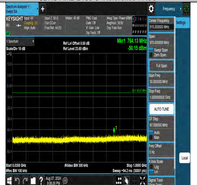
3DH5-Ant2-2480-30~1000-PASS
