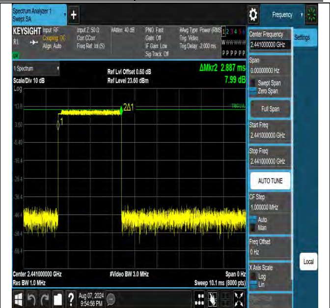
2DH5-Ant2-Hop-PASS
