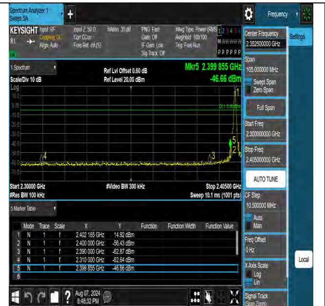
DH5-Ant2-2402-PASS
