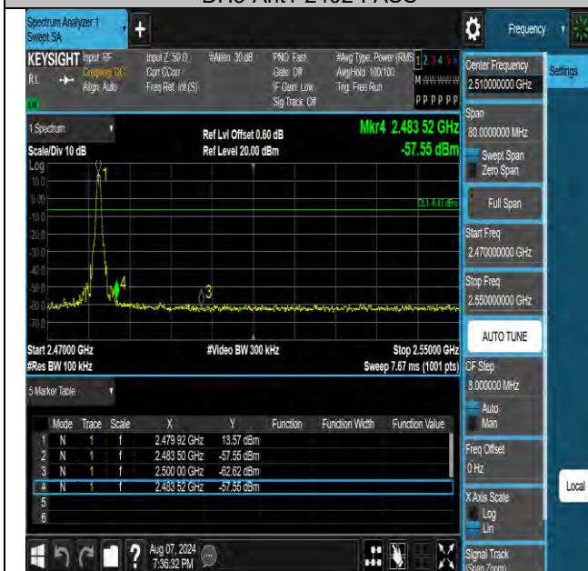
DH5-Ant1-2480-PASS
