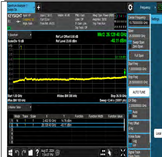
DH5-Ant1-2402-1000~26500-PASS
