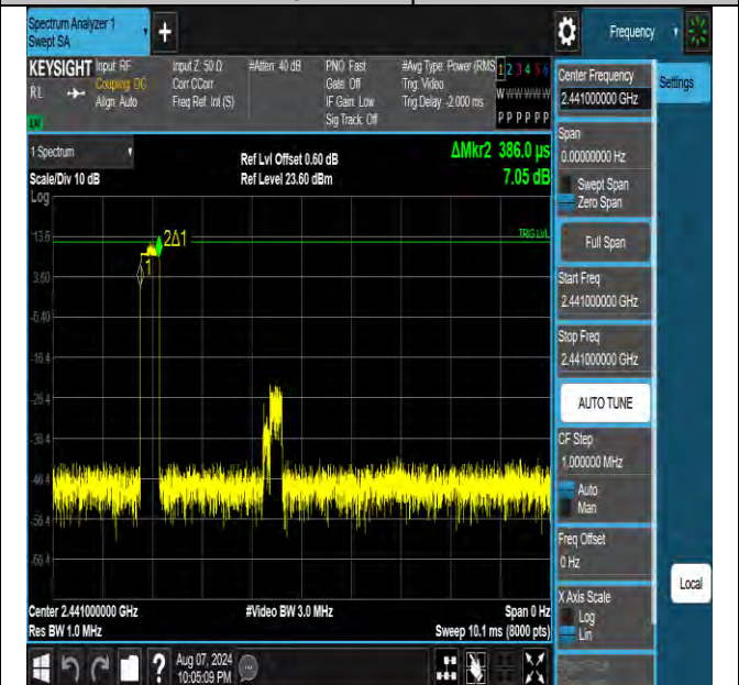
3DH1-Ant2-Hop-PASS
