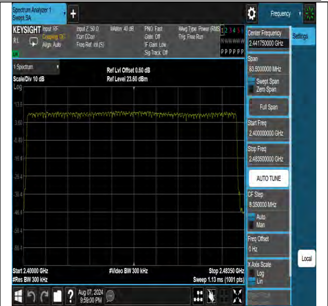
3DH5-Ant2-Hop-PASS
