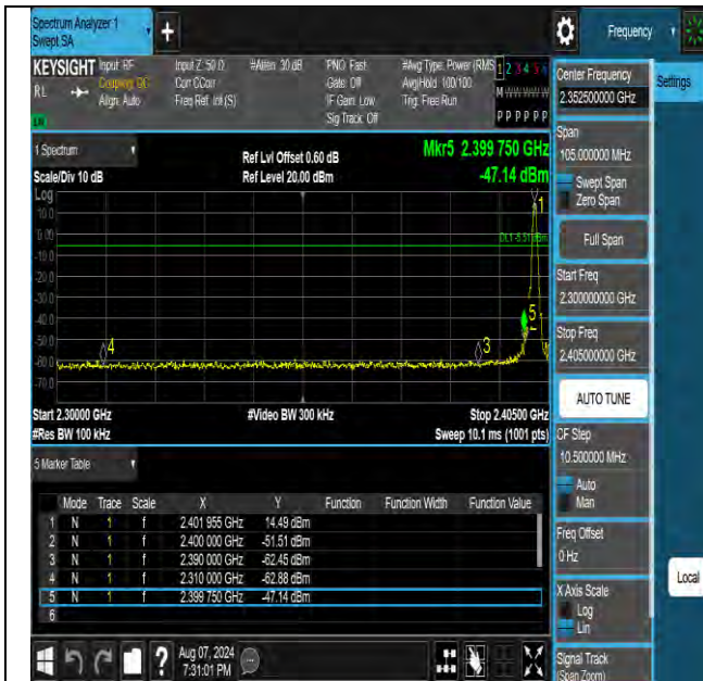
DH5-Ant1-2402-PASS
