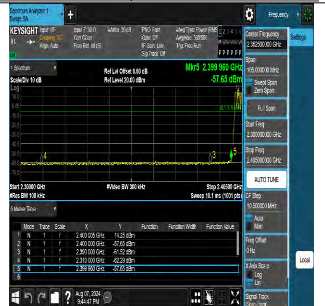
DH5-Ant2-Hop 2402-PASS
