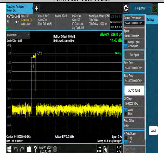
2DH1-Ant2-Hop-PASS
