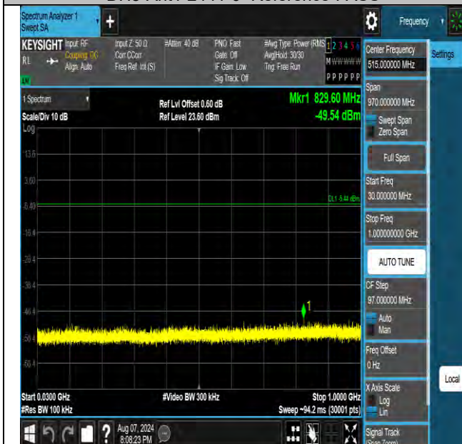
DH5-Ant1-2441-30~1000-PASS
