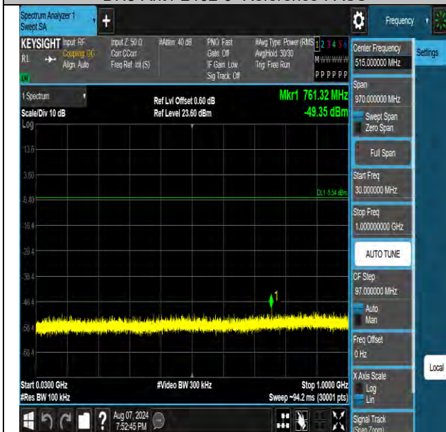
DH5-Ant1-2402-30~1000-PASS
