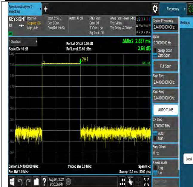
DH5-Ant1-Hop-PASS
