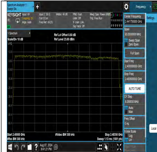
3DH5-Ant1-Hop-PASS
