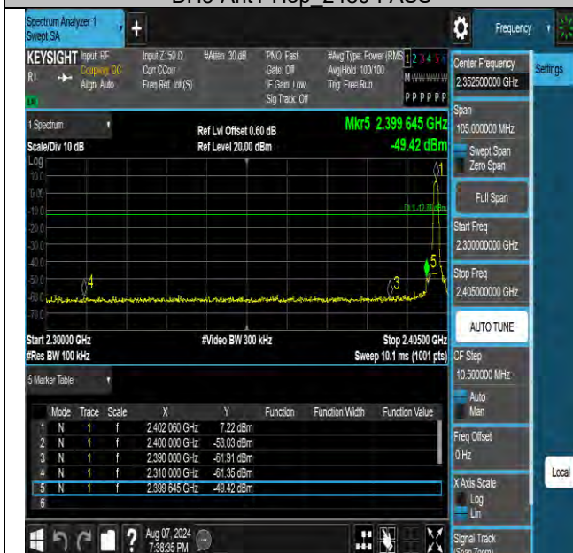
2DH5-Ant1-2402-PASS
