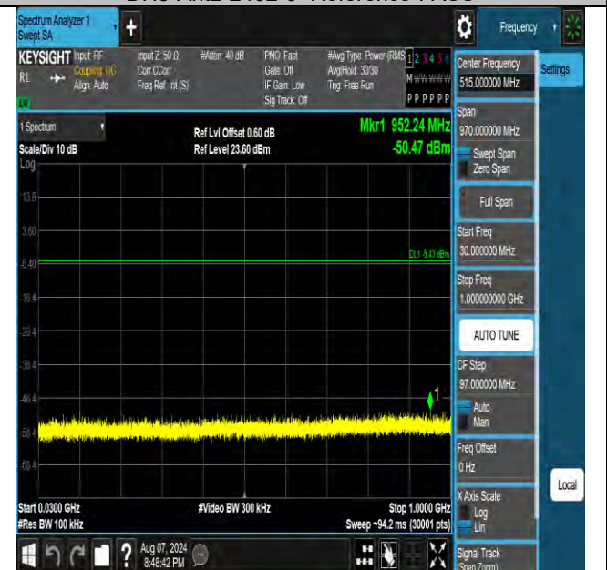
DH5-Ant2-2402-30~1000-PASS
