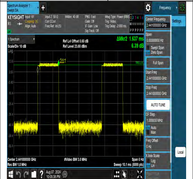
3DH3-Ant2-Hop-PASS
