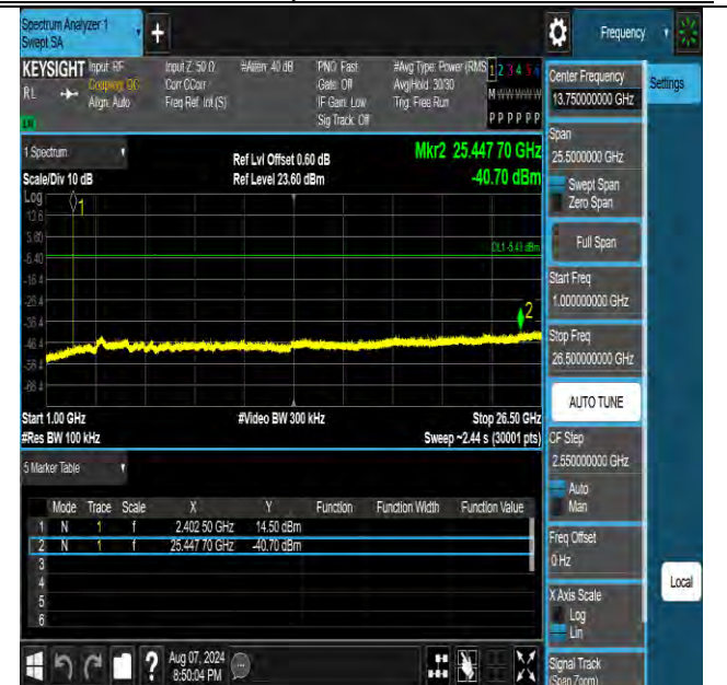
DH5-Ant2-2402-1000~26500-PASS
