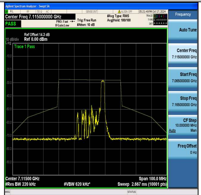
NTNV-11be20MIMO-Ant2-7115-26Tone-RU8-PASS
