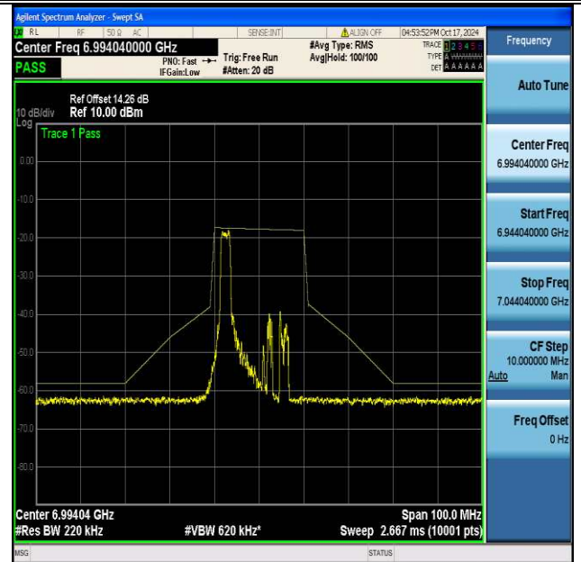
NTVN-11be20MIMO-Ant2-6995-26Tone-RU0-PASS
