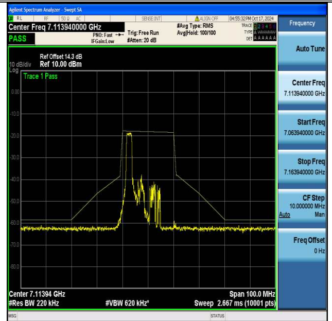
NTNV-11be20MIMO-Ant2-7115-26Tone-RU0-PASS
