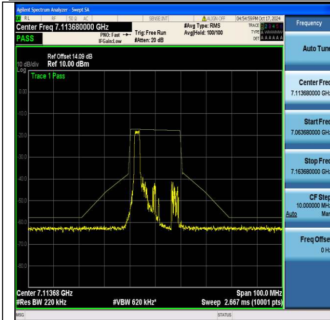
NTNV-11be20MIMO-Ant1-7115-26Tone-RU0-PASS
