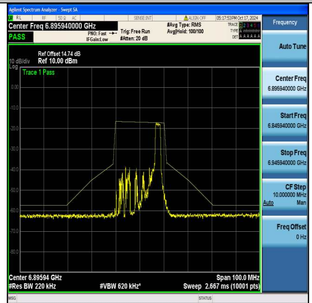
NTVN-11be20MIMO-Ant2-6895-26Tone-RU8-PASS
