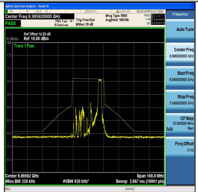
NTVN-11be20MIMO-Ant2-6995-26Tone-RU8-PASS
