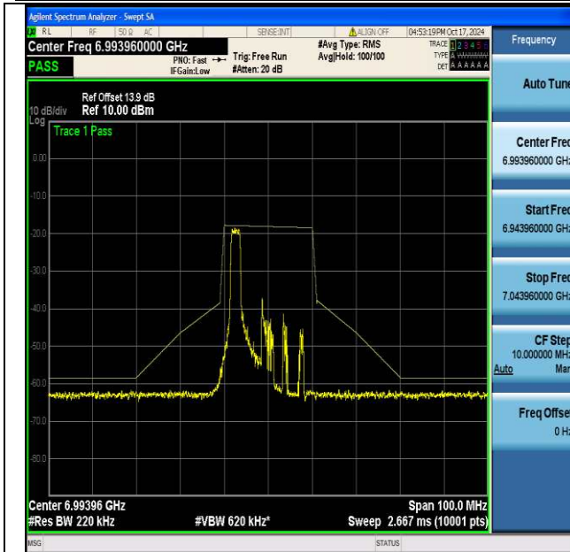
NTVN-11be20MIMO-Ant1-6995-26Tone-RU0-PASS
