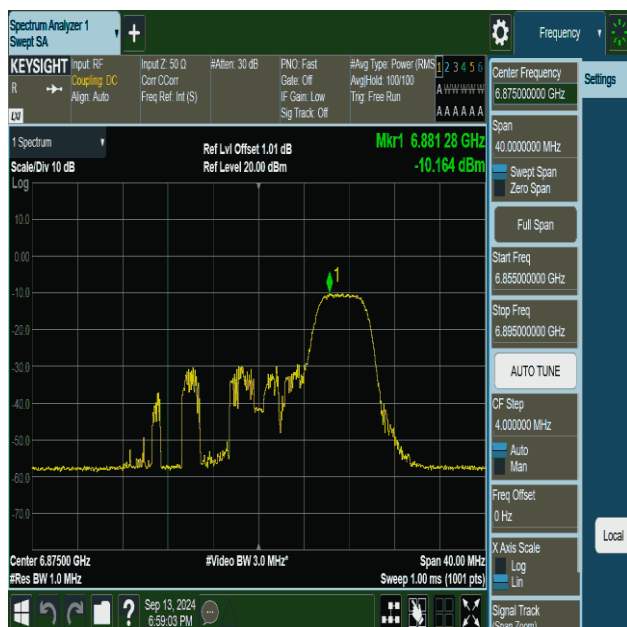
11be20MIMO-Ant1-6875-52Tone-RU40-PASS
