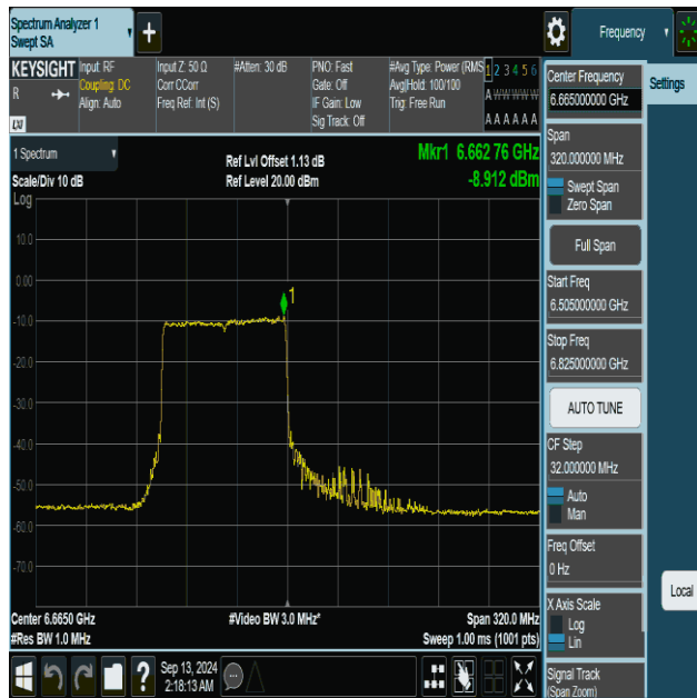
11be160MIMO-Ant1-6665-996Tone-RU67-PASS
