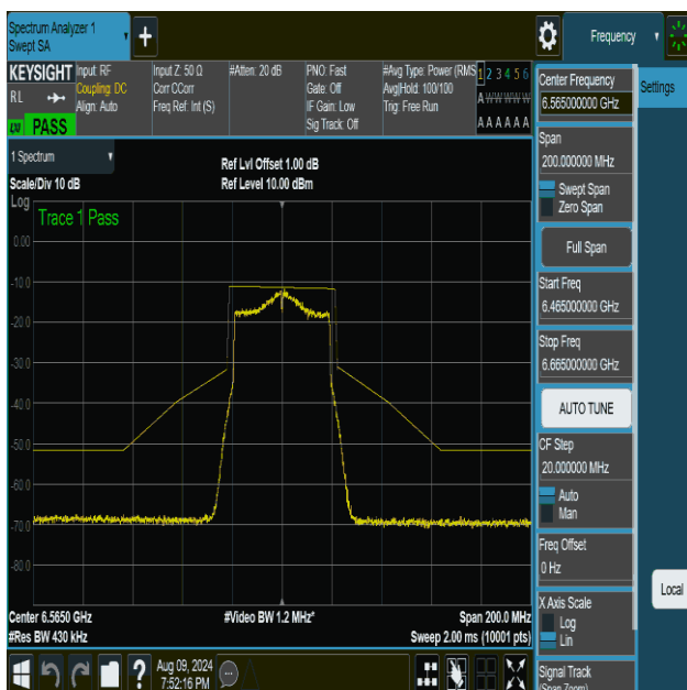
NTVN-11ax40MIMO-Ant1-6565-PASS
