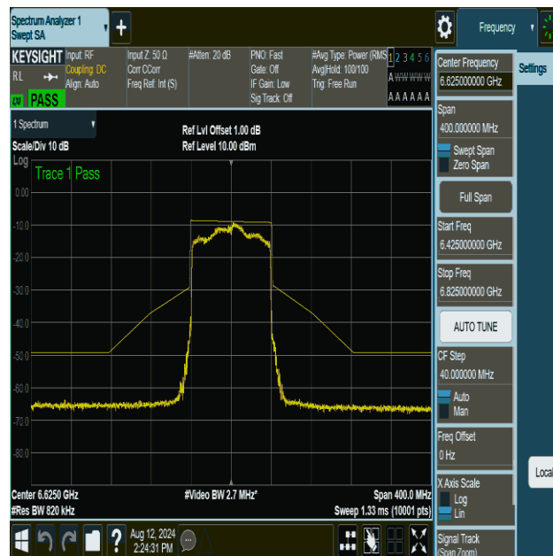
NTNV-11be80MIMO-Ant2-6625-PASS
