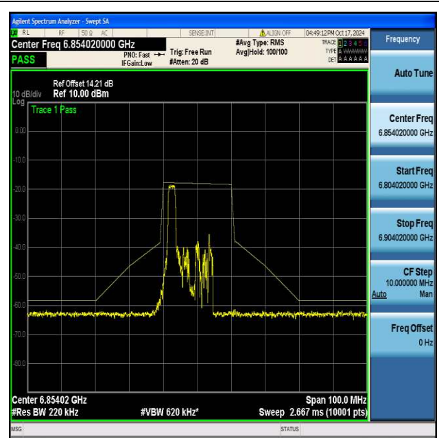
NTNV-11be20MIMO-Ant2-6855-26Tone-RU0-PASS
