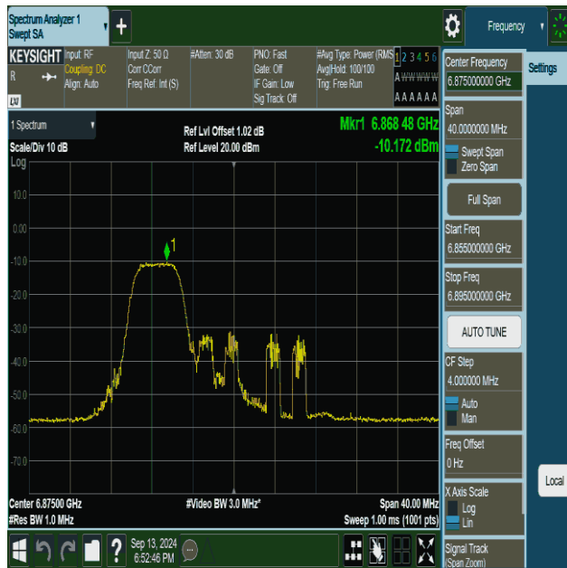
11be20MIMO-Ant1-6875-52Tone-RU37-PASS
