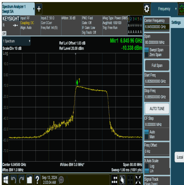
11be40MIMO-Ant1-6845-242Tone-RU62-PASS
