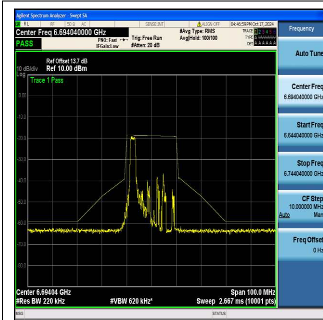
NTNV-11be20MIMO-Ant1-6695-26Tone-RU0-PASS
