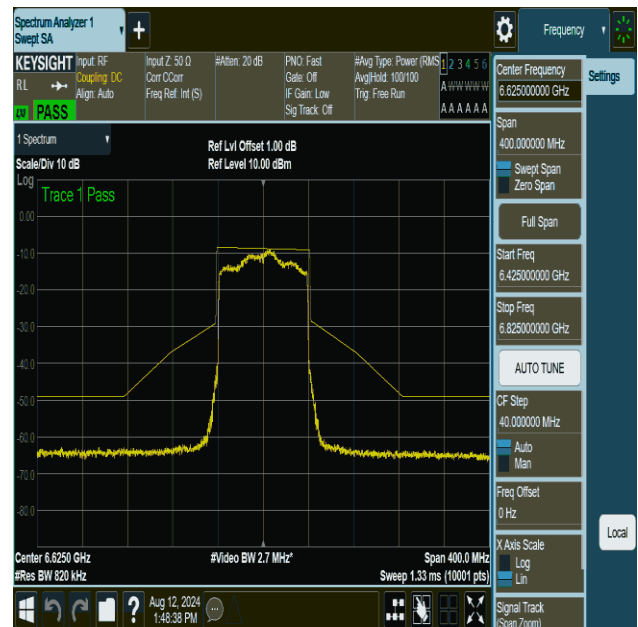
NTVN-11ax80MIMO-Ant2-6625-PASS
