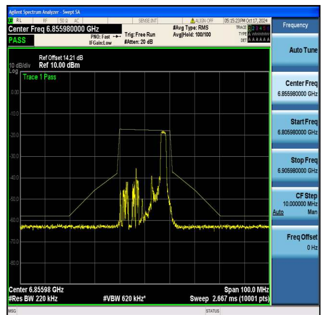
NTNV-11be20MIMO-Ant2-6855-26Tone-RU8-PASS
