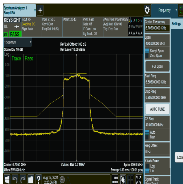
NTNV-11be80MIMO-Ant2-6705-PASS
