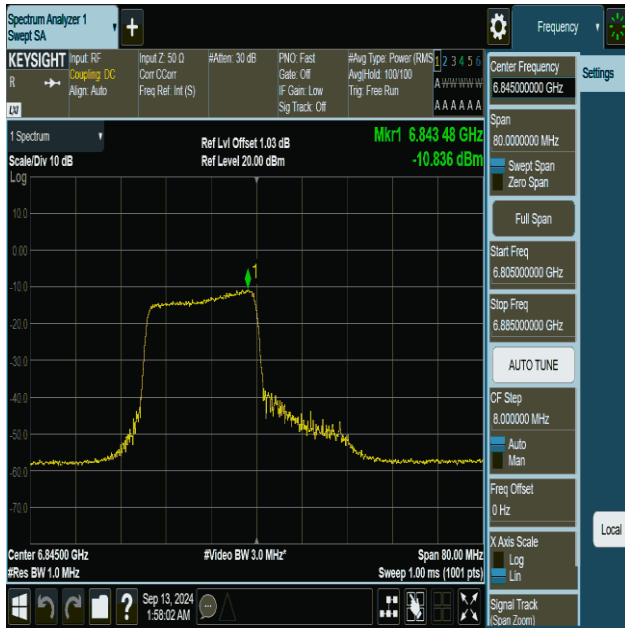
11be40MIMO-Ant1-6845-242Tone-RU61-PASS
