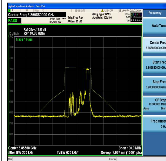
NTNV-11be20MIMO-Ant1-6855-26Tone-RU8-PASS
