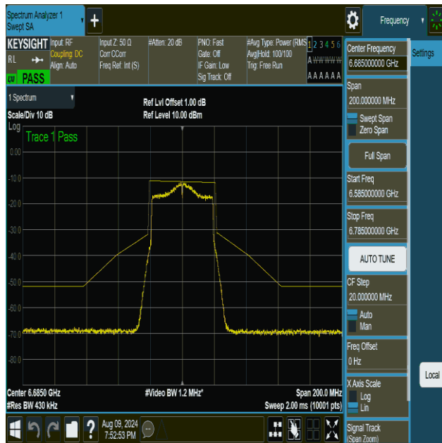
NTVN-11ax40MIMO-Ant1-6685-PASS
