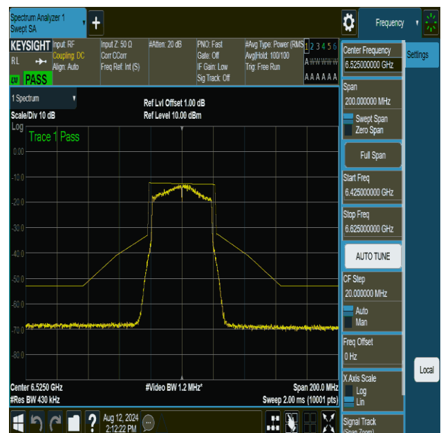
NTVN-11be40MIMO-Ant2-6525-PASS
