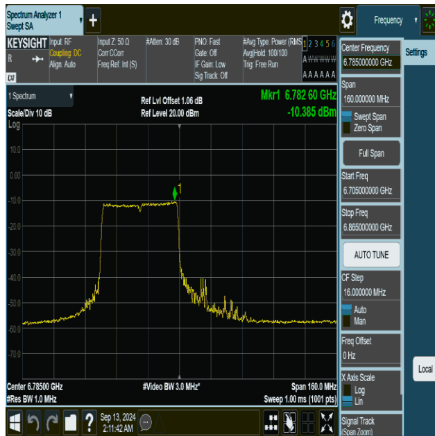
11be80MIMO-Ant1-6785-484Tone-RU65-PASS
