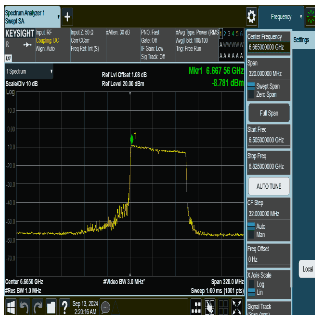
11be160MIMO-Ant1-6665-996Tone-RU68-PASS
