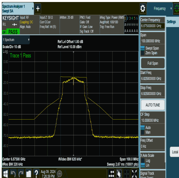
NTNV-11a-CDD-Ant1-6875-PASS
