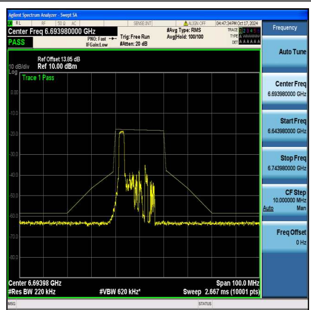
NTNV-11be20MIMO-Ant2-6695-26Tone-RU0-PASS
