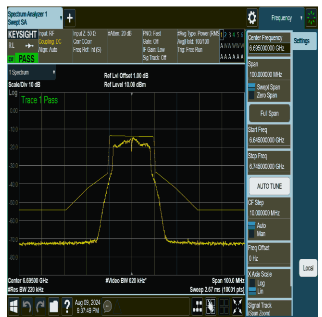
NTNV-11a-CDD-Ant2-6695-PASS
