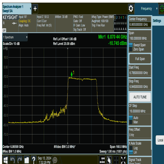
11be80MIMO-Ant1-6865-484Tone-RU66-PASS
