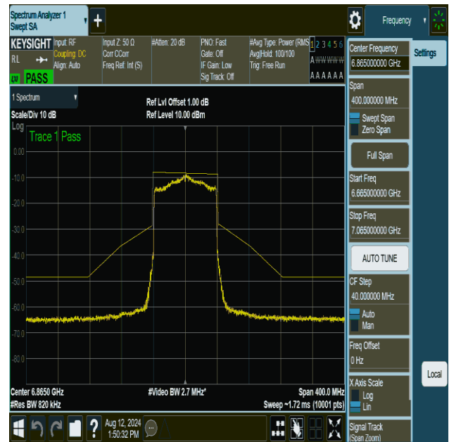
NTVN-11ax80MIMO-Ant2-6865-PASS
