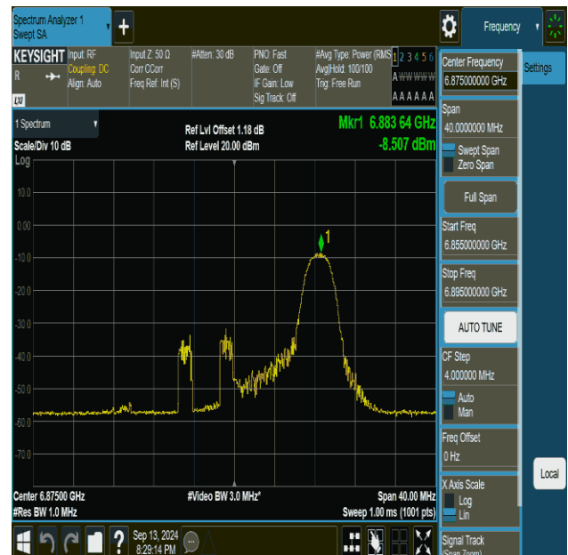
11be20MIMO-Ant2-6875-26Tone-RU8-PASS
