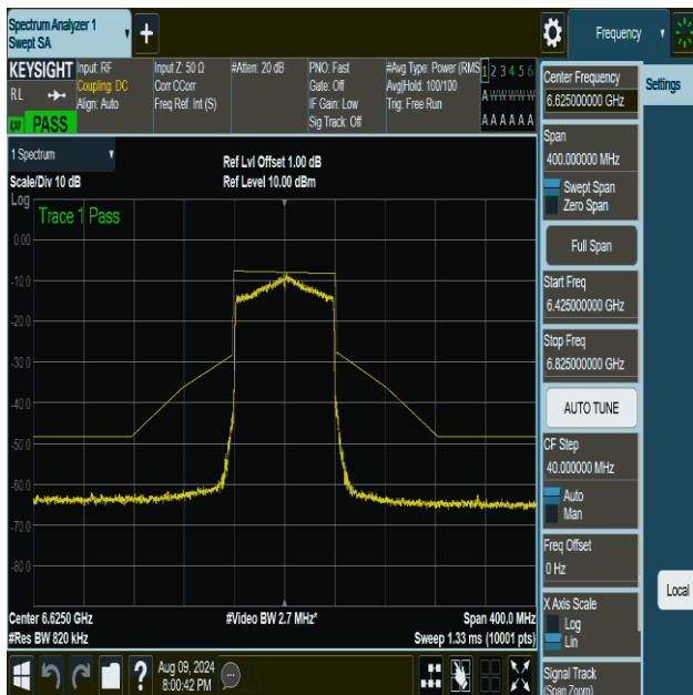
NTVN-11ax80MIMO-Ant1-6625-PASS
