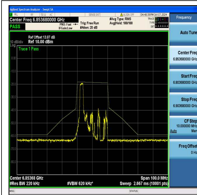
NTNV-11be20MIMO-Ant1-6855-26Tone-RU0-PASS
