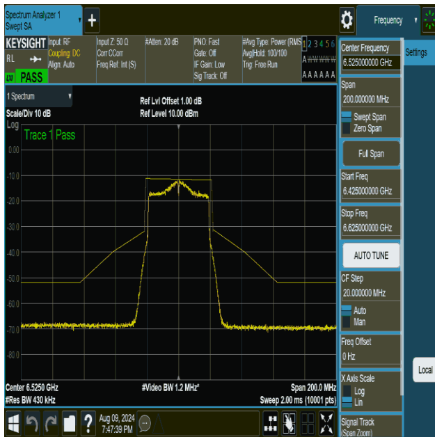
NTVN-11ax40MIMO-Ant1-6525-PASS
