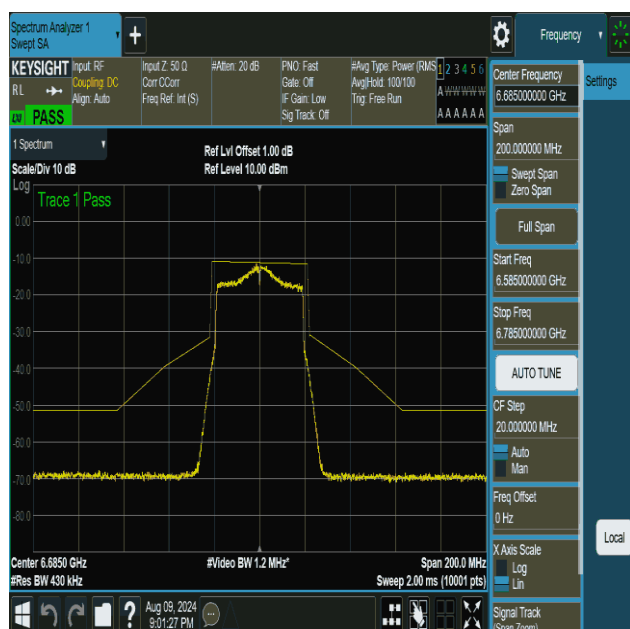
NTNV-11be40MIMO-Ant1-6685-PASS
