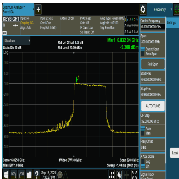
11be160MIMO-Ant1-6825-996Tone-RU68-PASS
