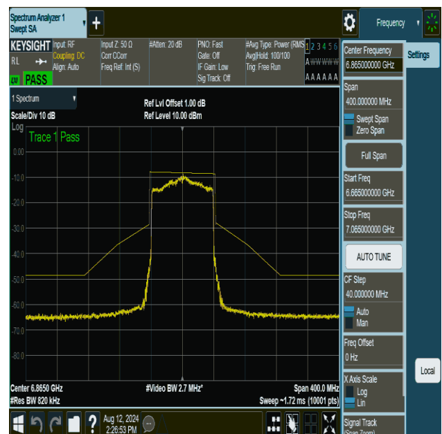
NTVN-11be80MIMO-Ant2-6865-PASS
