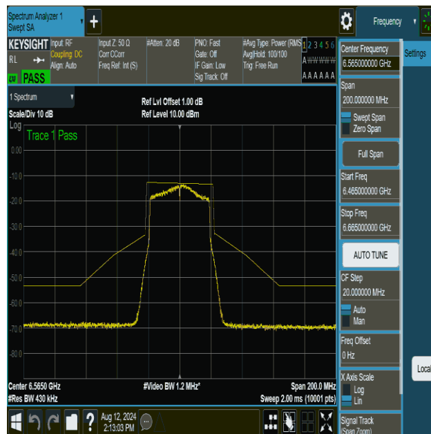
NTNV-11be40MIMO-Ant2-6565-PASS
