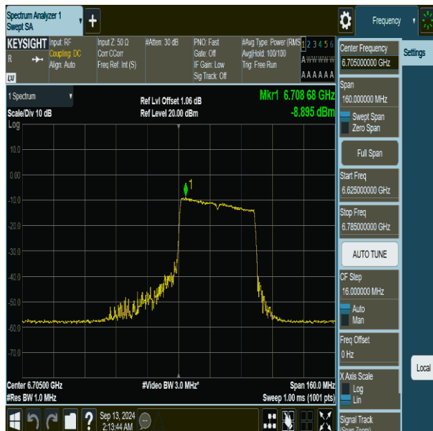
11be80MIMO-Ant1-6705-484Tone-RU66-PASS
