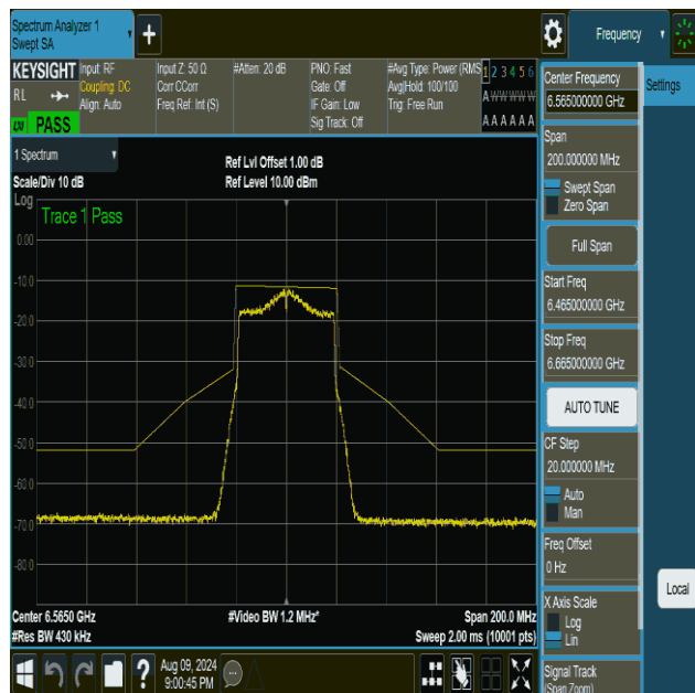
NTNV-11be40MIMO-Ant1-6565-PASS
