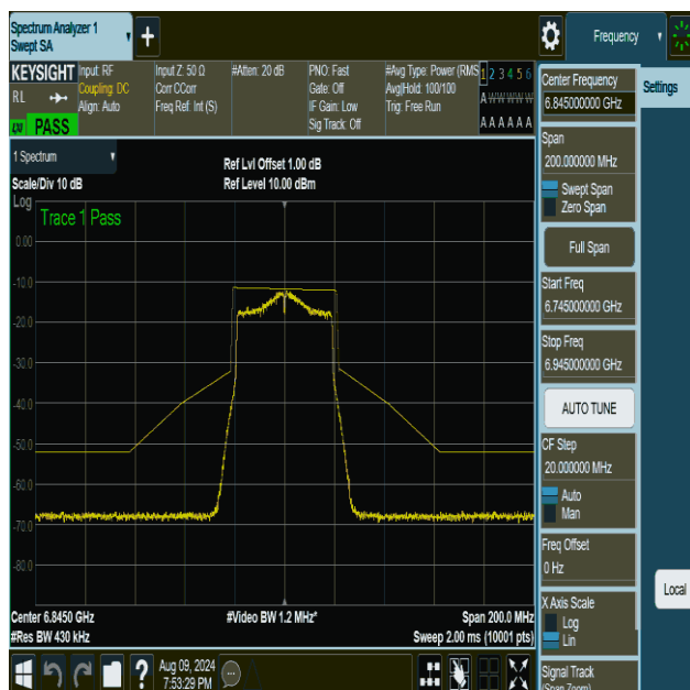
NTVN-11ax40MIMO-Ant1-6845-PASS
