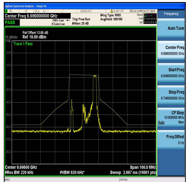
NTNV-11be20MIMO-Ant2-6695-26Tone-RU8-PASS
