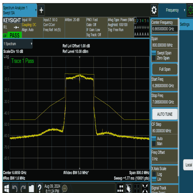
NTVN-11ax160MIMO-Ant1-6665-PASS
