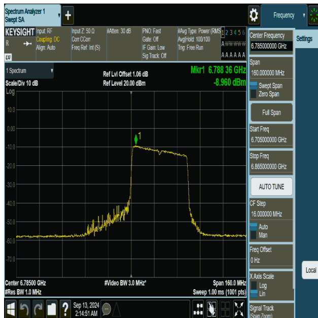
11be80MIMO-Ant1-6785-484Tone-RU66-PASS
