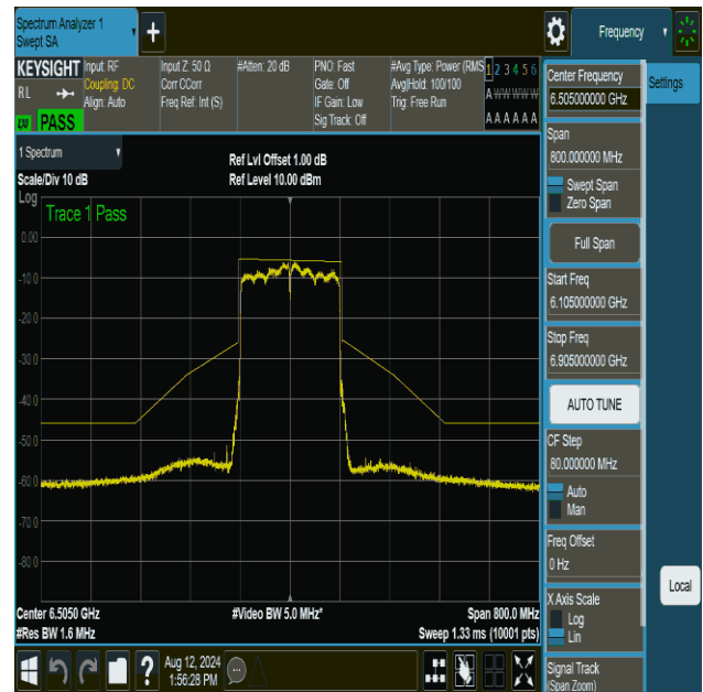
NTVN-11ax160MIMO-Ant2-6505-PASS
