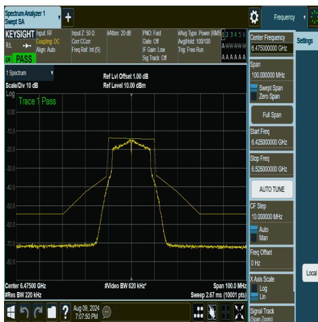
NTNV-11a-CDD-Ant1-6475-PASS
