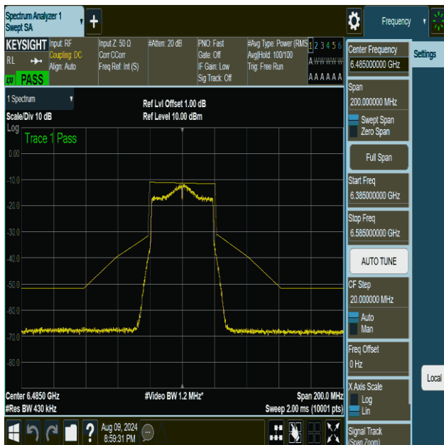
NTVN-11be40MIMO-Ant1-6485-PASS
