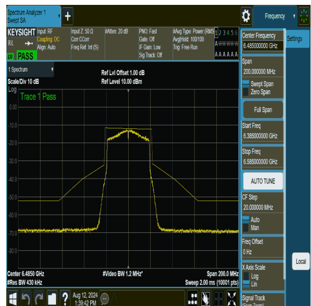
NTVN-11ax40MIMO-Ant2-6485-PASS
