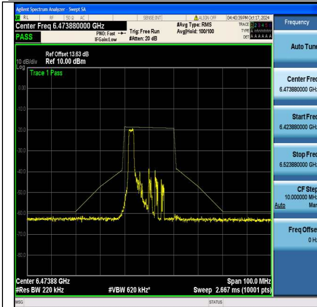
NTVN-11be20MIMO-Ant1-6475-26Tone-RU0-PASS
