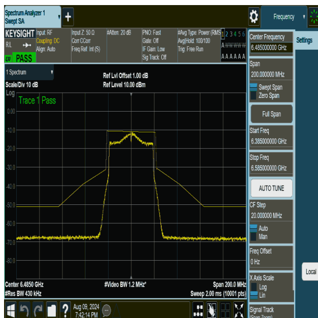
NTVN-11ax40MIMO-Ant1-6485-PASS
