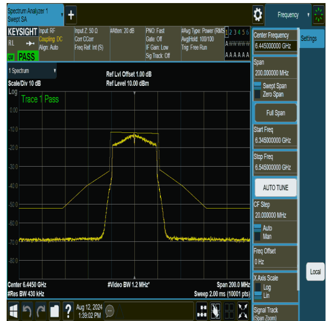
NTVN-11ax40MIMO-Ant2-6445-PASS
