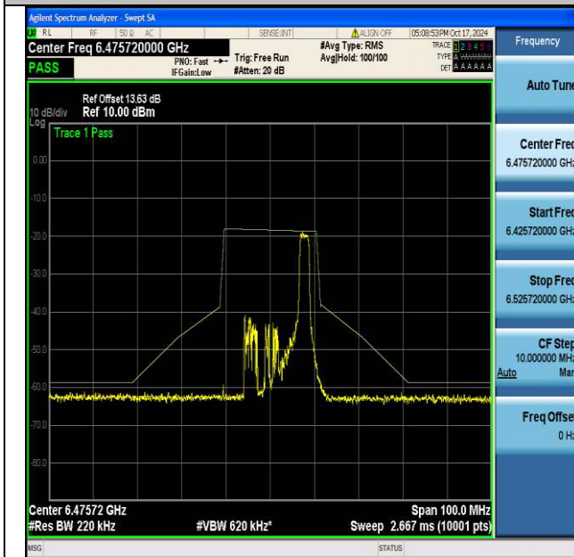
NTVN-11be20MIMO-Ant1-6475-26Tone-RU8-PASS
