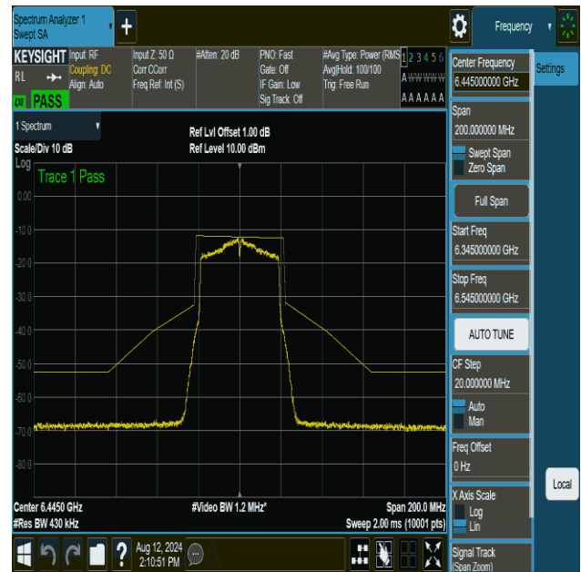
NTVN-11be40MIMO-Ant2-6445-PASS
