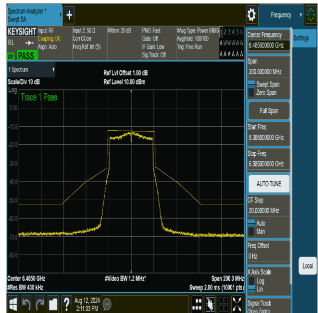
NTVN-11be40MIMO-Ant2-6485-PASS
