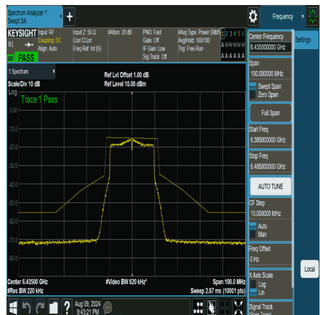
NTVN-11ax20MIMO-Ant2-6435-PASS
