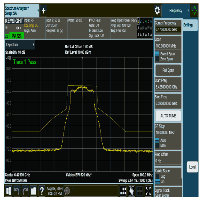
NTNV-11a-CDD-Ant2-6475-PASS
