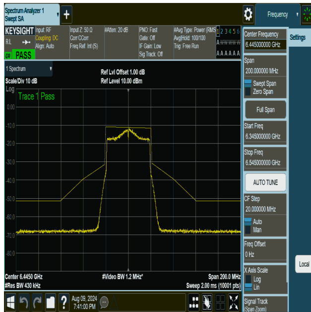
NTVN-11ax40MIMO-Ant1-6445-PASS
