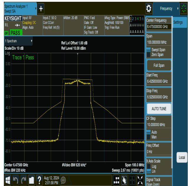
NTNV-11be20MIMO-Ant2-6475-PASS
