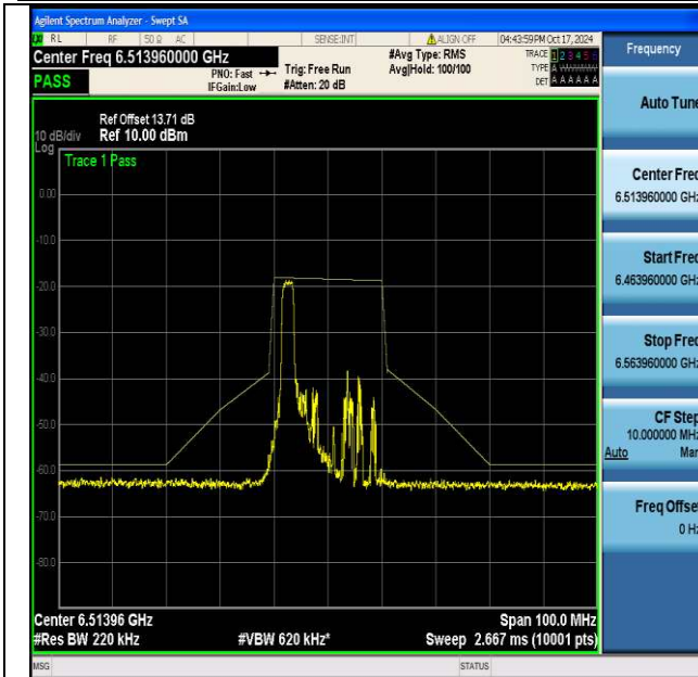
NTVN-11be20MIMO-Ant1-6515-26Tone-RU0-PASS
