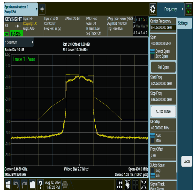
NTVN-11ax80MIMO-Ant2-6465-PASS
