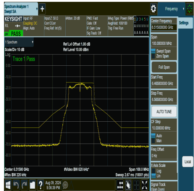
NTVN-11a-CDD-Ant2-6515-PASS
