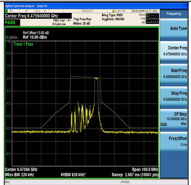
NTVN-11be20MIMO-Ant2-6475-26Tone-RU8-PASS
