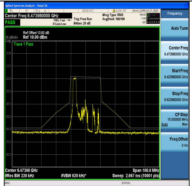
NTVN-11be20MIMO-Ant2-6475-26Tone-RU0-PASS
