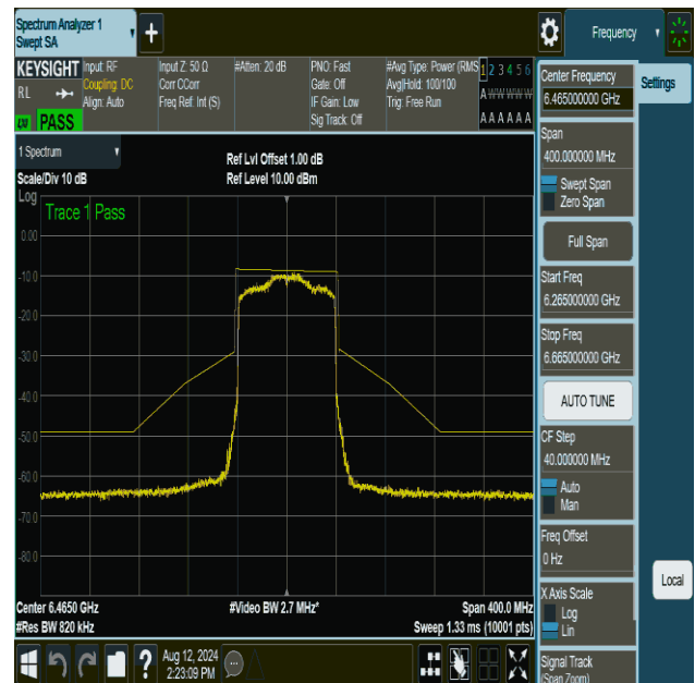
NTVN-11be80MIMO-Ant2-6465-PASS
