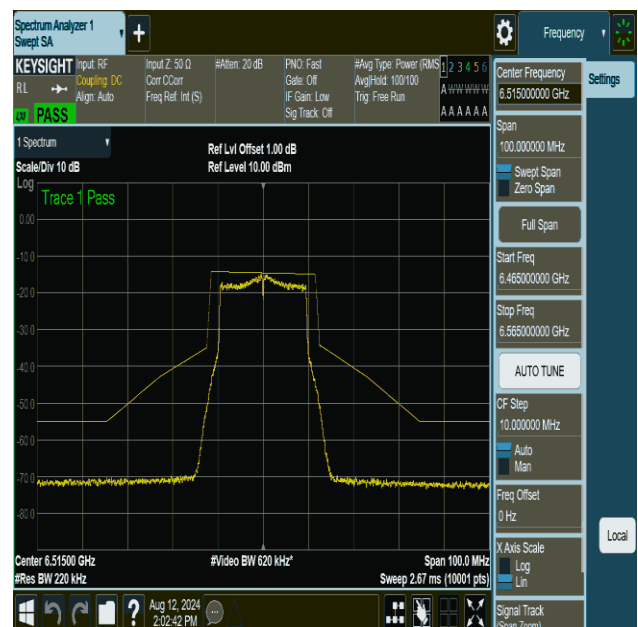
NTNV-11be20MIMO-Ant2-6515-PASS
