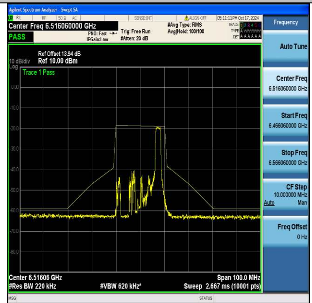
NTVN-11be20MIMO-Ant2-6515-26Tone-RU8-PASS
