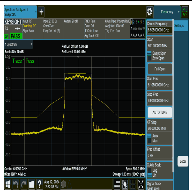
NTNV-11be160MIMO-Ant2-6505-PASS
