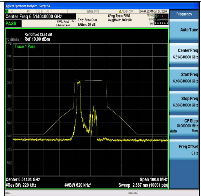
NTVN-11be20MIMO-Ant2-6515-26Tone-RU0-PASS
