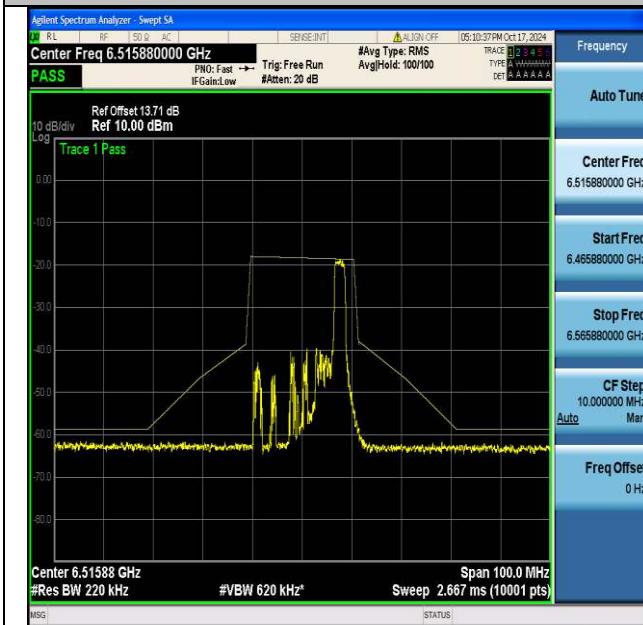
NTVN-11be20MIMO-Ant1-6515-26Tone-RU8-PASS
