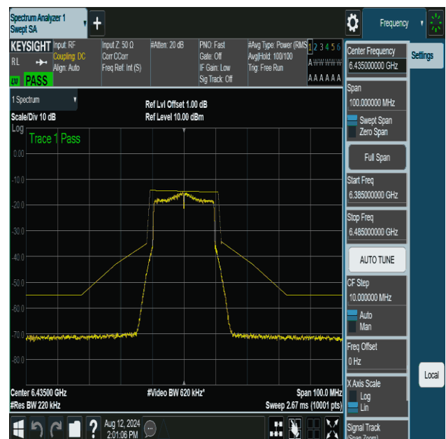
NTVN-11be20MIMO-Ant2-6435-PASS
