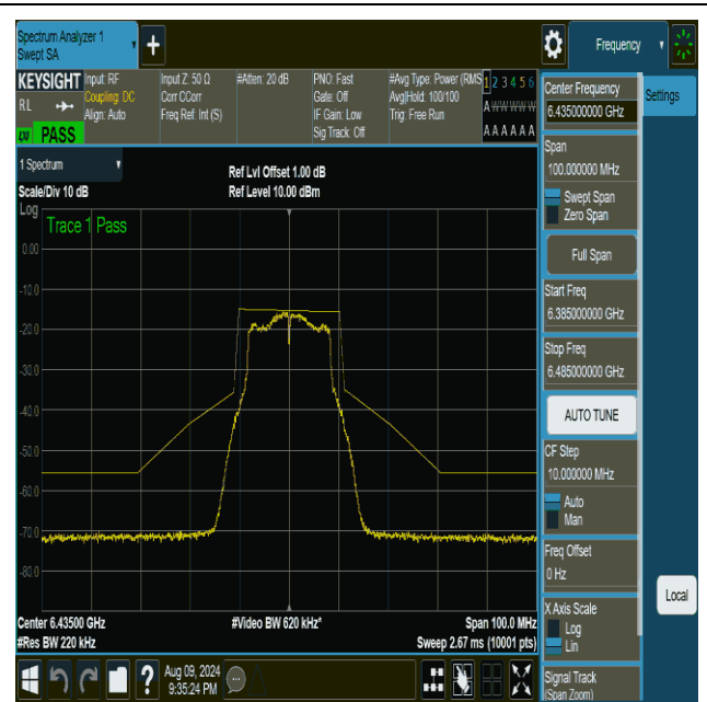
NTNV-11a-CDD-Ant2-6435-PASS
