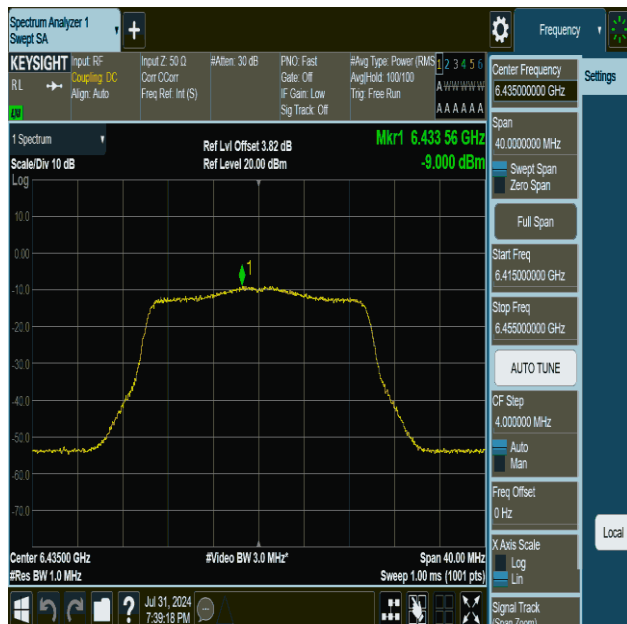
11ax20MIMO-Ant1-6435-PASS
