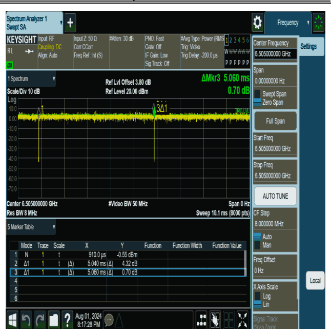
NTNV-11be160MIMO-Ant2-6505
