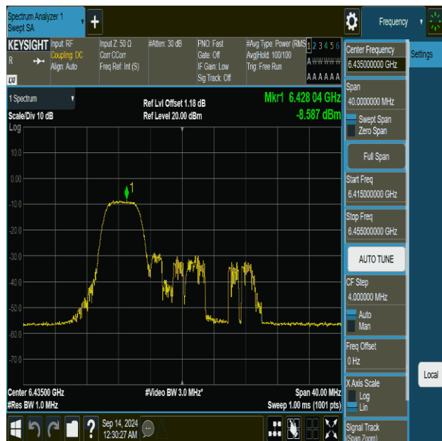
11be20MIMO-Ant2-6435-52Tone-RU37-PASS
