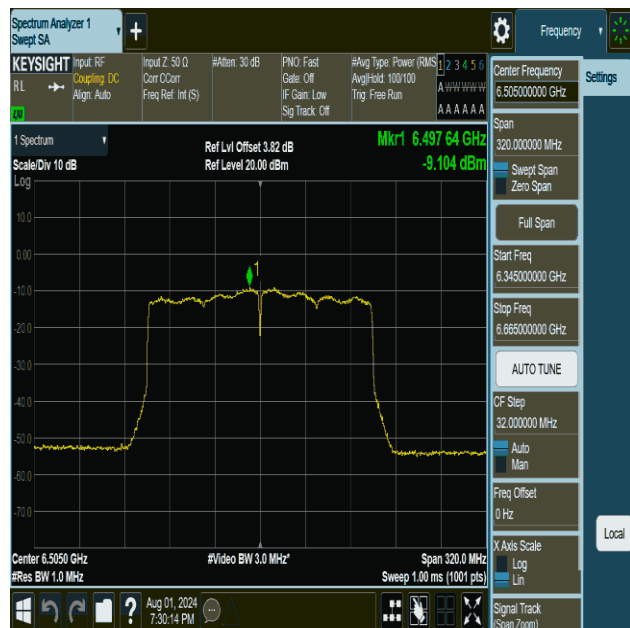
11ax160MIMO-Ant2-6505-PASS
