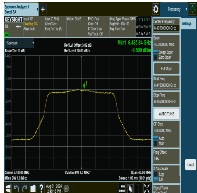
11ax20MIMO-Ant2-6435-PASS
