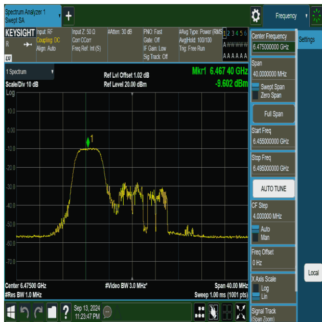
11be20MIMO-Ant1-6475-52Tone-RU37-PASS
