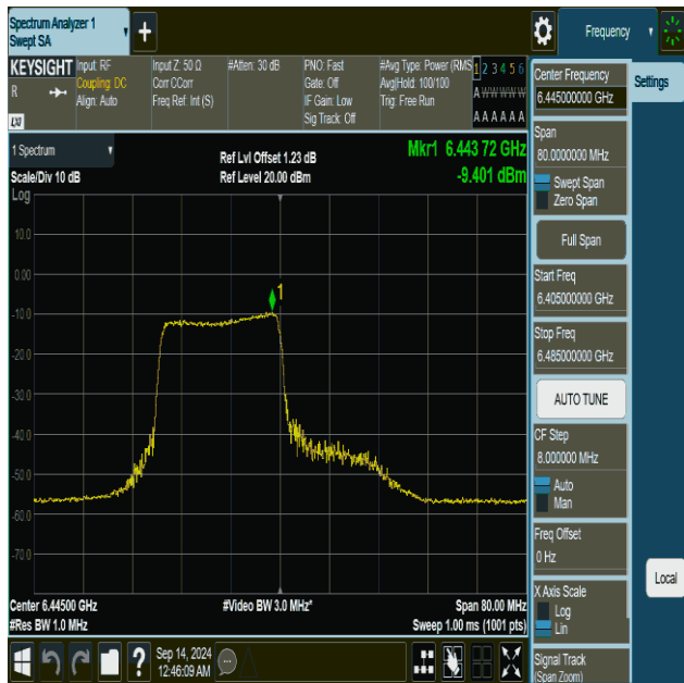
11be40MIMO-Ant1-6445-242Tone-RU61-PASS
