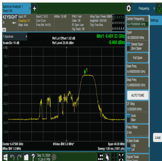
11be20MIMO-Ant1-6475-52Tone-RU40-PASS
