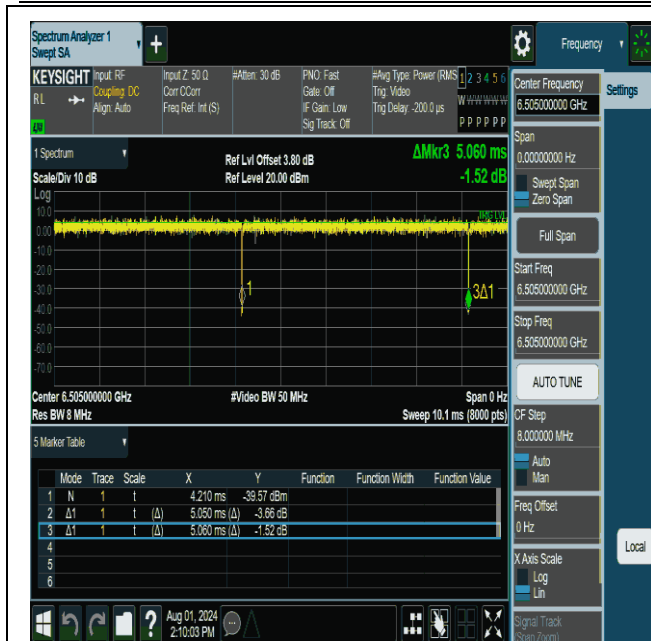
NTNV-11be160MIMO-Ant1-6505
