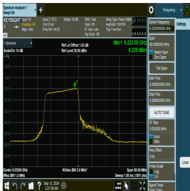
11be40MIMO-Ant2-6525-242Tone-RU61-PASS
