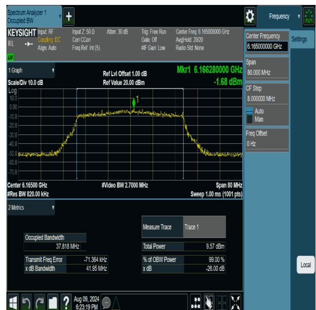
11be40MIMO-Ant2-6165-PASS
