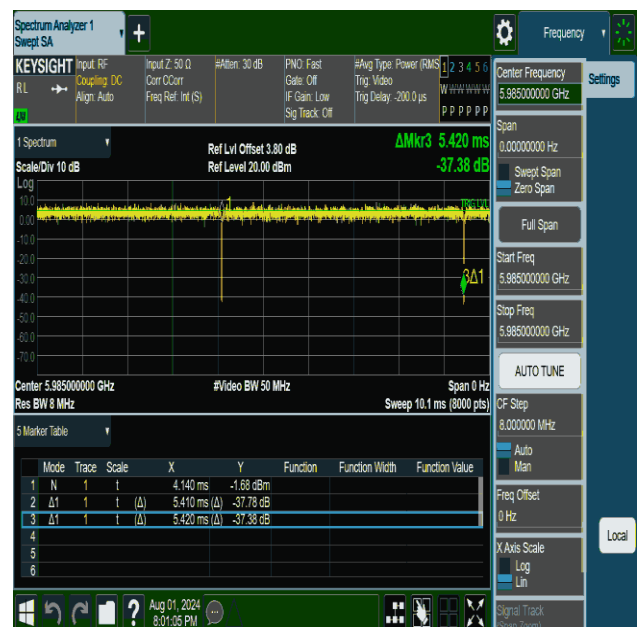
NTNV-11be80MIMO-Ant2-5985
