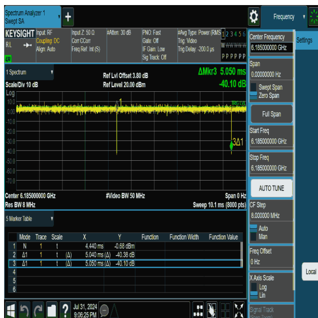
NTNV-11ax160MIMO-Ant1-6185
