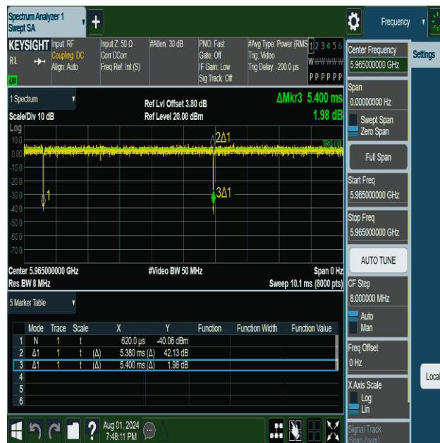
NTNV-11be40MIMO-Ant2-5965
