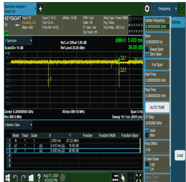
NTNV-11be80MIMO-Ant2-6385
