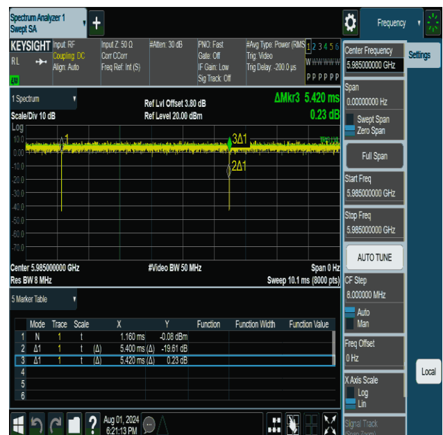
NTNV-11ax80MIMO-Ant2-5985
