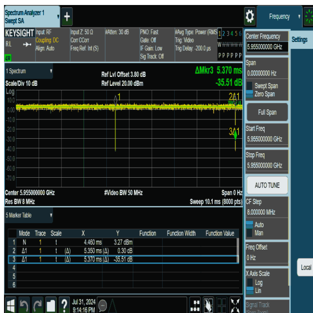
NTVN-11be20MIMO-Ant1-5955
