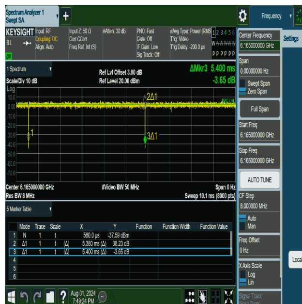
NTNV-11be40MIMO-Ant2-6165
