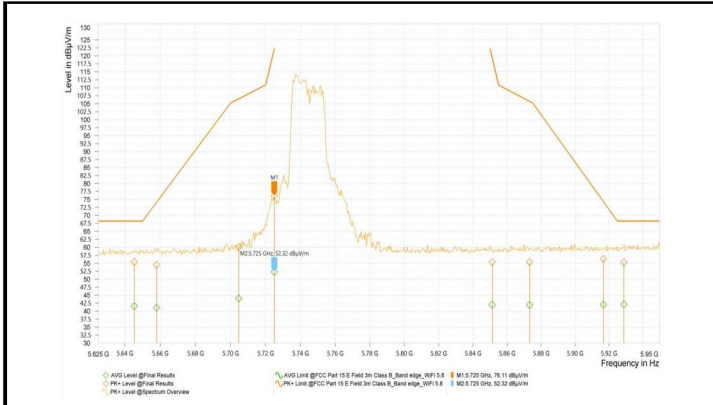
Wi-Fi 5G_11AX20_5745_52Tone_RU37
